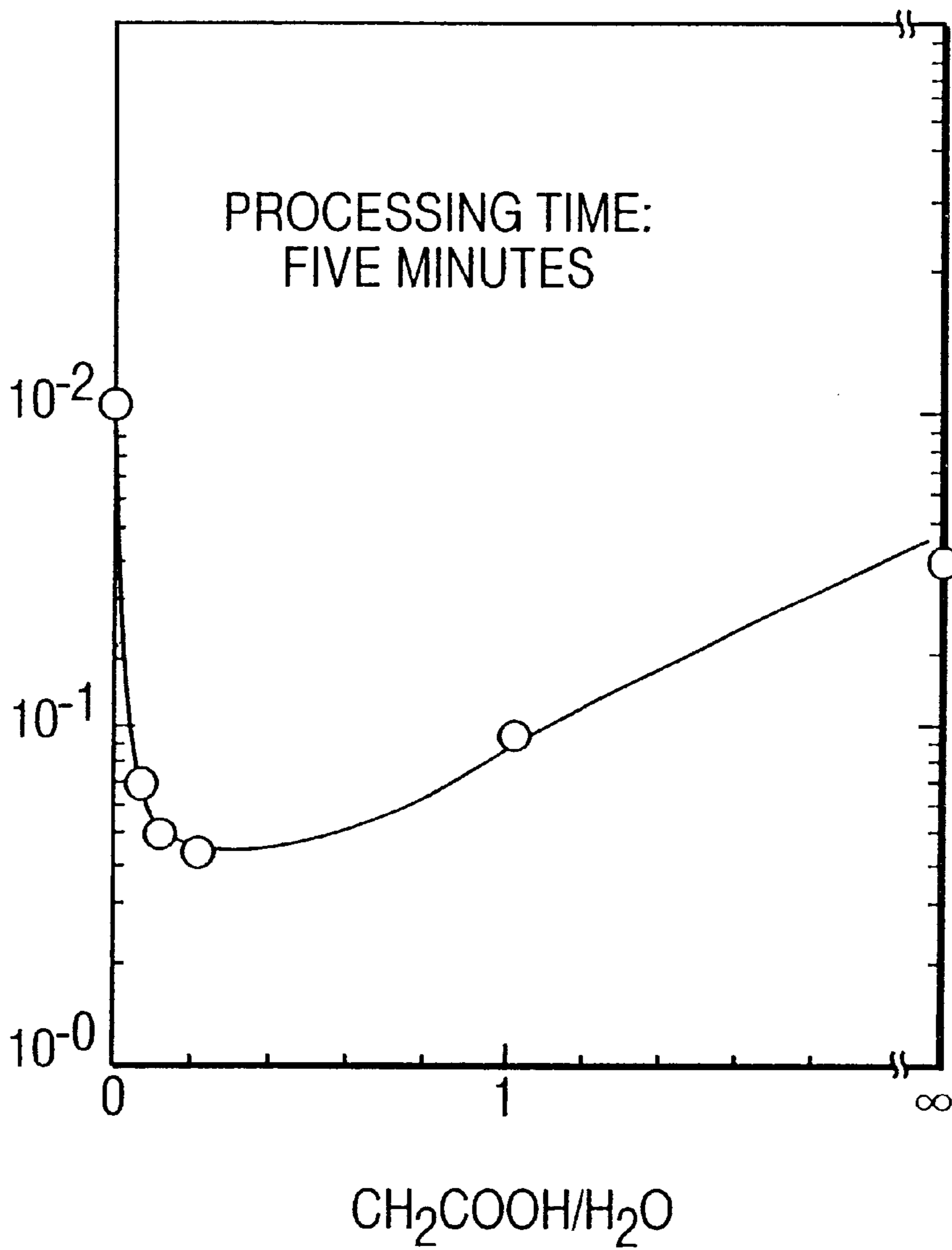
ACETIC ACID CONCENTRATION AND CORROSION OCCURENCE PERCENTAGE IN ACETIC ACID WASHING
