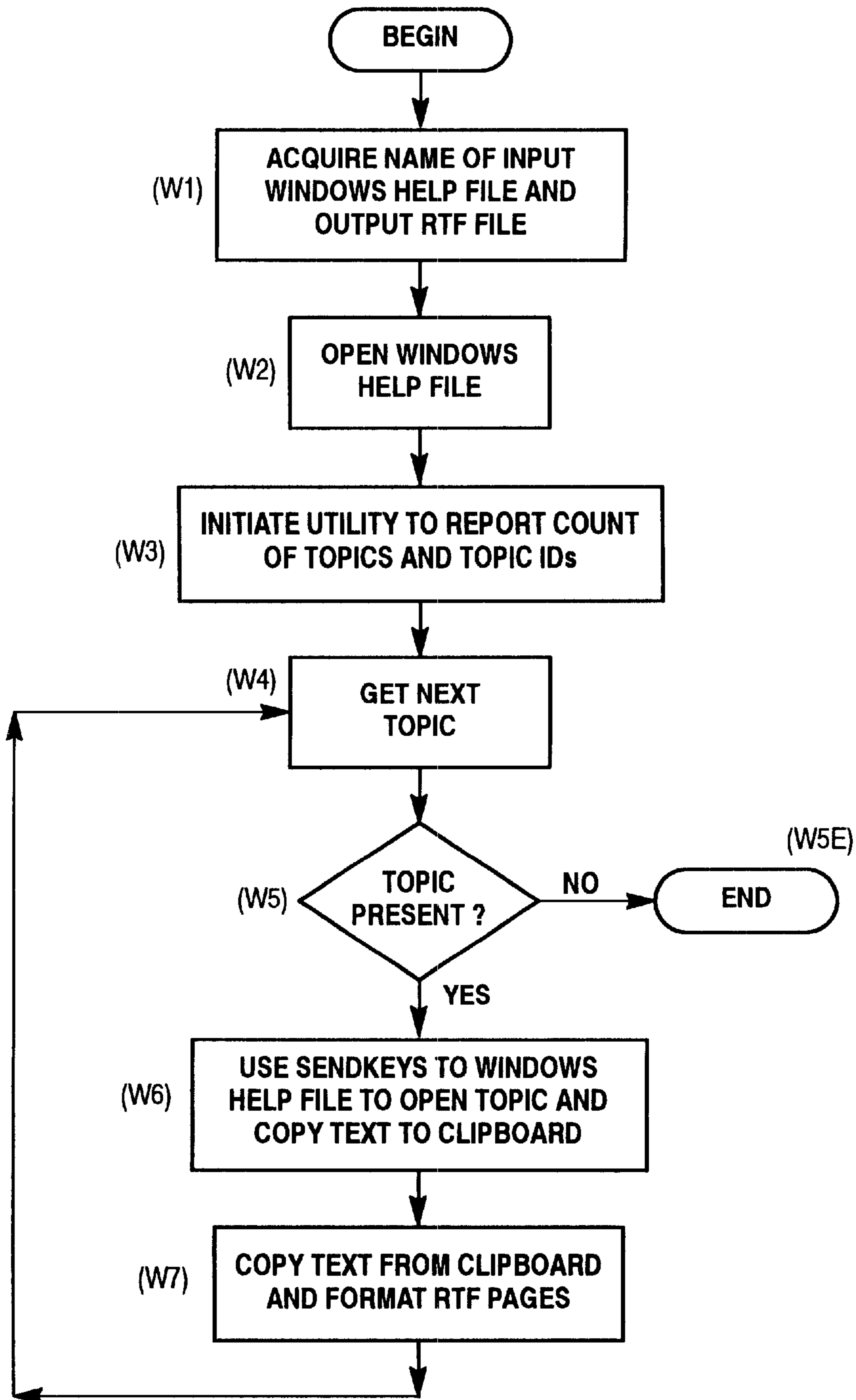
CONVERTING WINDOWS HELP FILE TO RTF
