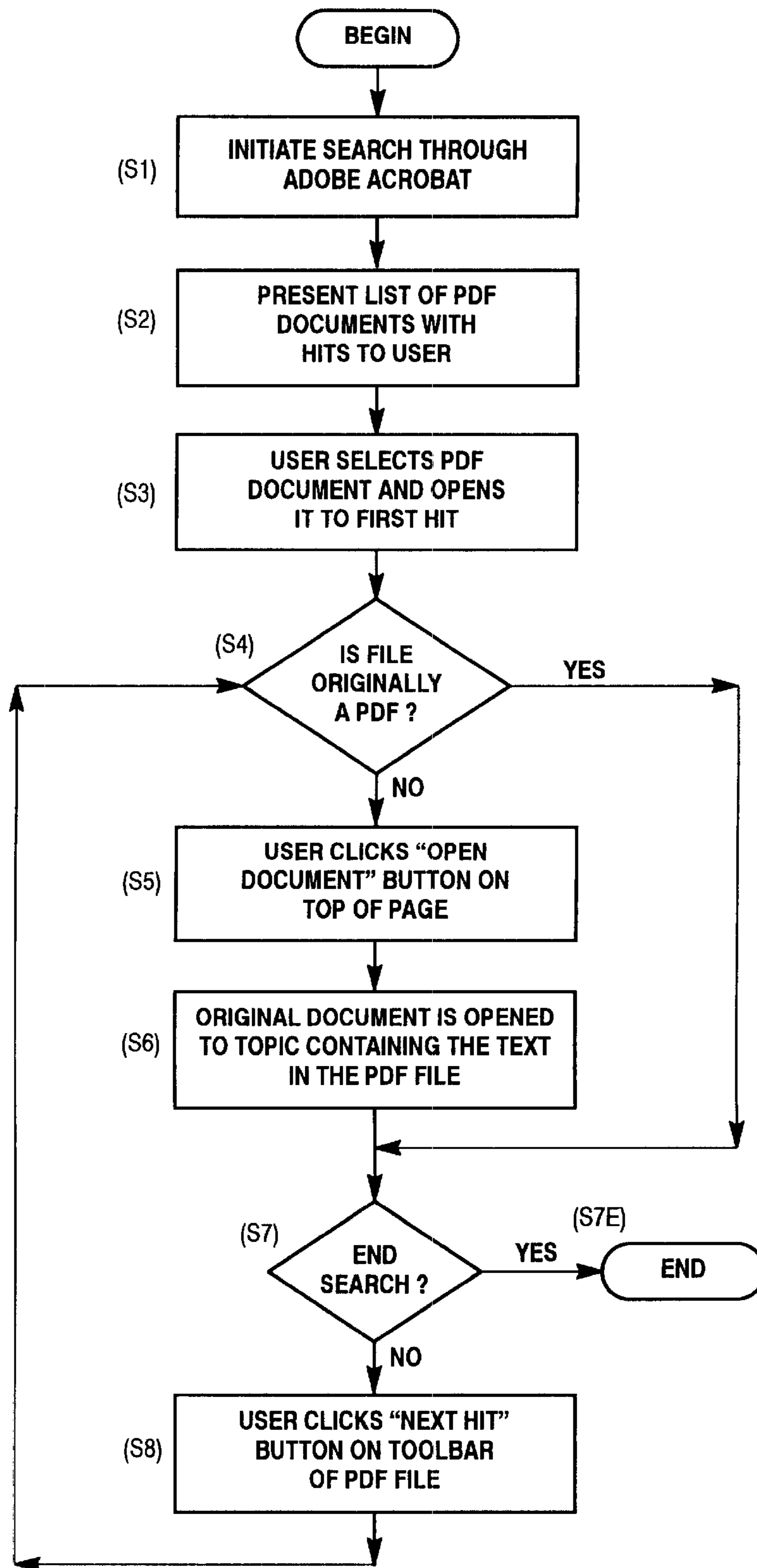
SEARCHING MULTIPLE FILE TYPES VIA PDF COPIES
