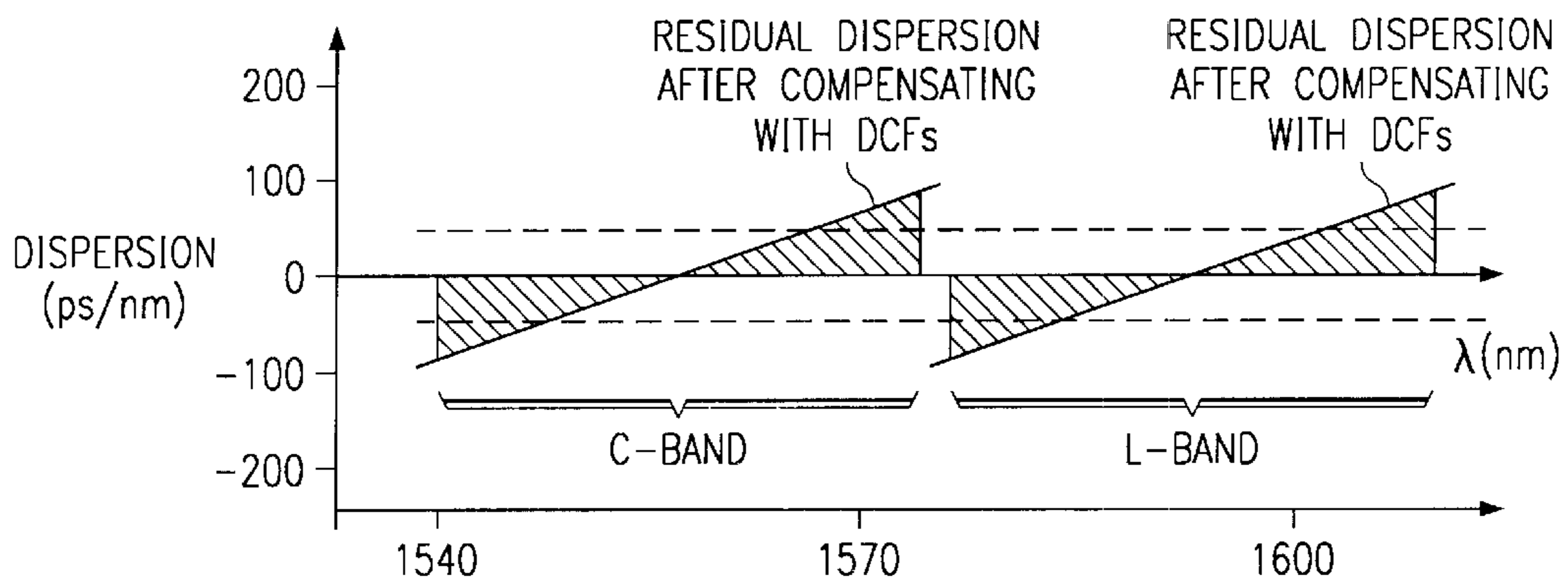
FIG. 3a --- 40-GBIT/S NRZ DISPERSION LIMITS
