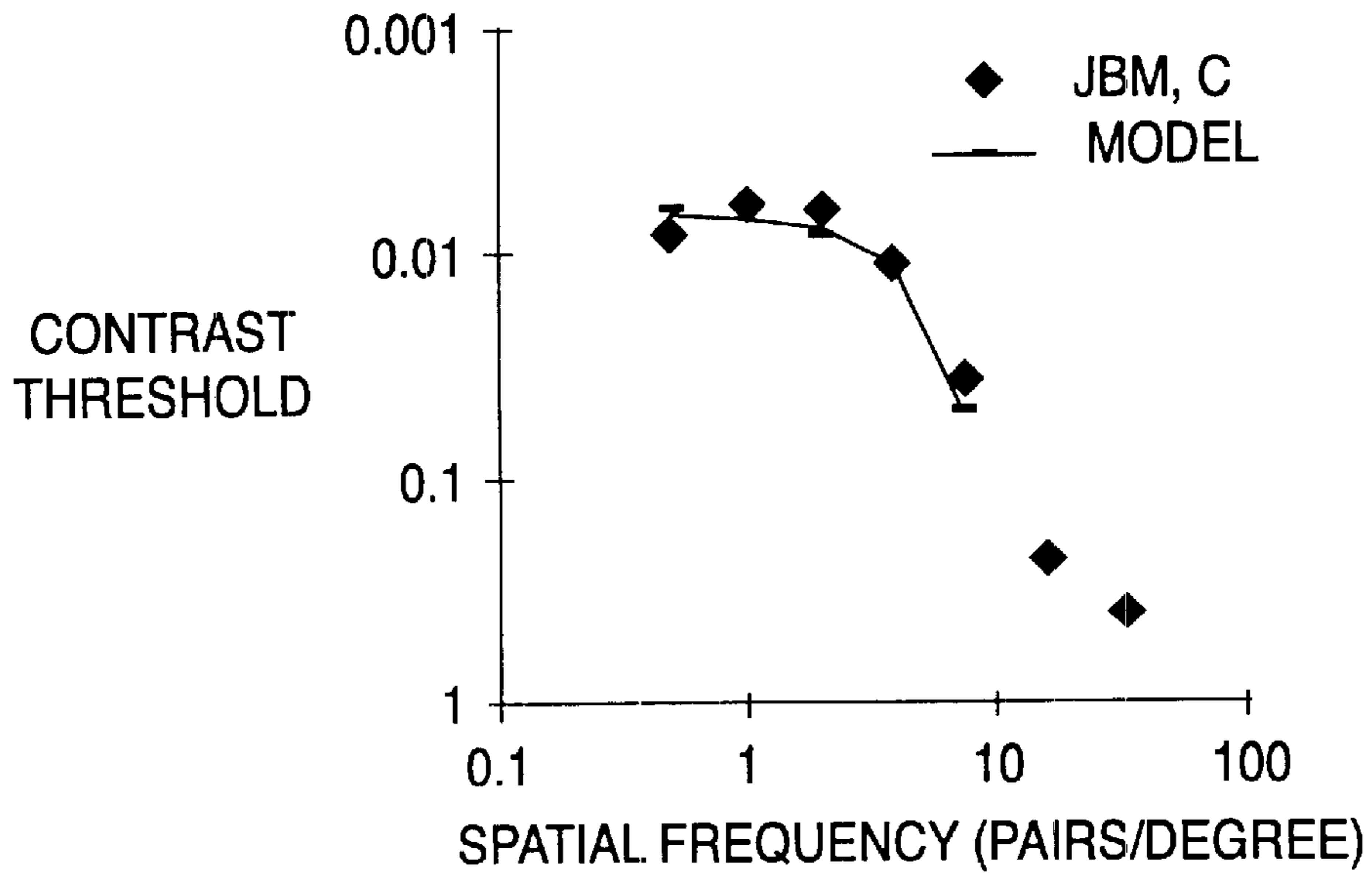
FIG. 14 CHECKERBOARD DETECTION
