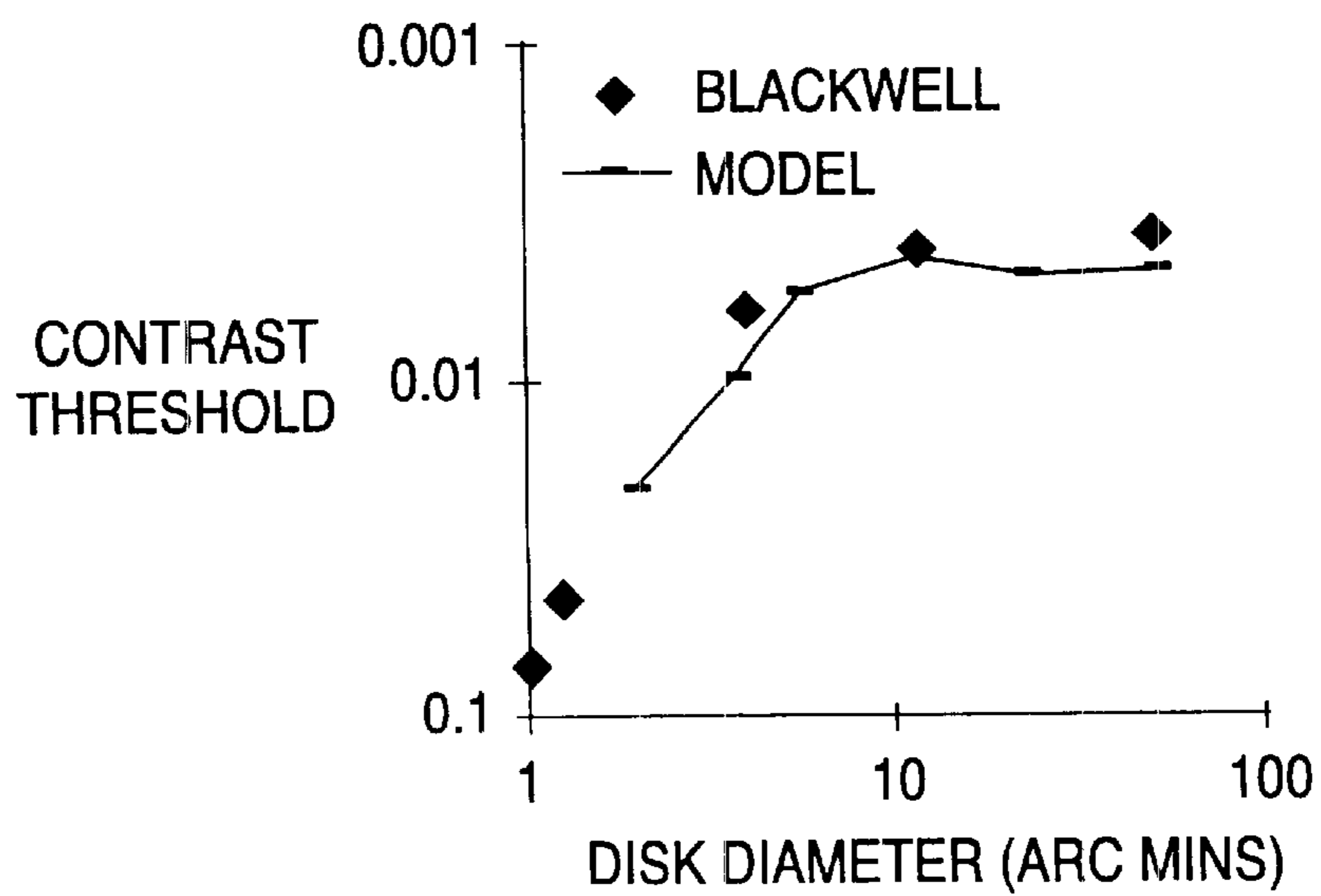
FIG. 13 DISK DETECTION
