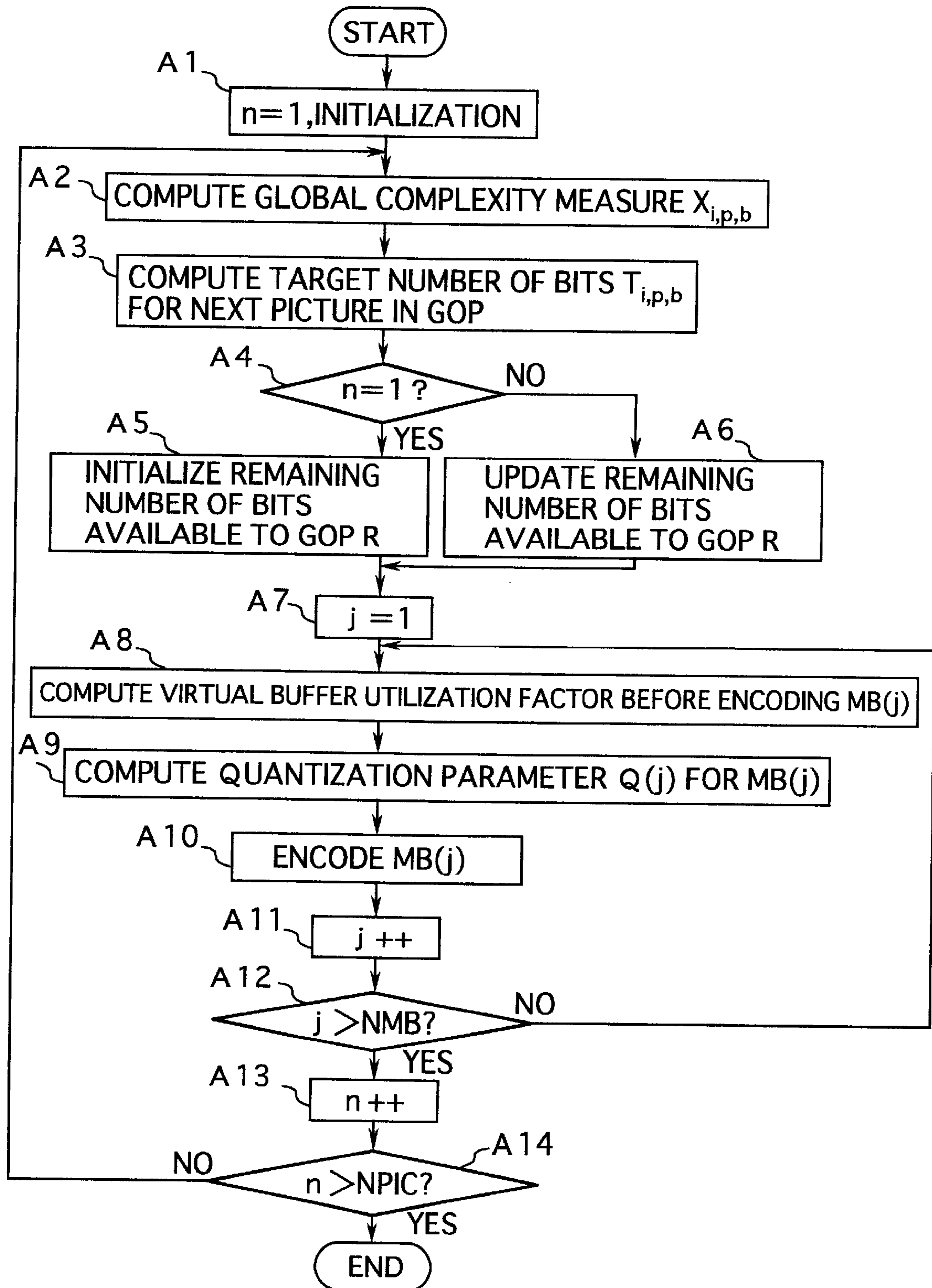
FIG. 19 PRIOR ART
