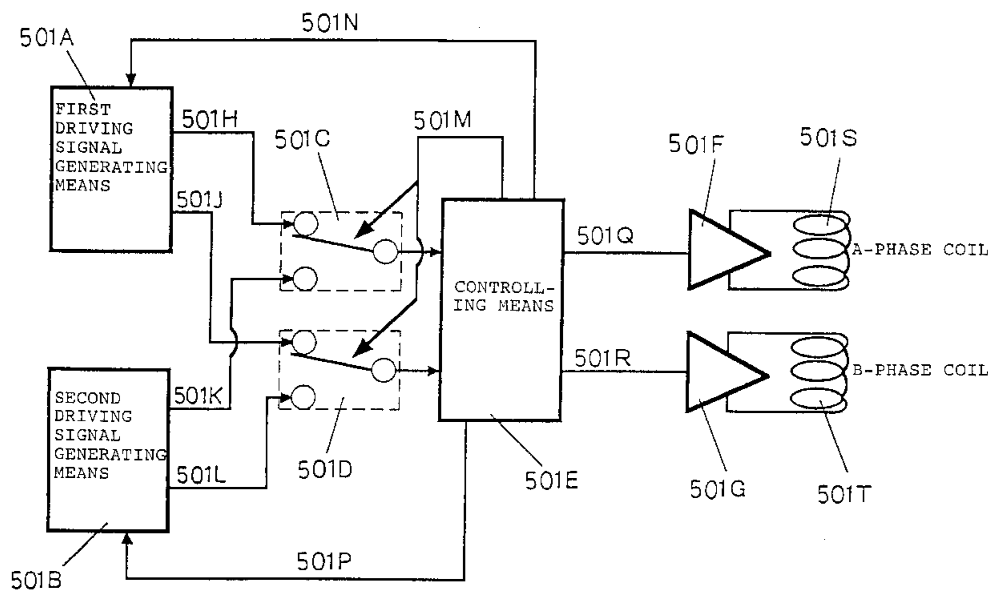
STEPPING MOTOR CONTROL CIRCUIT OF PRESENT INVENTION
