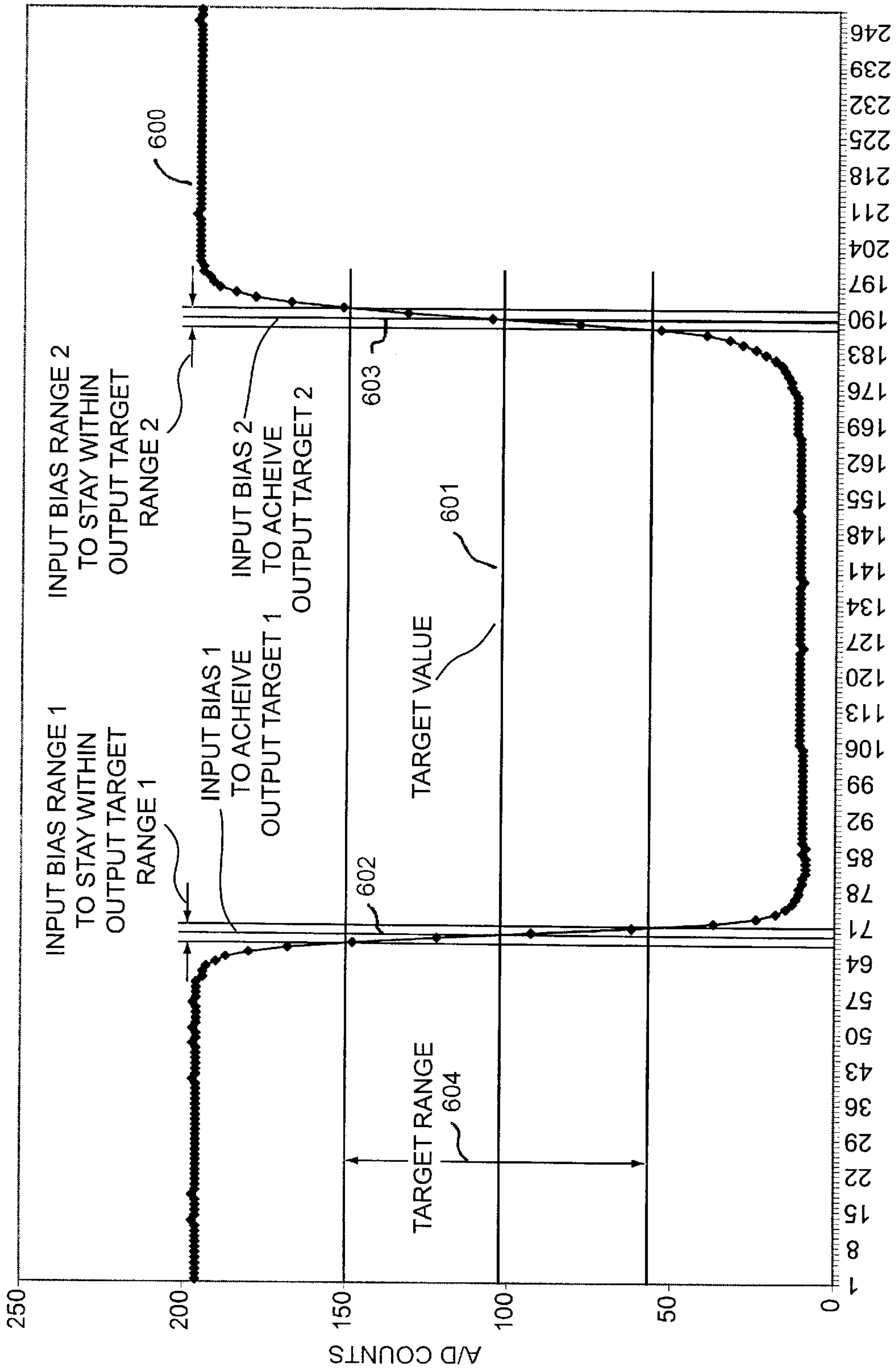
BIAS PWM VALUE
