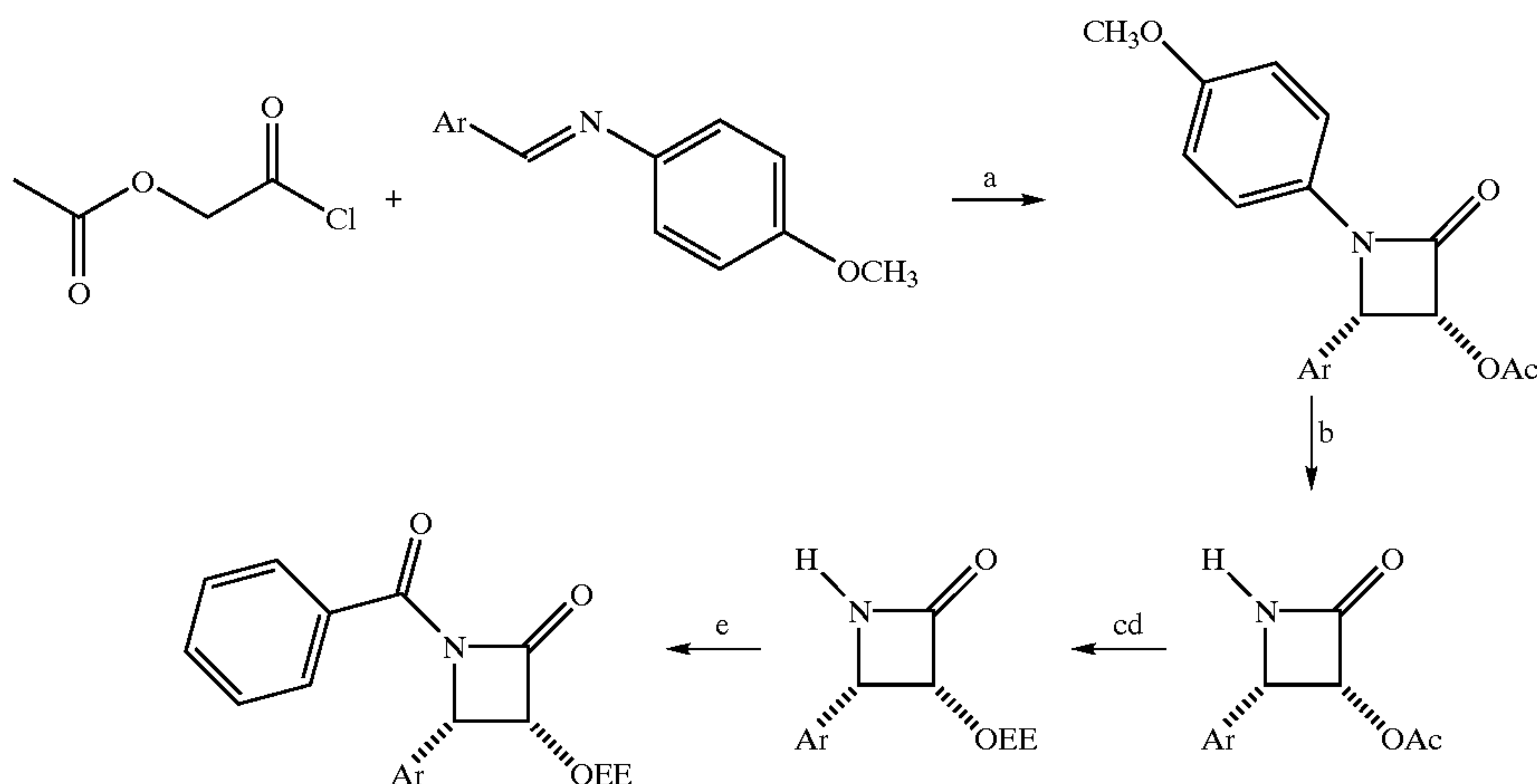
Scheme B
