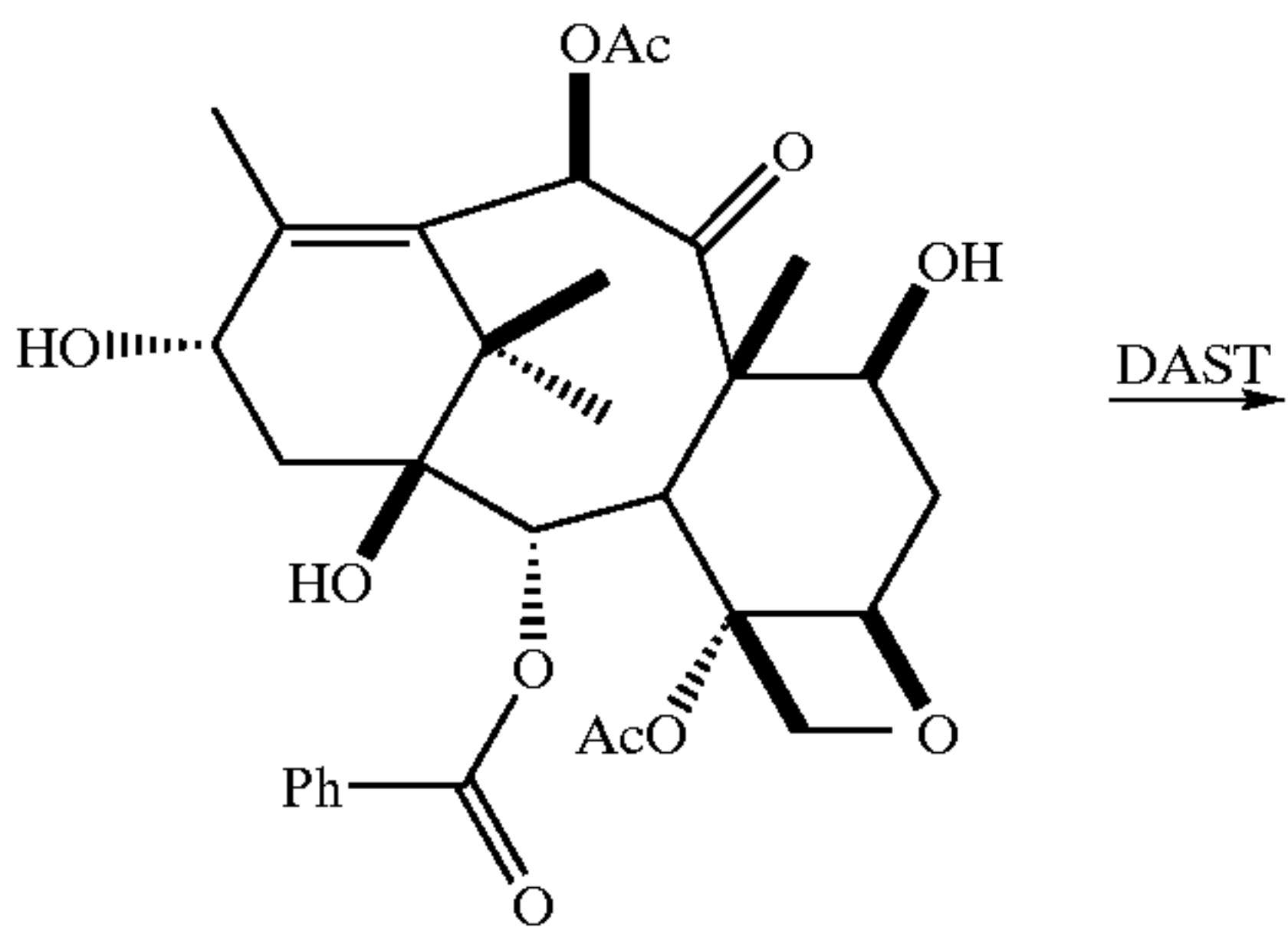
REACTION SCHEME 12
