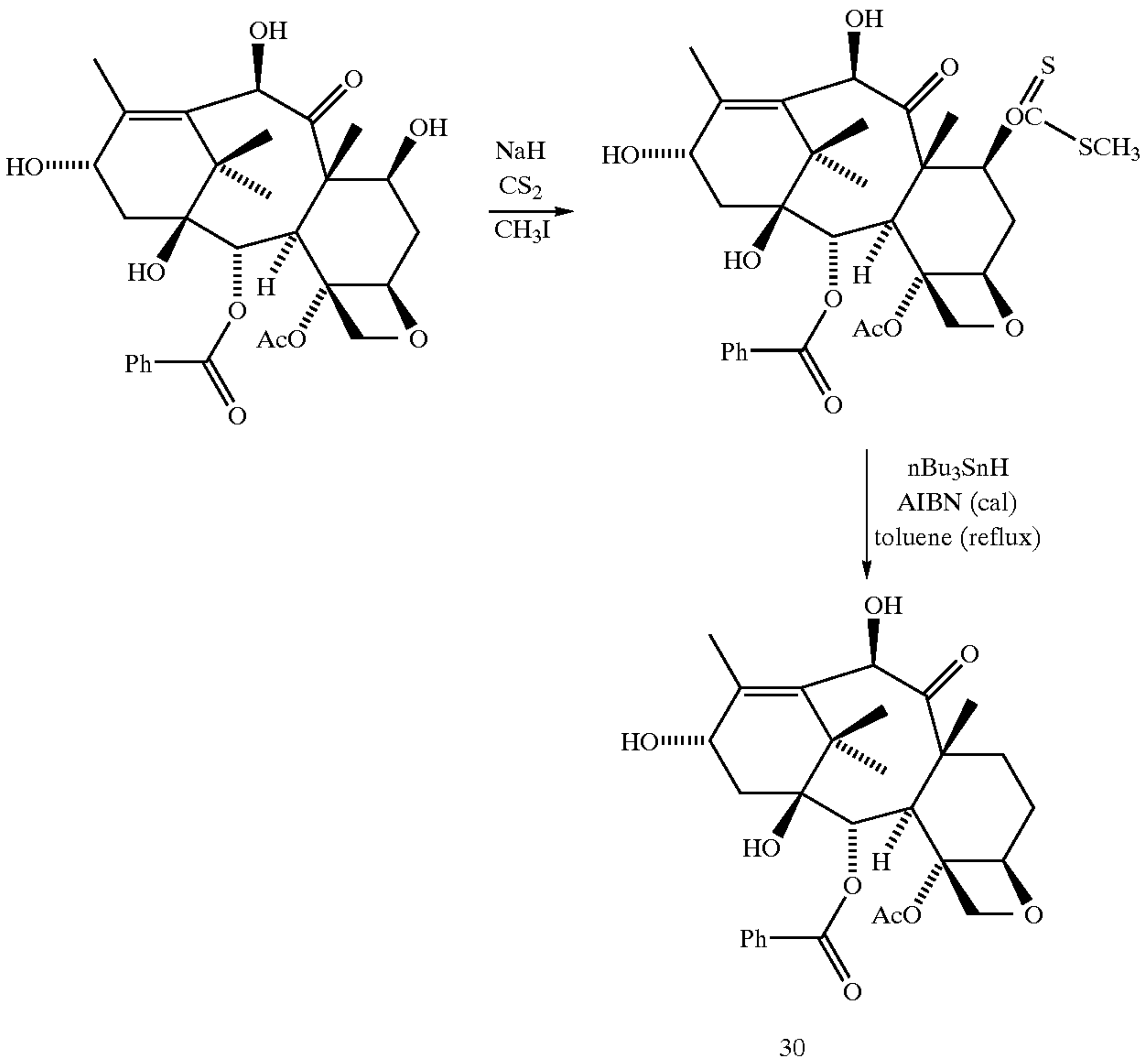
REACTION SCHEME 11
