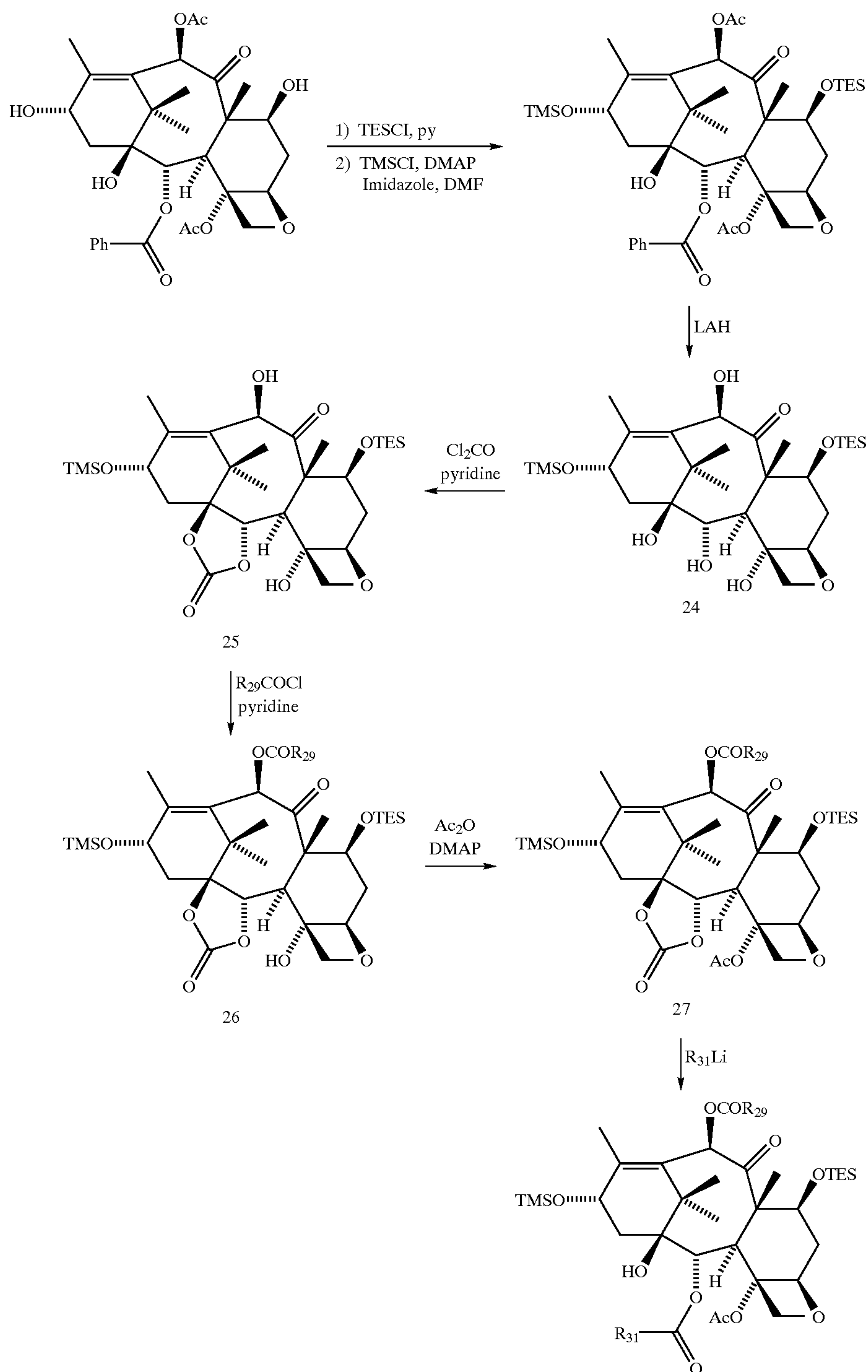
Scheme 10
