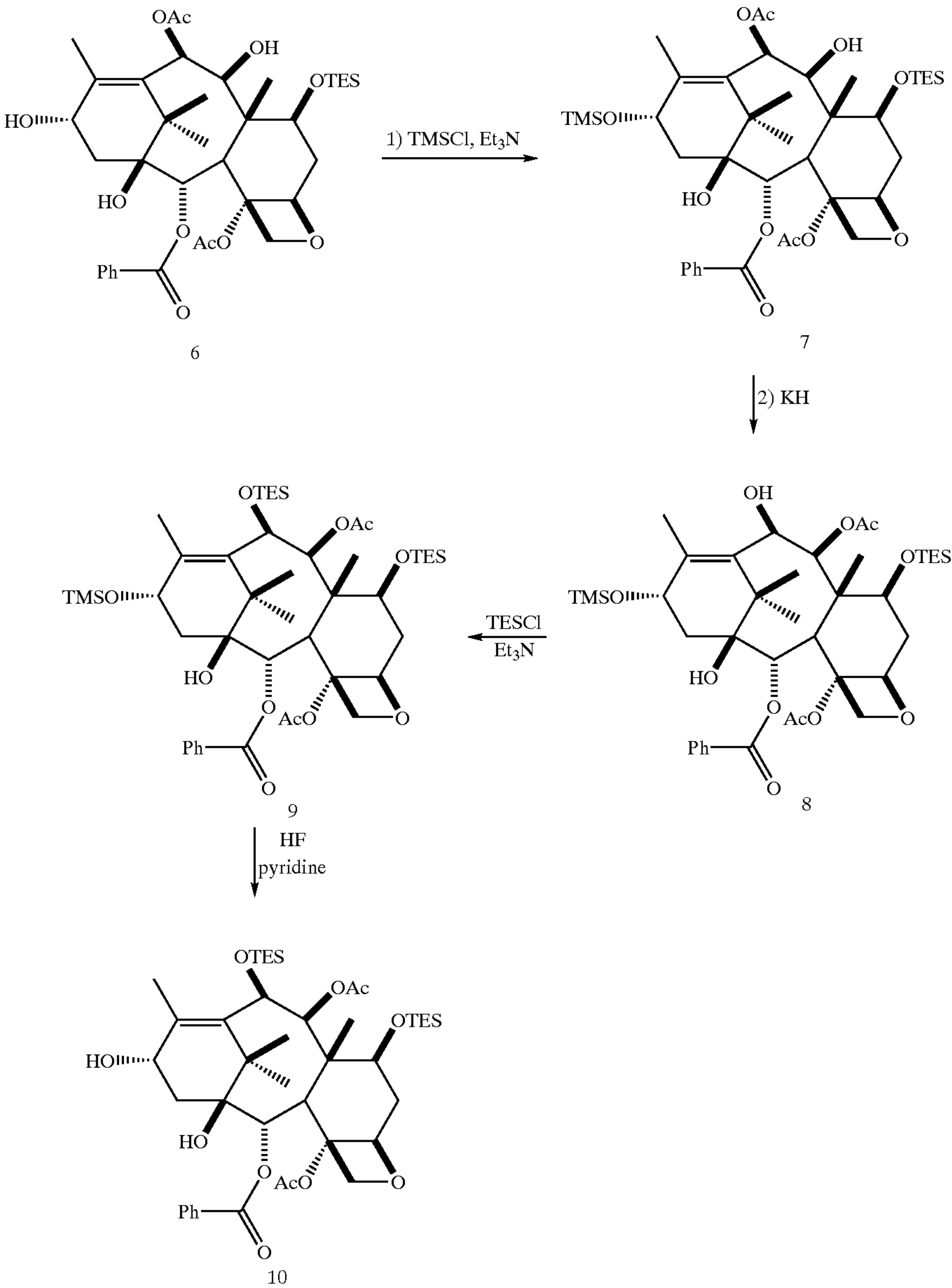
REACTION SCHEME 2
