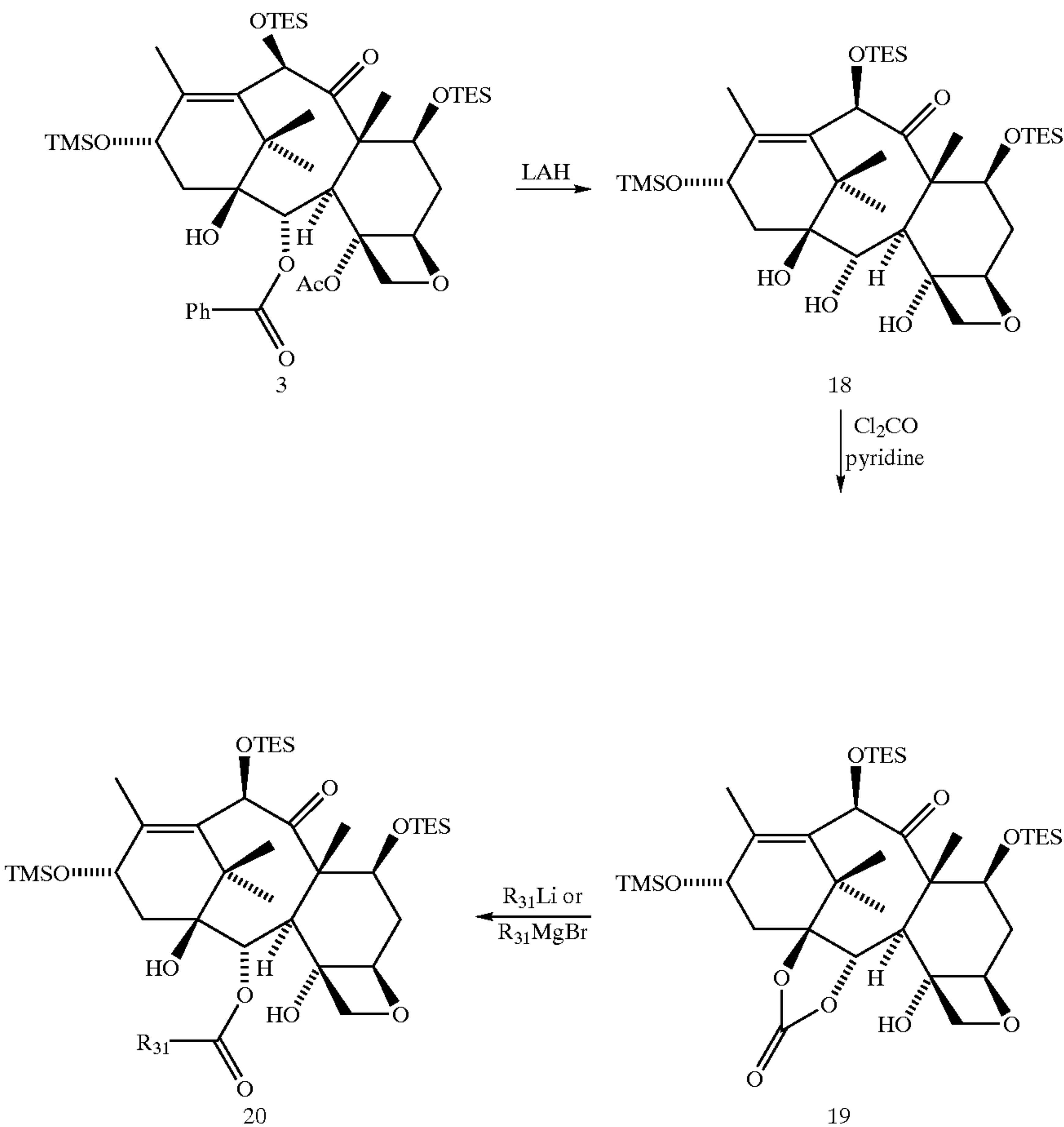
Scheme 6
