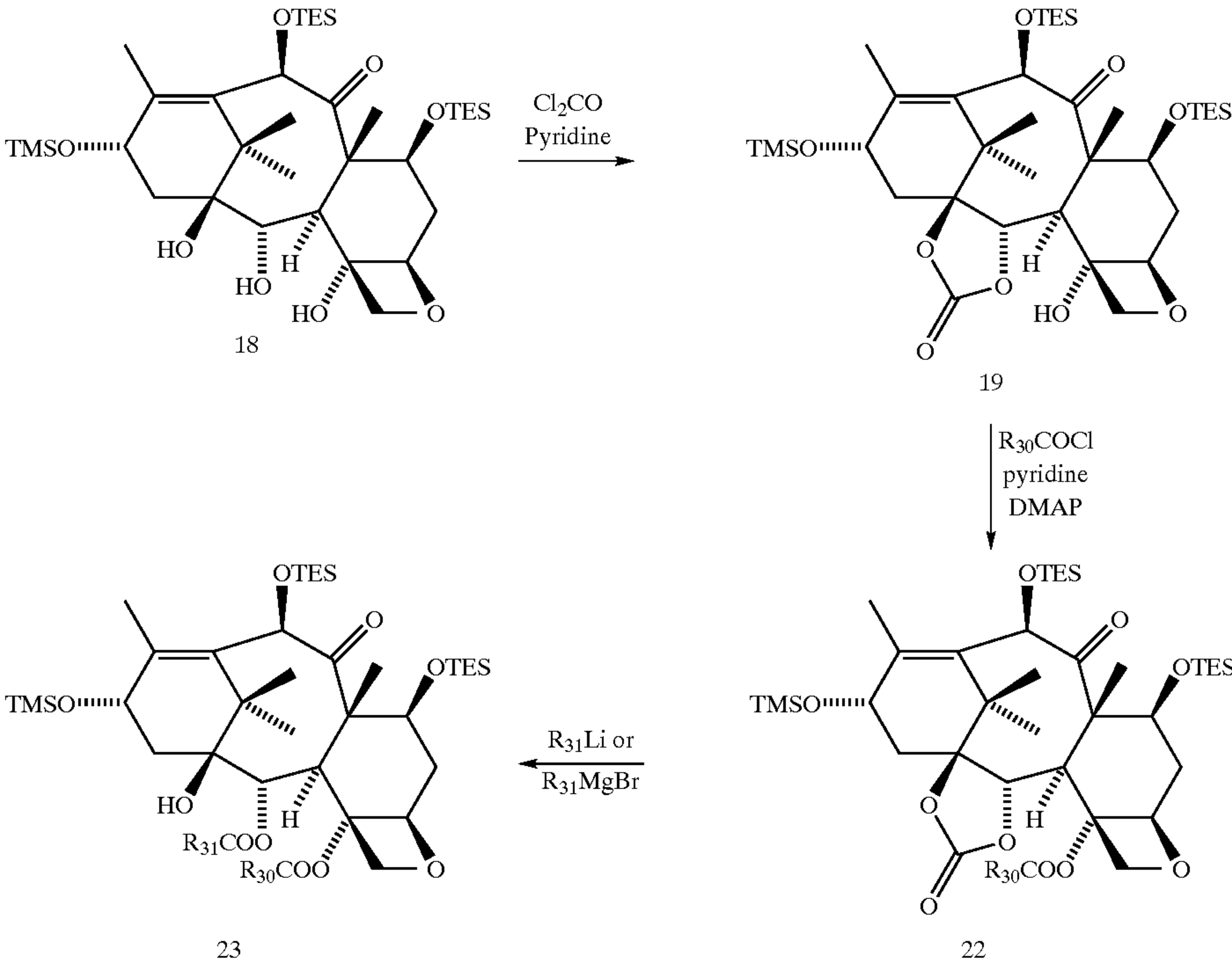
Scheme 9
