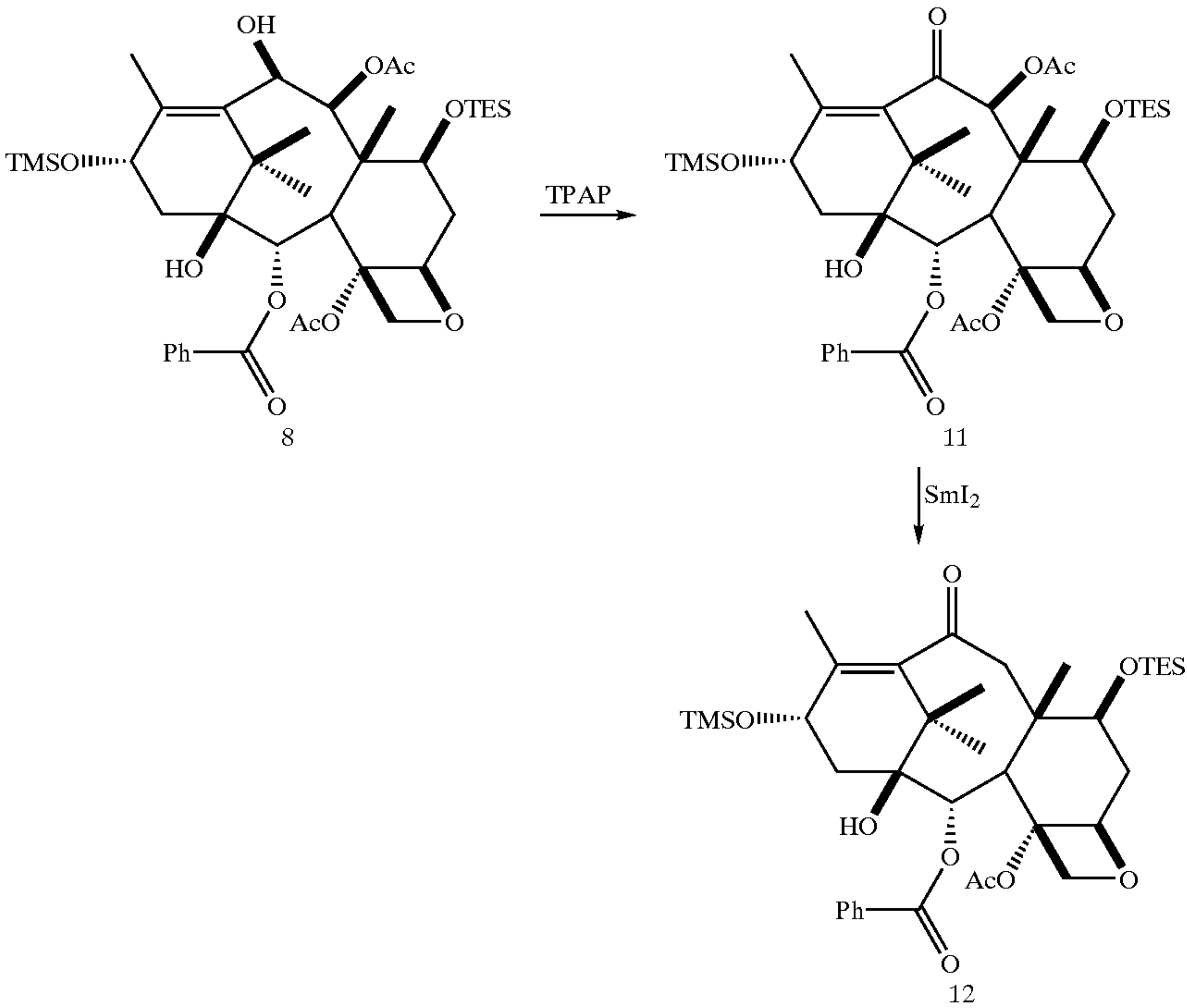
REACTION SCHEME 3
