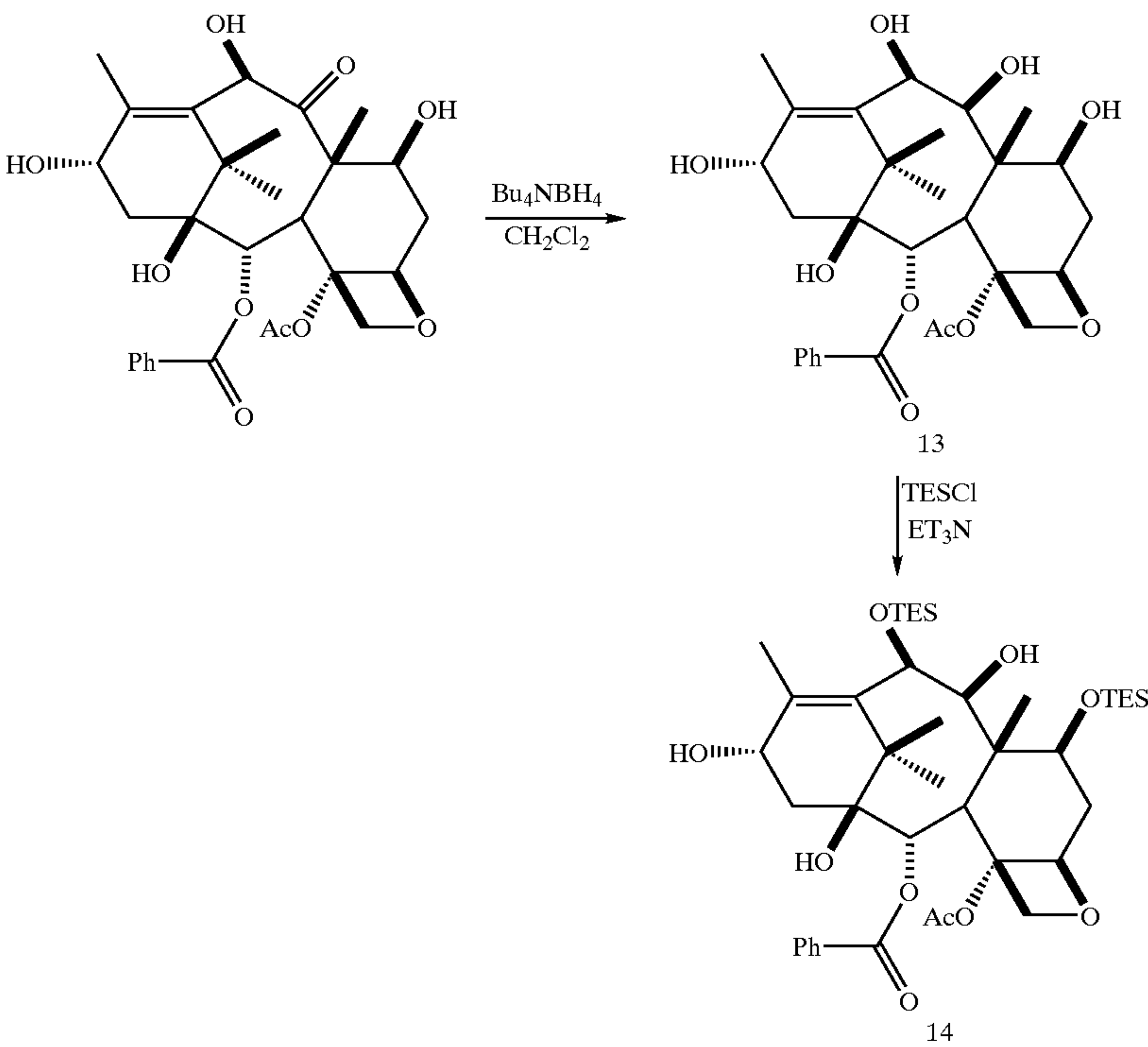
REACTION SCHEME 4
