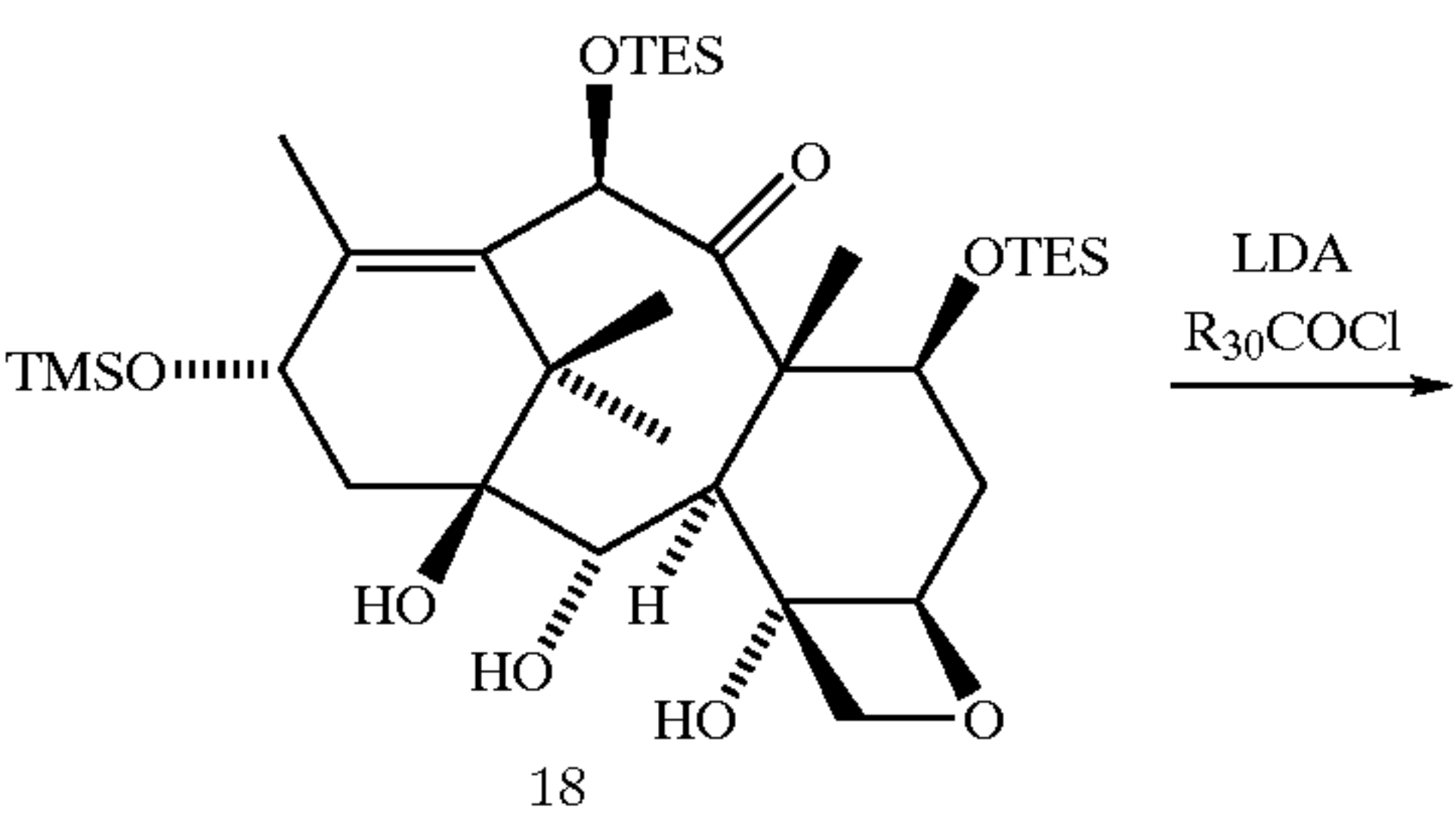
Scheme 7
