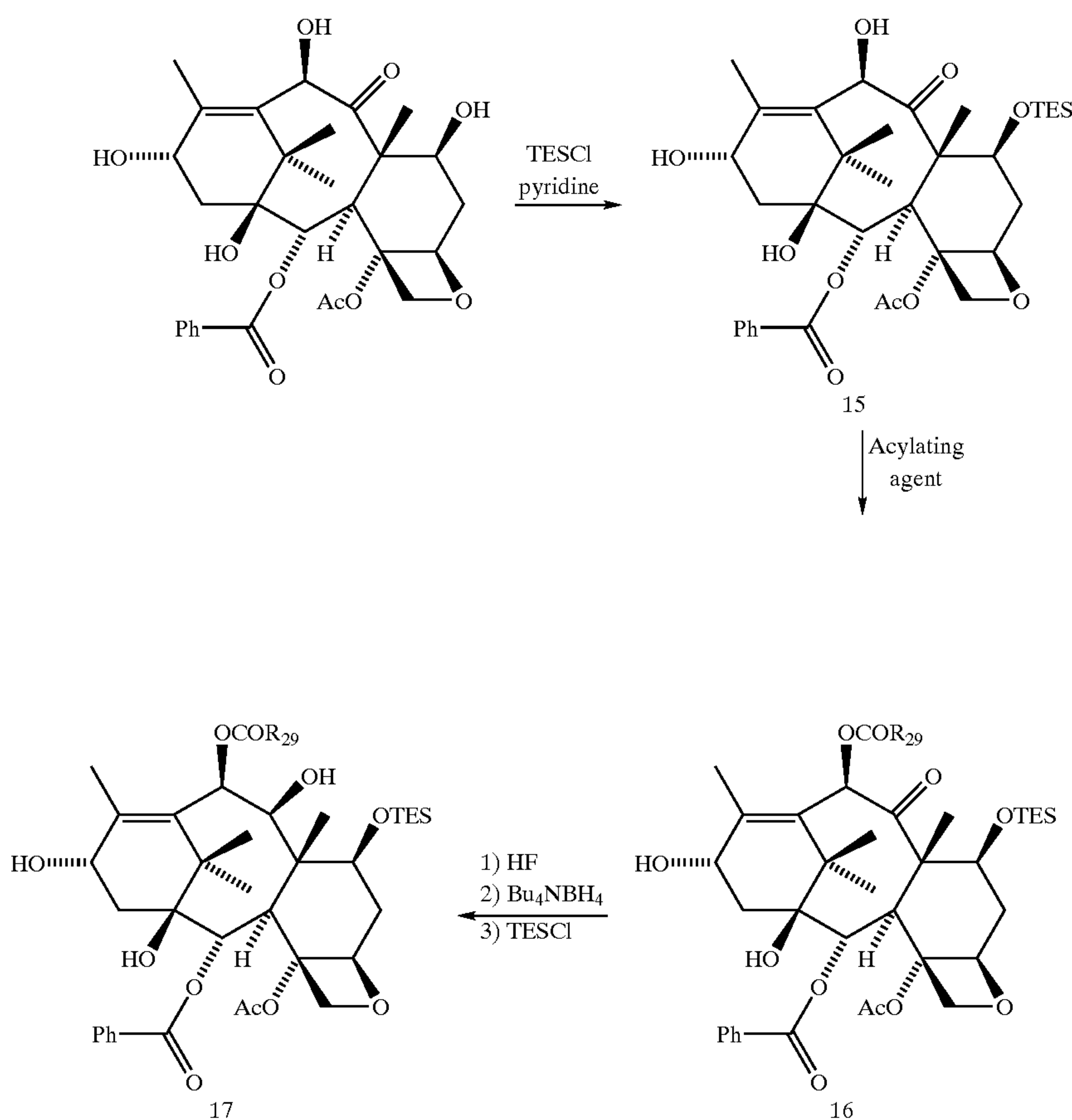
REACTION SCHEME 5
