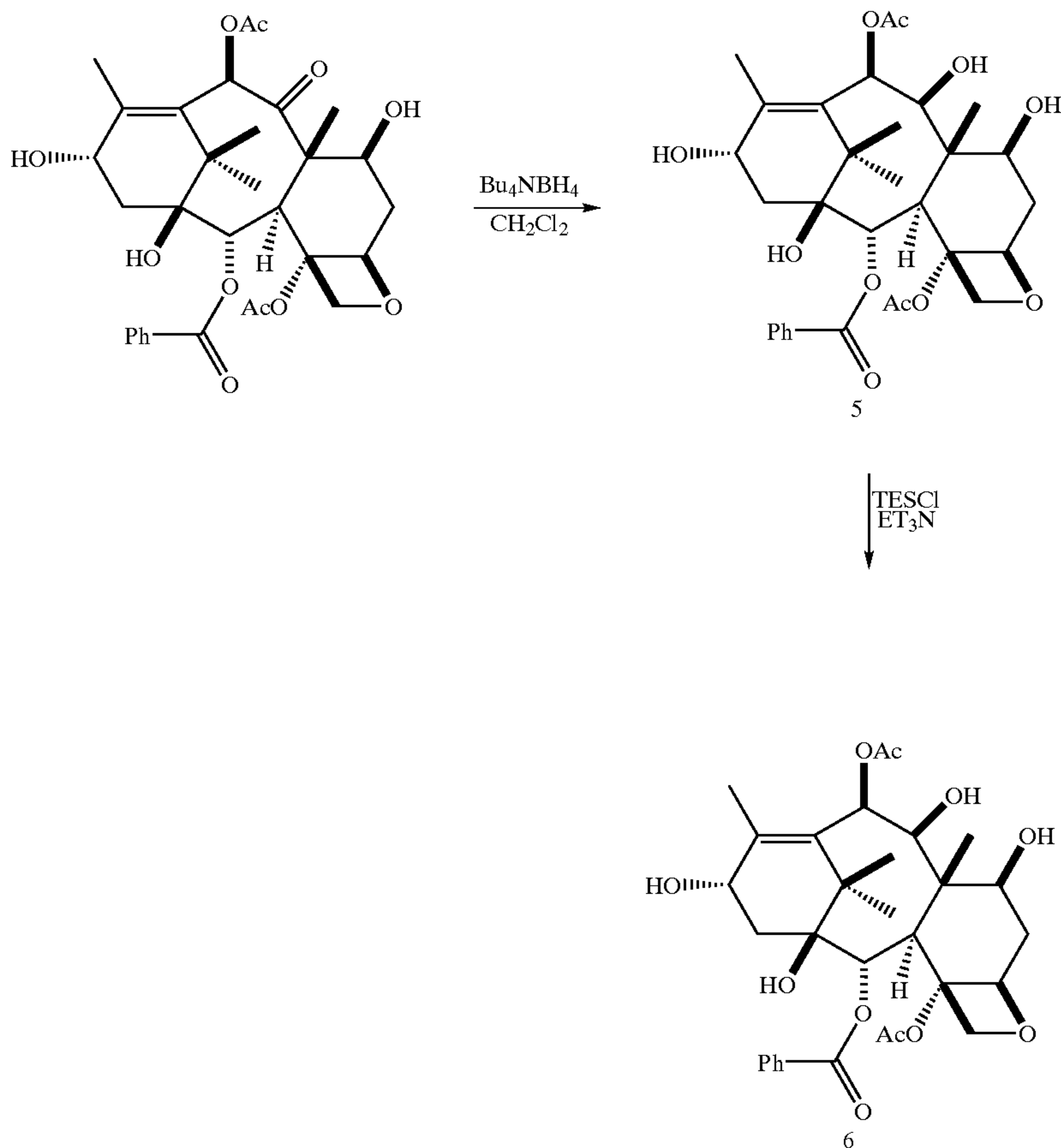
REACTION SCHEME 1
