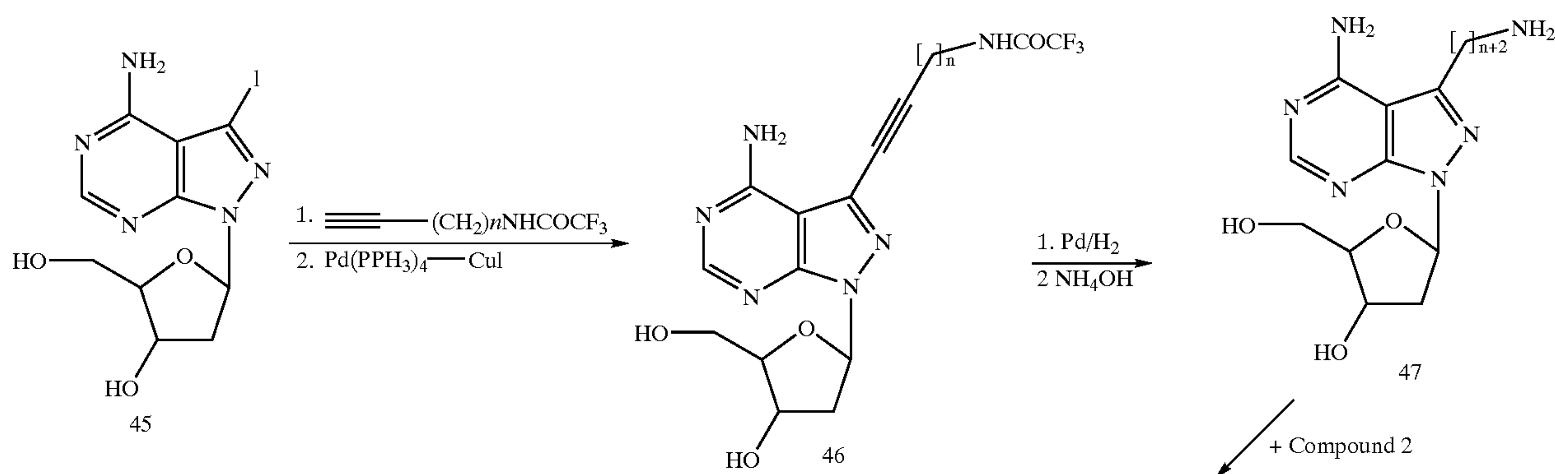
REACTION SCHEME 11
