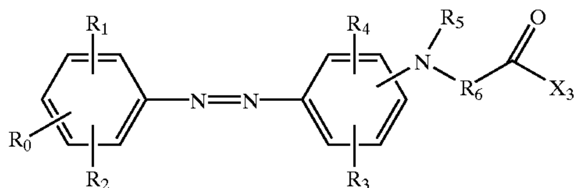
Formula 3A
