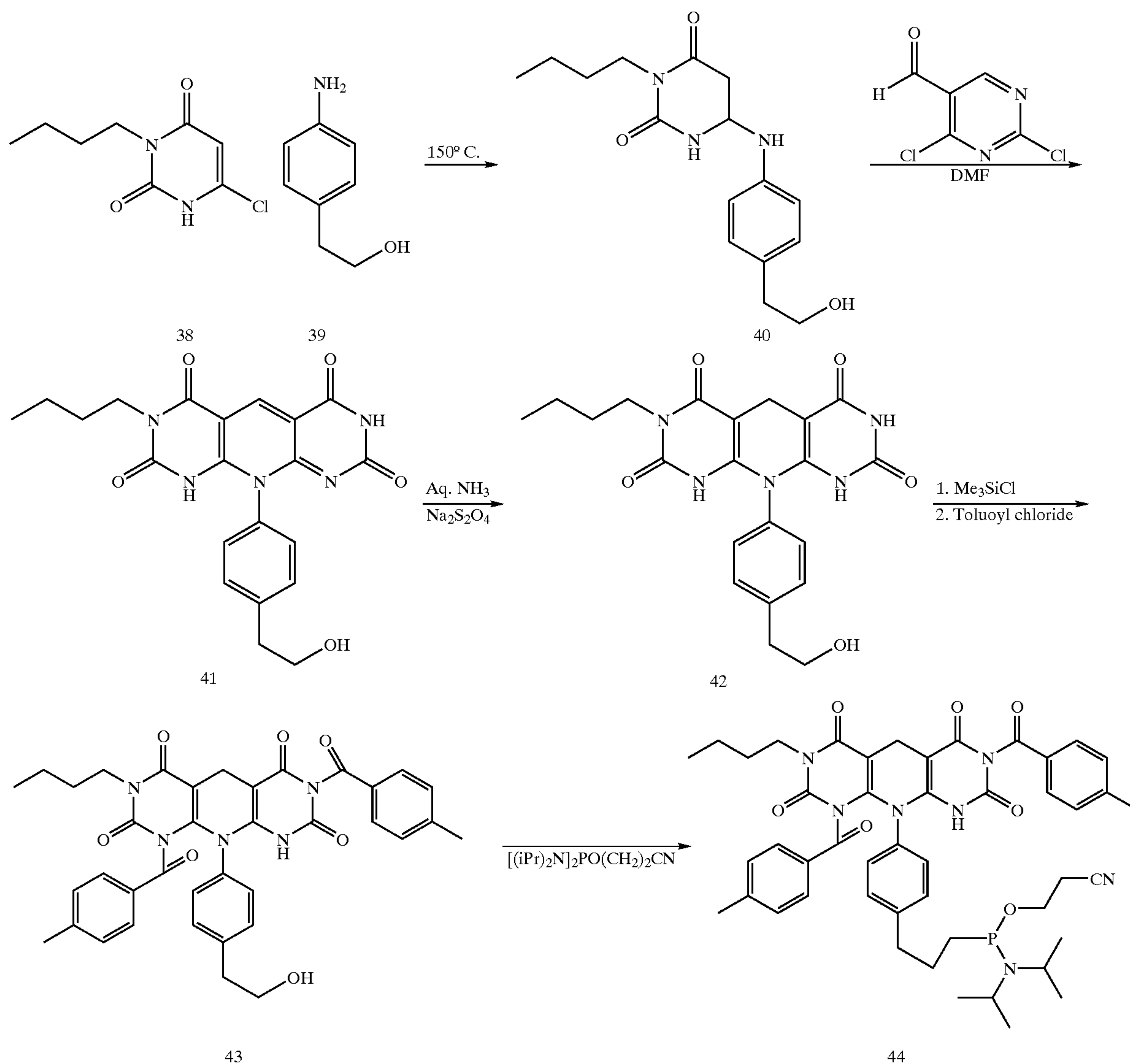
Reaction Scheme 10
