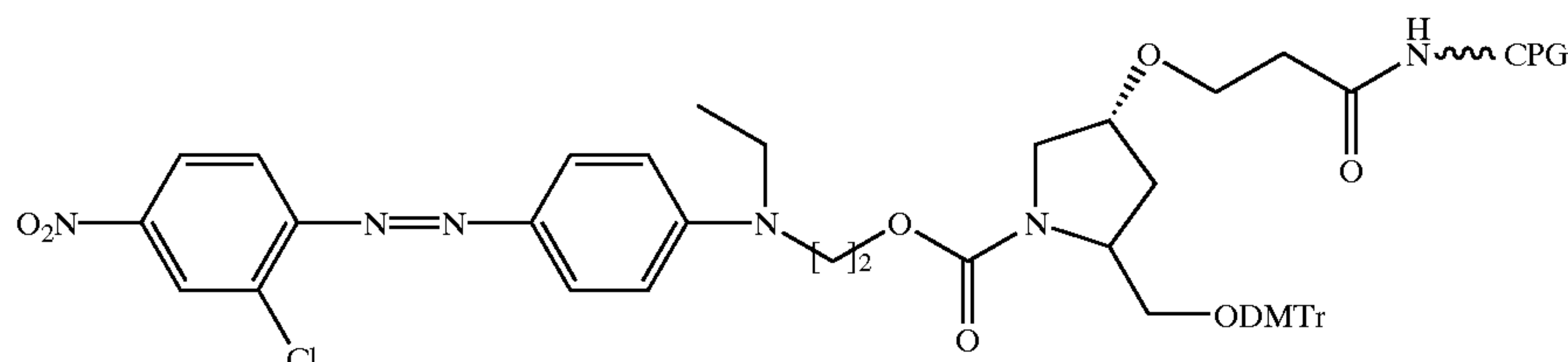
RED 13-pyrrolidine-DMTr-CPG, 12
