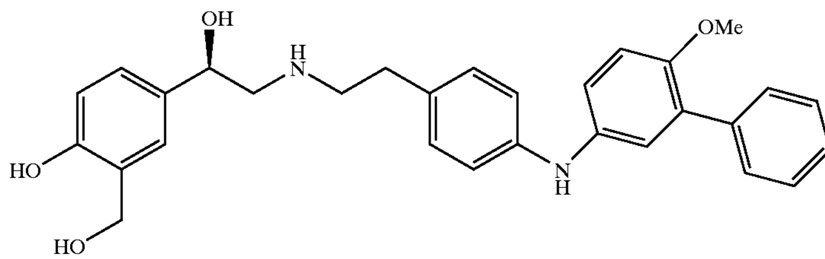
N-{2-[4-(3-phenyl-4-methoxyphenyl)aminophenyl]ethyl}-(R)-2-hydroxy-2-(3-hydroxymethyl-4-hydroxyphenyl)ethylamine
