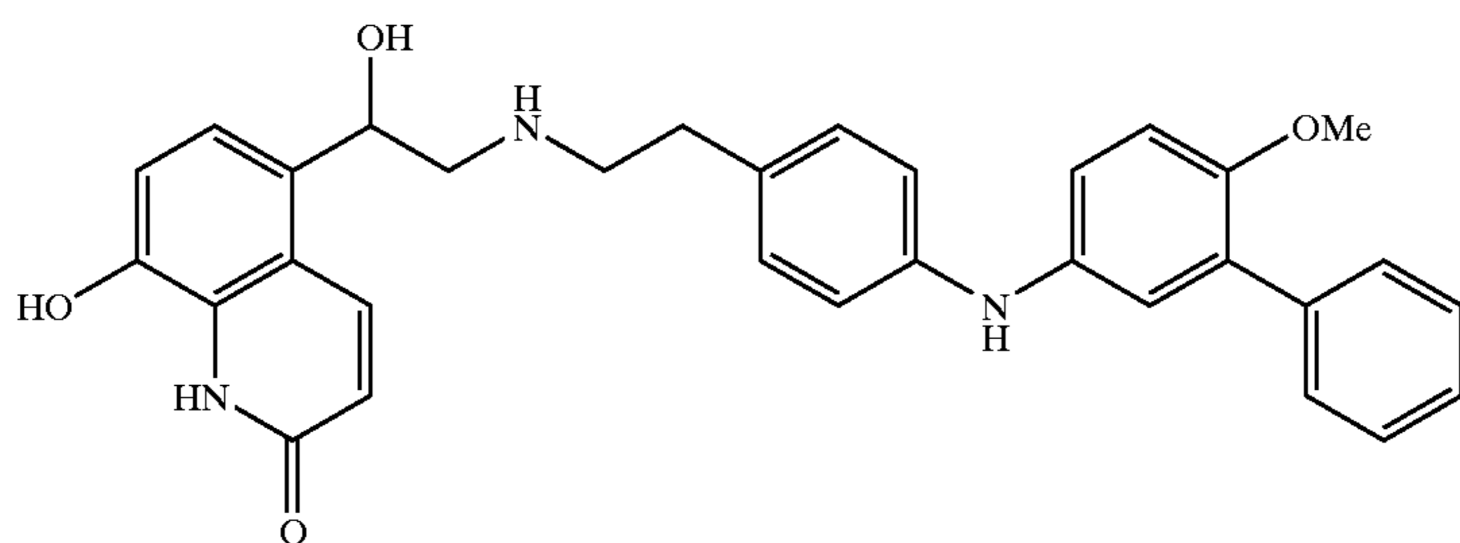
N-{2-[4-(3-phenyl-4-methoxyphenyl)aminophenyl]ethyl}-2-hydroxy-2-(8-hydroxy-2(1H)-quinolinon-5-yl)ethylamine
