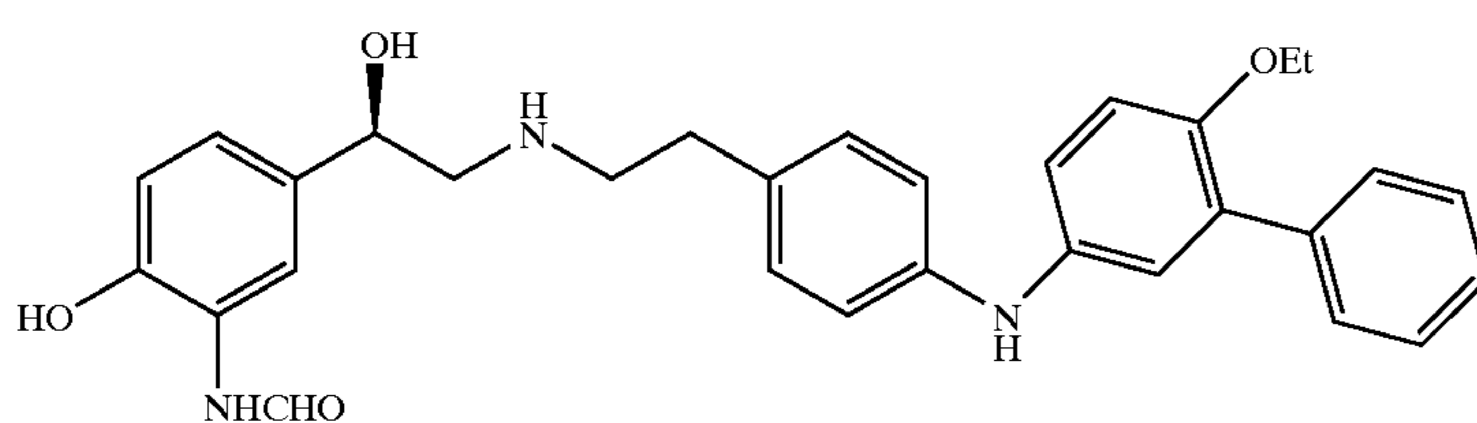
N-{2-[4-(3-phenyl-4-ethoxyphenyl)aminophenyl]ethyl}-(R)-2-hydroxy-2-(3-formamido-4-hydroxyphenyl)ethylamine
