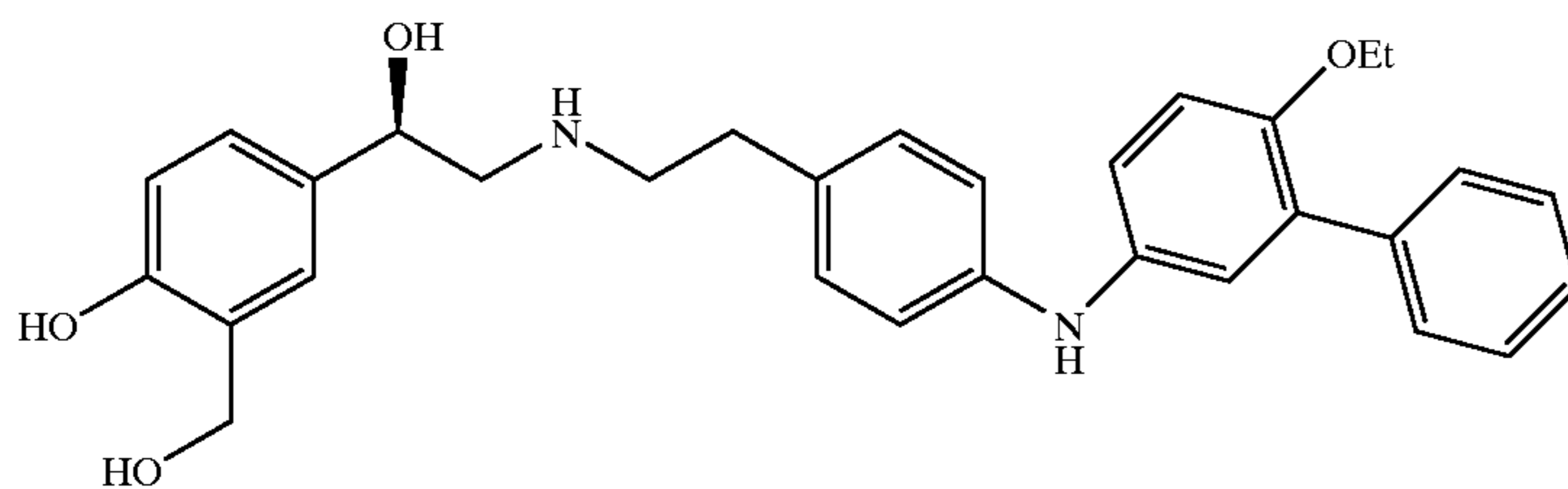
N-{2-[4-(3-phenyl-4-ethoxyphenyl)aminophenyl]ethyl}-(R)-2-hydroxy-2-(3-hydroxymethyl-4-hydroxyphenyl)ethylamine
