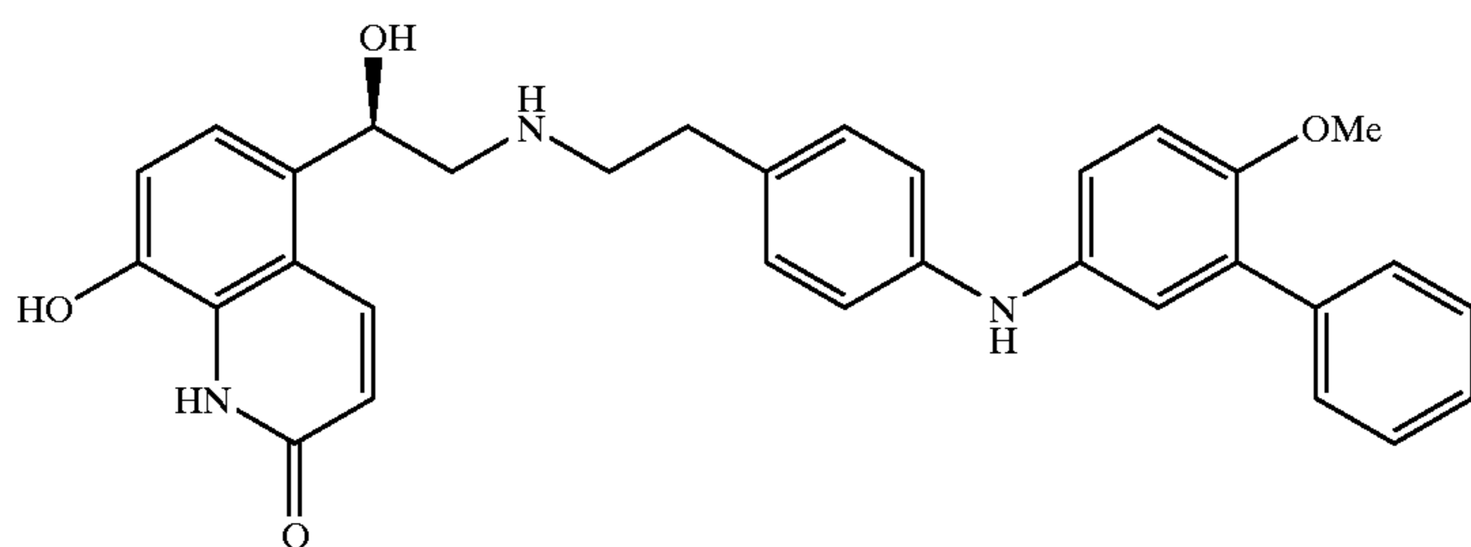
N-{2-[4-(3-phenyl-4-methoxyphenyl)aminophenyl]ethyl}-(R)-2-hydroxy-2-(8-hydroxy-2(1H)-quinolinon-5-yl)ethylamine
