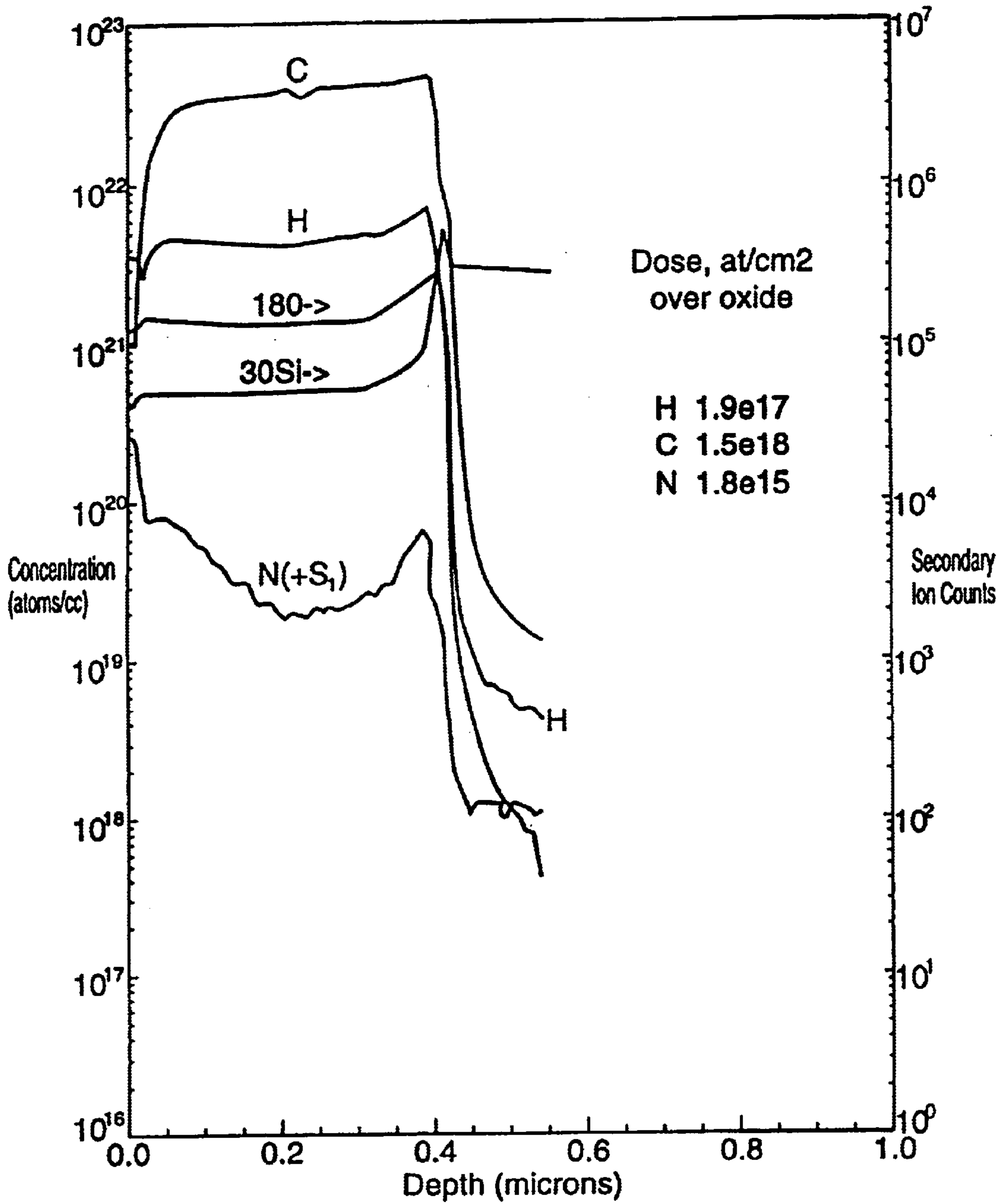
FIG. 13 SIMS Profile Analysis
