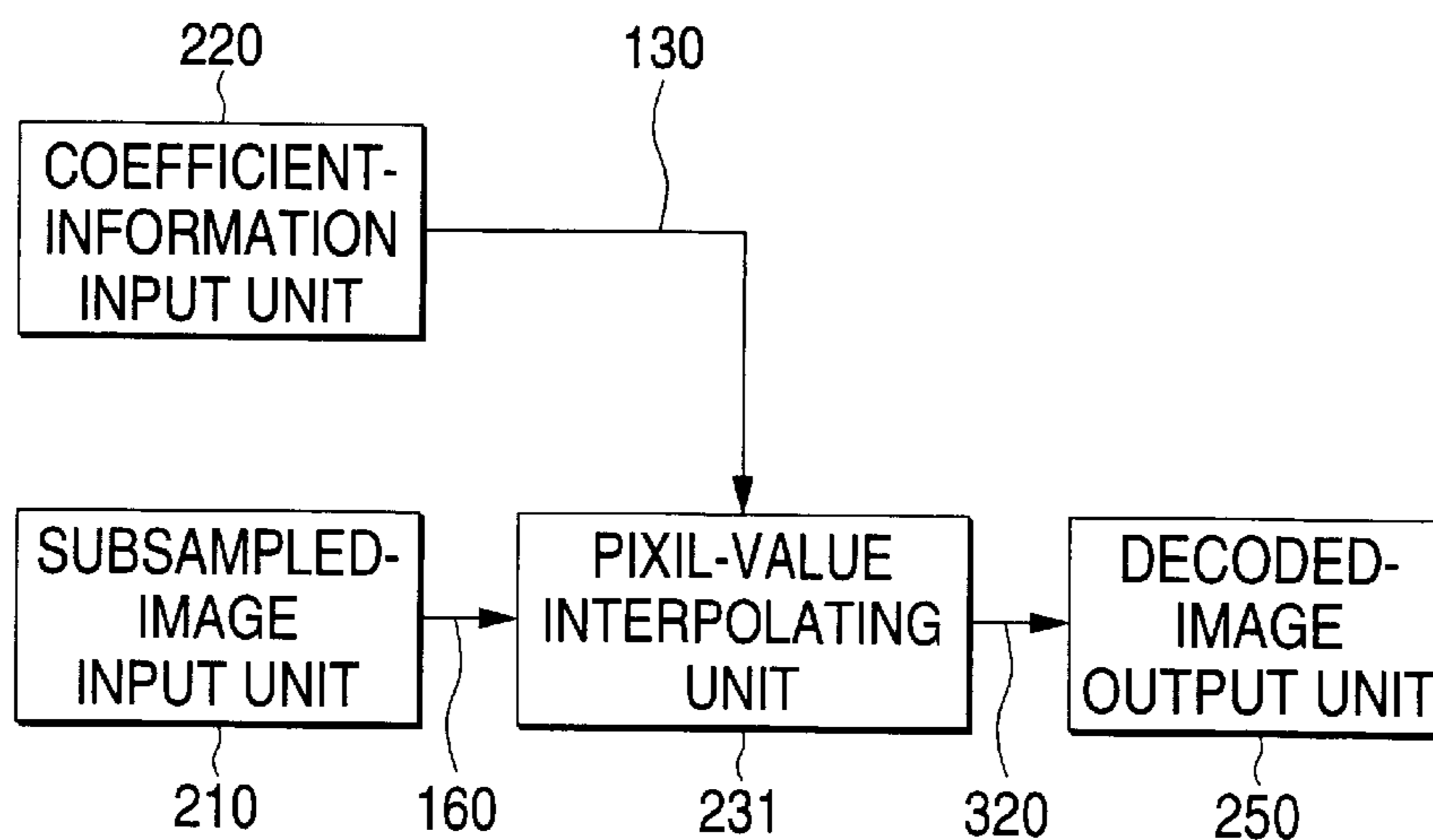
DECODING APPARATUS FOR DIRECTLY INTERPOLATING PIXEL VALUES
