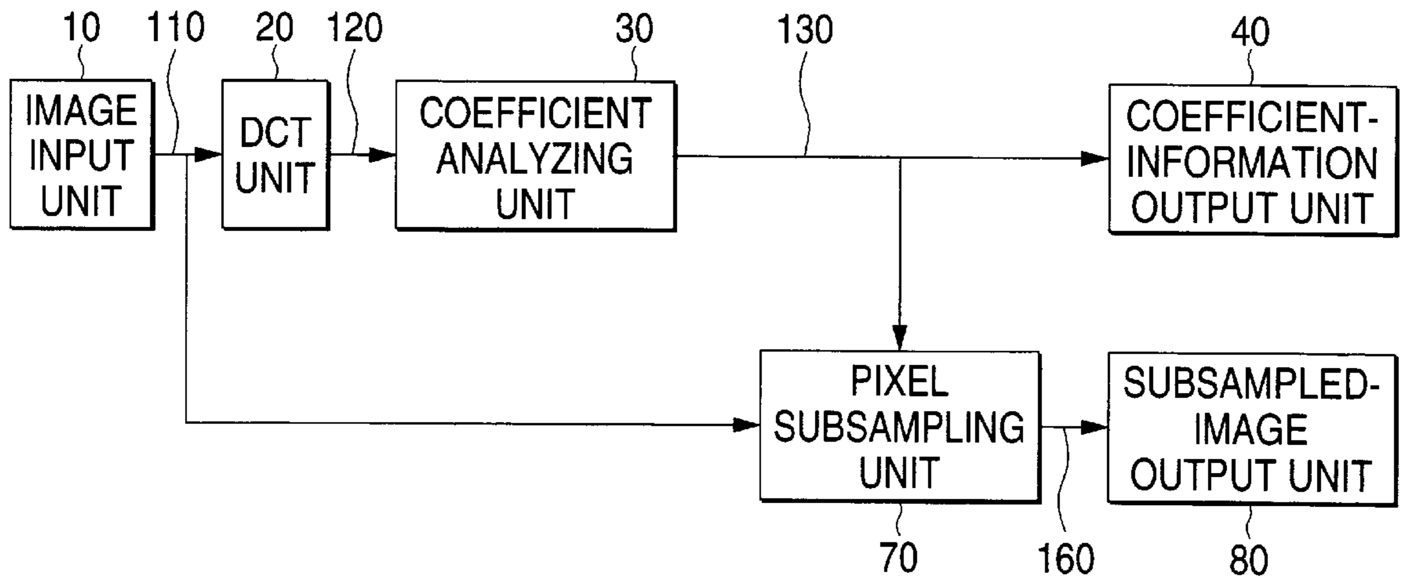
ENCODING APPARATUS FOR DIRECTLY SUBSAMPLING AN INPUT IMAGE
