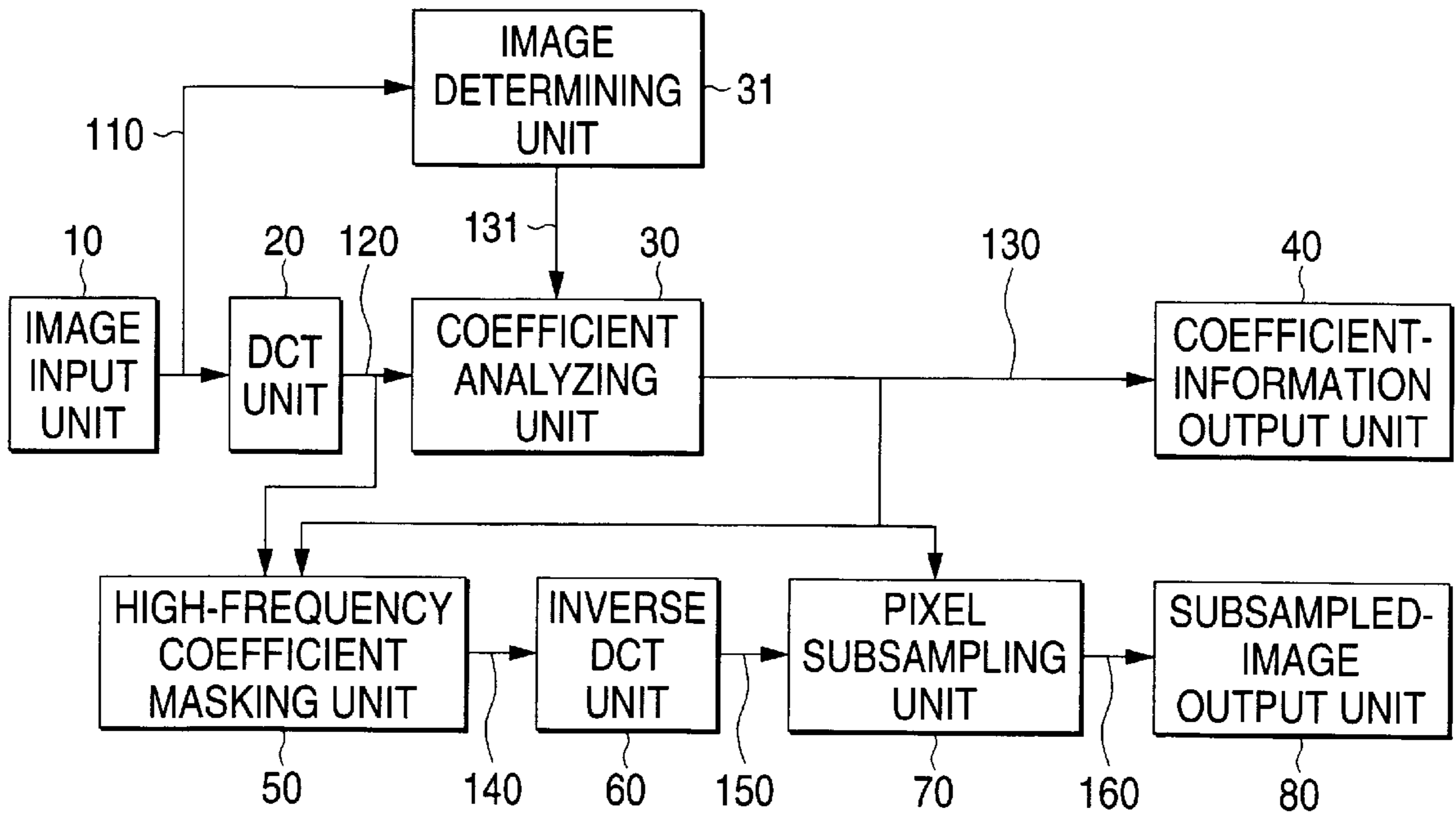
ENCODING APPARATUS FOR DYNAMICALLY CHANGING THRESHOLDS
