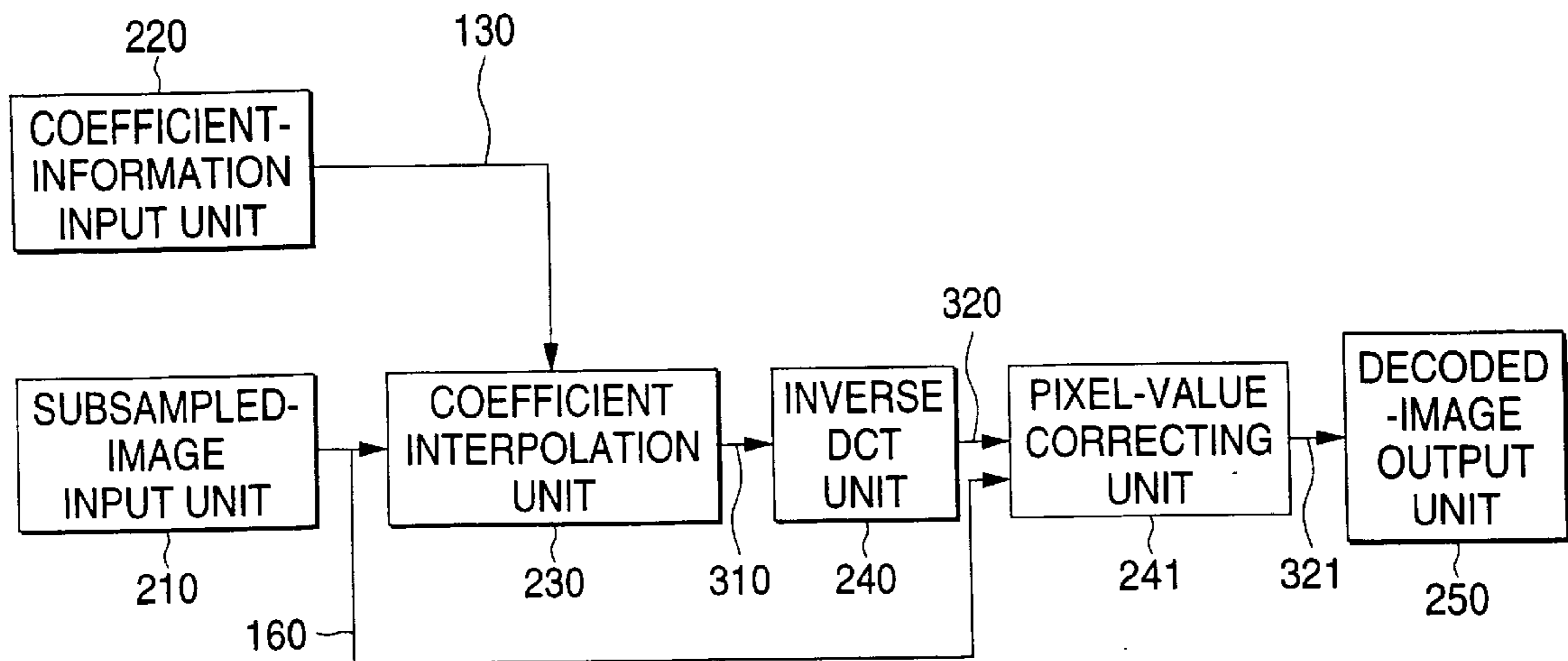
DECODER HIGHLY RESISTIVE AGAINST ALIASING IN ENCODING
