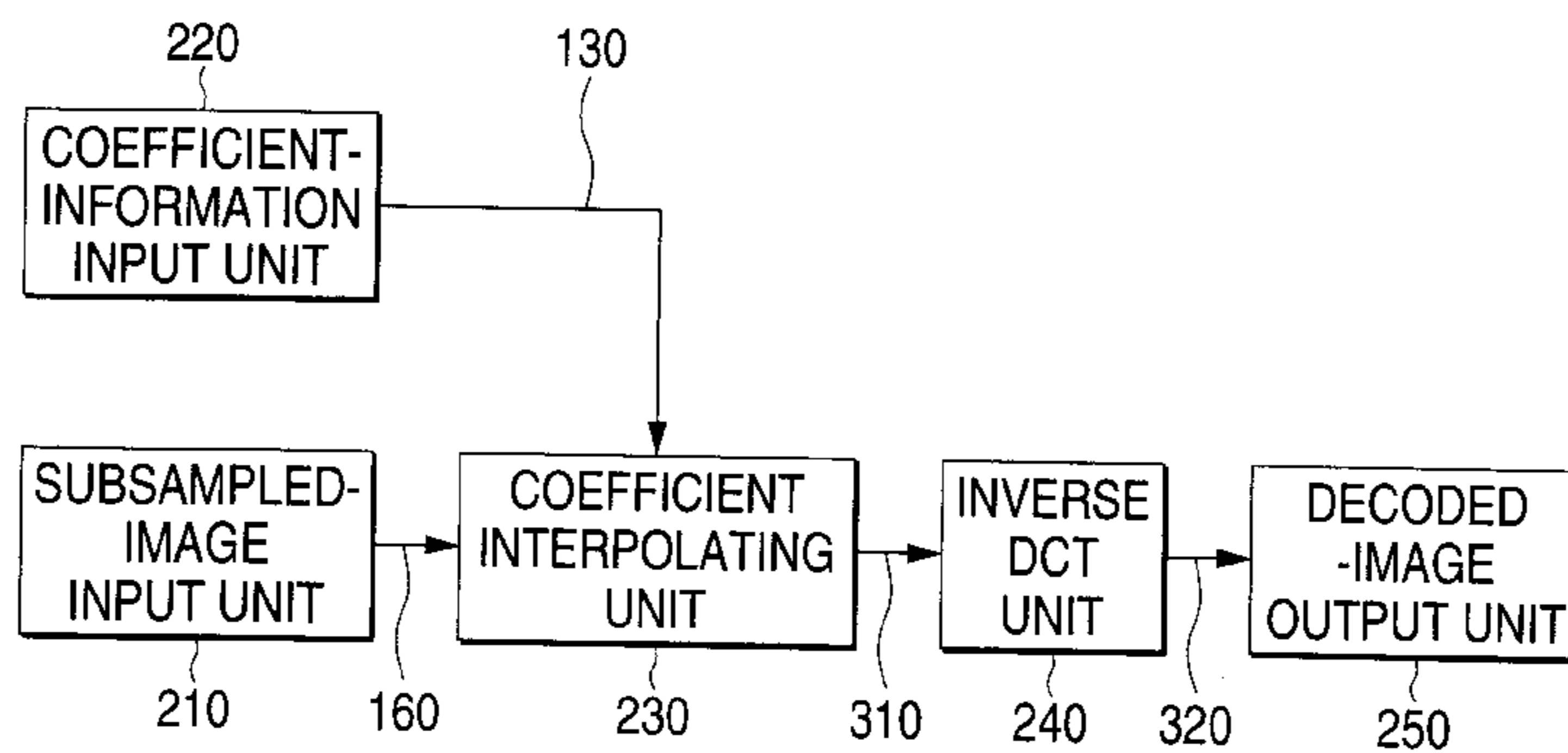
DECODING SIDE
