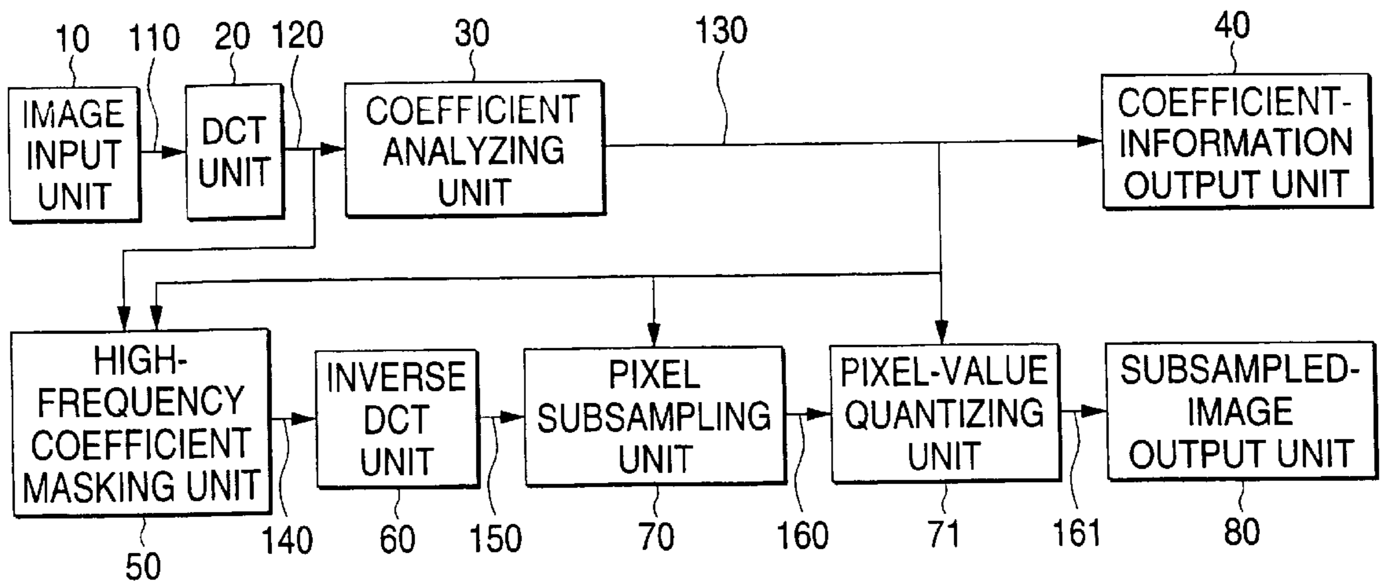
ENCODING APPARATUS FOR QUANTIZING PIXEL VALUES
