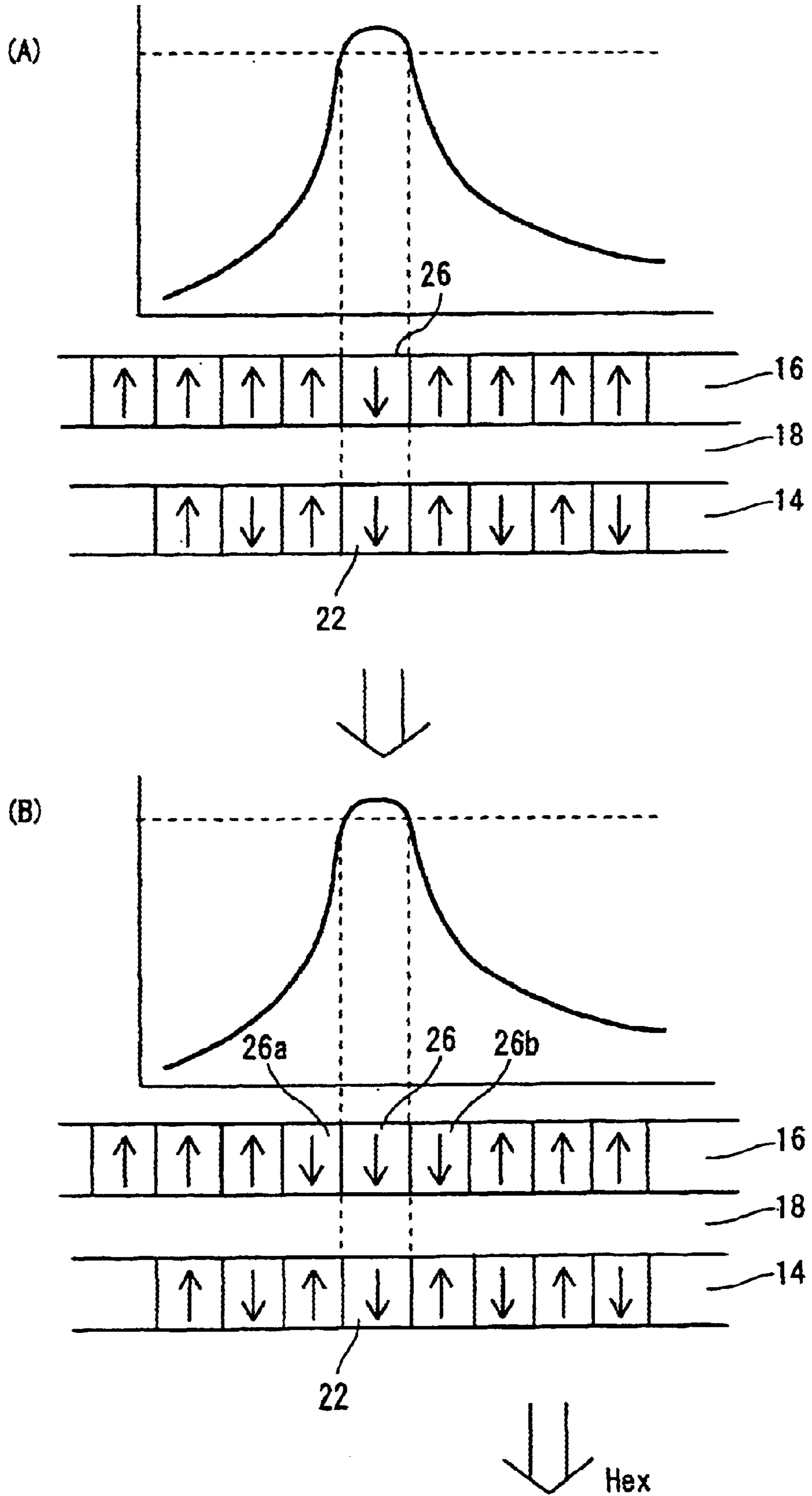
FIG. 2 PRIOR ART
