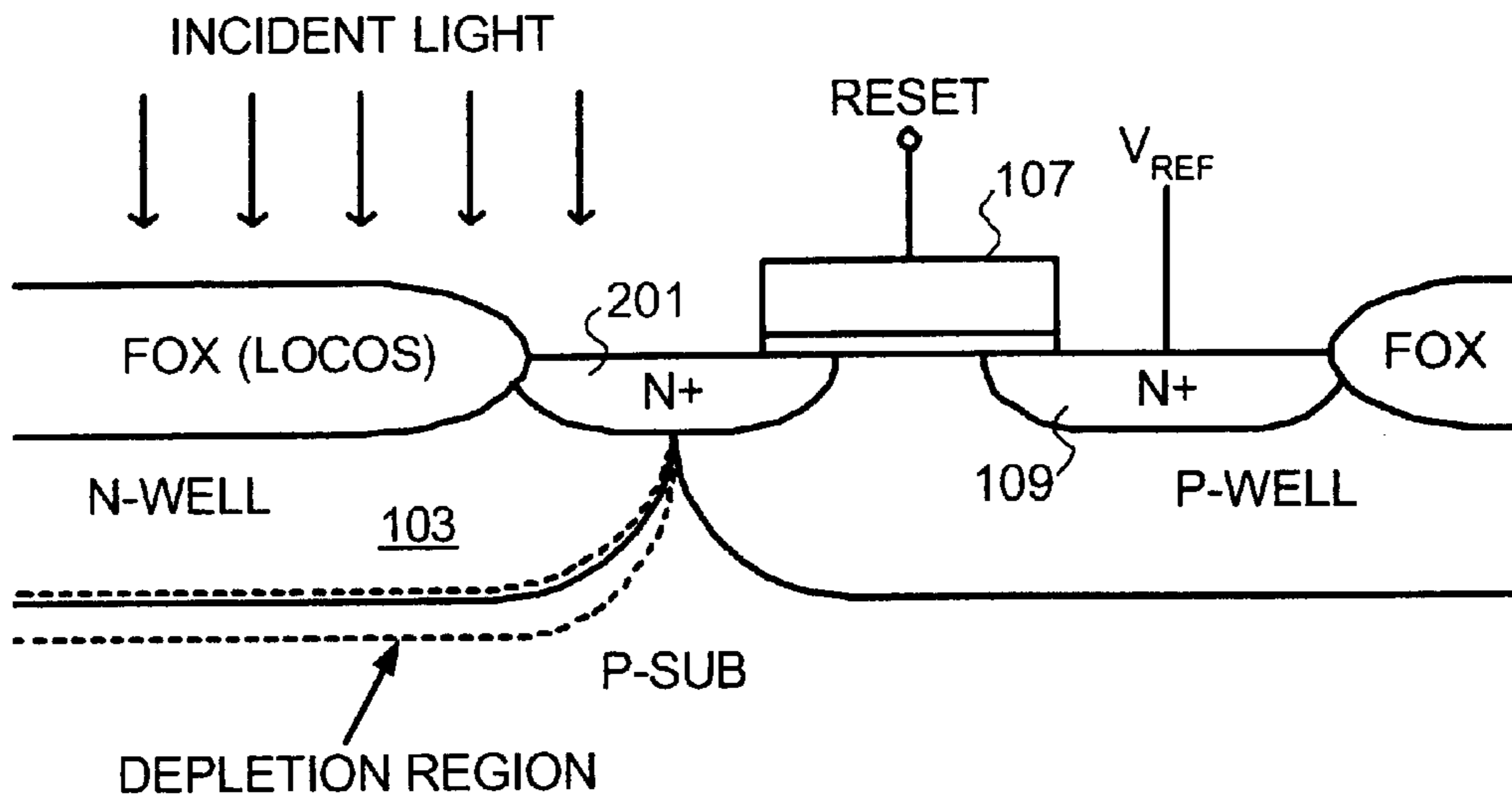
FIGURE 2 (PRIOR ART)
