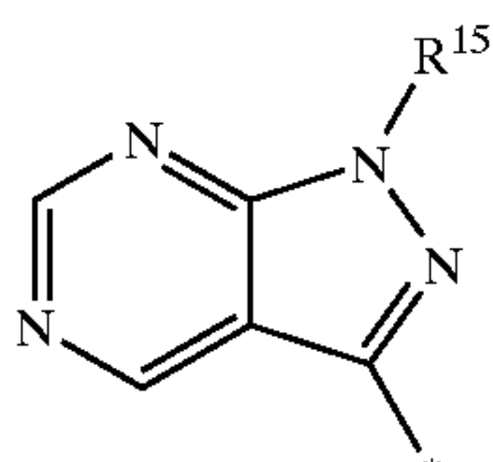
1H-pyrazolo[3,4-d]- pyrimidinyl
