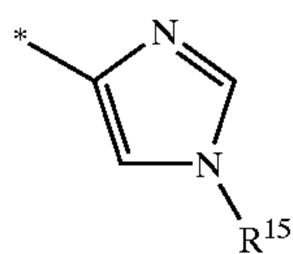
imidazol-4-yl
