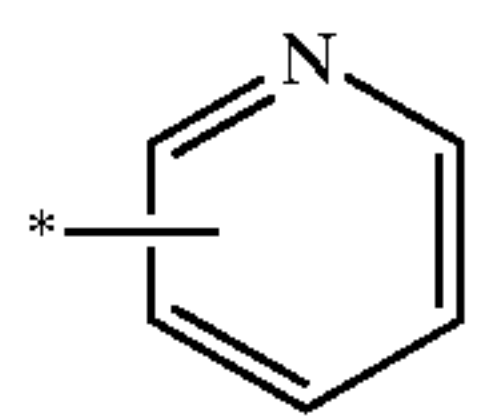
pyridyl
