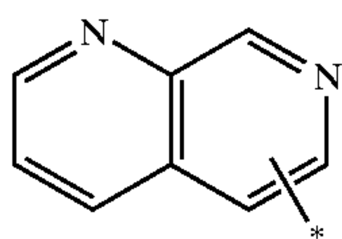
1,7-naphthyridinyl
