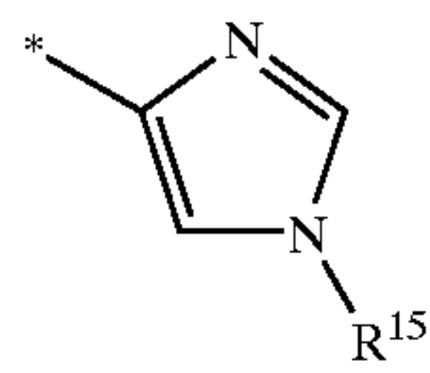
imidazol-4-yl
