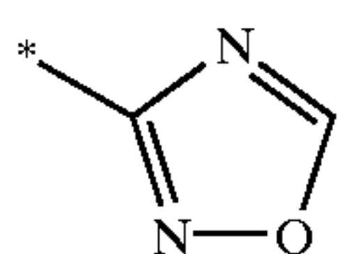
1,2,4-oxadiazol-3-yl
