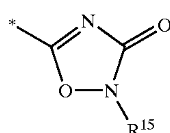
1,2,4-oxadiazol- 3-on-5-yl
