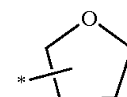
tetrahydrofuranlyl
