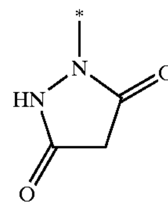
pyrazolidin-3,5-dion-1-yl
