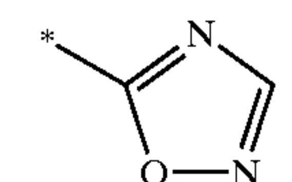
1,2,4-oxadiazol-5-yl
