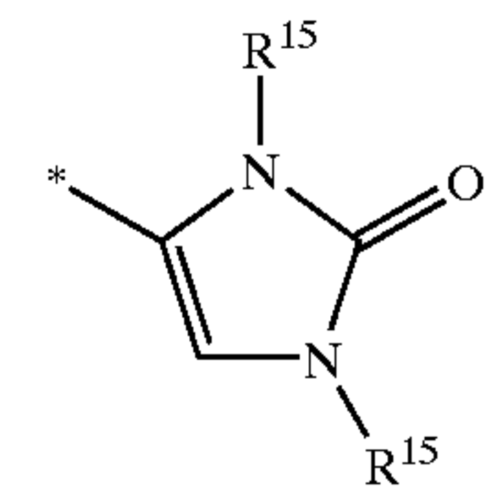
imidazolidin-2-on-4-yl
