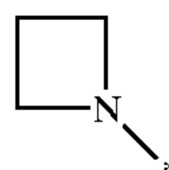
azetidin-1-yl
