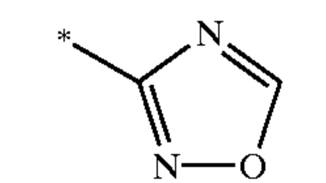
1,2,4-oxadiazol-3-yl
