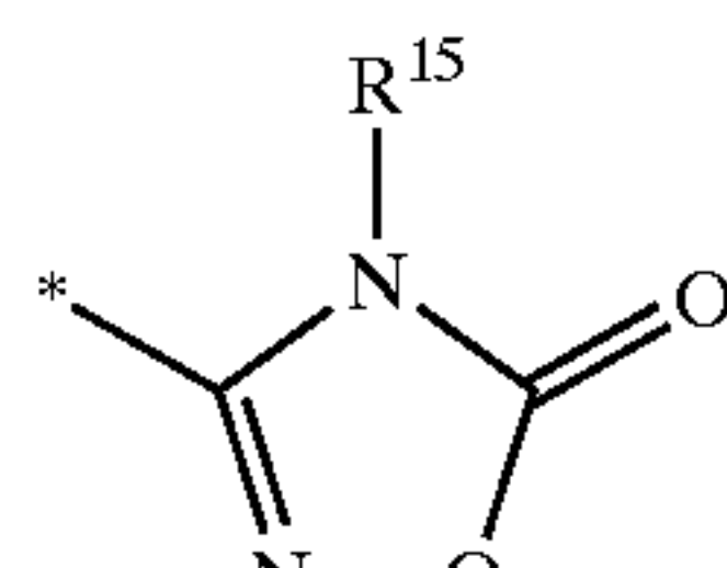
1,2,4-oxadiazol- 5-on-3-yl
