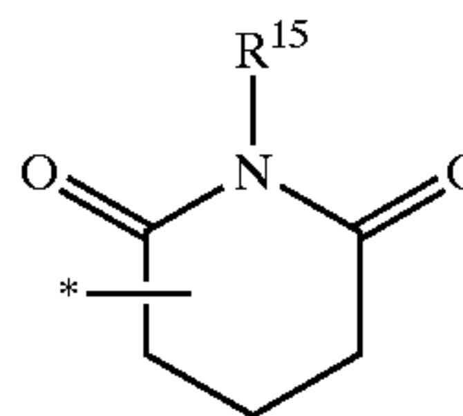
glutarimidyl
