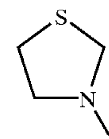
thiazolidin-3-yl
