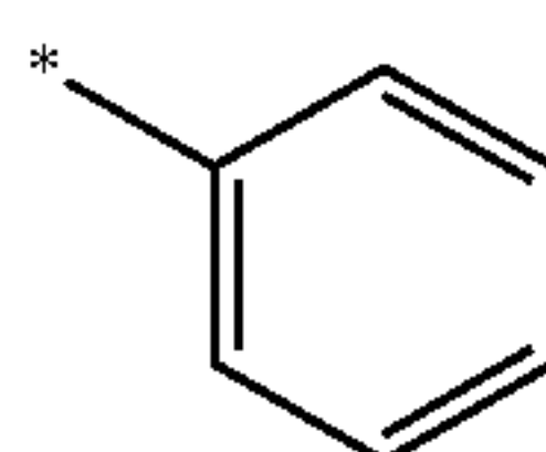
phenyl
