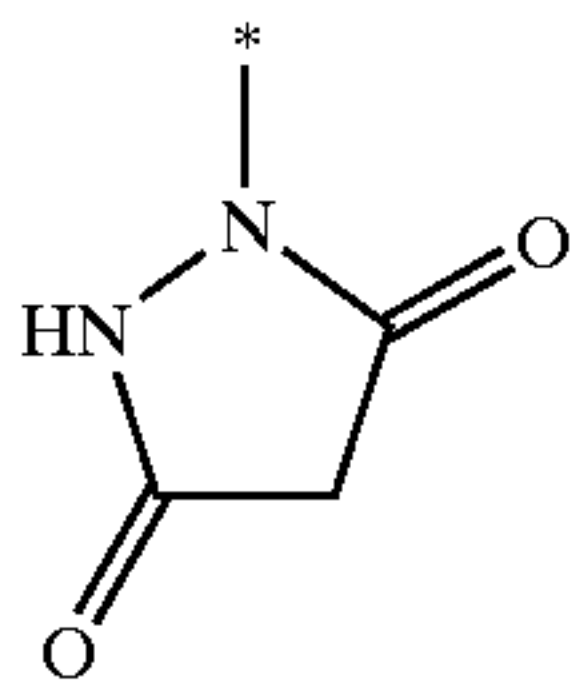
pyrazolidin-3,5-dion-1-yl
