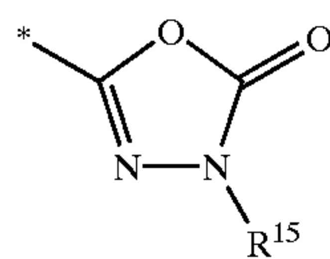
1,3,4-oxadiazol- 2-on-5-yl
