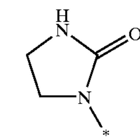
imidazolidin-2-on-1-yl
