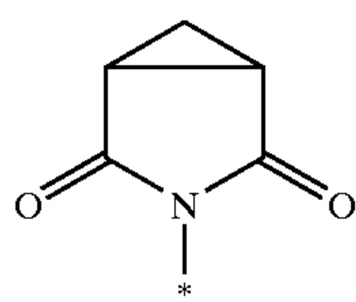
3-azabicyclo[3.1.0]-hexane-2,4-dion-3-yl
