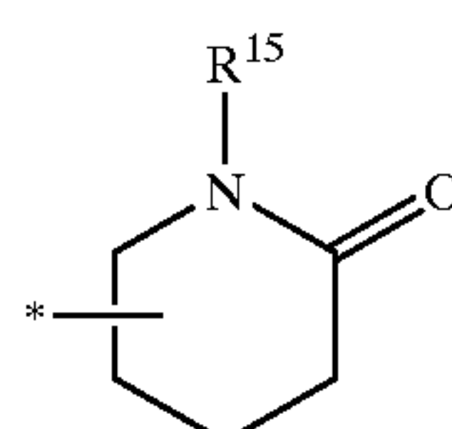
2-piperidonyl
