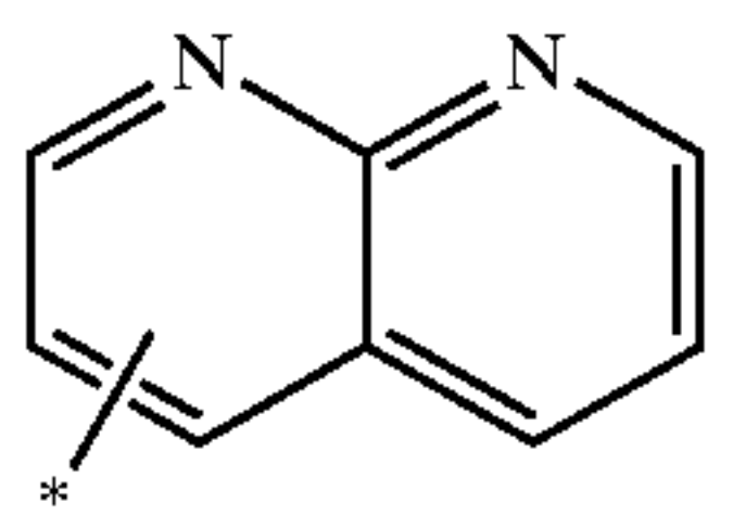
1,8-naphthyridinyl
