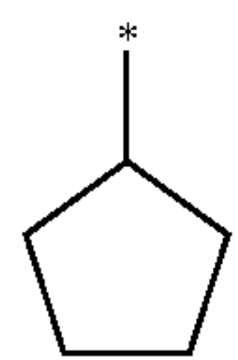
cyclopentyl
