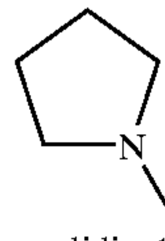
pyrrolidin-1-yl
