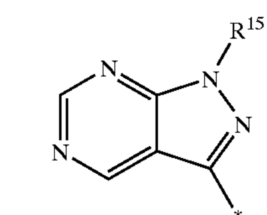
1H-pyrazolo[3,4-d]-pyrimidinyl
