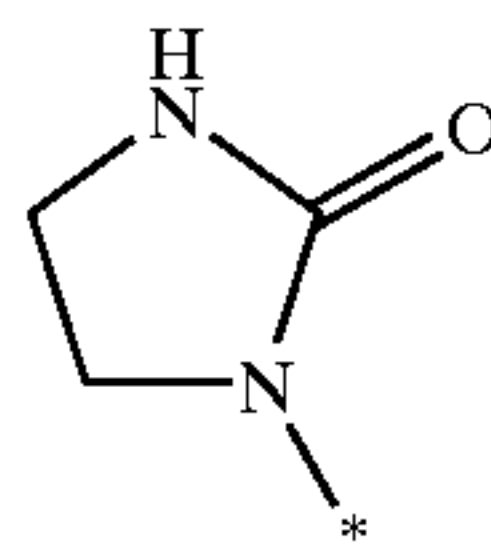
imidazolidin-2-on-1-yl
