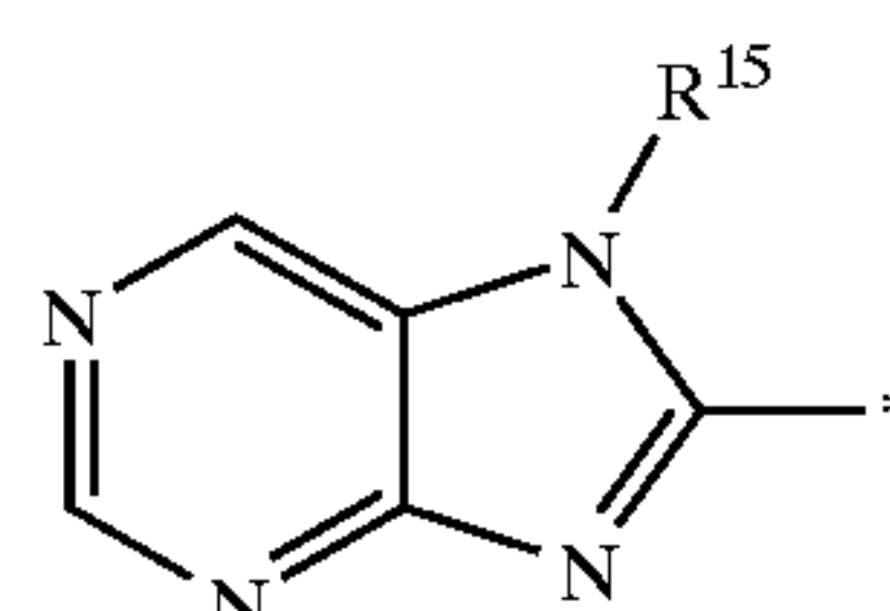
1H-puriny
