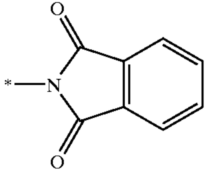
phthalimid-1-yl; 1H-isoindeole-1,3(2H)-dion-1-yl
