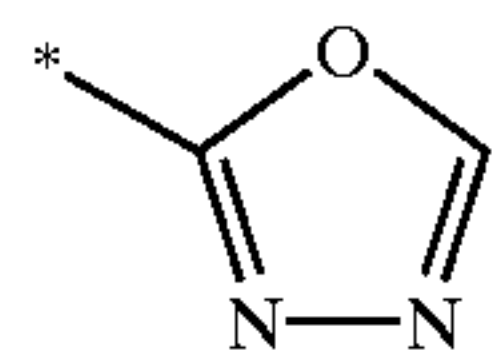
1,3,4-oxadiazolyl
