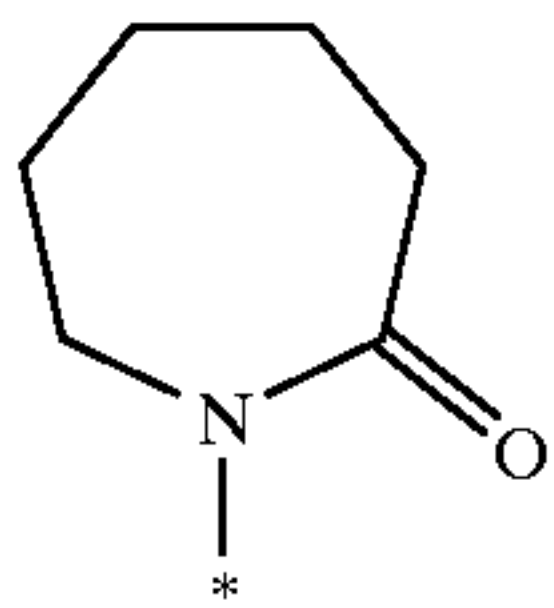
2H-azepin-2-on-1-yl
