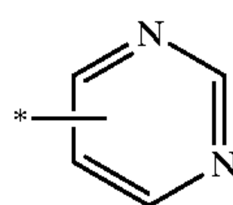
pyrimidinyl
