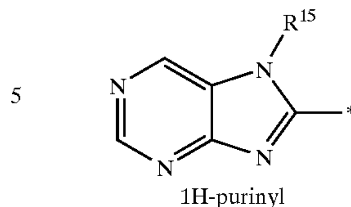
1H-purinyl
