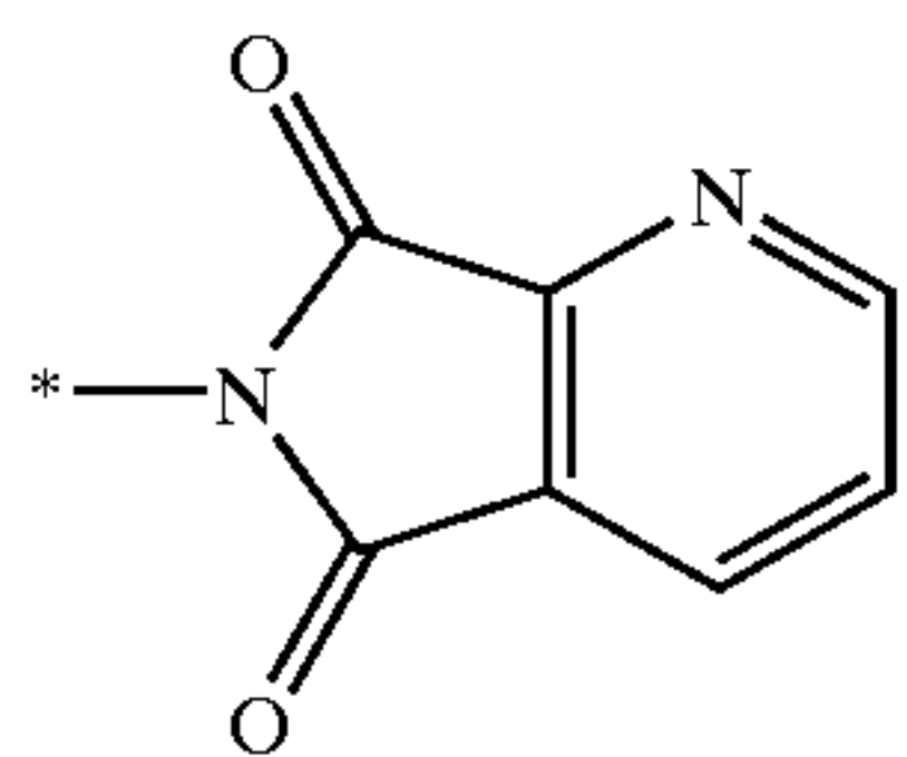
pyrrolo[3,4-b]pyridin-5,7-dion-6-yl
