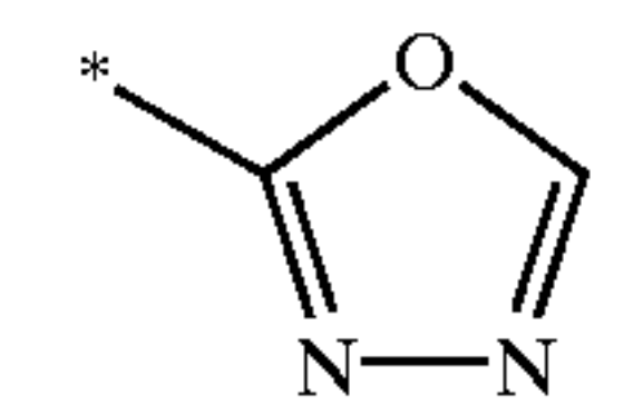
1,3,4-oxadiazolyl
