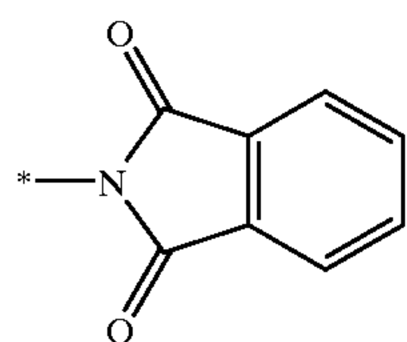
phthalimid-1-yl; 1H-isoindole-1,3(2H)-dion-1-yl
