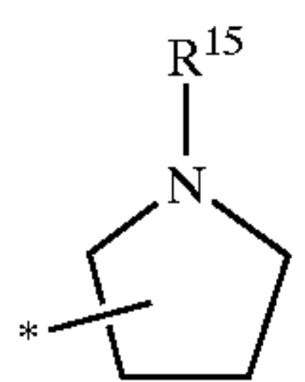
pyrrolidinyl
