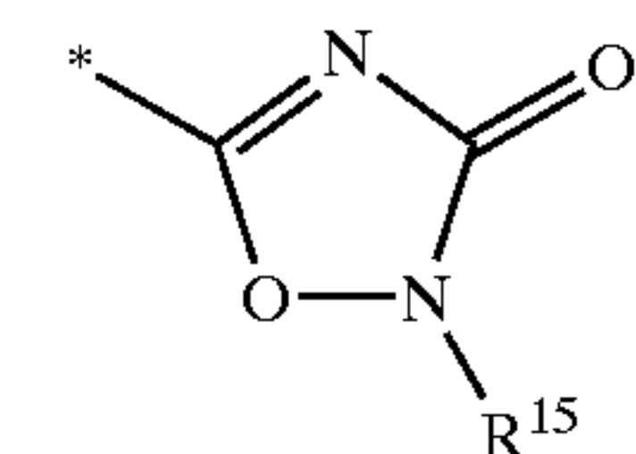
1,2,4-oxadiazol-3-on-5-yl
