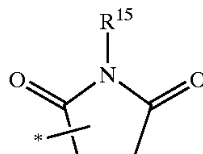
succinimidyl
