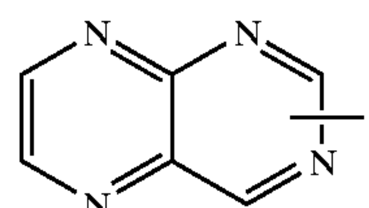
pteridinyl
