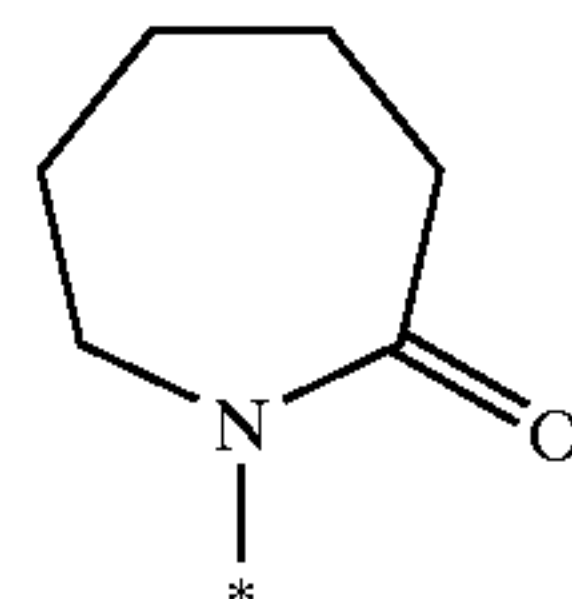
2H-azepin-2-on-1-yl
