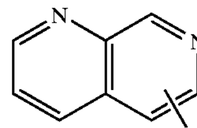
1,7-naphthyridinyl
