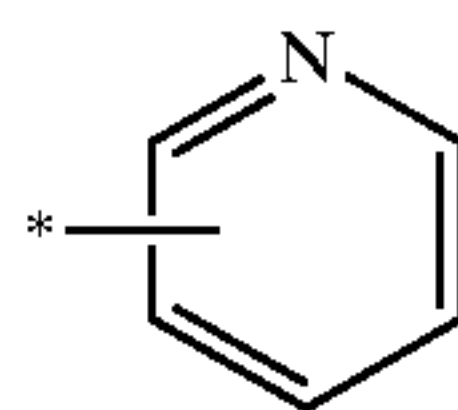
pyridyl
