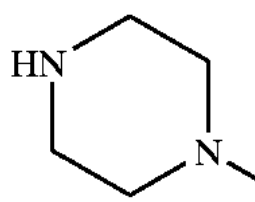
piperazin-1-yl
