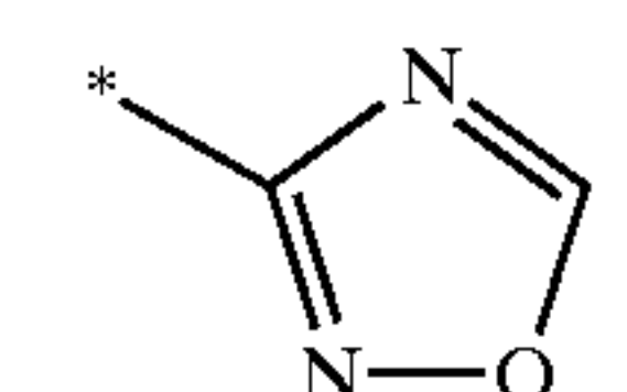
1,2,4-oxadiazol-3-yl
