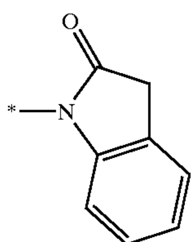
1,3-dihydro-indol-2-on-1-yl
