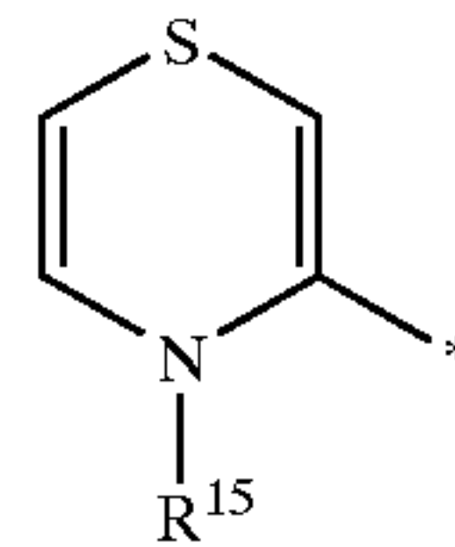
parathiazin-3-yl
