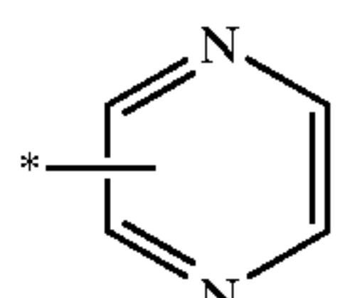
pyrazinyl
