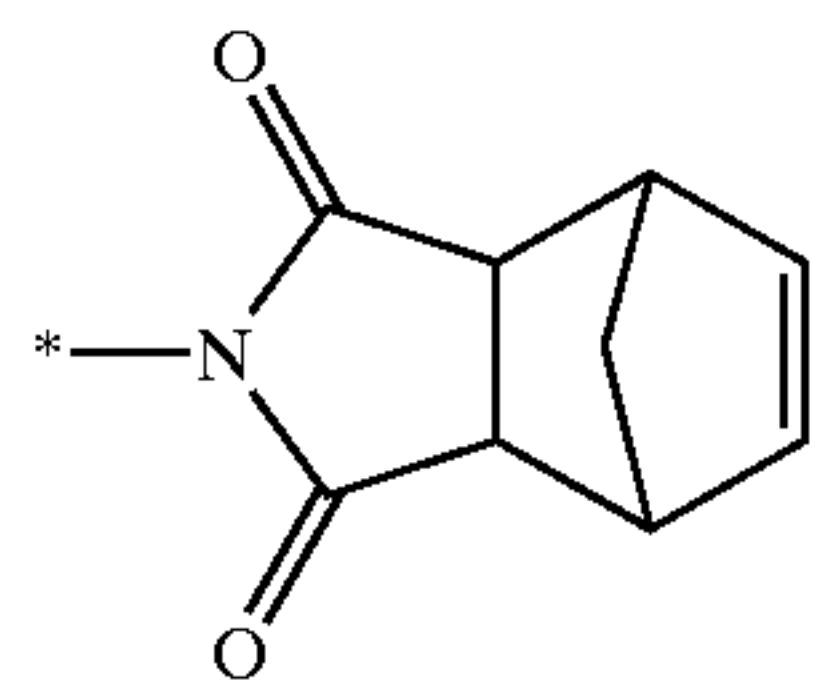
norborn-5-en-2,3-dicarboximid-1-yl
