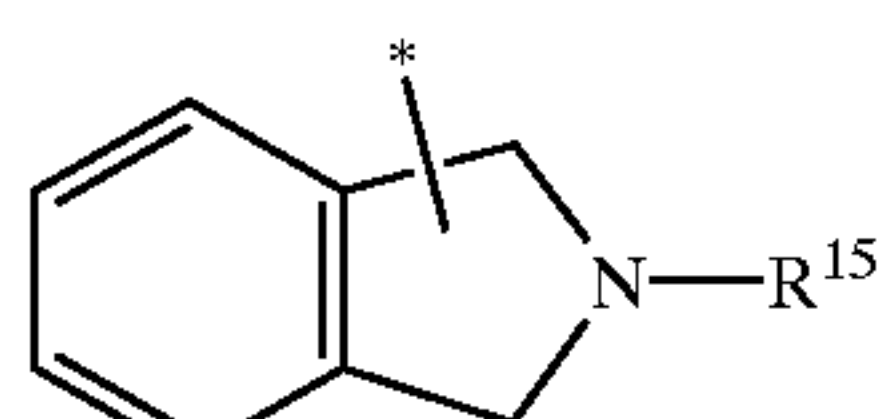
isoindolinyl
