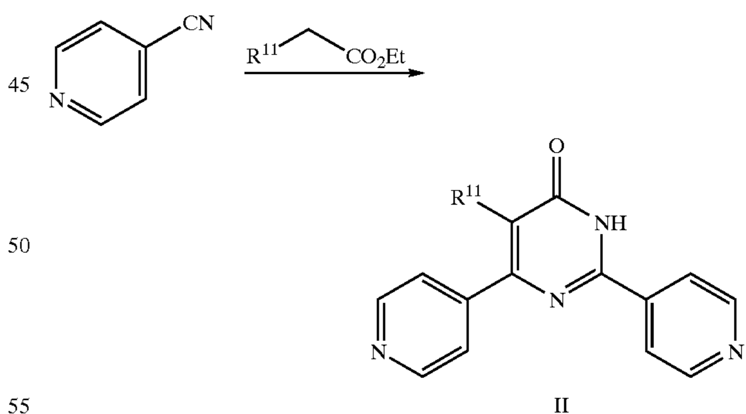
Scheme 6
