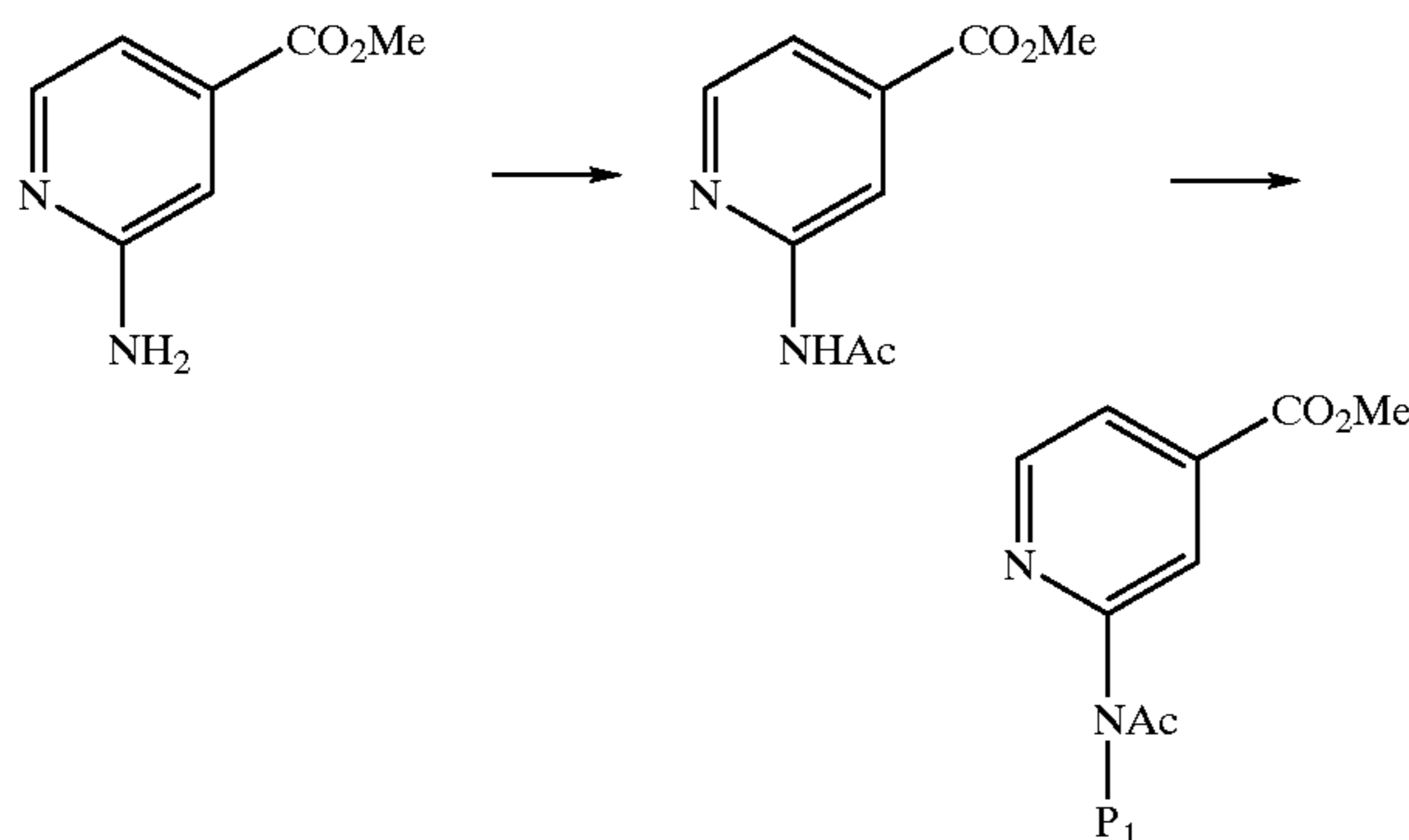
Scheme 5
