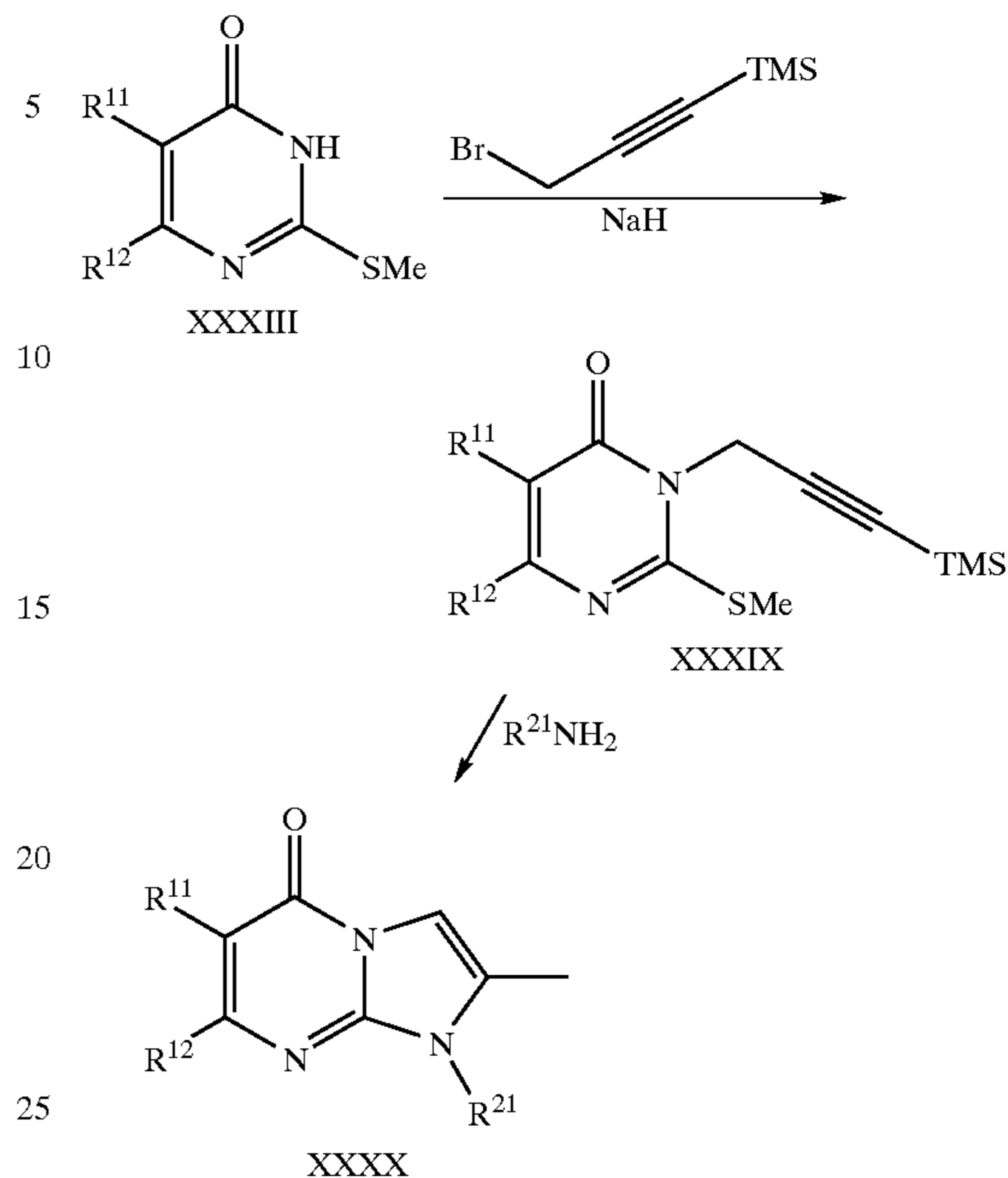
Scheme 15
