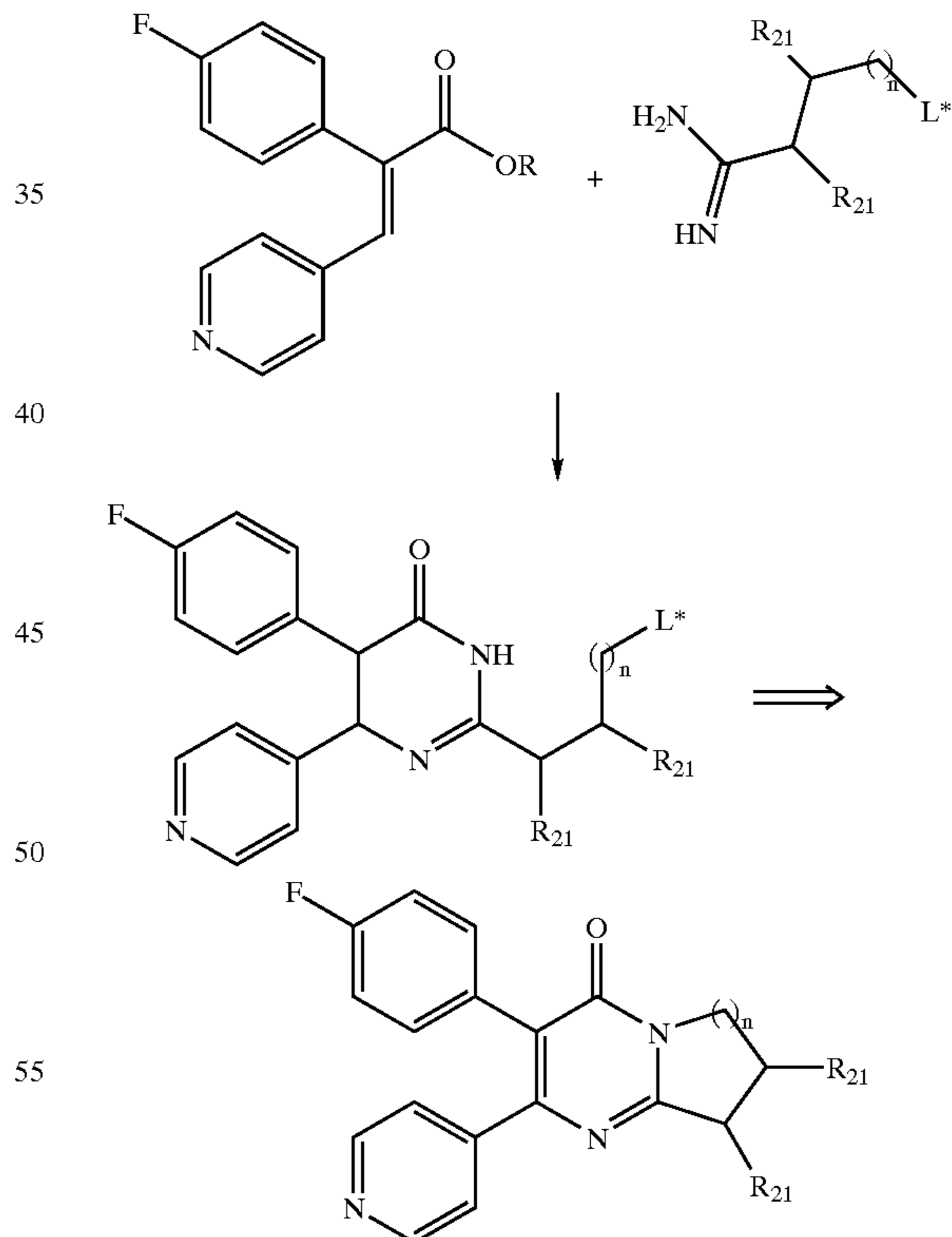
Scheme 16
