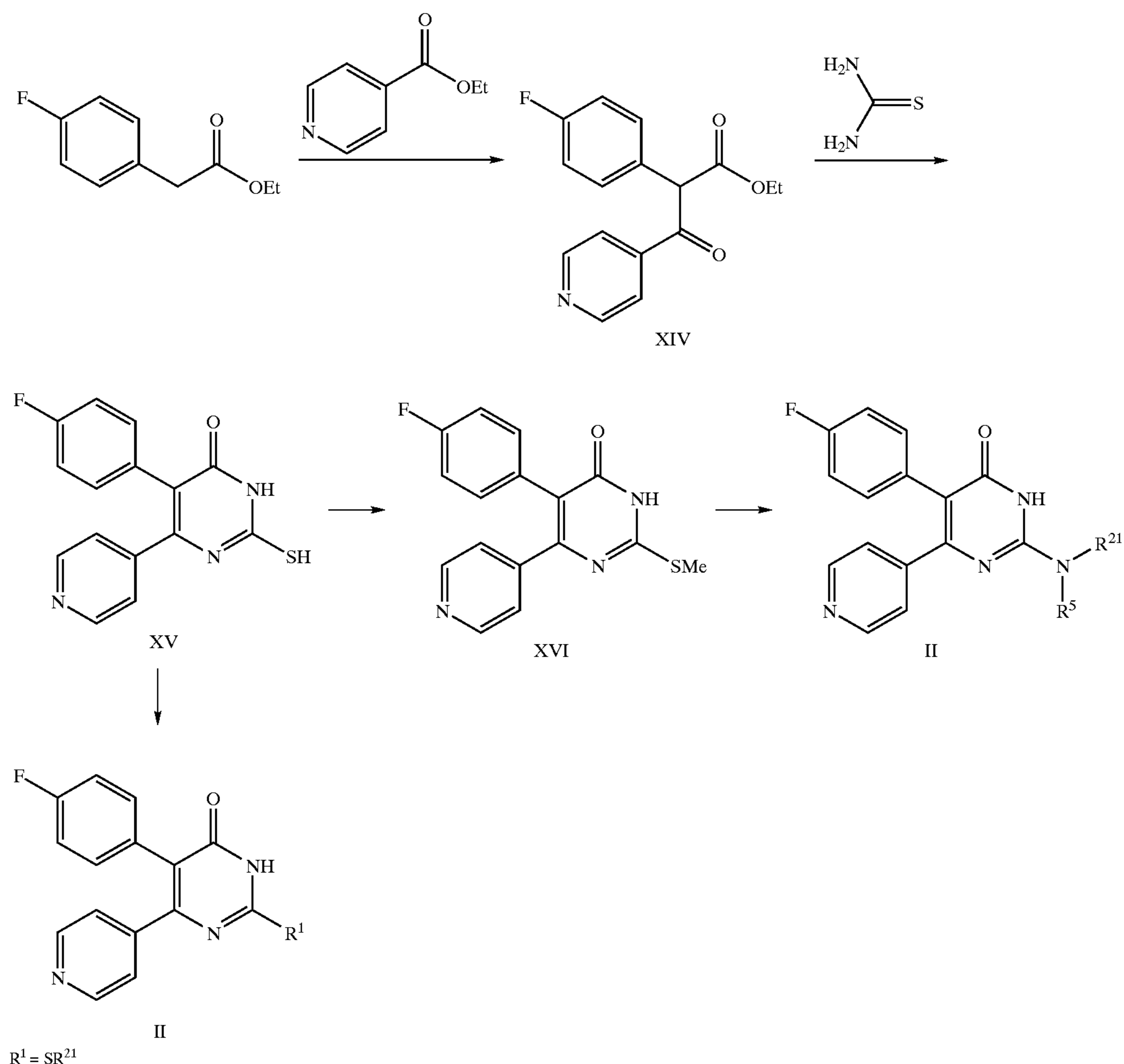
Scheme 3
