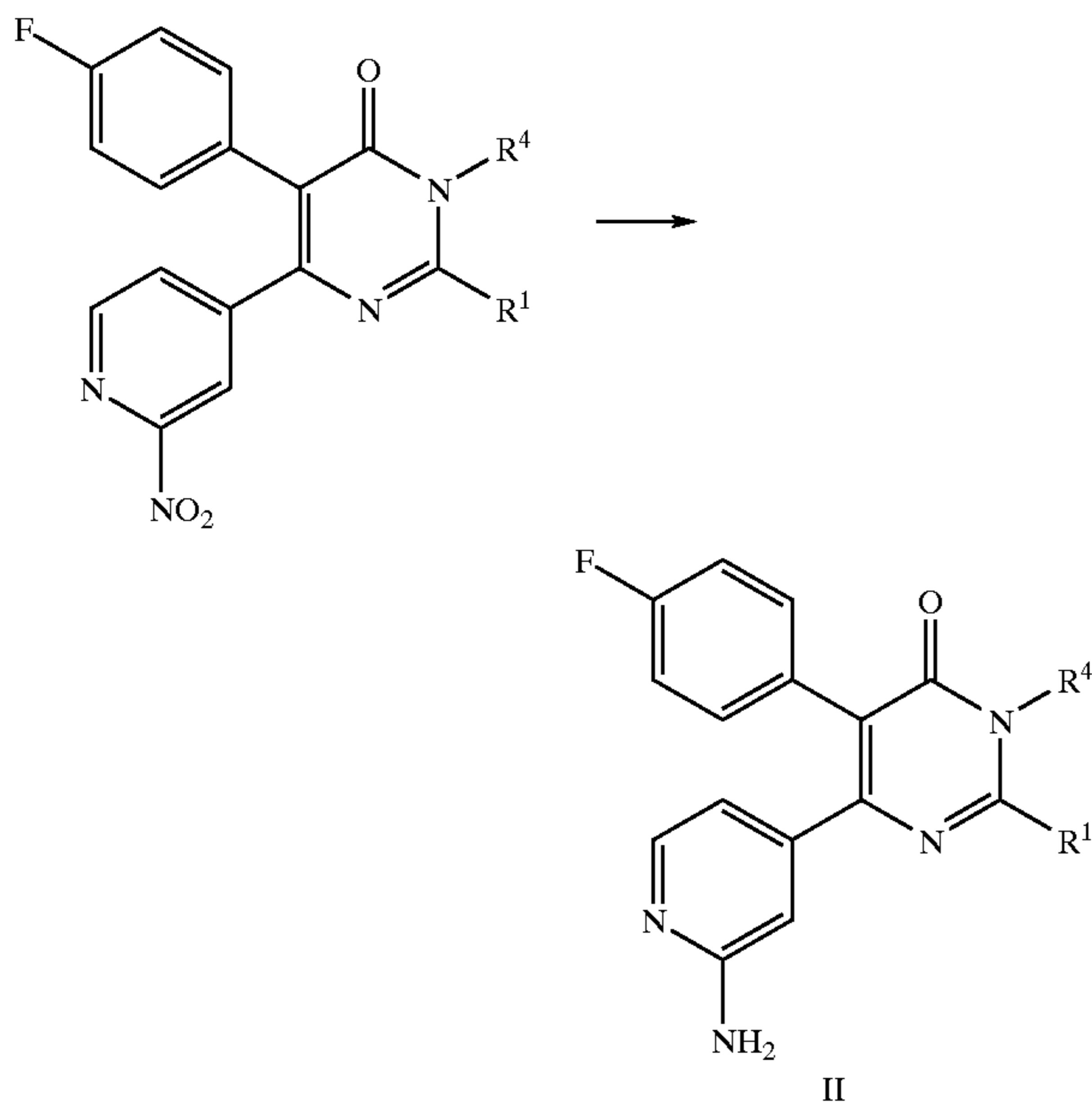
Scheme 4
