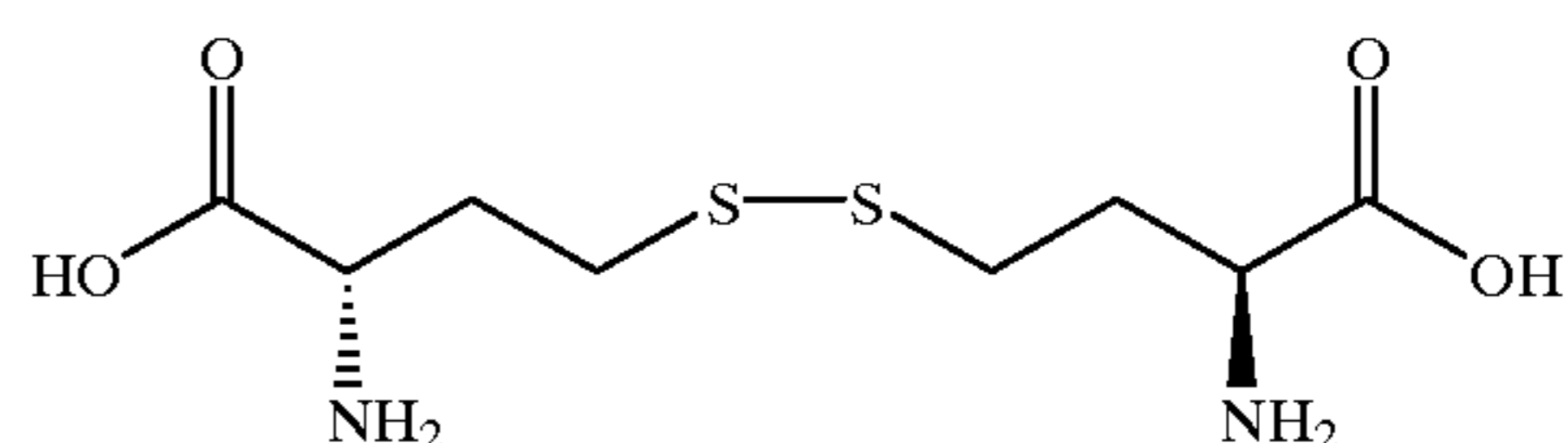
L-Homocystine MW 268.35 99.9 HI
