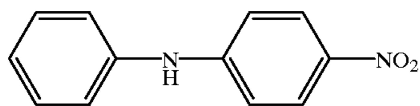
4-nitrodiphenylamine
