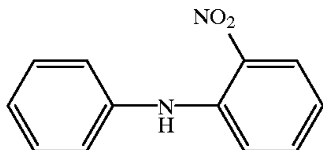
4-nitrodiphenylamine
