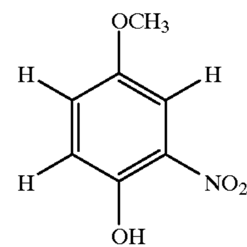
4-methoxy-2-nitrophenol
