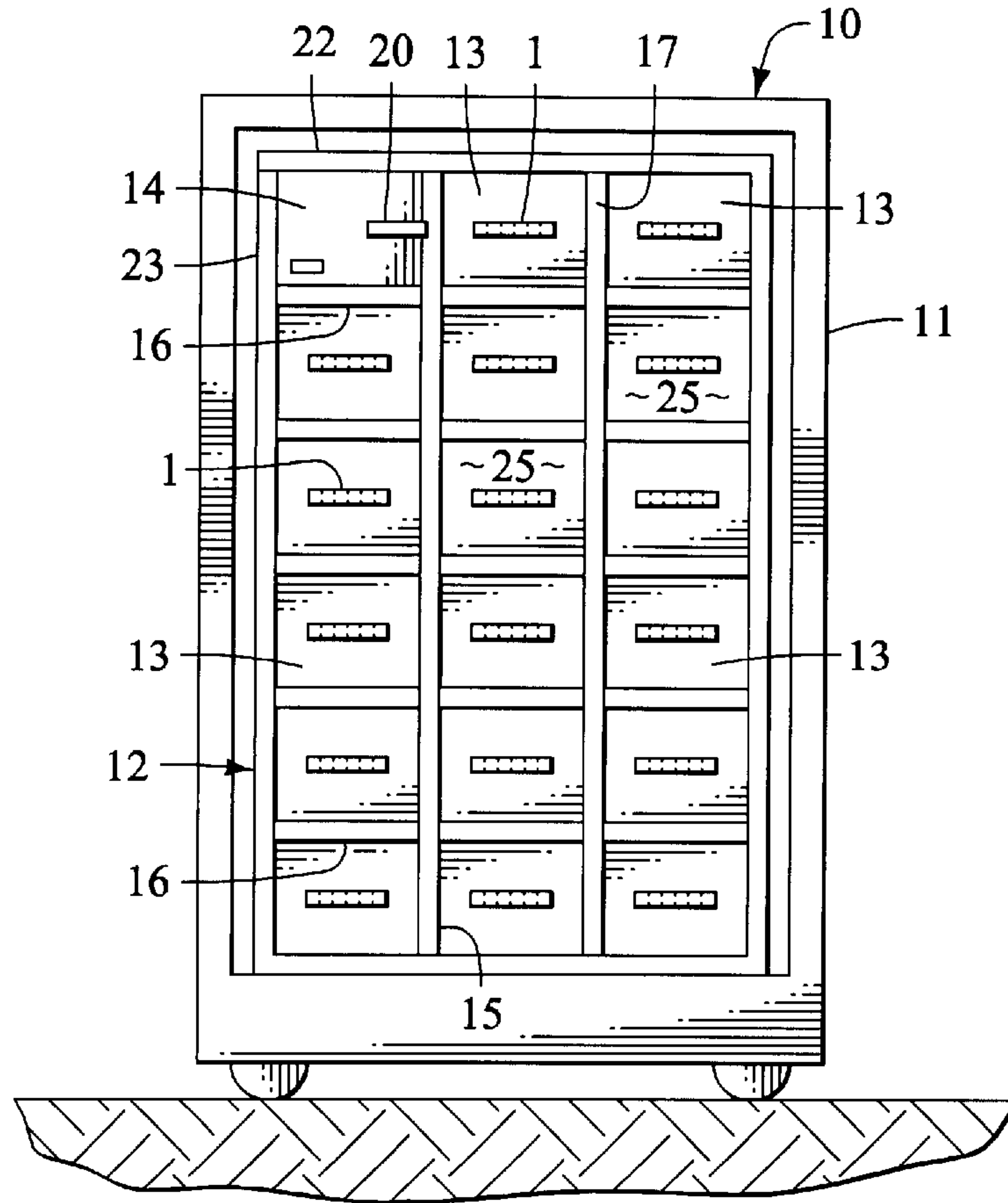
FIG. 2 PRIOR ART
