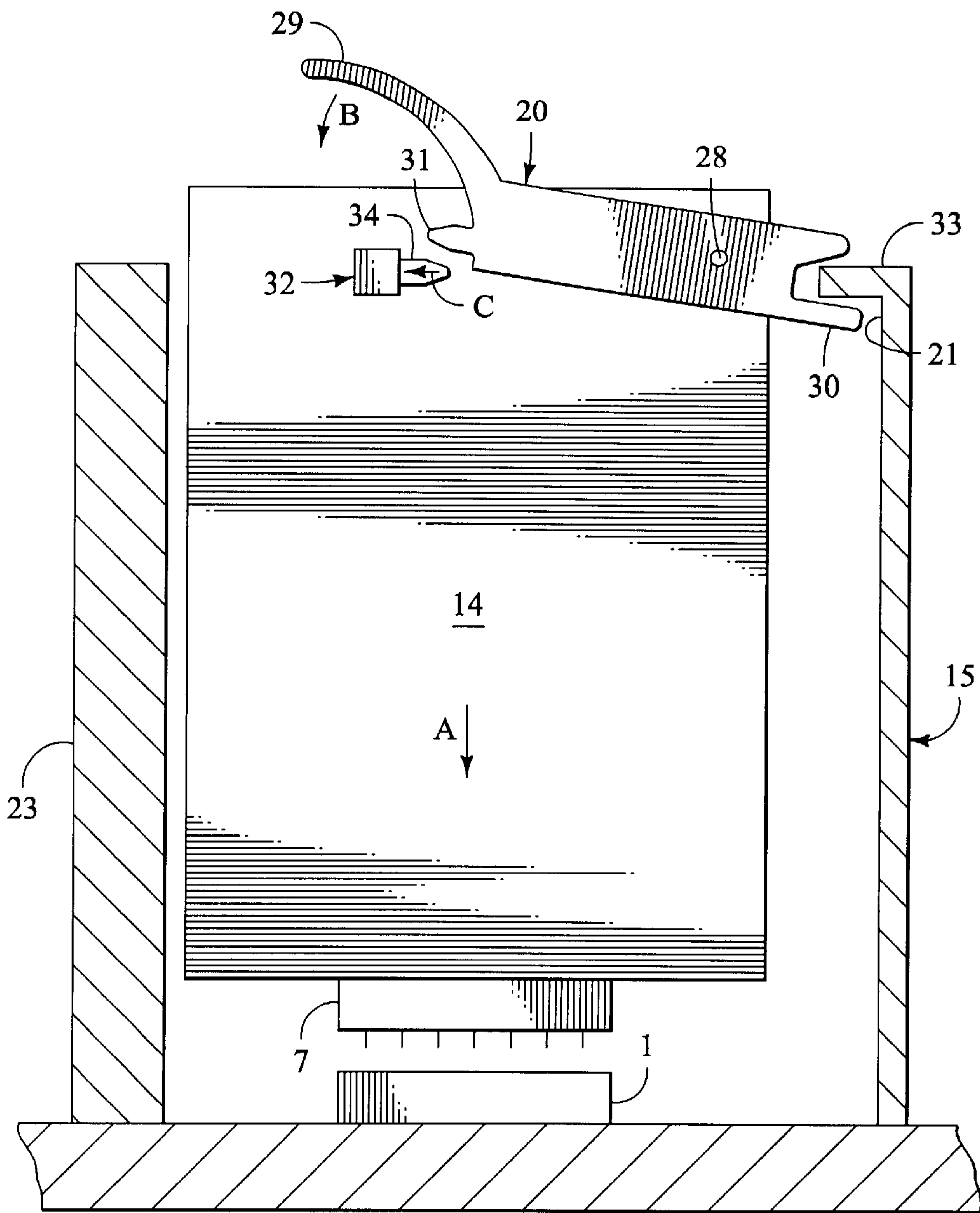
FIG.5 PRIOR ART
