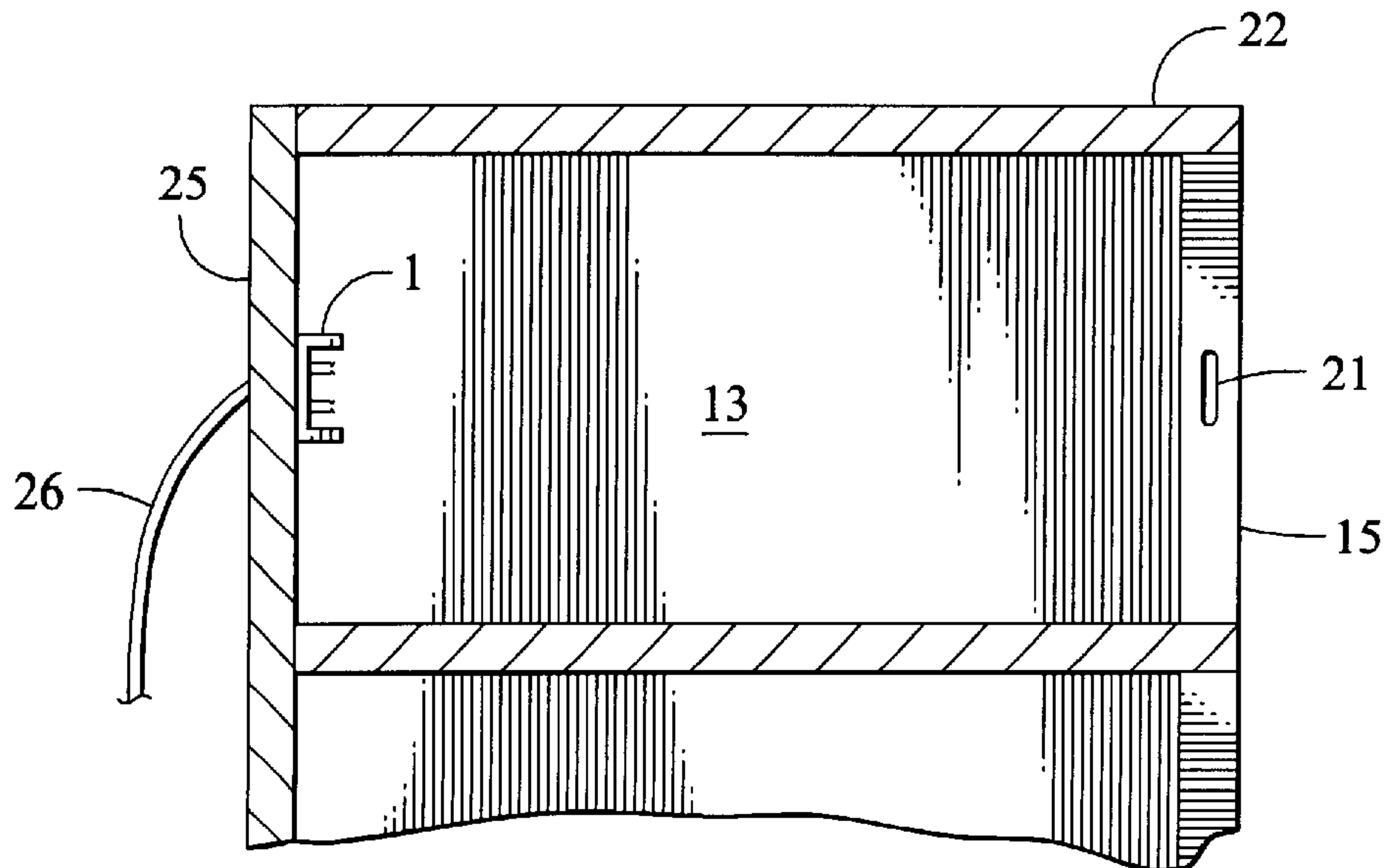
FIG. 3 PRIOR ART
