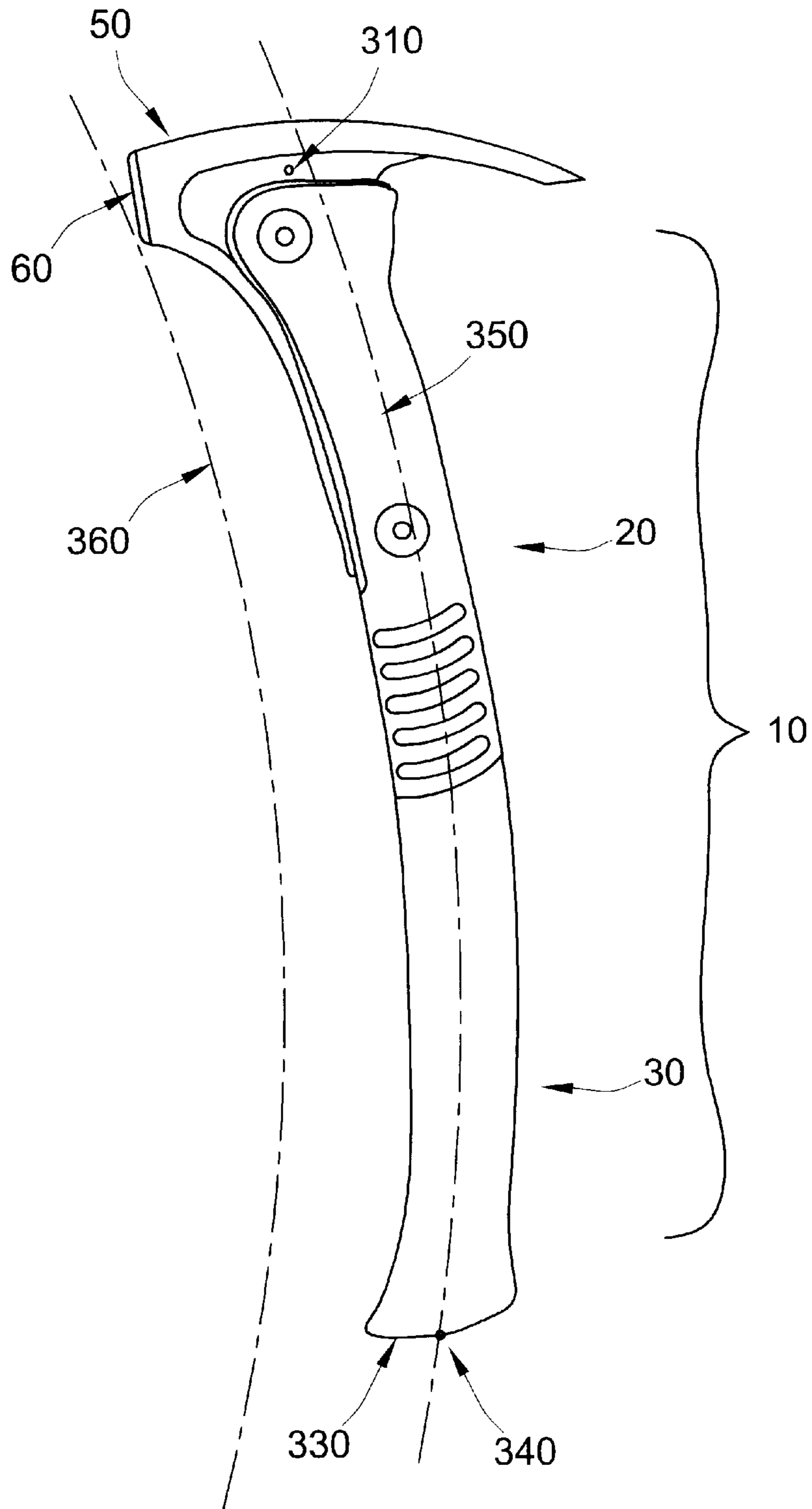
FIG. 1d
