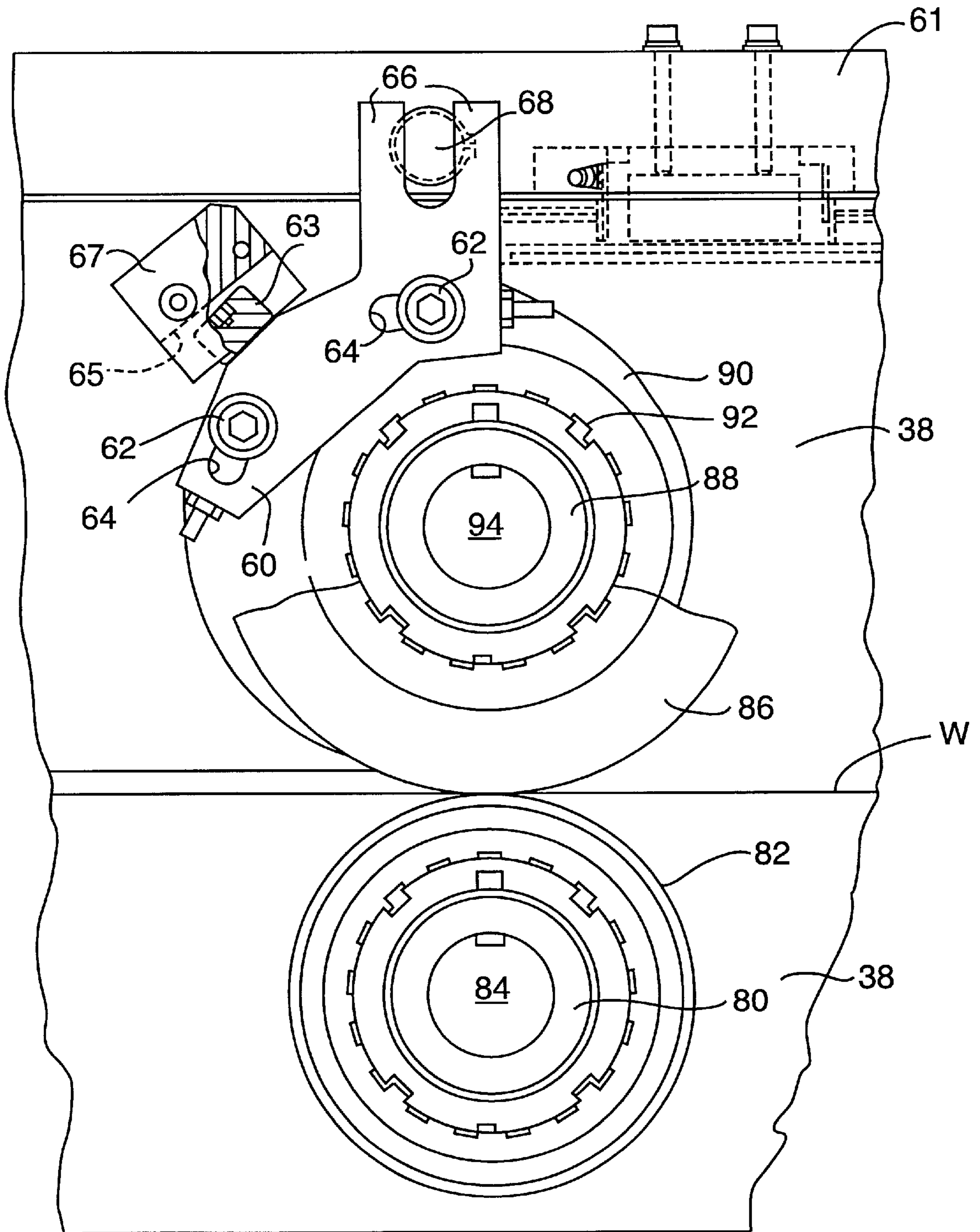
FIG. 1 PRIOR ART
