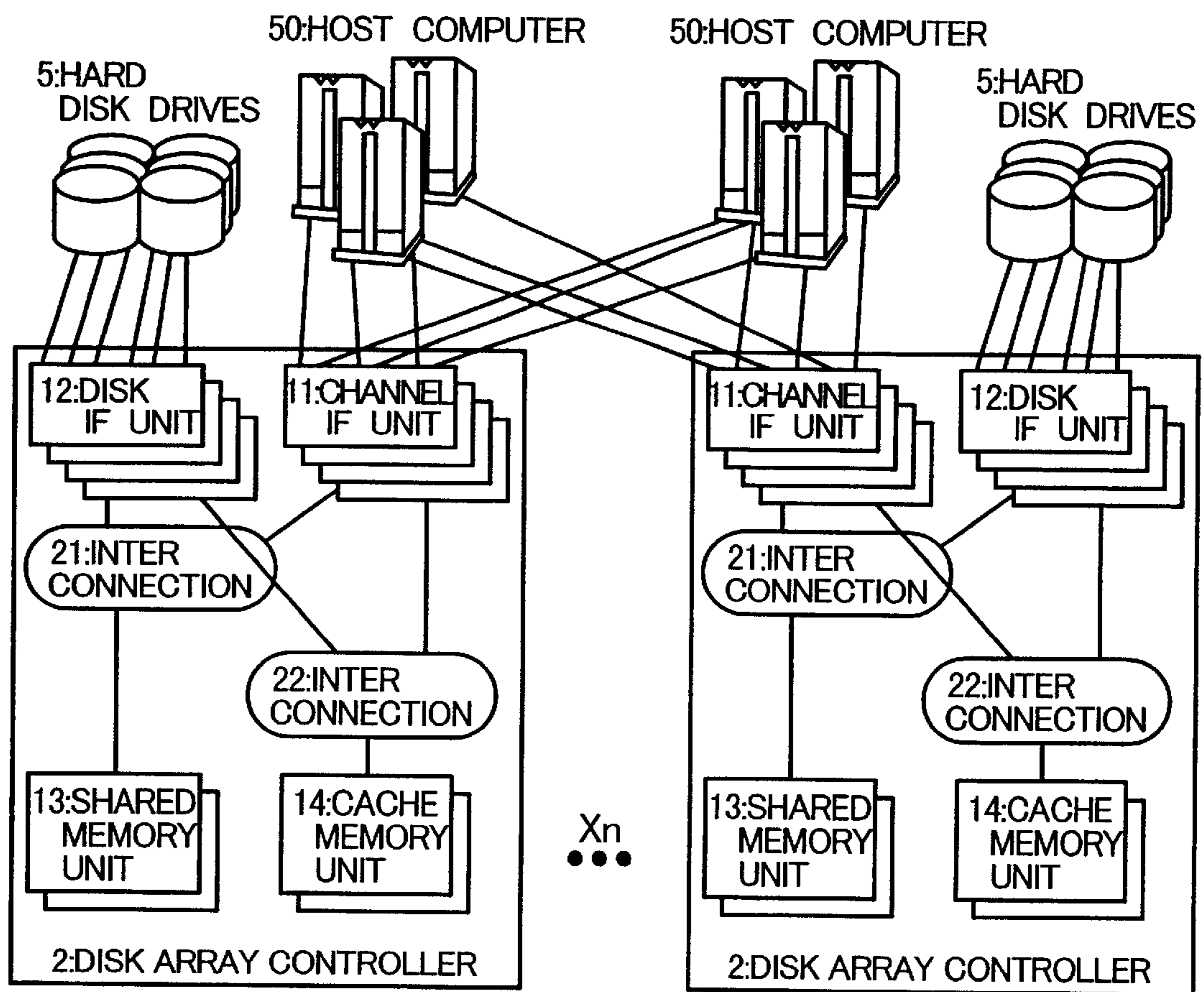
FIG.2 (PRIOR ART)
