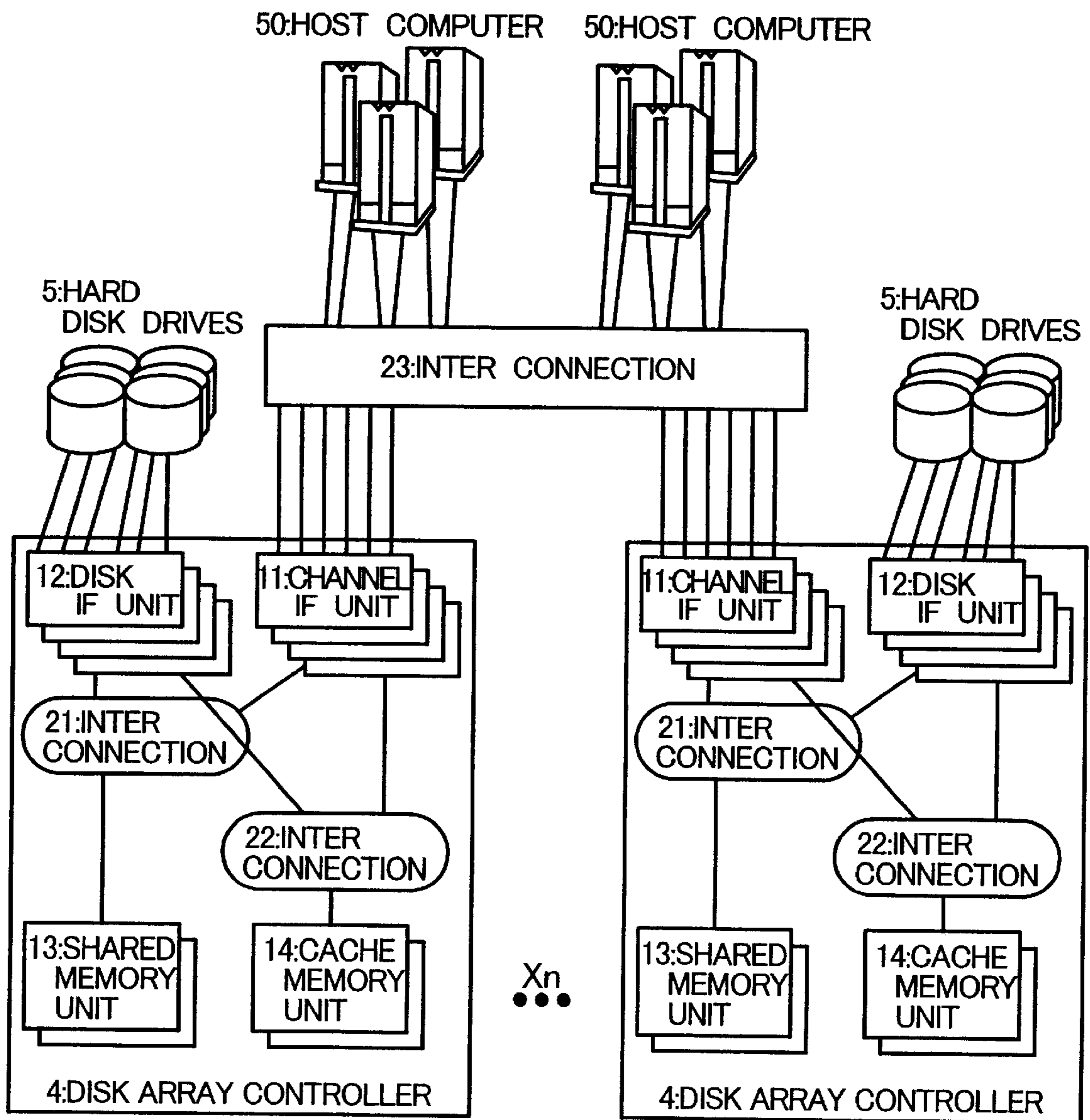
FIG.4 (PRIOR ART)
