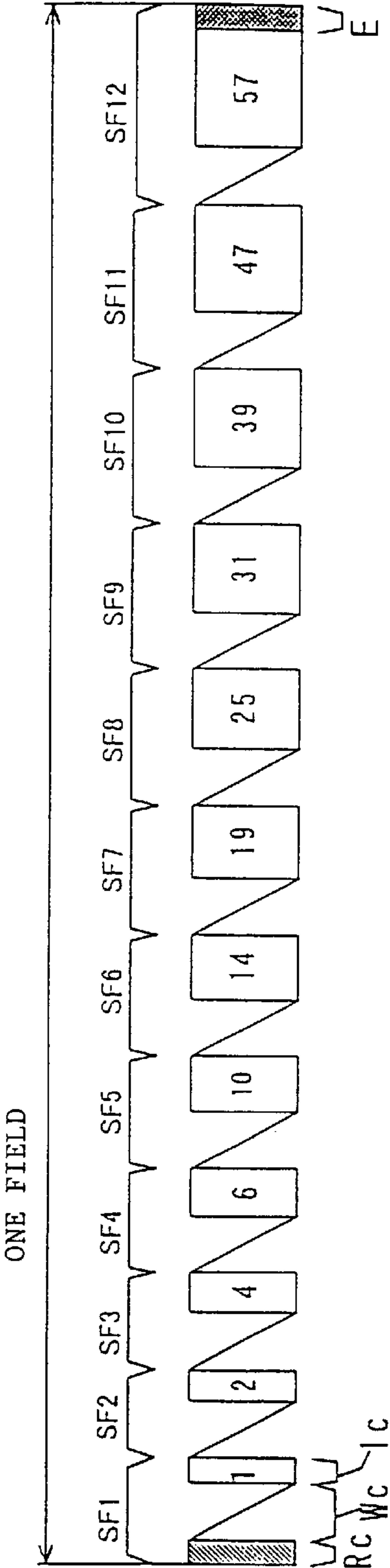
FIG. 47B EVEN FIELD (B)
