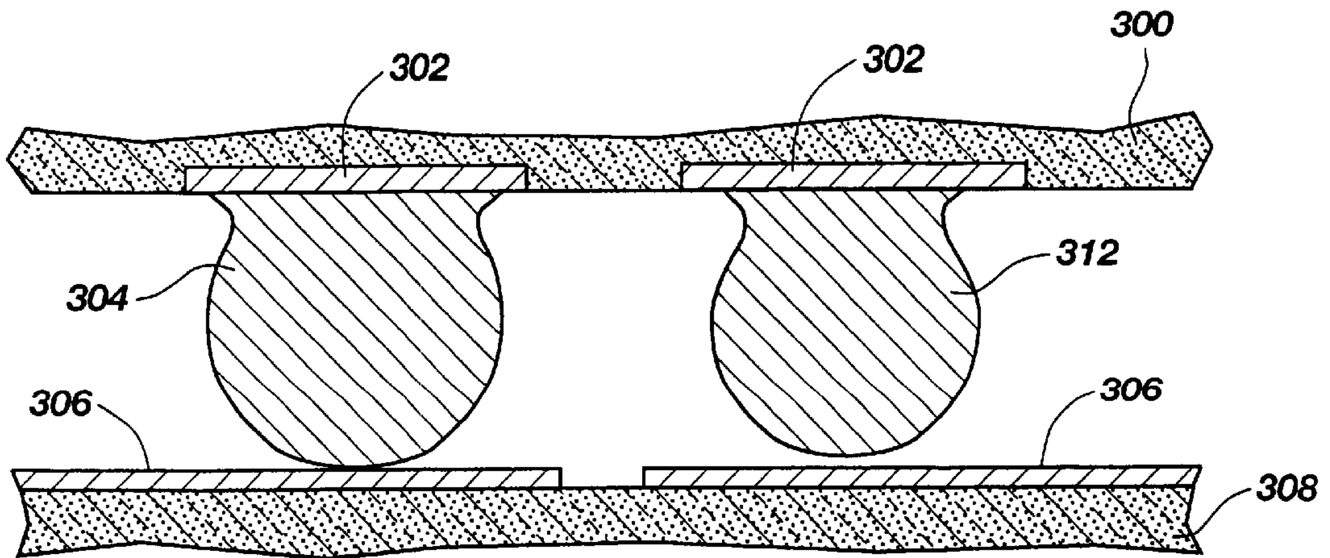
Fig. 32 (PRIOR ART)
