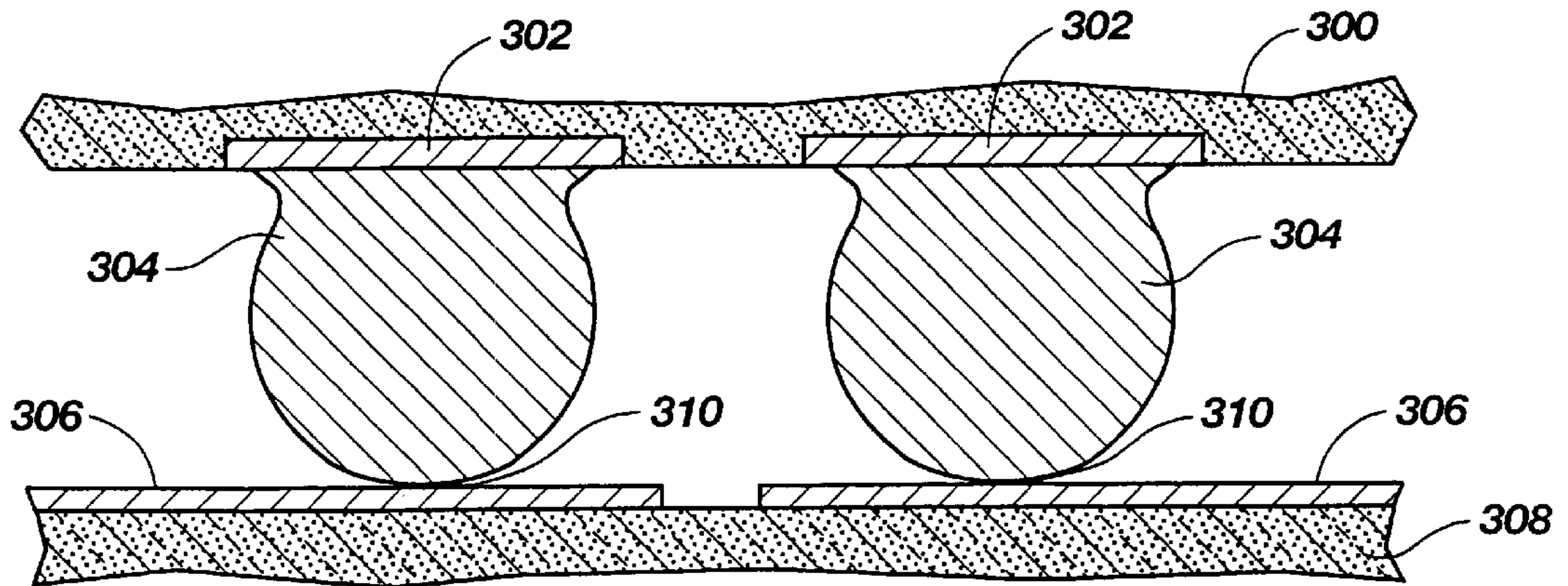
Fig. 31 (PRIOR ART)
