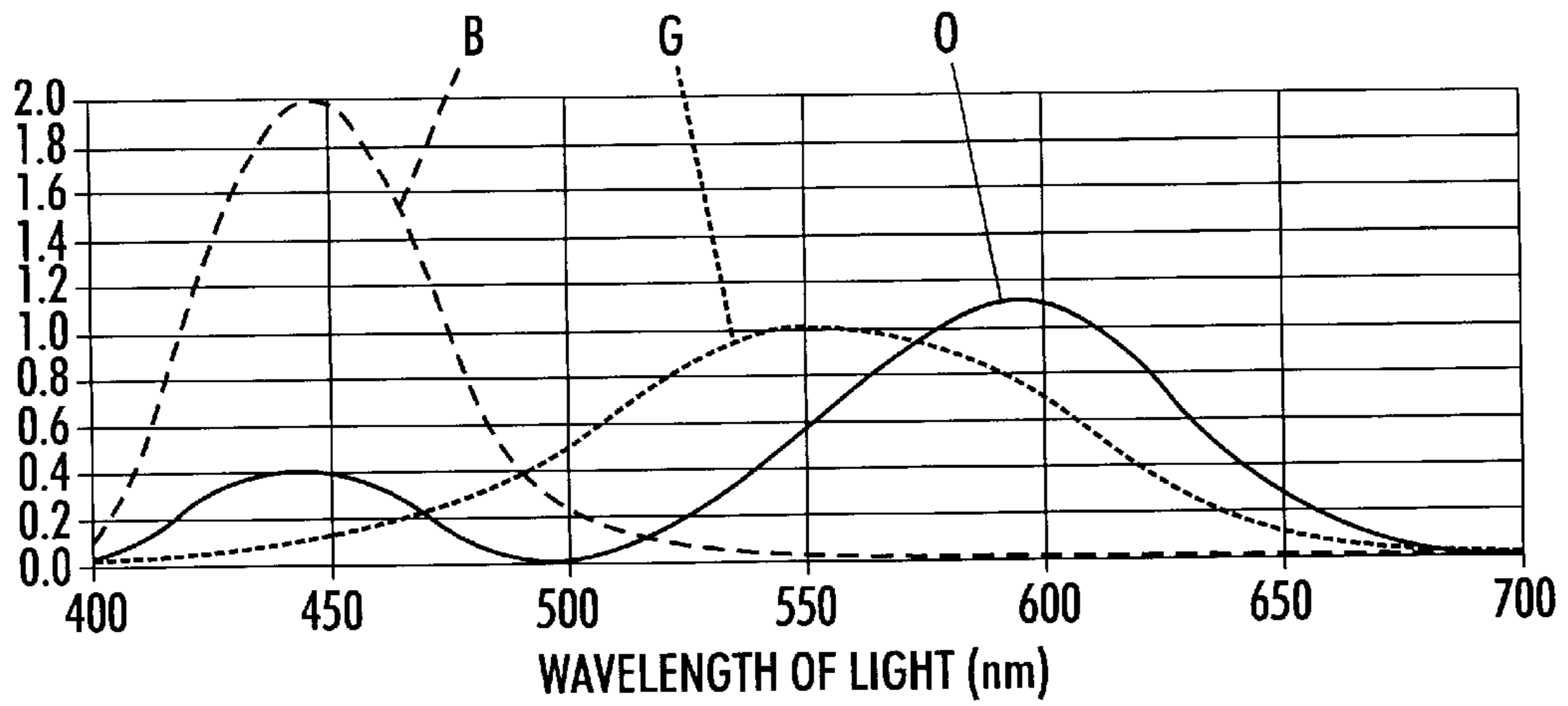
FIG. 3 PRIOR ART
