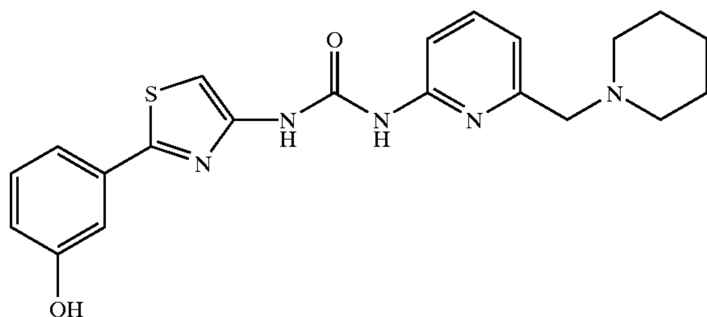
1-[2-(3-Hydroxyphenyl)thiazol-4-yl]-3-(6-piperidin-1-ylmethyl-pyridin-2-yl)urea
