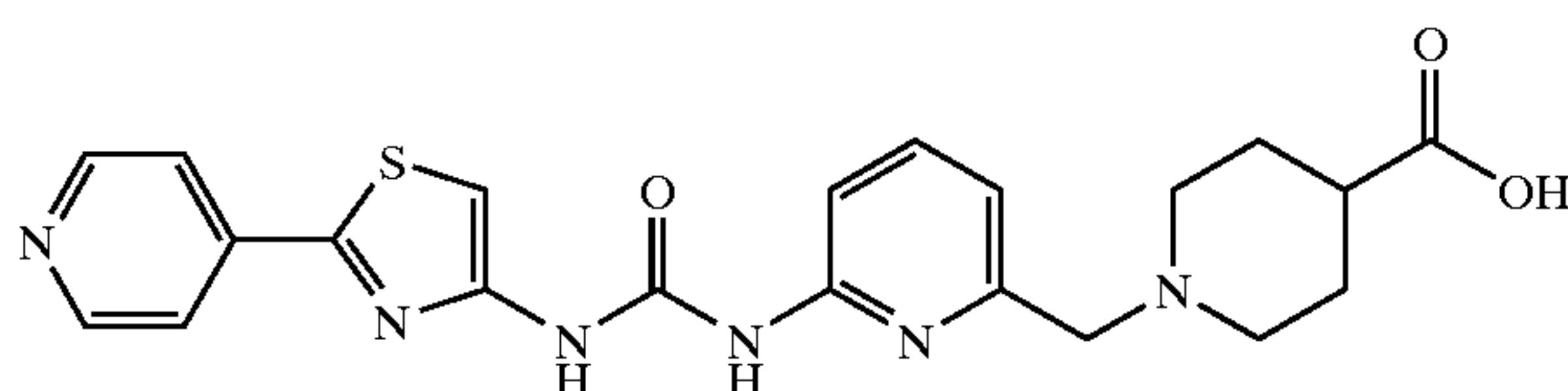
1-{6-[3-(2-(4-Pyridinyl)-4-thiazolyl)ureido]-pyridin-2-ylmethyl}-piperidine-4-carboxylic acid
