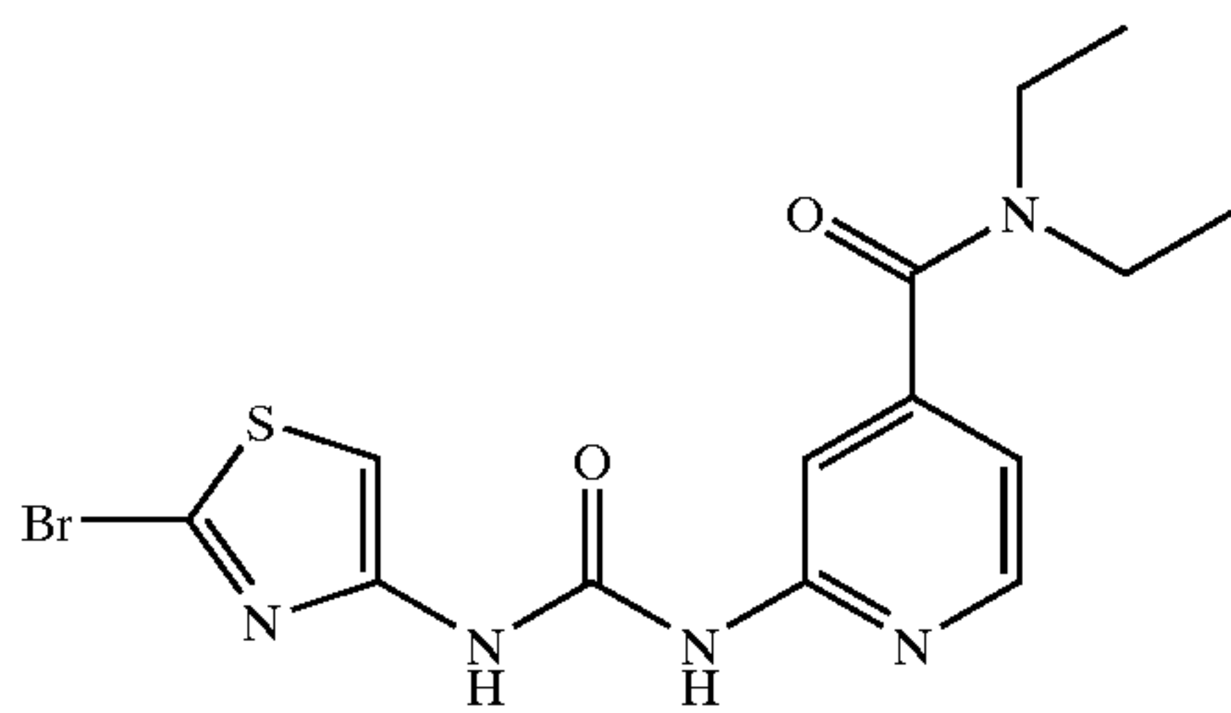
2-[3-(2-Bromo-thiazol-4-yl)-ureido]-N,N-diethyl-isonicotinamide
