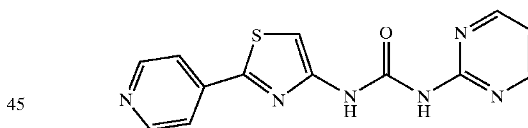
1-(2-Pyridin-4-yl-thiazol-4-yl)-3-pyrimidin-2-yl-urea
