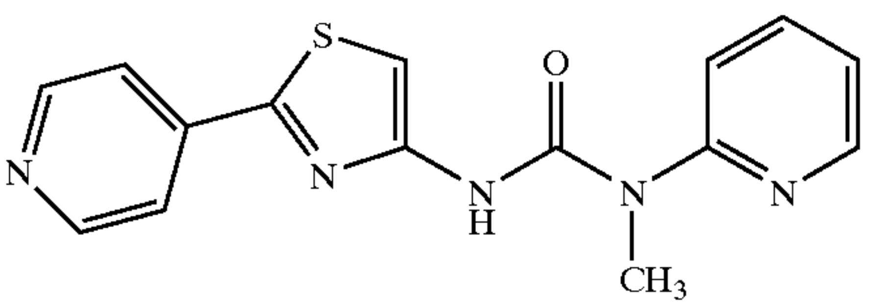
N-[2-(4-Pyridinyl)-4-thiazolyl]-N'-2-pyridinyl-N'-methylurea
