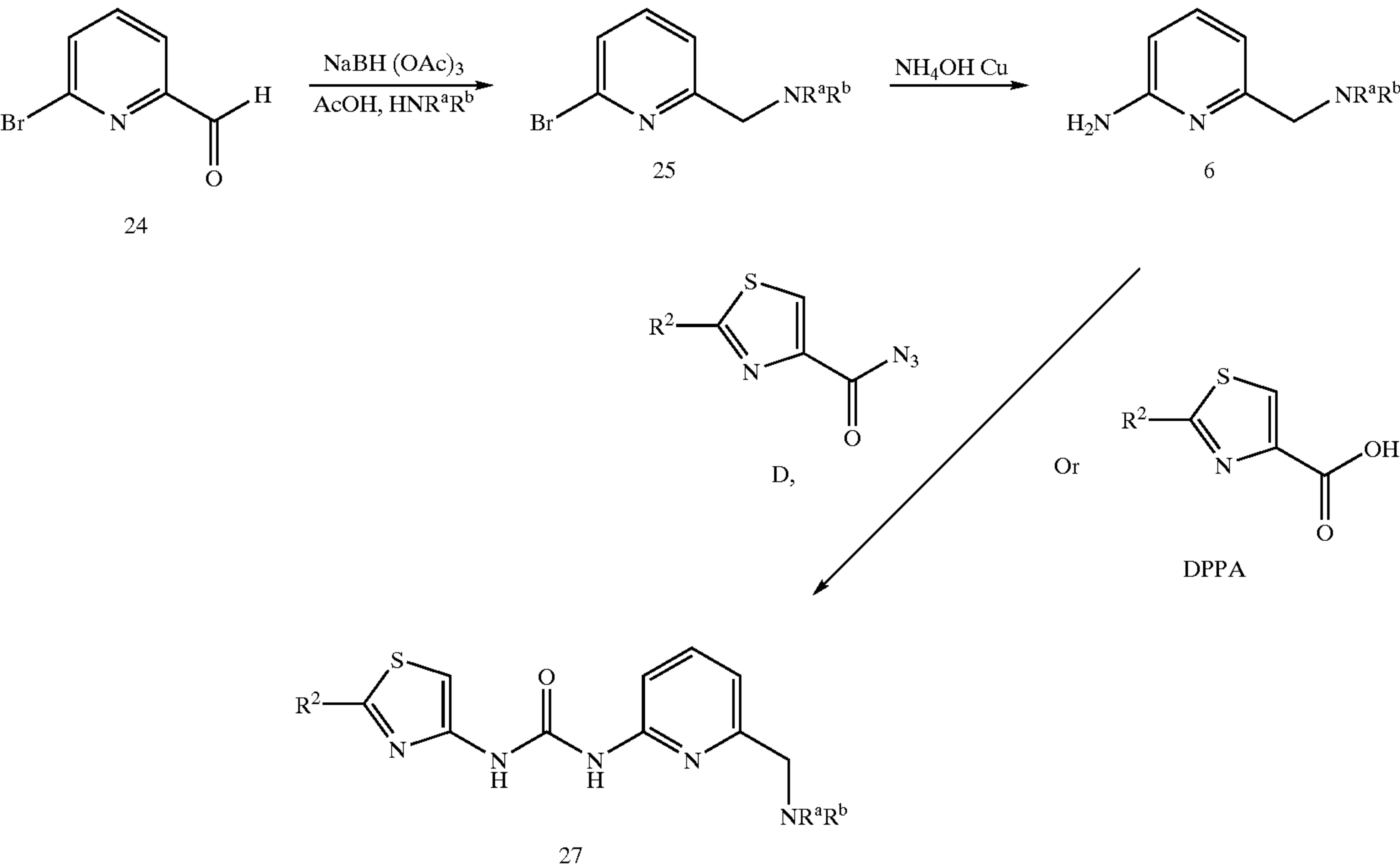
Scheme 5
