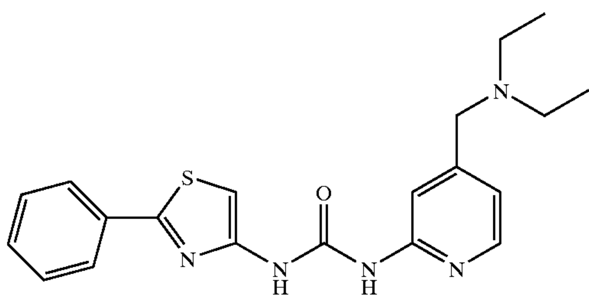
1-(4-Diethylaminomethyl-pyridin-2-yl)-3-(2-phenyl-thiazol-4-yl)-urea
