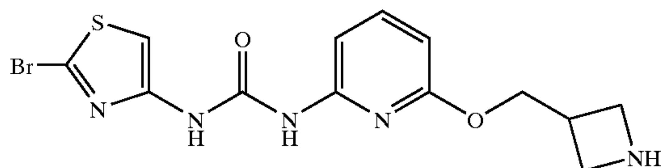
1-[6-(Azetidin-3-ylmethoxy)-pyridin-2-yl]-3-(2-bromo-thiazol-4-yl)-urea
