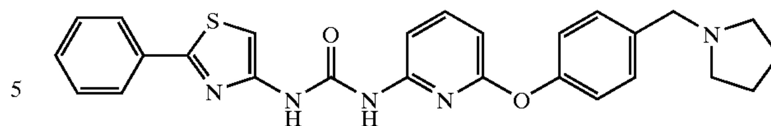
1-(2-phenylthiazol-4-yl)-3-(6-pyrrolidin-1-ylmethylphenoxy)pyridin-2-ylurea
