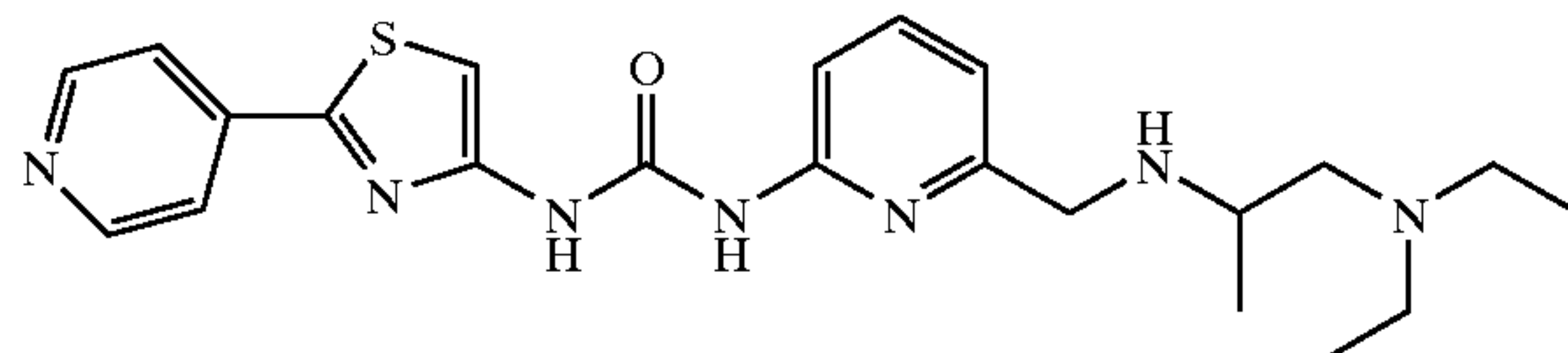
1-{6-[2-Diethylamino-1-methylethylamino)methyl]-pyridin-2-yl}-3-(2-pyridin-4-yl-thiazol-4-yl)urea
