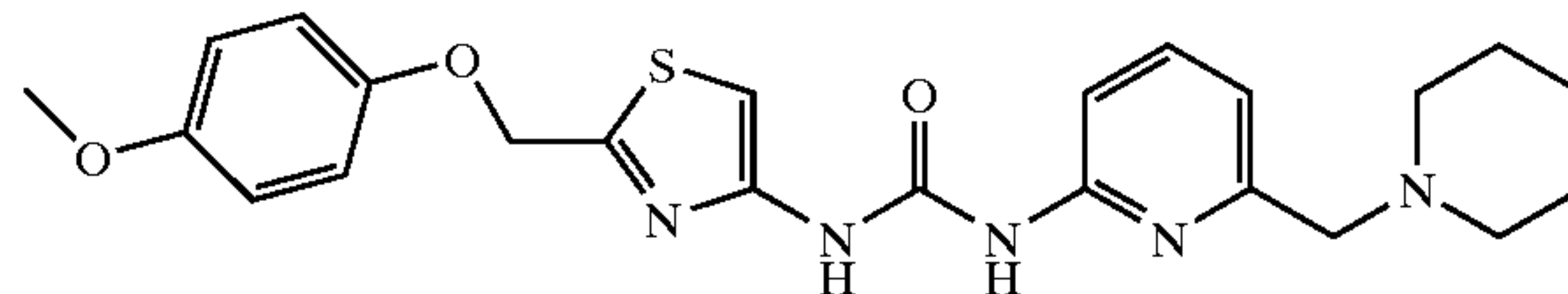
1-[2-(4-Methoxyphenoxy)methyl]thiazol-4-yl]-3-(6-piperidin-1-ylmethyl-pyridin-2-yl)urea
