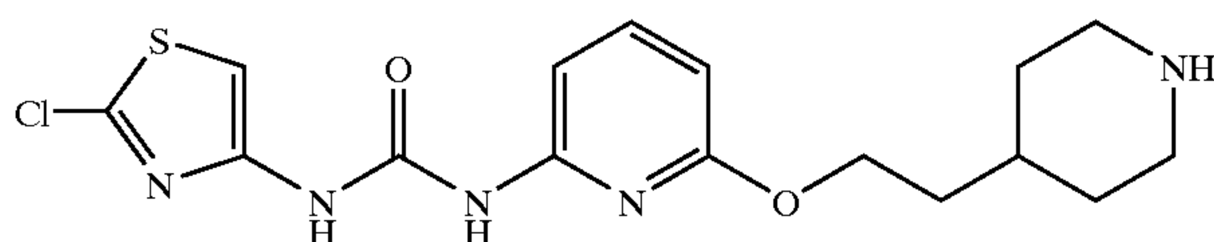
1-(2-Chloro-thiazol-4-yl)-3-[6-(2-piperidin-4-ylethoxy)-pyridin-2-yl]-urea
