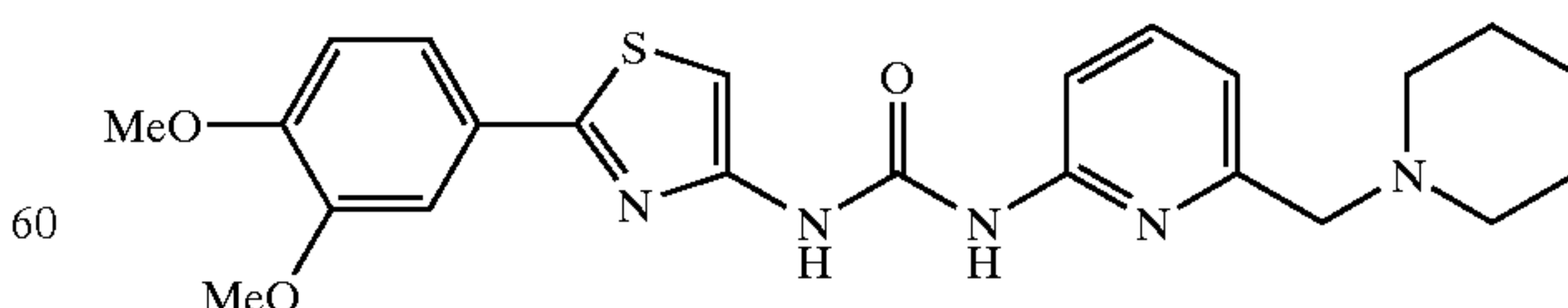
1-[2-(3,4-Dimethoxyphenyl)thiazol-4-yl]-3-(6-piperidin-1-ylmethylpyridin-2-yl)urea
