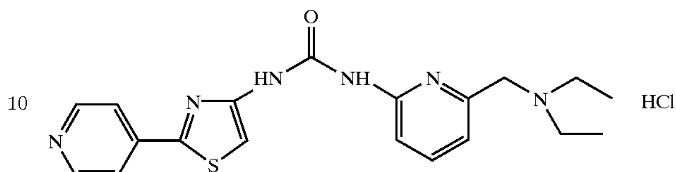
N-[2-(4-Pyridinyl)-4-thiazolyl]-N'-2-[6-(N,N-diethylaminomethylamino)pyridinyl]urea Hydrochloride
