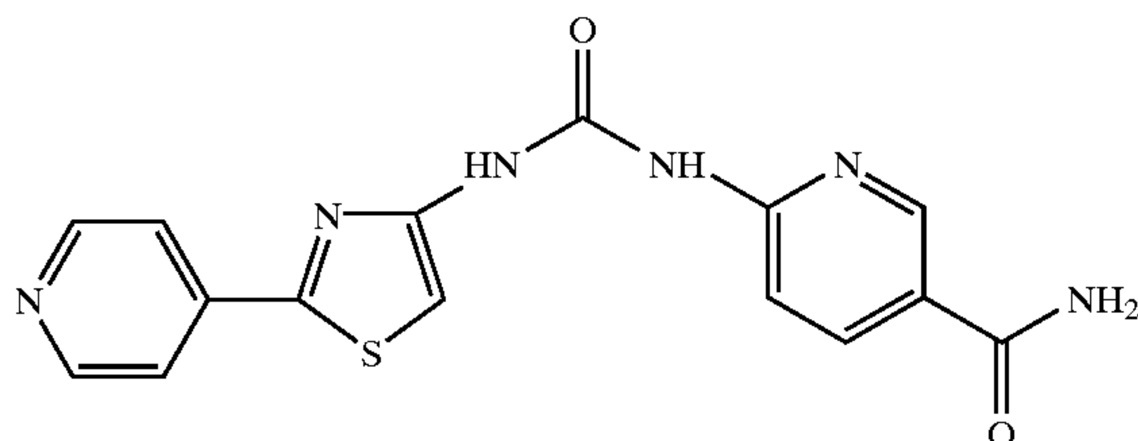
[[2-(4-Pyridinyl)-4-thiazolylamino]carbonyl]amino]-2-pyridinyl-5-carboxamide
