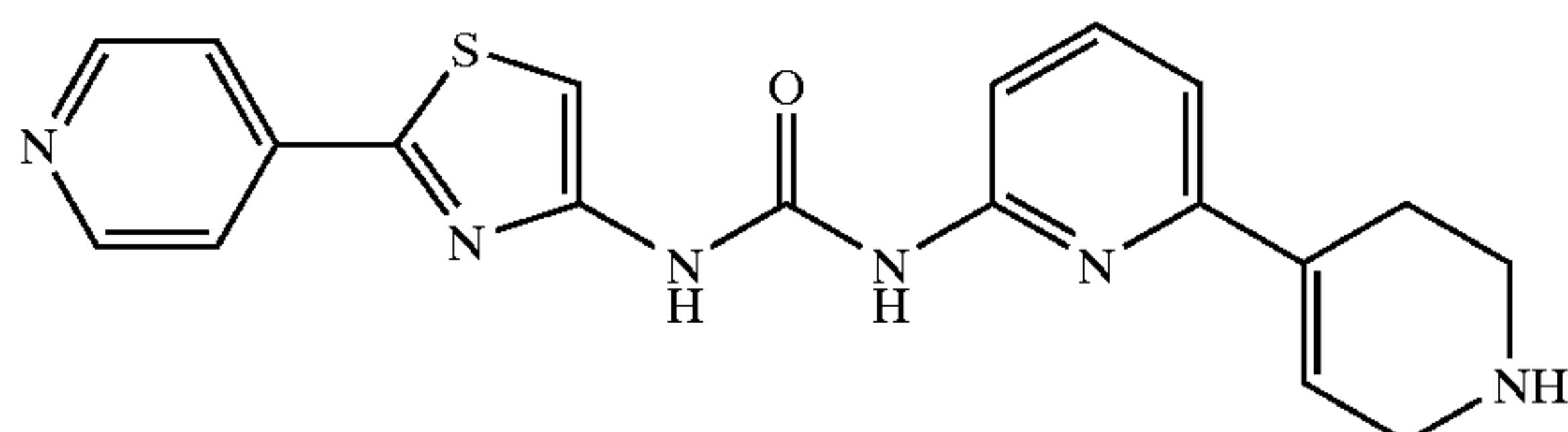
1-(2-Pyridin-4-yl-thiazol-4-yl)-3-(1',2',3',6'-tetrahydro-[2,4']bipyridinyl-6-yl)-urea
