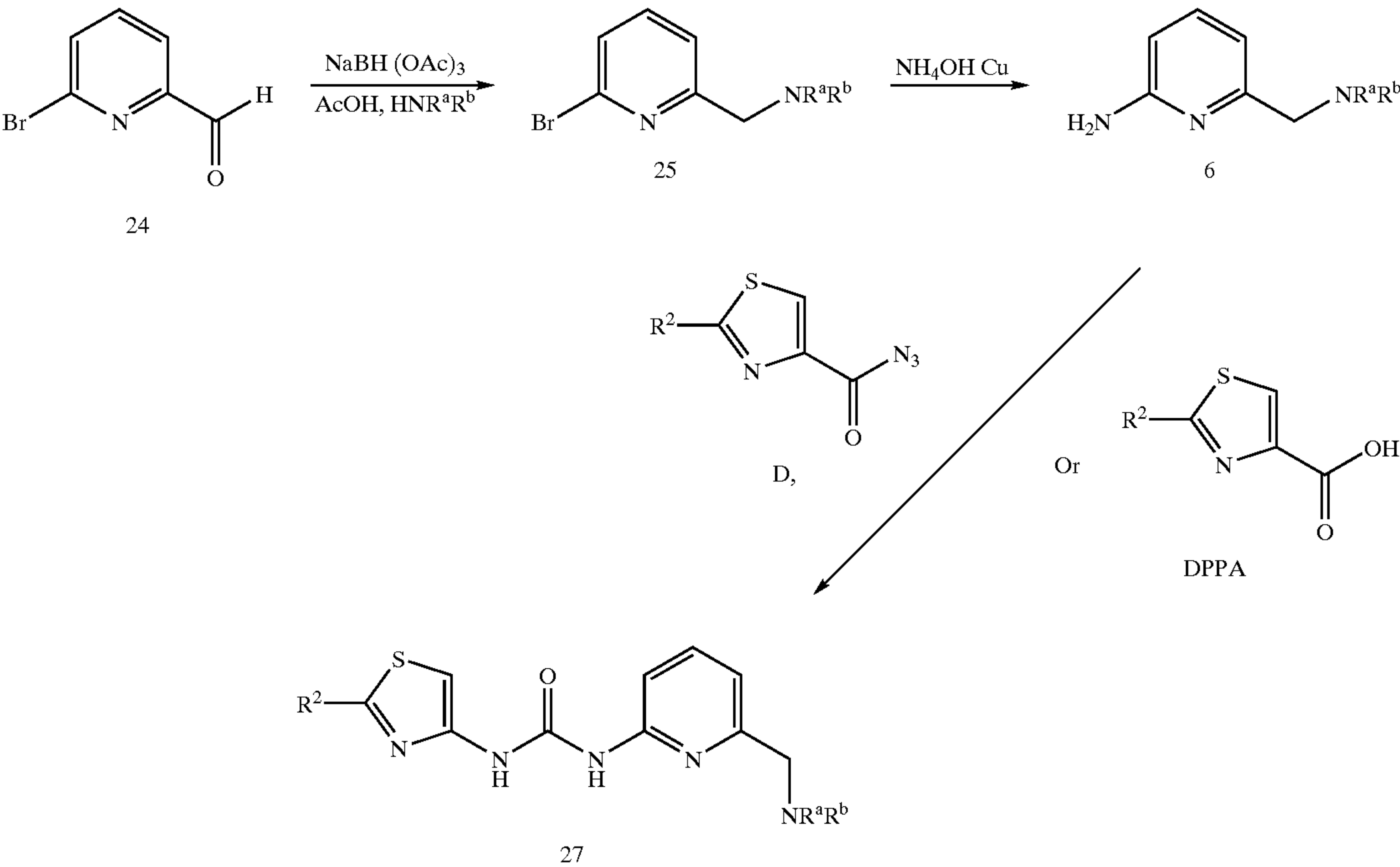
Scheme 5
