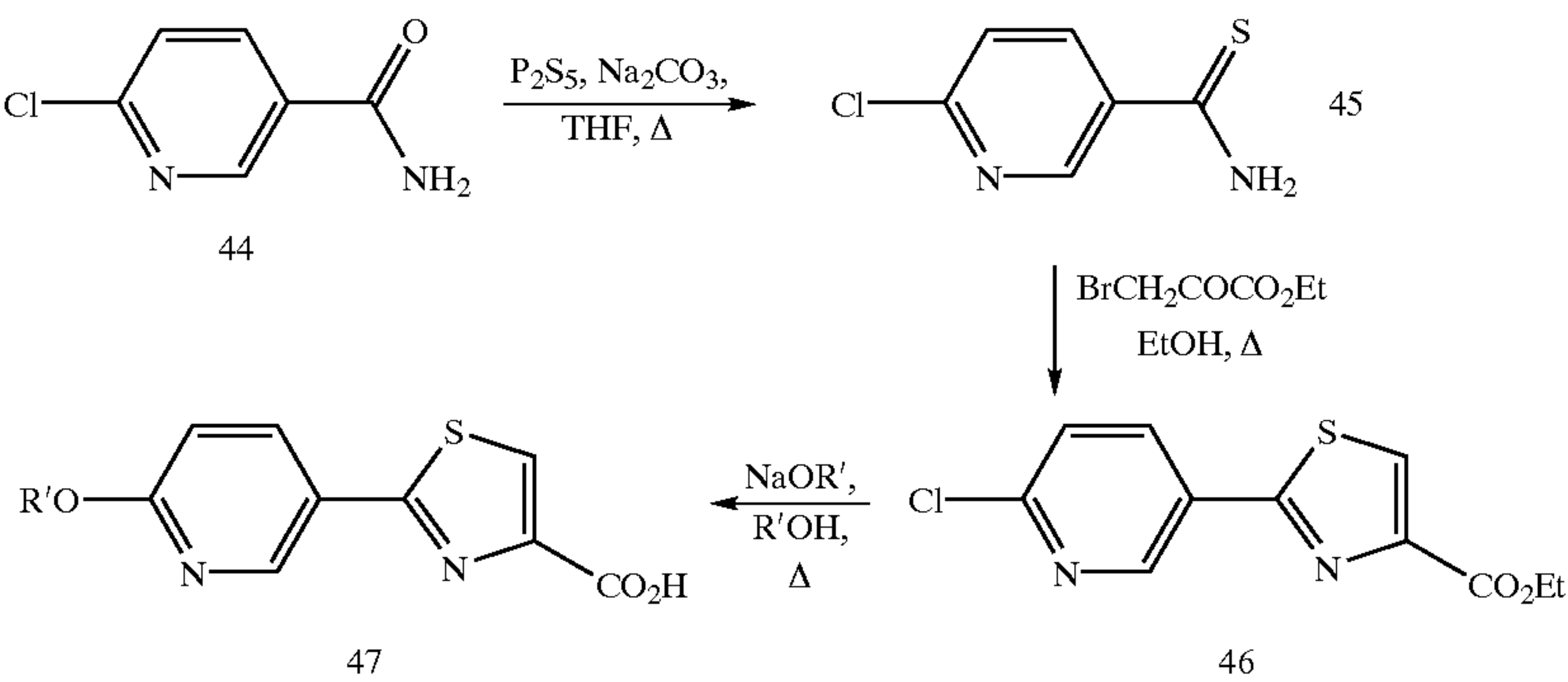
Scheme 13
