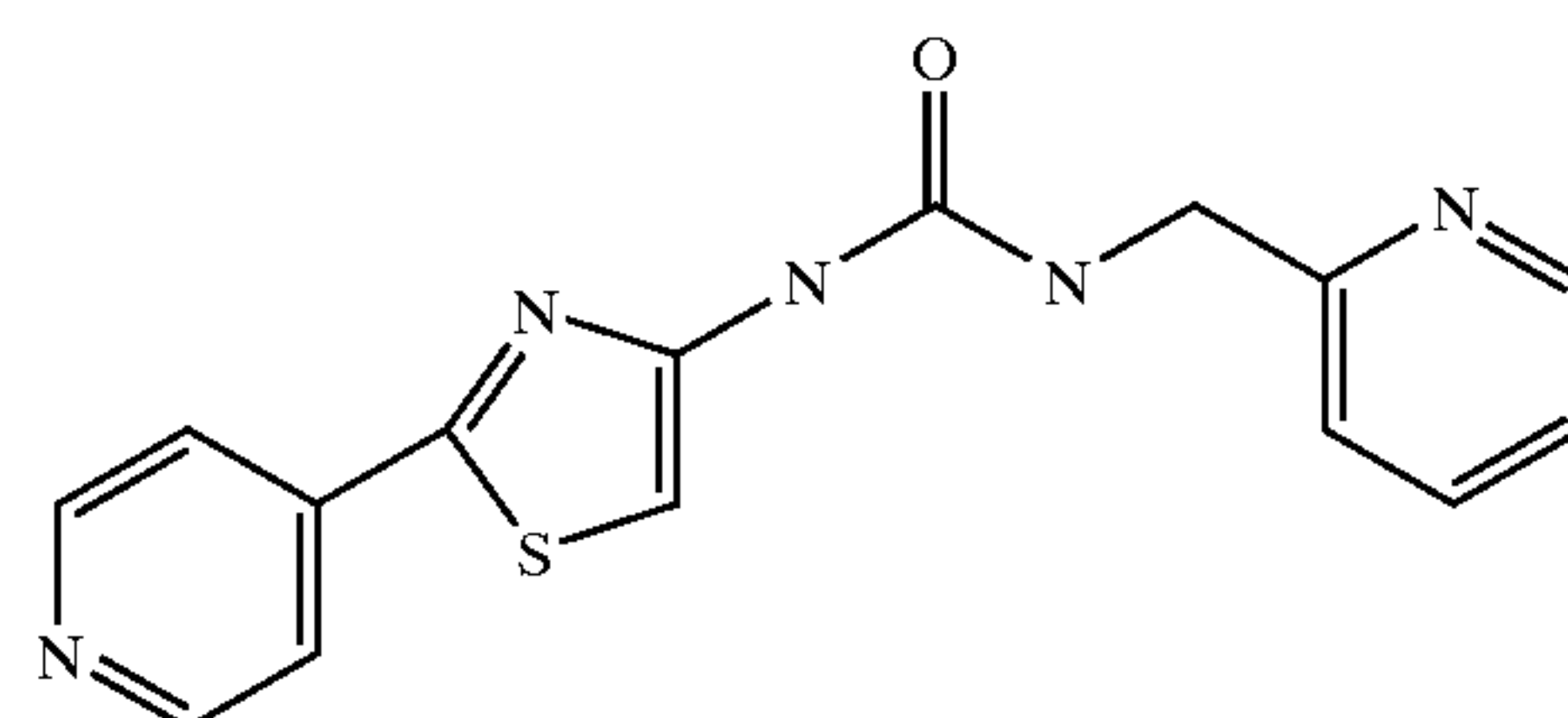
1-(Pyridin-2-ylmethyl)-3-(2-pyridin-4-yl-thiazol-4-yl)urea
