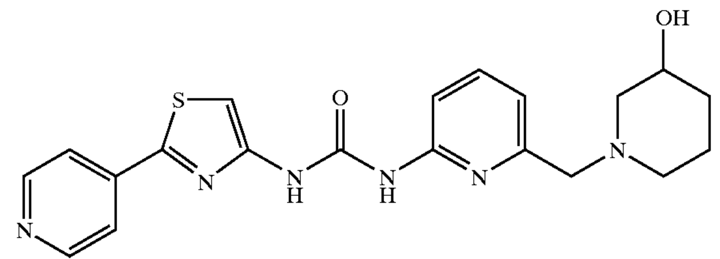
1-[6-(3-Hydroxy-piperidin-1-ylmethyl)-pyridin-2-yl]-3-(2-pyridin-4-yl-thiazol-4-yl)-urea
