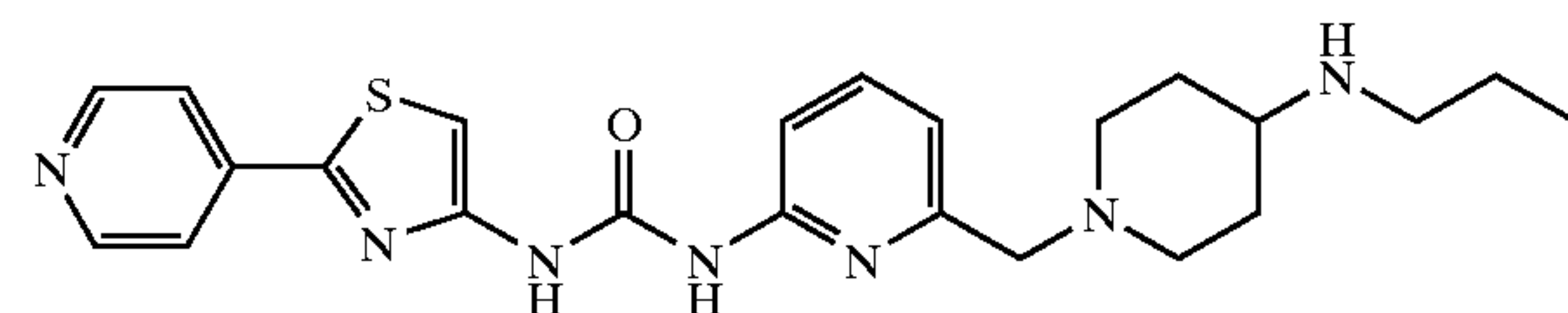
1-[6-[4-(Propylamino)piperidin-1-ylmethyl]pyridin-2-yl]-3-(2-pyridin-4-yl-thiazol-4-yl)urea
