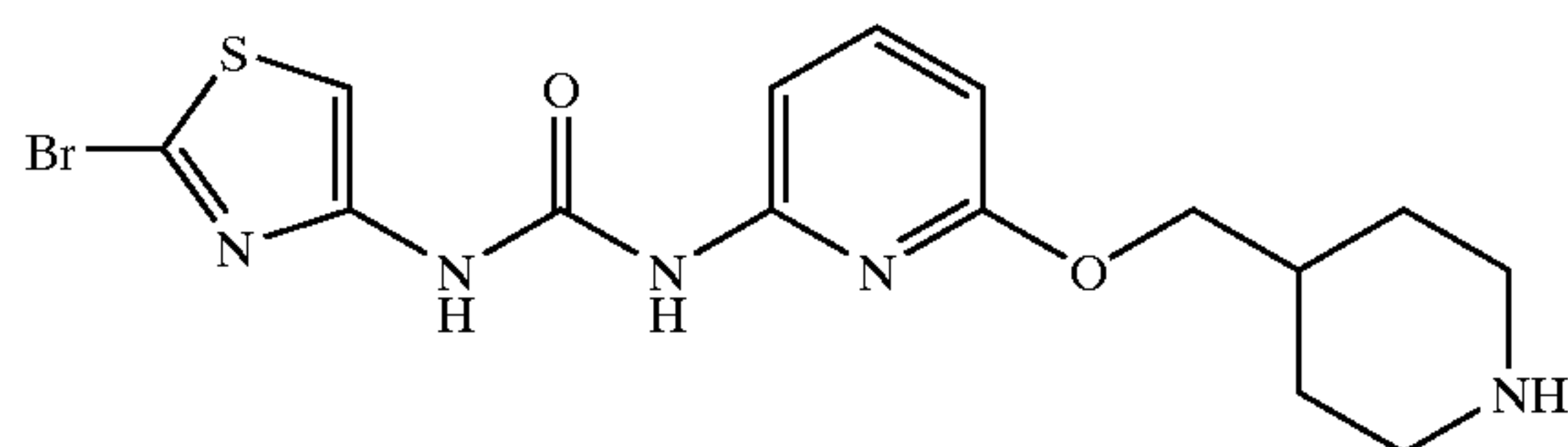
1-(2-Bromo-thiazol-4-yl)-3-[6-(piperidin-4-ylmethoxy)-pyridin-2-yl]-urea
