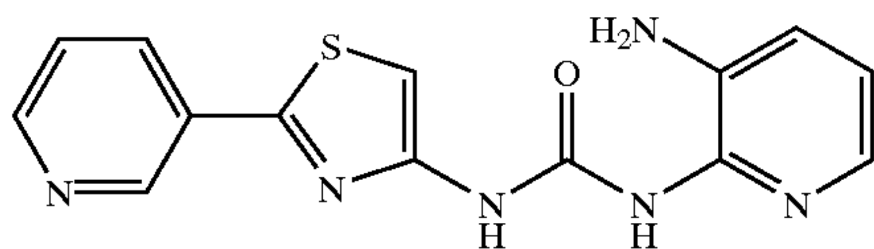
1-(3-Amino-pyridin-2-yl)-3-(2-pyridin-3-yl-thiazol-4-yl)-urea
