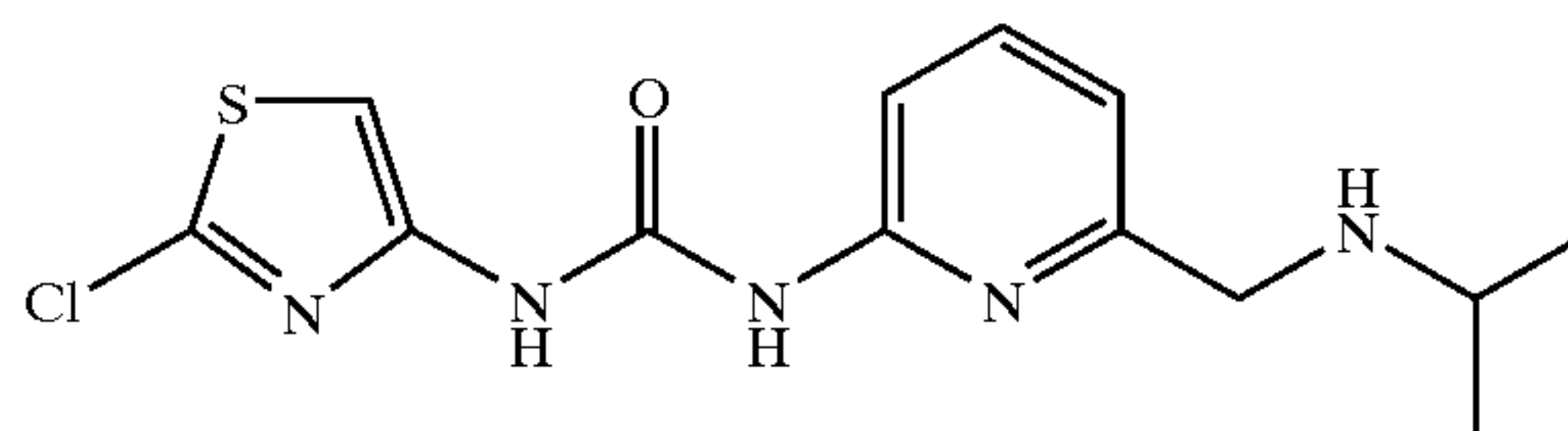
1-(2-Chloro-thiazol-4-yl)-3-[6-(isopropylamino-methyl)-pyridin-2-yl]-urea
