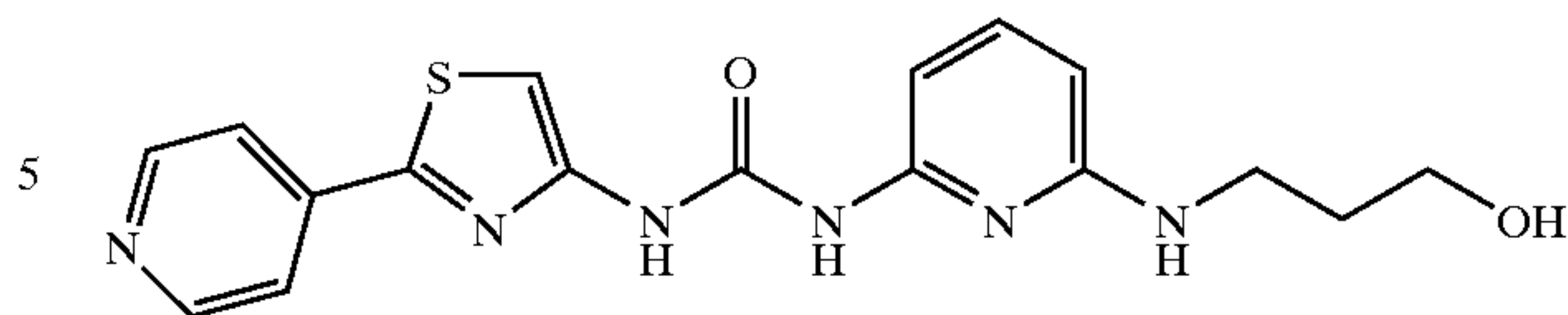
1-[6-(3-Hydroxy-propylamino)-pyridin-2-yl]-3-(2-pyridin-4-yl-thiazol-4-yl)-urea
