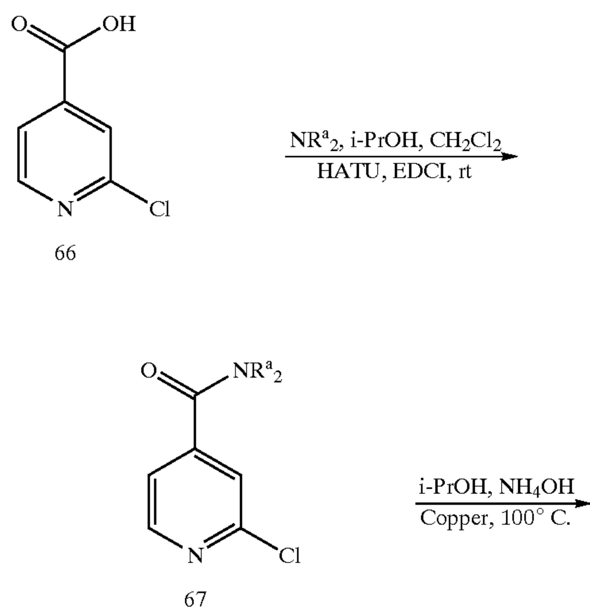
Scheme 18
