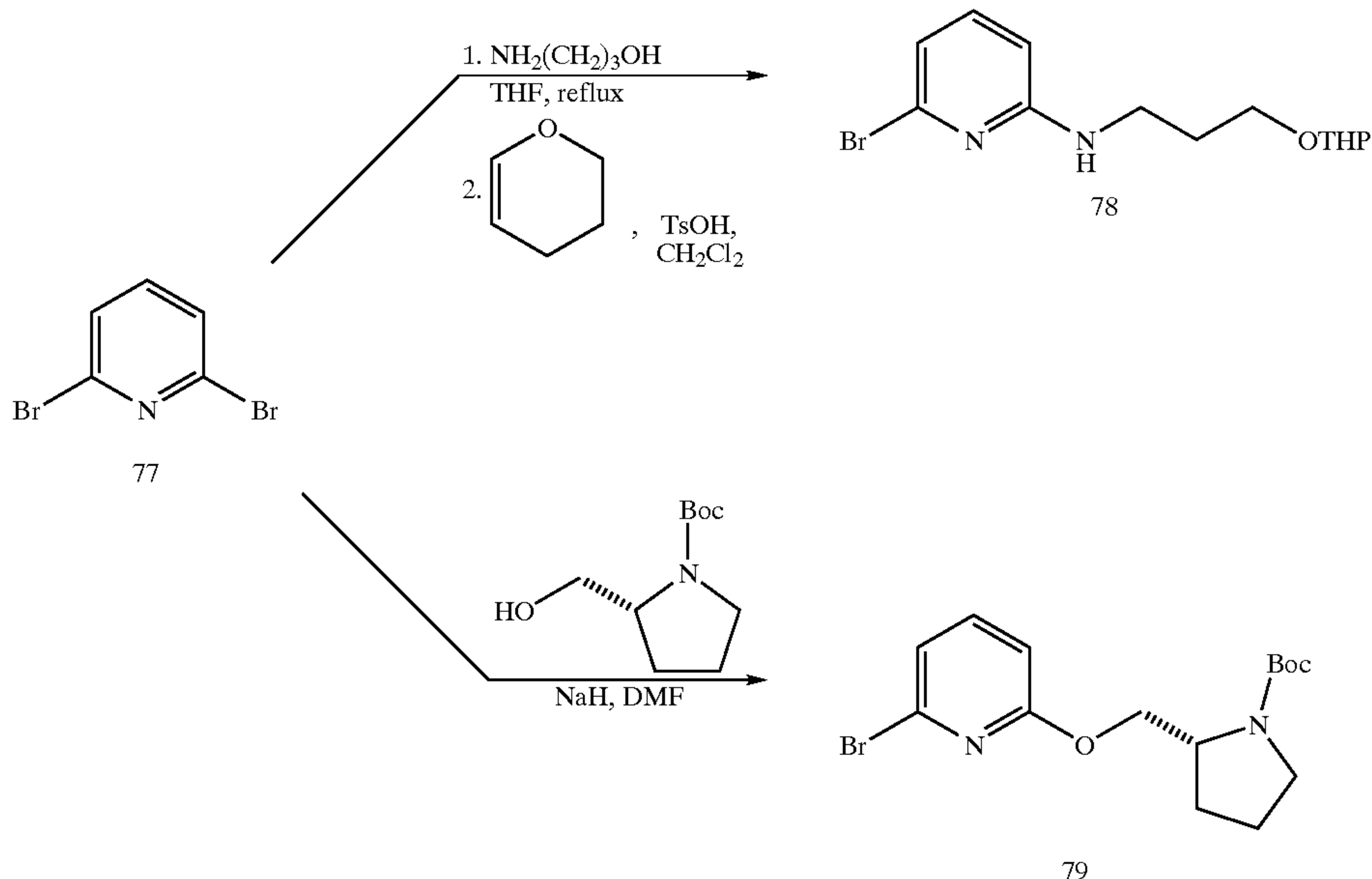
Scheme 21
