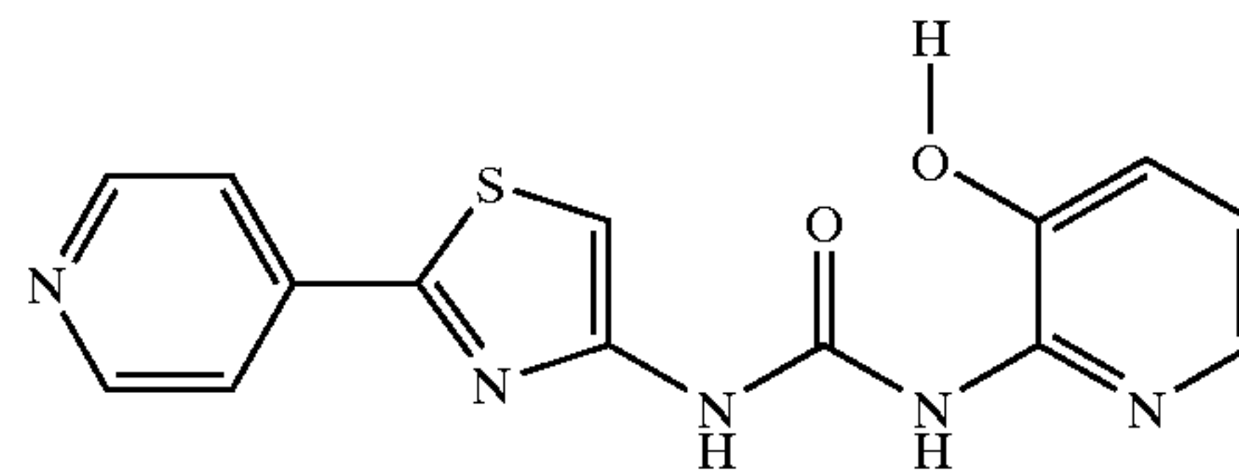
1-(3-Amino-pyridin-2-yl)-3-(2-pyridin-4-yl-thiazol-4-yl)-urea
