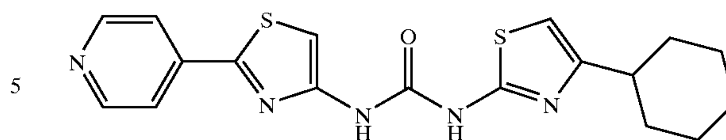
1-(4-Cyclohexylthiazol-2-yl)-3-[2-(pyridin-4-yl)-thiazol-4-yl]urea
