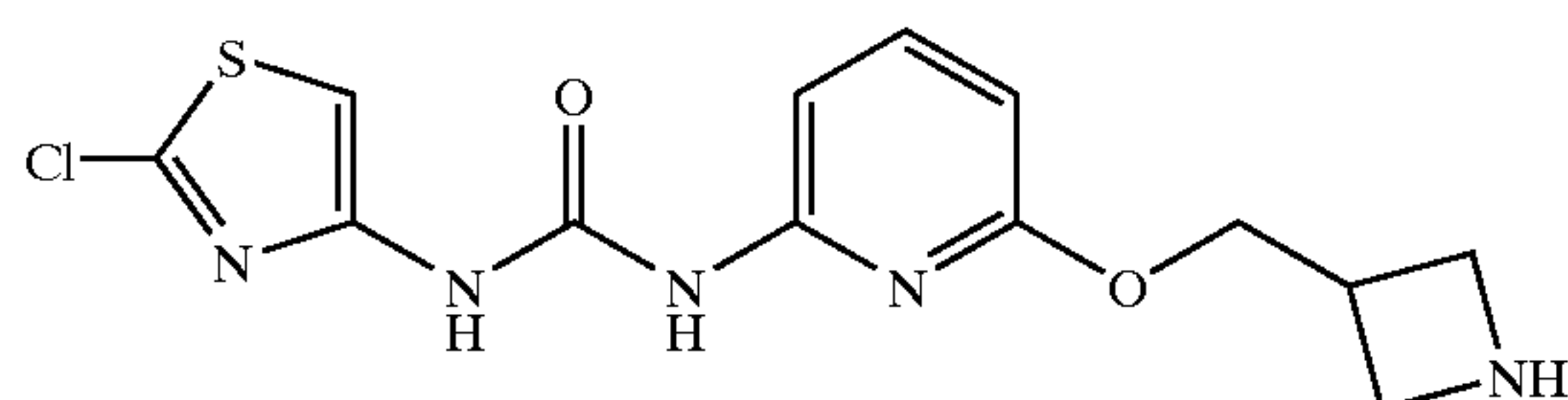
1-[6-(Azetidin-3-ylmethoxy)-pyridin-2-yl]-3-(2-chloro-thiazol-4-yl)-urea
