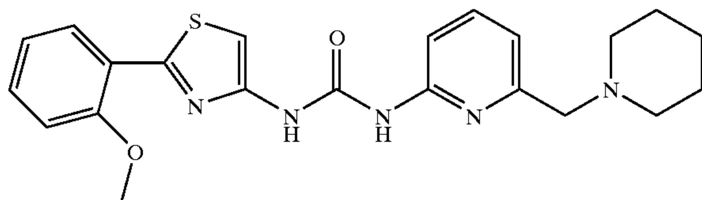
1-[2-(2-Methoxyphenyl)thiazol-4-yl]-3-(6-piperidin-1-ylmethyl-pyridin-2-yl)urea
