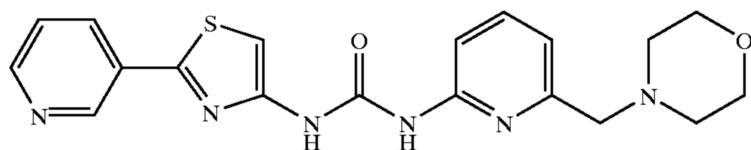
1-[6-(Morpholin-4-ylmethyl)-pyridin-2-yl]-3-[(2-pyridin-3-yl)thiazol-4-yl]urea
