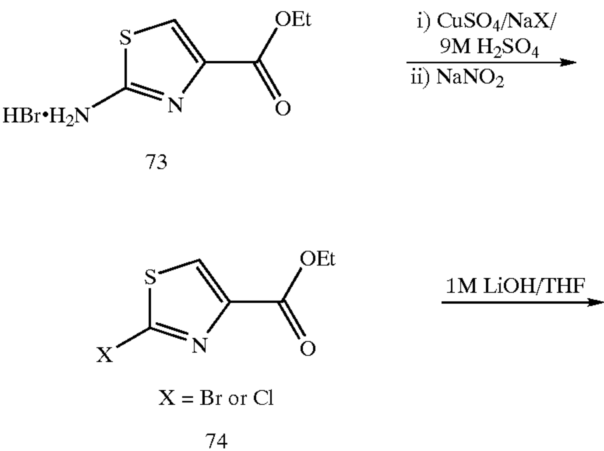
Scheme 20
