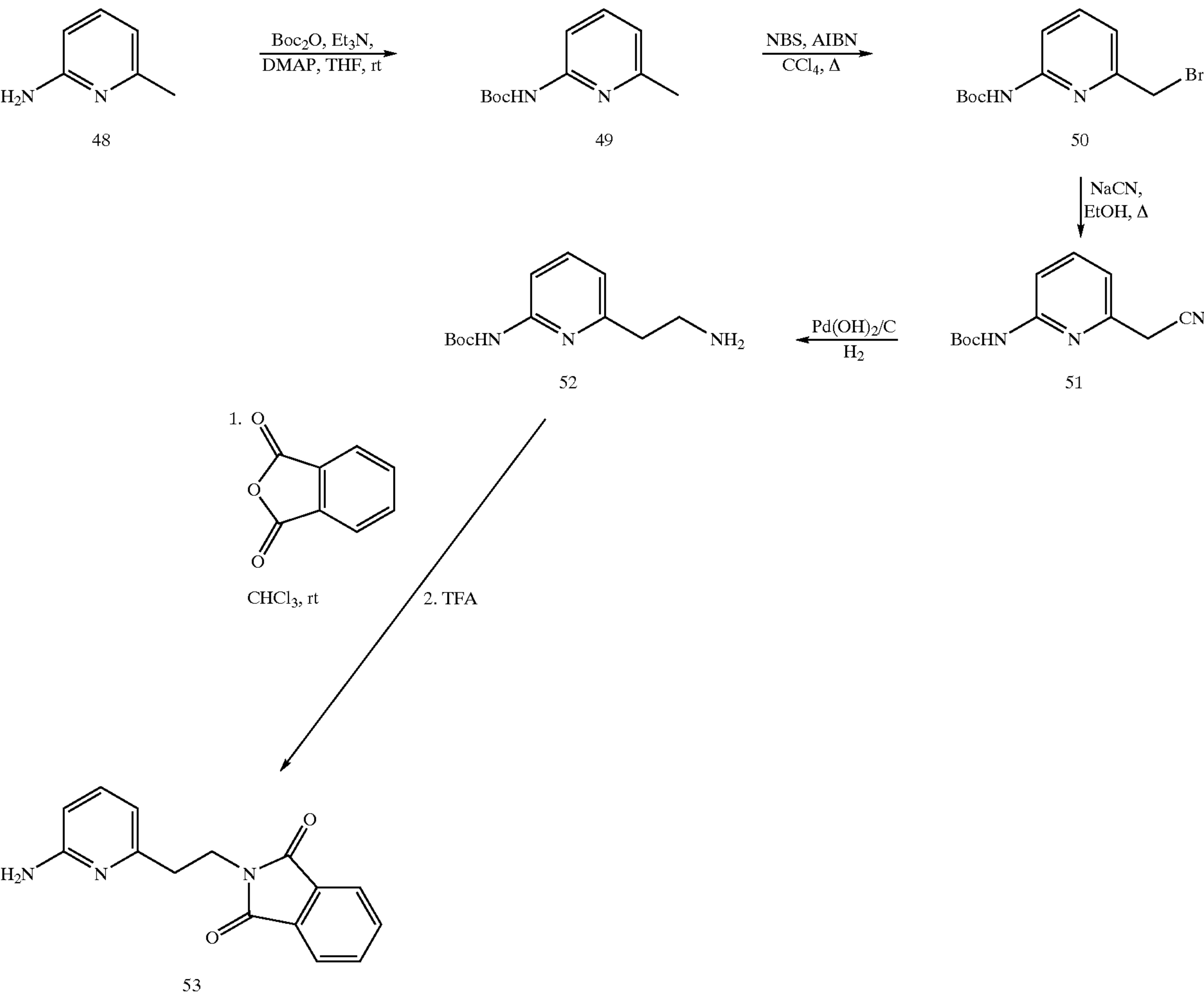
Scheme 14
