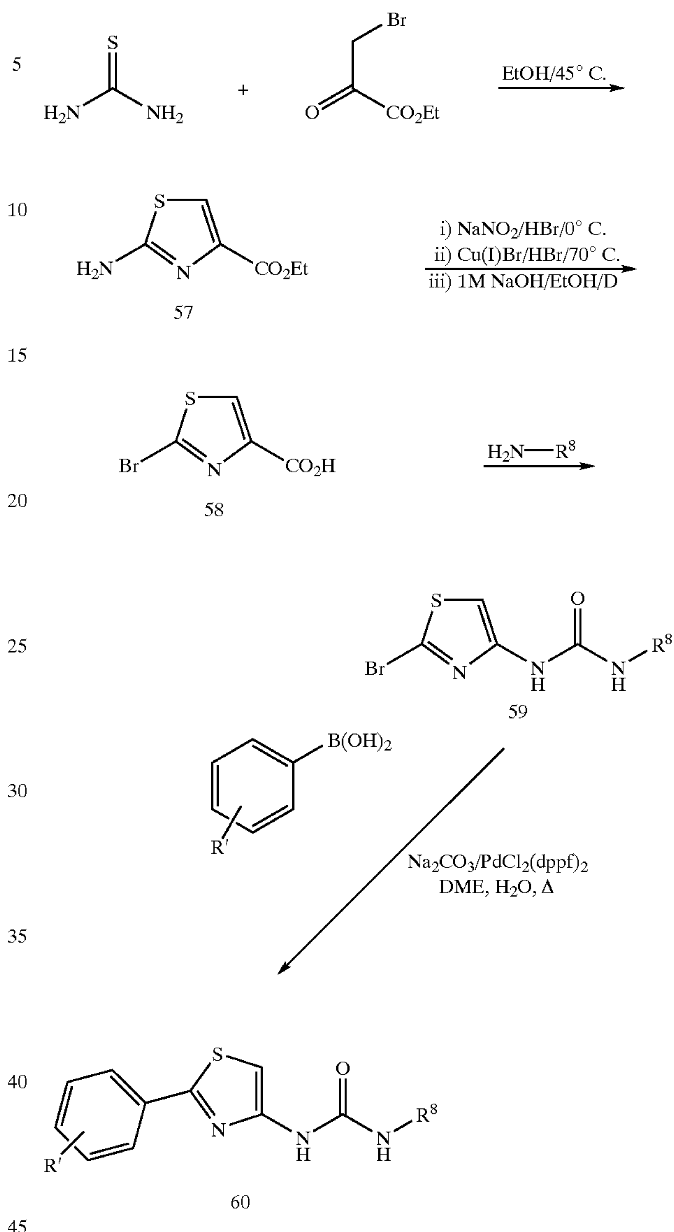
Scheme 16
