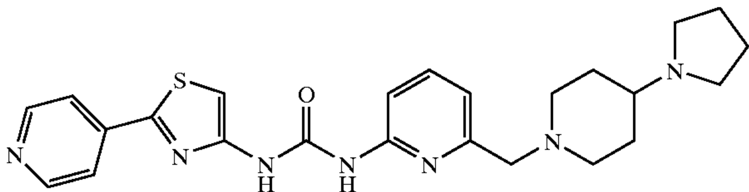
1-(2-Pyridin-4-yl-thiazol-4-yl)-3-[6-(4-pyrrolidin-1-yl-piperidin-1-ylmethyl)-pyridin-2-yl]-urea
