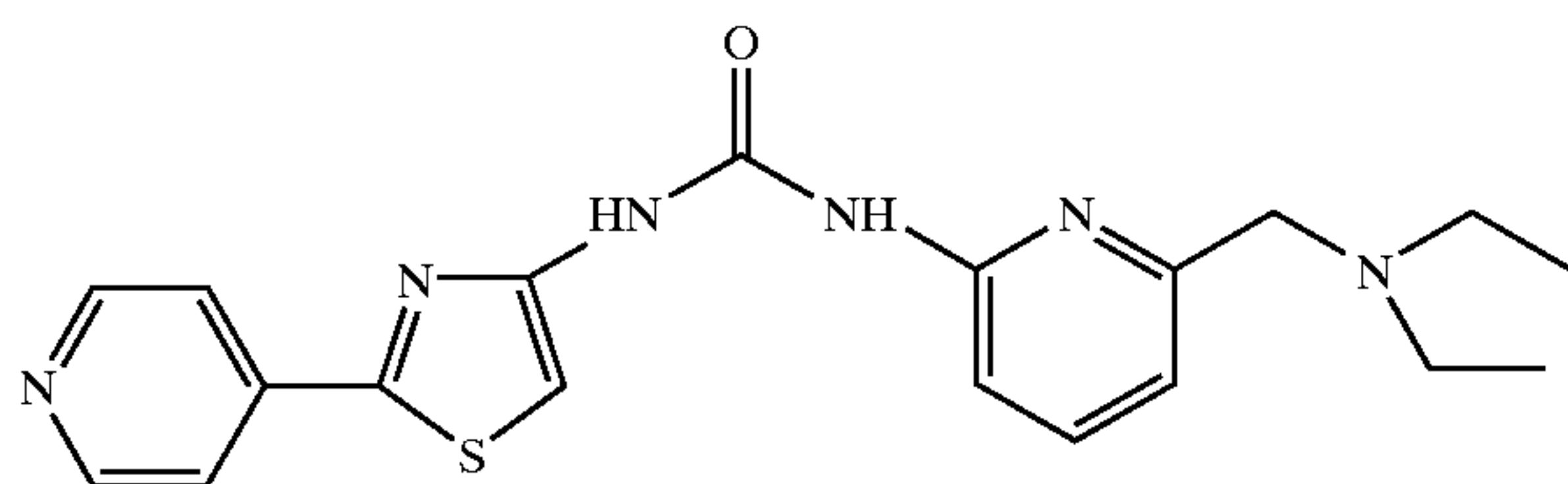
N-[2-(4-Pyridinyl)-4-thiazolyl]-N'-2-[6-(N,N-diethylaminomethylamino)pyridinyl]urea
