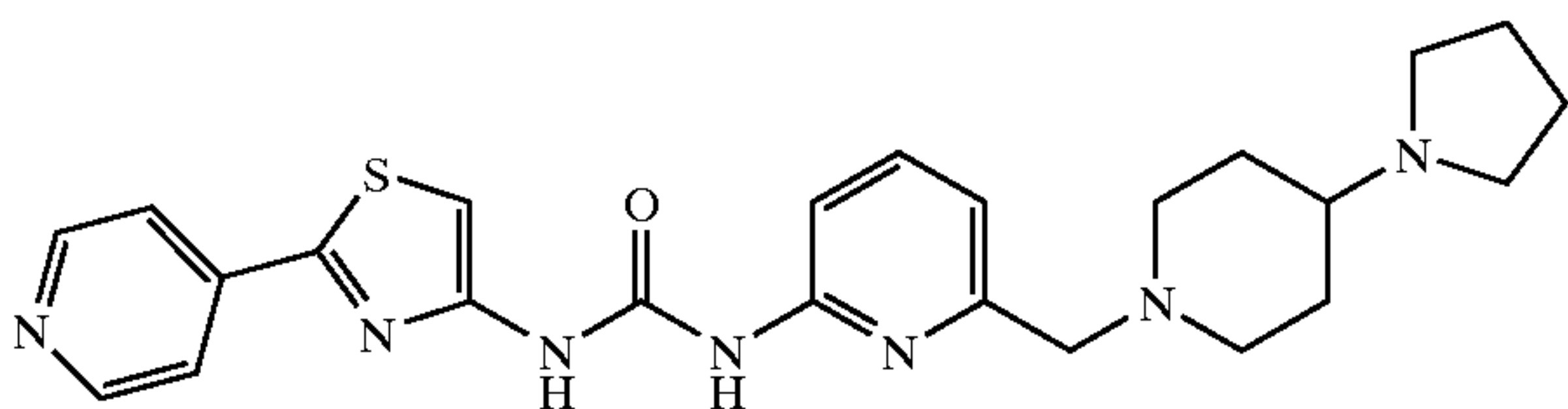
1-(2-Pyridin-4-yl-thiazol-4-yl)-3-[6-(4-pyrrolidin-1-yl-piperidin-1-ylmethyl)-pyridin-2-yl]-urea
