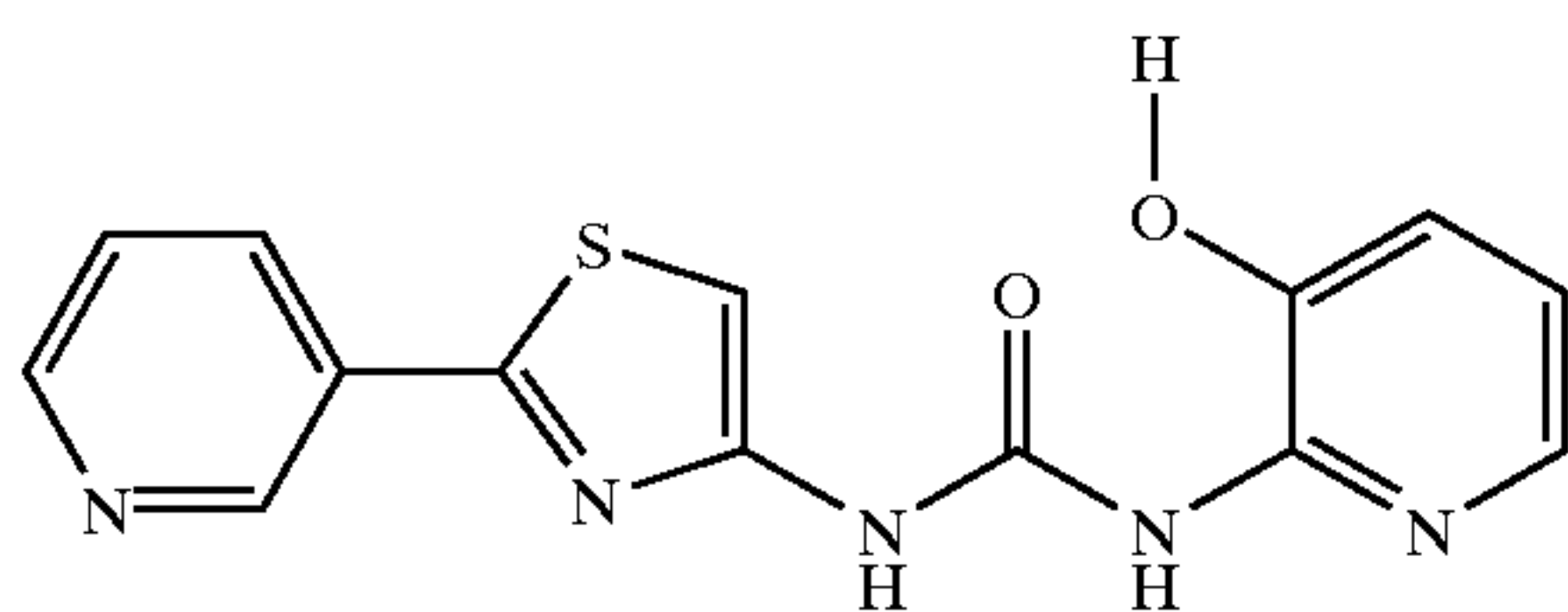
1-(3-Hydroxy-pyridin-2-yl)-3-(2-pyridin-3-yl-thiazol-4-yl)-urea
