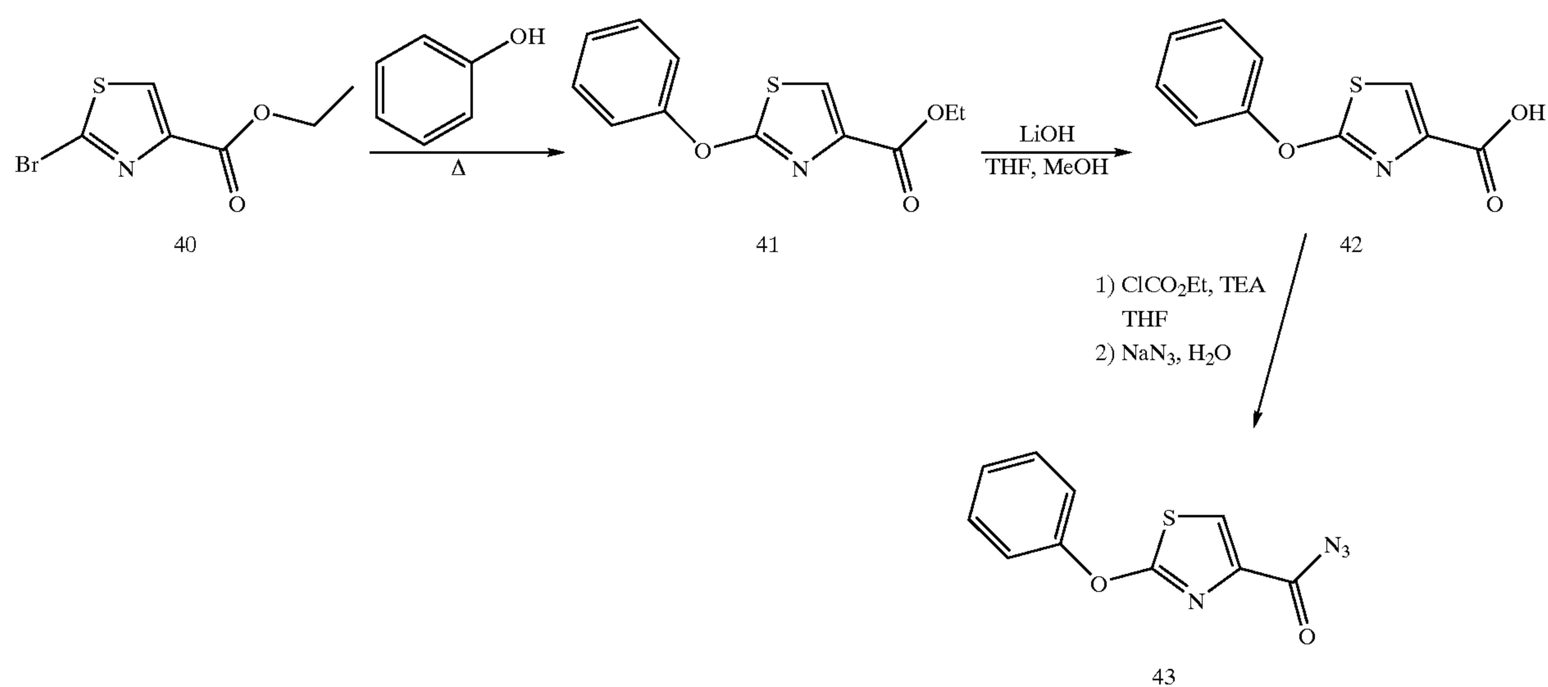
Scheme 12
