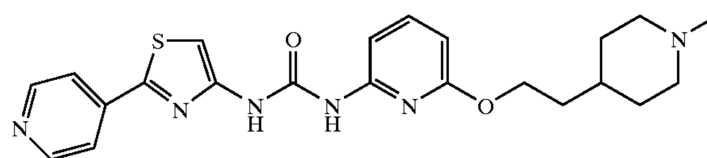
1-{6-[2-(1-Methylpiperidin-4-yl)ethoxy]pyridin-2-yl}-3-(2-pyridin-4-yl-thiazol-4-yl)urea
