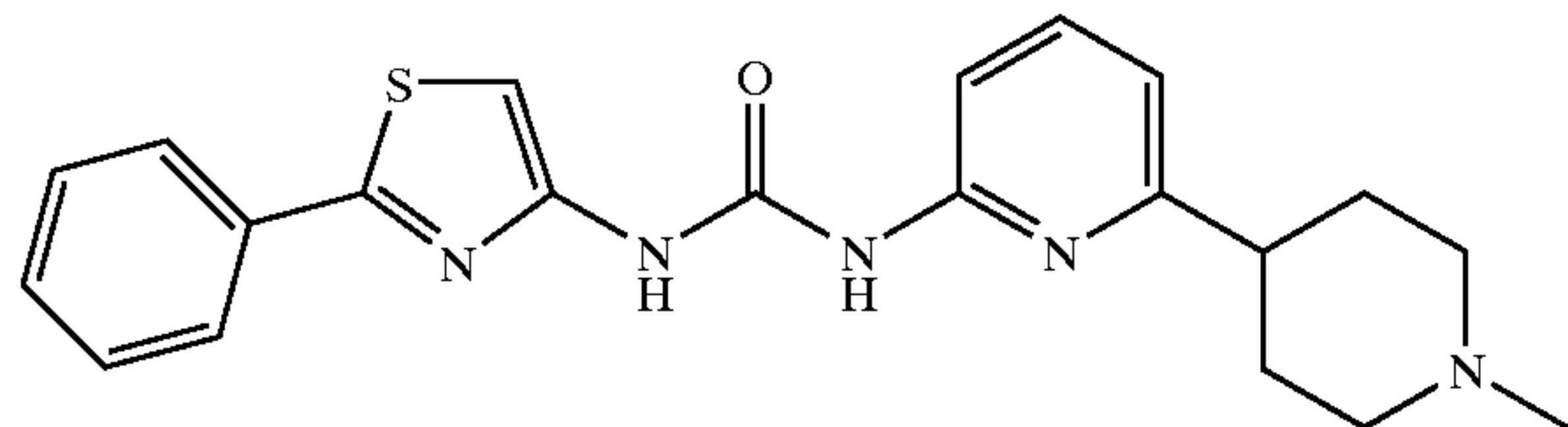
1-(1'-Methyl-1',2',3',4',5',6'-hexahydro-[2,4']bipyridinyl-6-yl)-3-(2-phenyl-thiazol-4-yl)-urea
