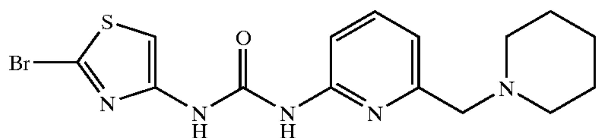
1-(2-Bromothiazol-4-yl)-3-(6-piperidin-1-ylmethylpyridin-2-yl)urea
