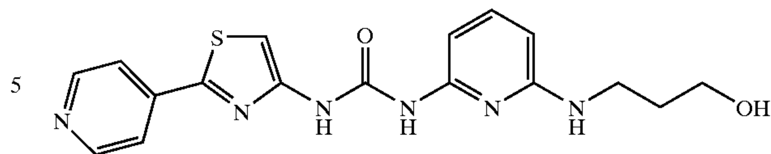
1-[6-(3-Hydroxy-propylamino)-pyridin-2-yl]-3-(2-pyridin-4-yl-thiazol-4-yl)-urea
