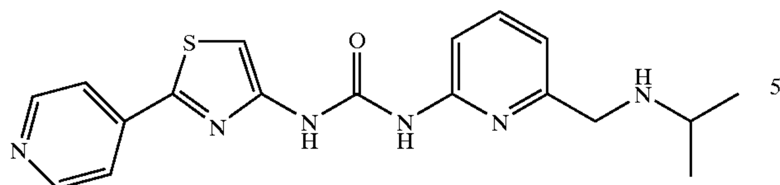
1-[6-(Isopropylamino-methyl)-pyridin-2-yl]-3-(2-pyridin-4-yl-thiazol-4-yl)-urea
