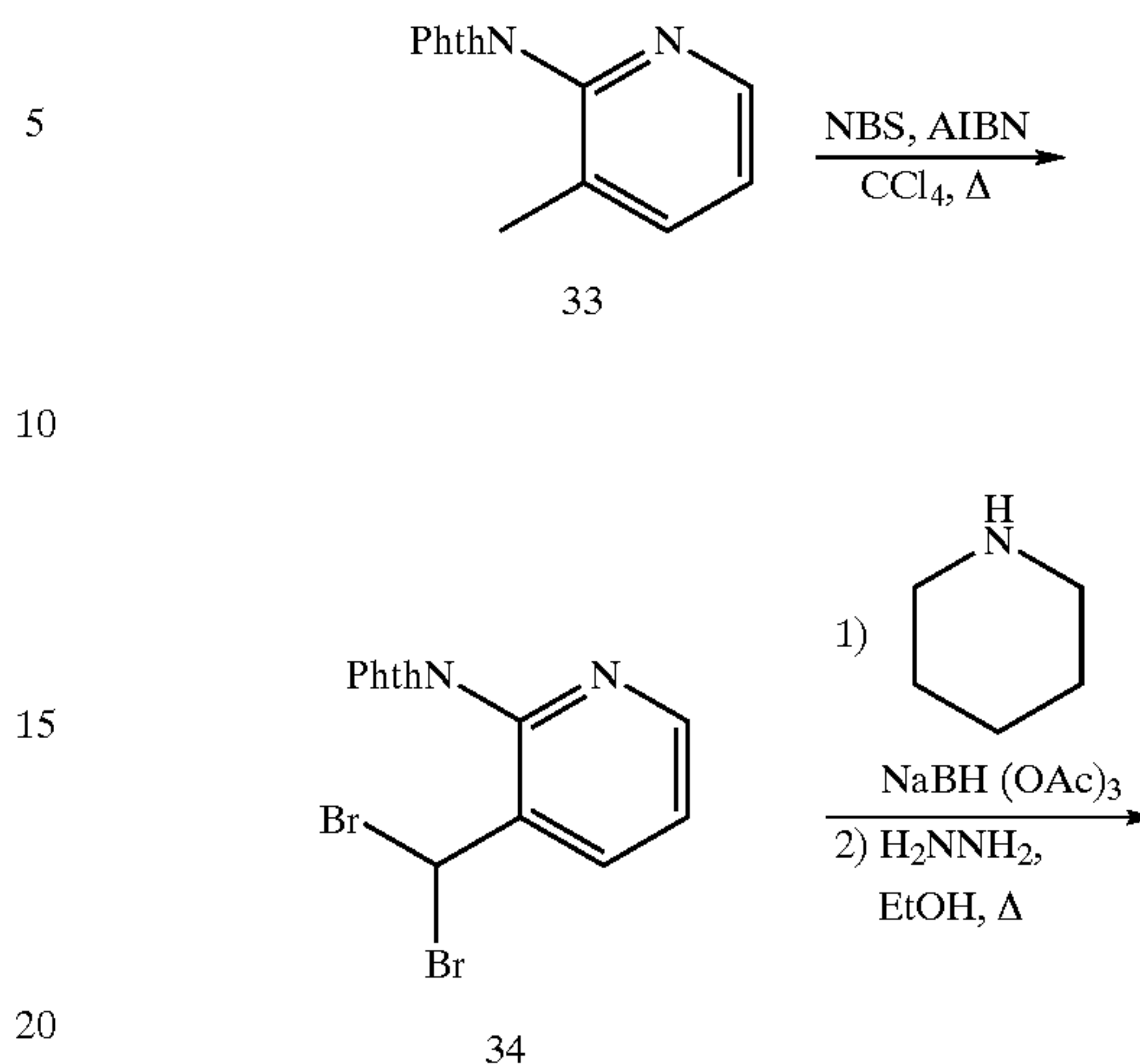
Scheme 9
