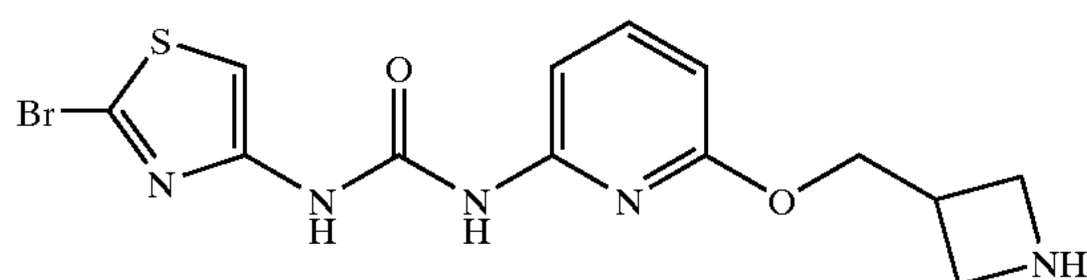
1-[6-(Azetidin-3-ylmethoxy)-pyridin-2-yl]-3-(2-bromo-thiazol-4-yl)-urea
