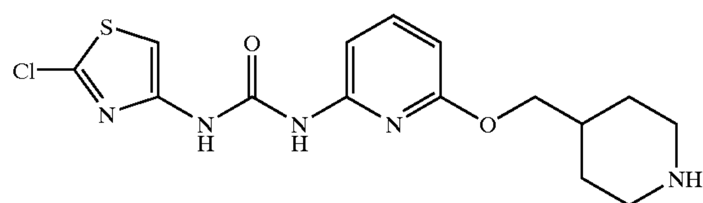
1-(2-Chloro-thiazol-4-yl)-3-[6-(piperidin-4-ylmethoxy)-pyridin-2-yl]-urea
