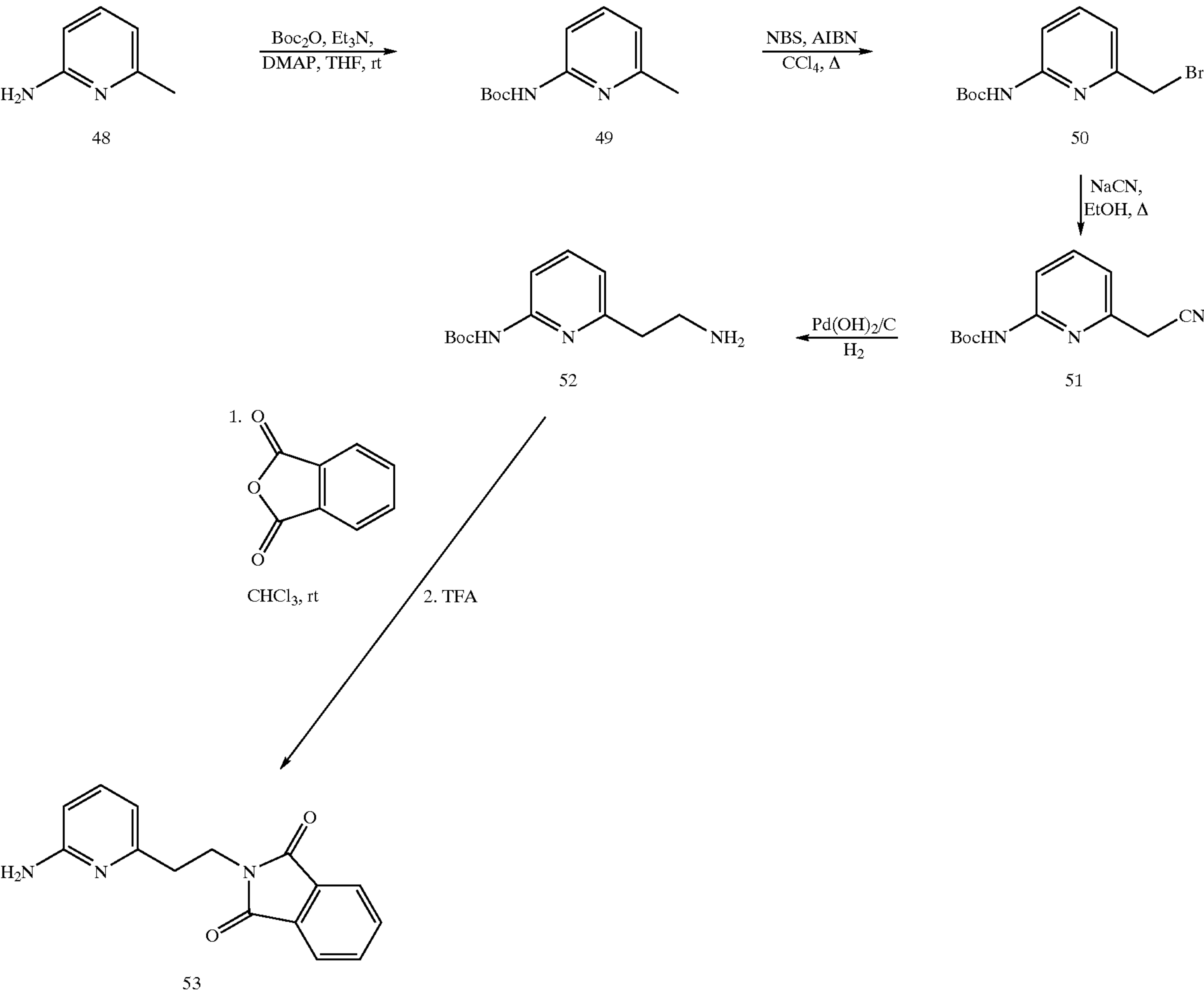
Scheme 14
