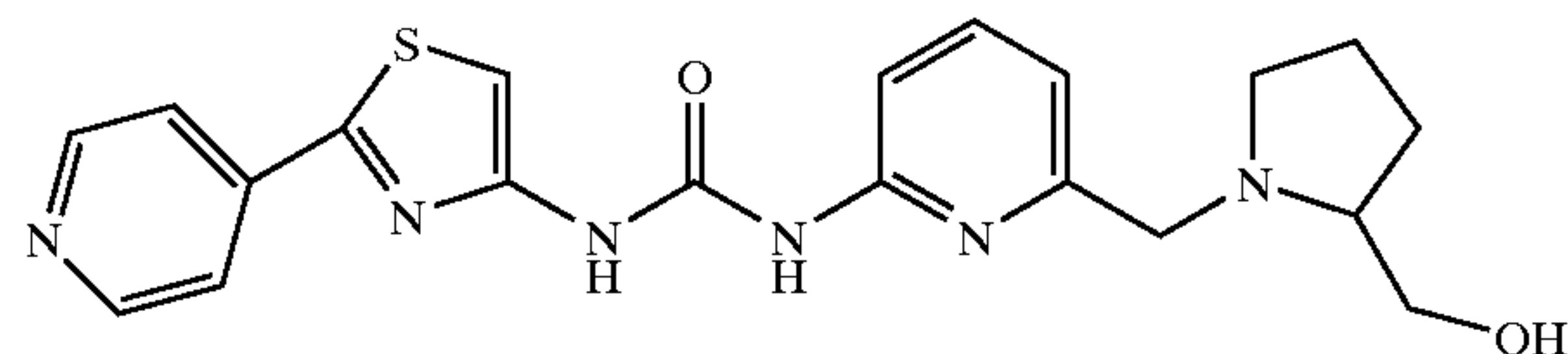
1-[6-(2-Hydroxymethylpyrrolidin-1-ylmethyl)-pyridin-2-yl]-3-(2-pyridin-4-yl-thiazol-4-yl)urea
