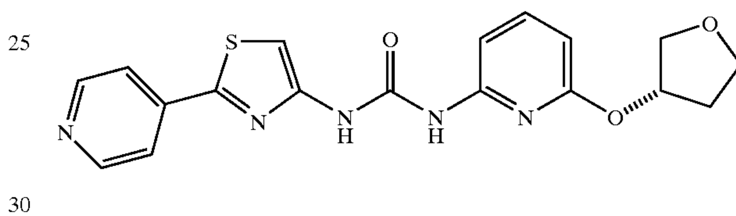
1-(2-Pyridin-4-yl-thiazol-4-yl)-3-[6-(tetrahydro-furan-3-yloxy)-pyridin-2-yl]-urea
