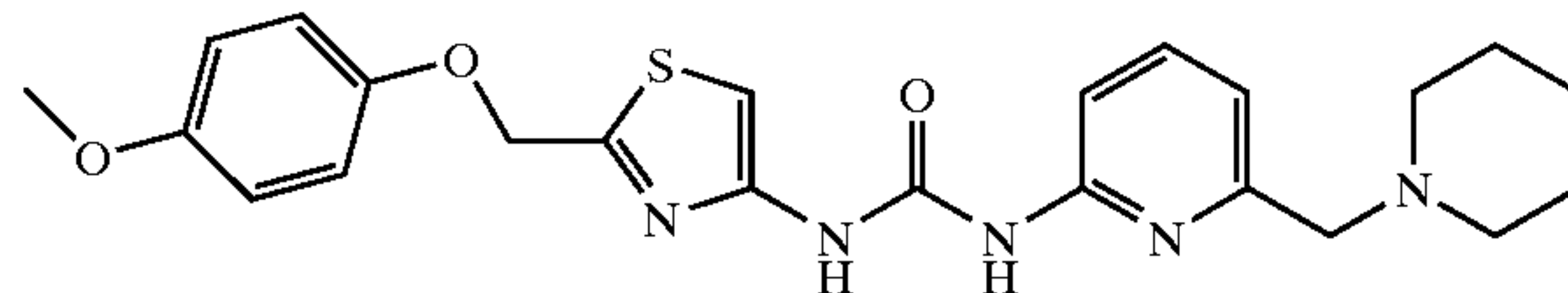
1-[2-(4-Methoxyphenoxy)methyl]thiazol-4-yl]-3-(6-piperidin-1-ylmethyl-pyridin-2-yl)urea
