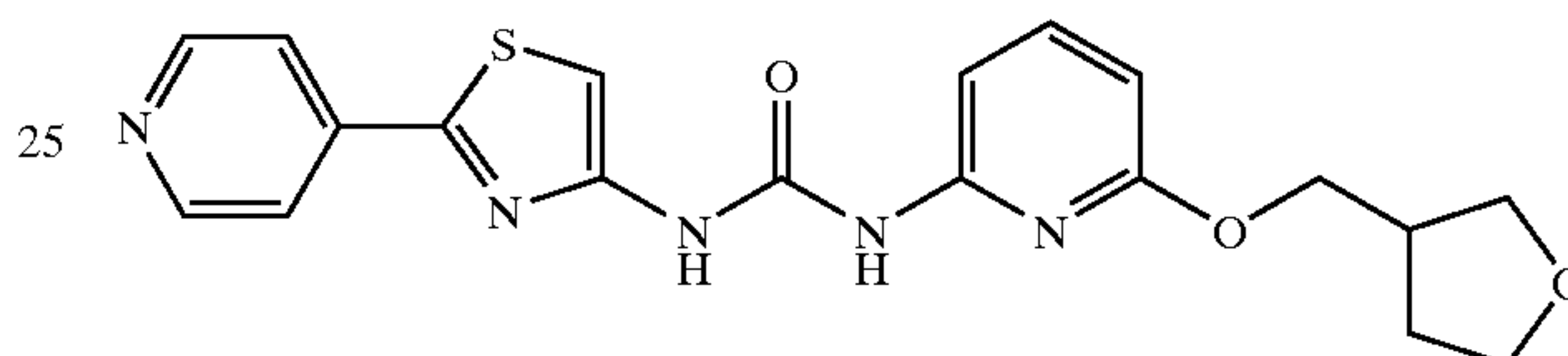
1-(2-Pyridin-4-yl-thiazol-4-yl)-3-[6-(tetrahydro-furan-3-ylmethoxy)-pyridin-2-yl]-urea
