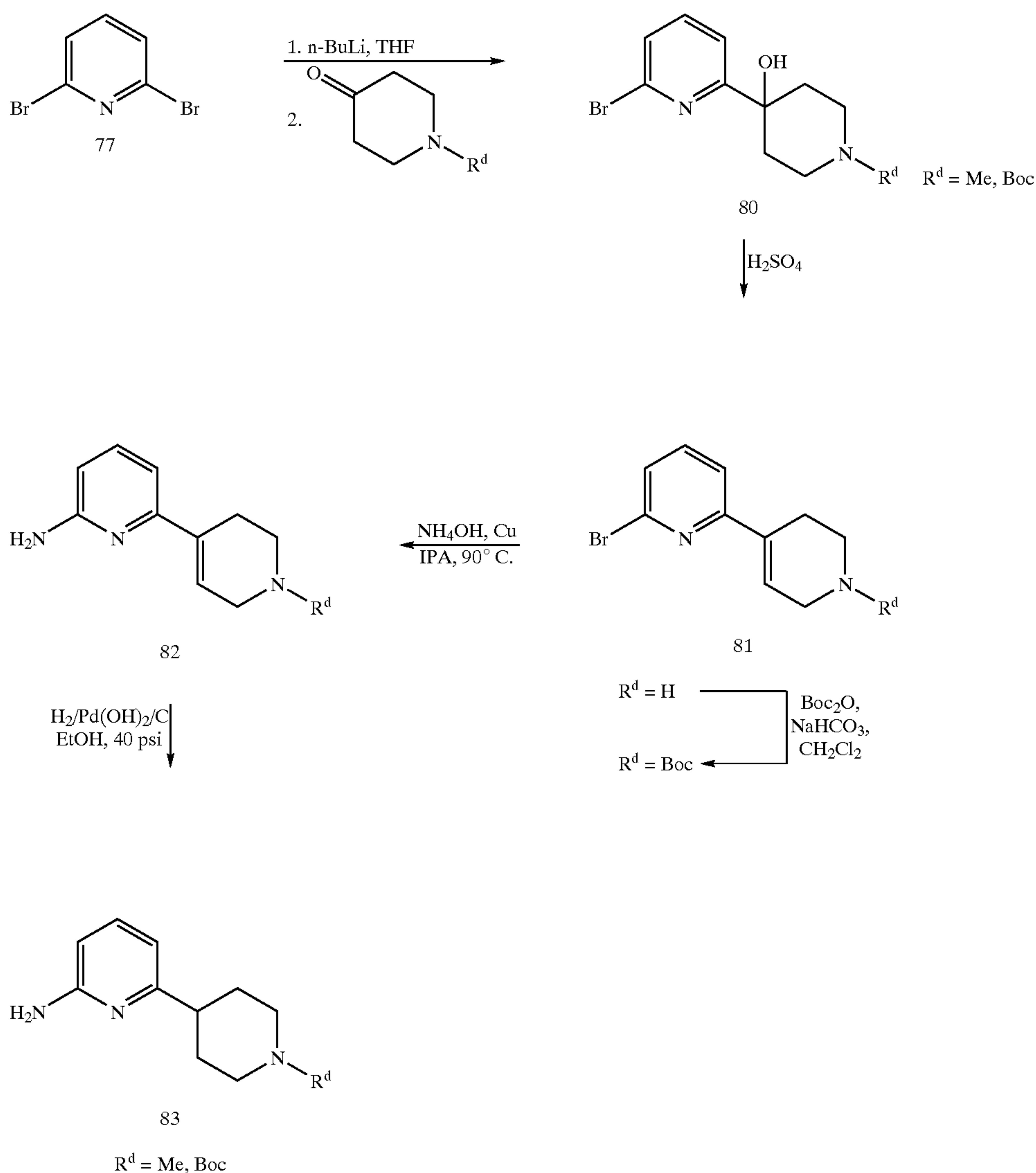
Scheme 22
