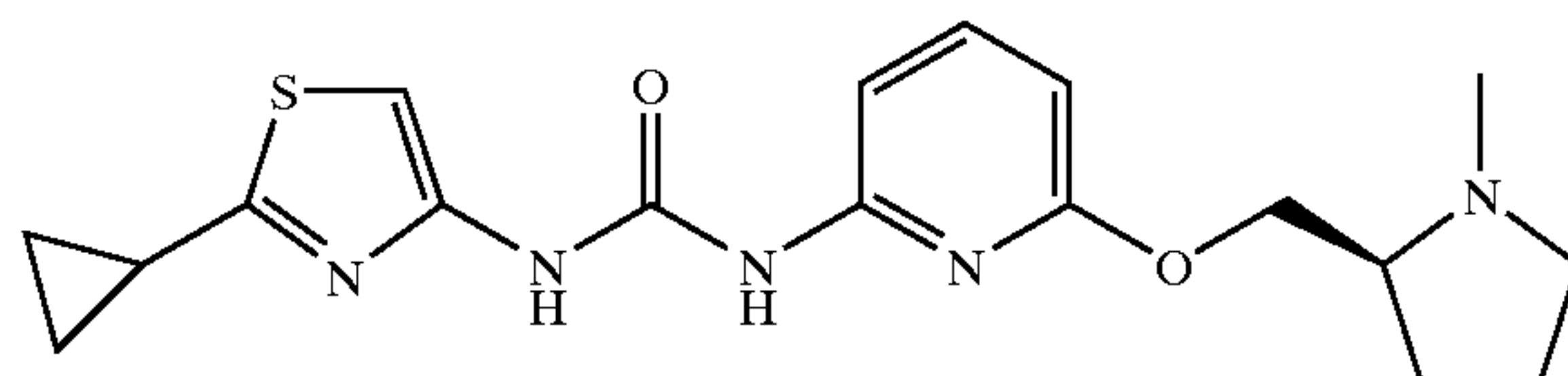
1-(2-Cyclopropyl-thiazol-4-yl)-3-[6-(1-methyl-pyrrolidin-2-ylmethoxy)-pyridin-2-yl]-urea
