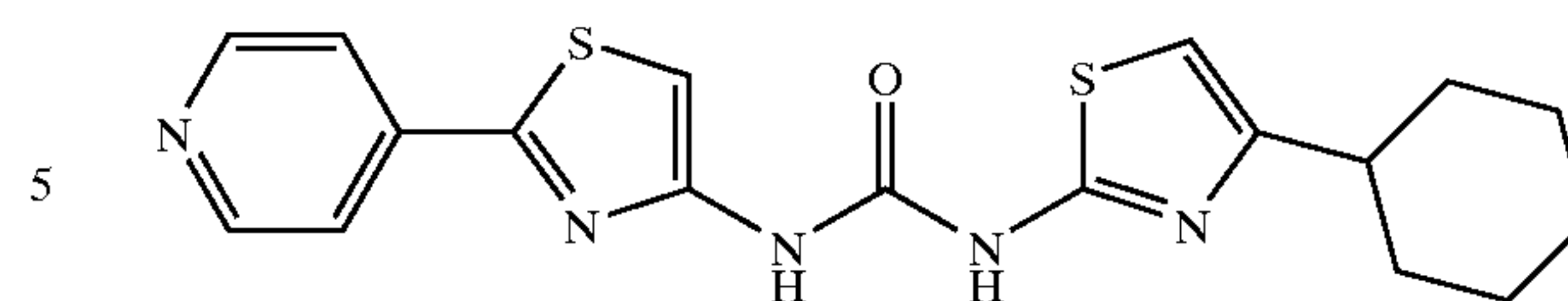
1-(4-Cyclohexylthiazol-2-yl)-3-[2-(pyridin-4-yl)-thiazol-4-yl]urea
