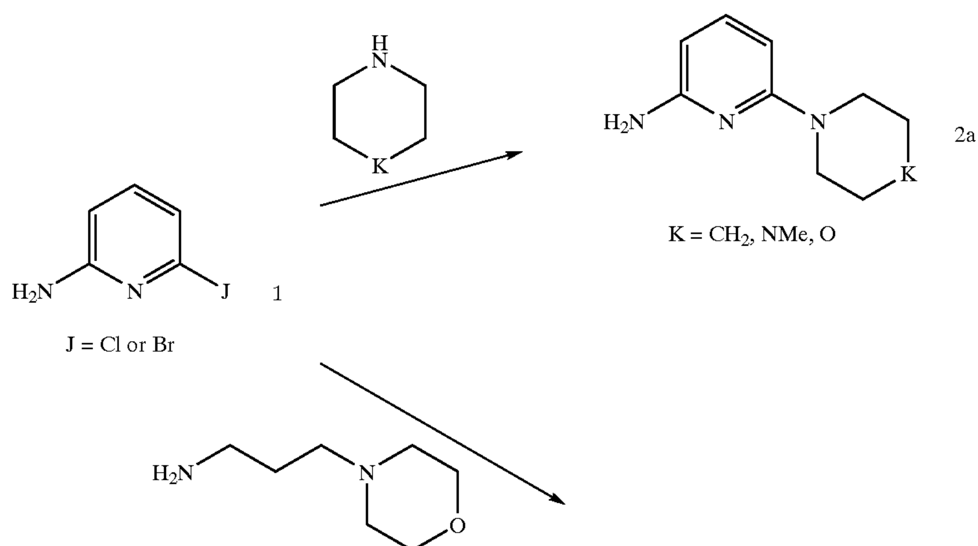
Scheme 1
