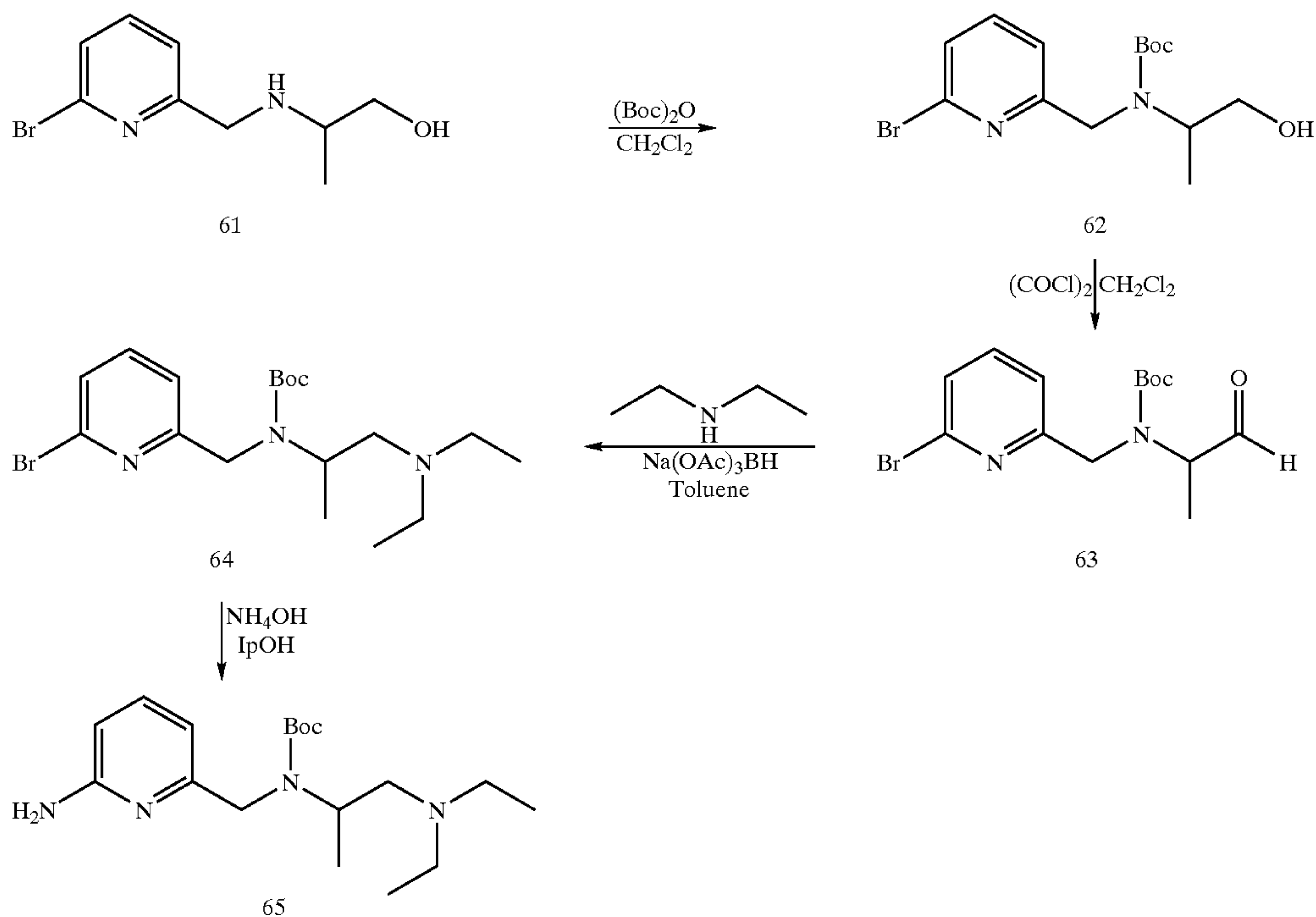
Scheme 17
