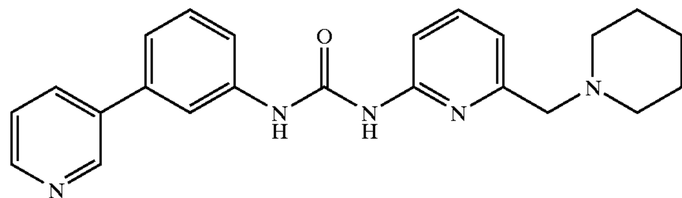
1-[6-(Piperidin-1-ylmethyl)pyridin-2-yl]-3-(3-pyridin-3-yl-phenyl)urea
