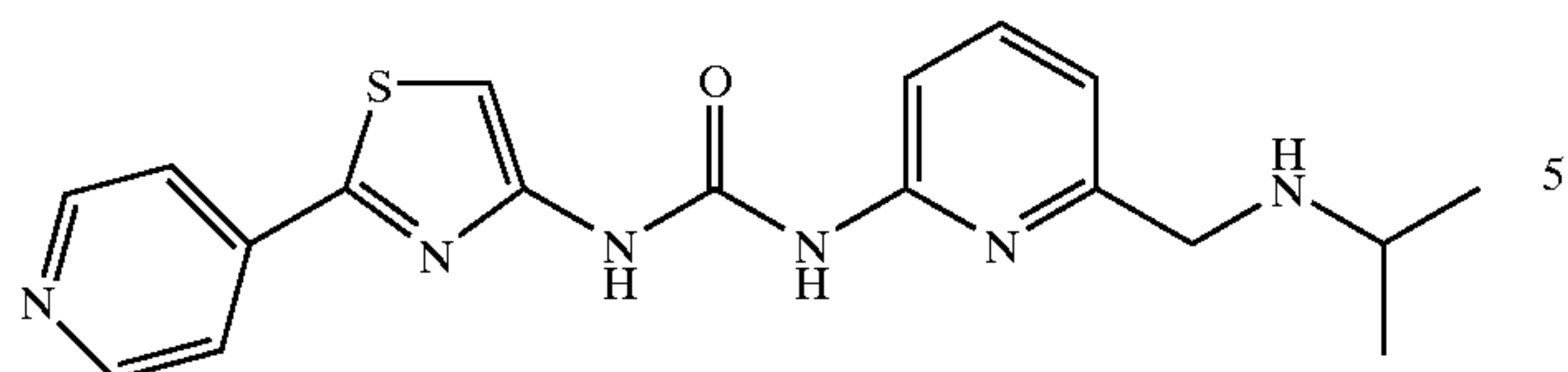
1-[6-(Isopropylamino-methyl)-pyridin-2-yl]-3-(2-pyridin-4-yl-thiazol-4-yl)-urea
