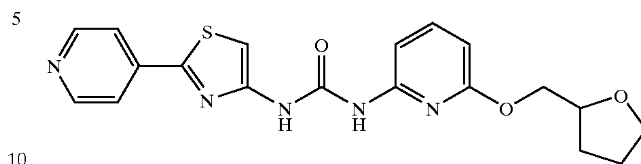
1-(2-Pyridin-4-yl-thiazol-4-yl)-3-[6-(tetrahydro-furan-2-ylmethoxy)-pyridin-2-yl]-urea
