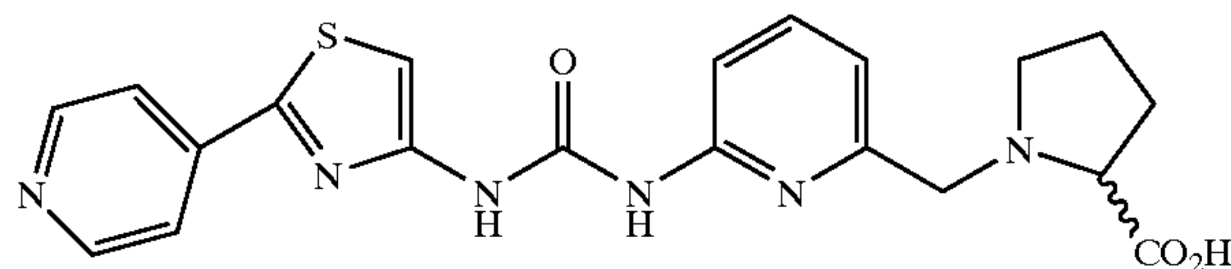
1-{6-[3-(2-Pyridin-4-yl-thiazol-4-yl)ureido]-pyridin-2-ylmethyl}-pyrrolidine-2-carboxylic Acid
