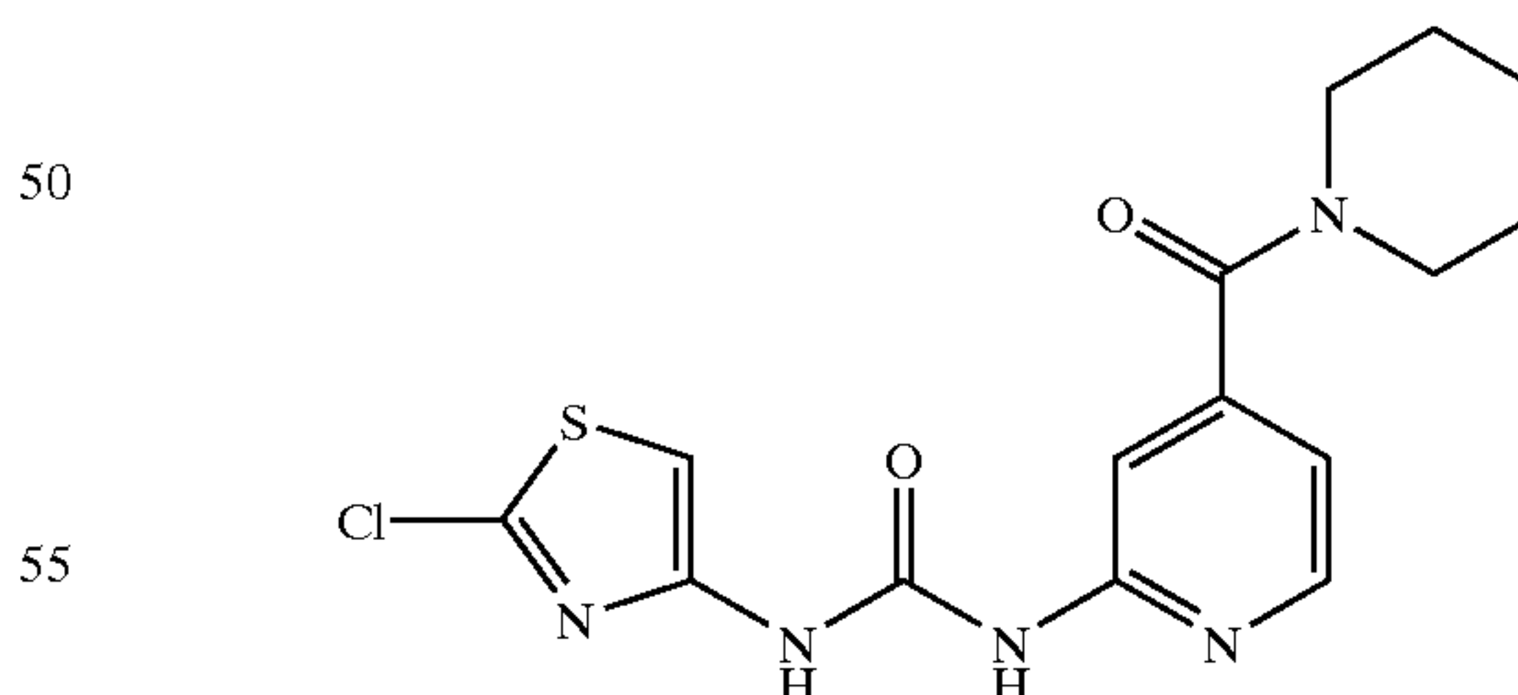
1-(2-Pyridin-4-yl-thiazol-4-yl)-3-[6-(2,2,6,6-tetramethyl-piperidin-1-ylmethyl)-pyridin-2-yl]-urea
