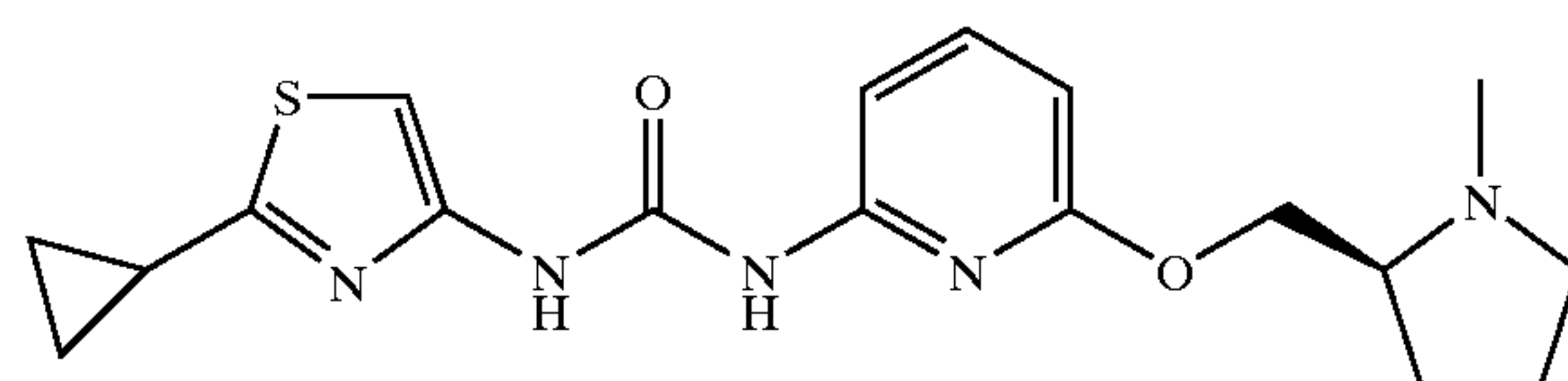
1-(2-Cyclopropyl-thiazol-4-yl)-3-[6-(1-methyl-pyrrolidin-2-ylmethoxy)-pyridin-2-yl]-urea
