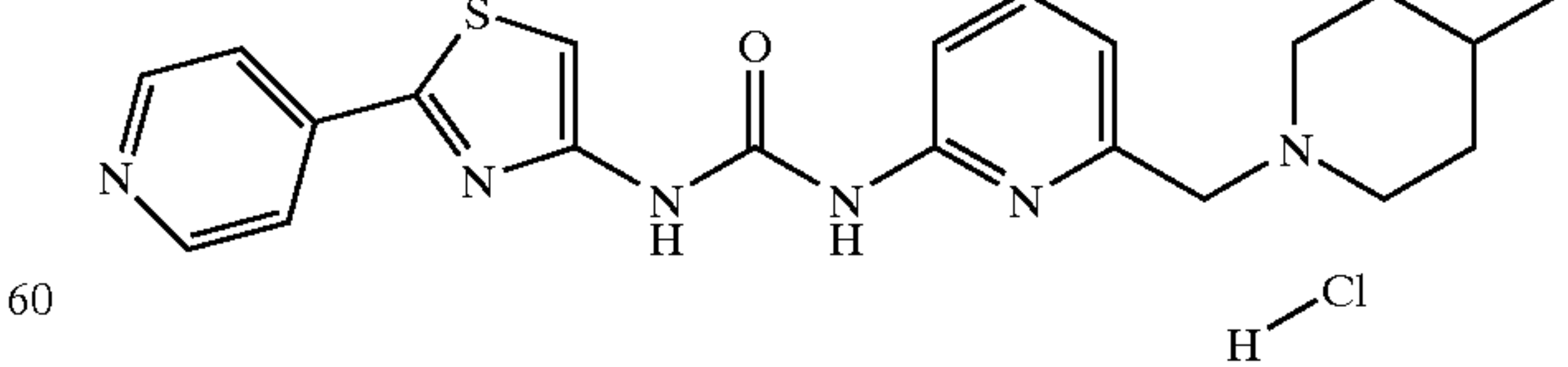
1-[6-(4-Methylpiperidin-1-ylmethyl)pyridin-2-yl]-3-(2-pyridin-4-yl-thiazol-4-yl)urea hydrochloride
