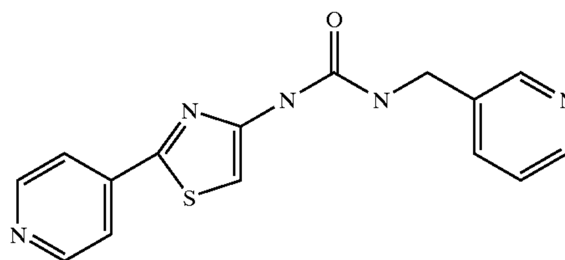
1-(Pyridin-3-ylmethyl)-3-(2-pyridin-4-yl-thiazol-4-yl)urea
