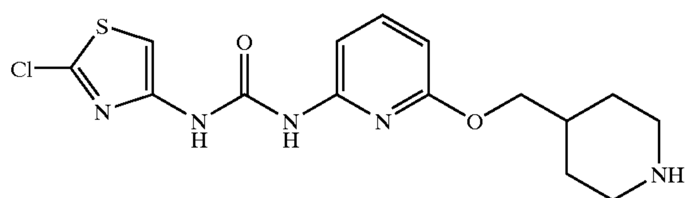
1-(2-Chloro-thiazol-4-yl)-3-[6-(piperidin-4-ylmethoxy)-pyridin-2-yl]-urea
