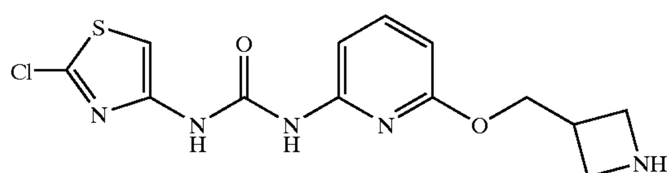
1-[6-(Azetidin-3-ylmethoxy)-pyridin-2-yl]-3-(2-chloro-thiazol-4-yl)-urea
