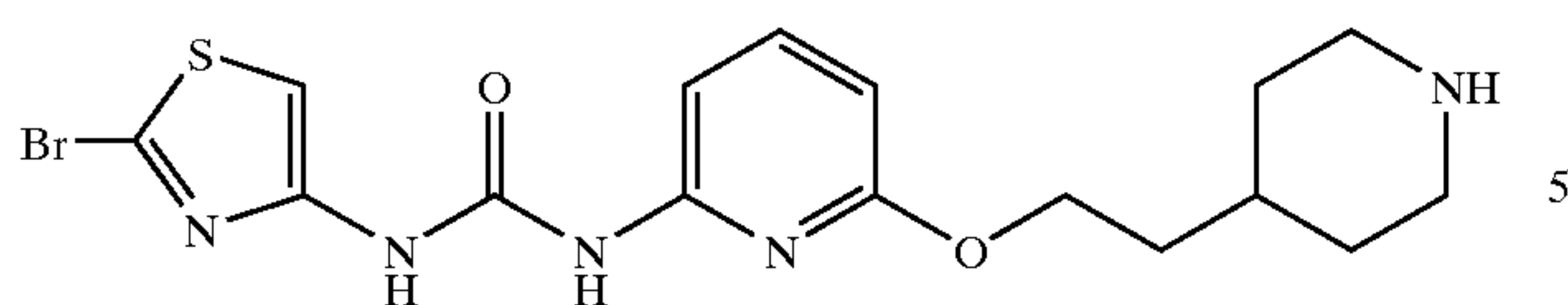
1-(2-Bromo-thiazol-4-yl)-3-[6-(2-piperidin-4-ylethoxy)-pyridin-2-yl]-urea
