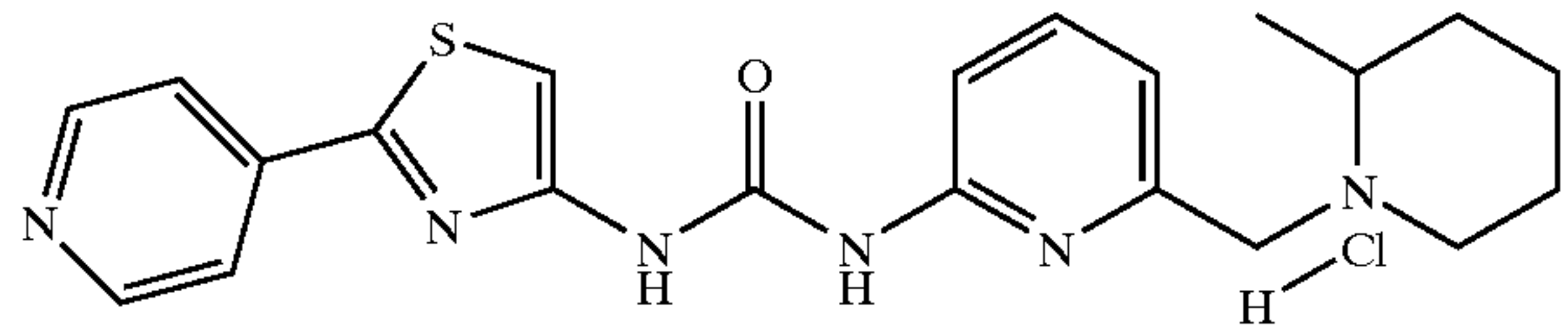
1-[6-(2-Methylpiperidin-1-ylmethyl)pyridin-2-yl]-3-(2-pyridin-4-yl-thiazol-4-yl)urea
