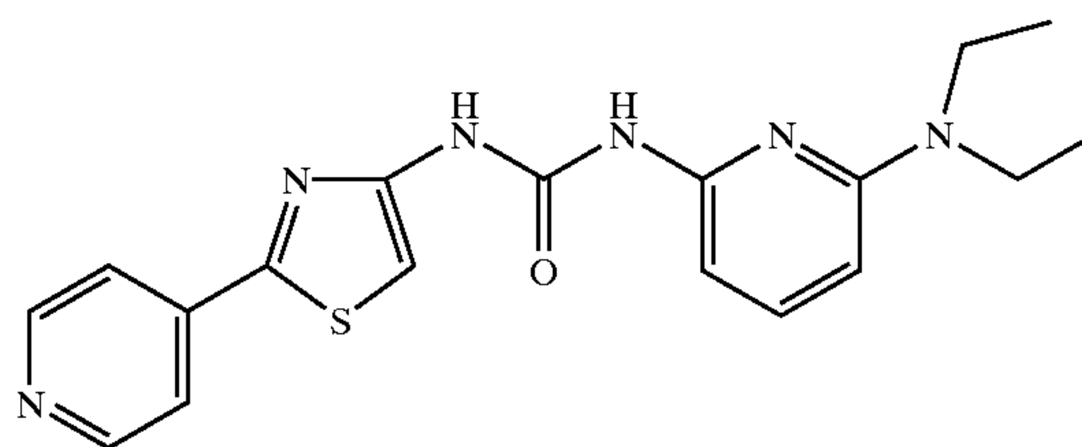
N-[2-(4-Pyridinyl)-4-thiazolyl]-N'-2-[6-(N,N-diethylamino)pyridinyl]urea
