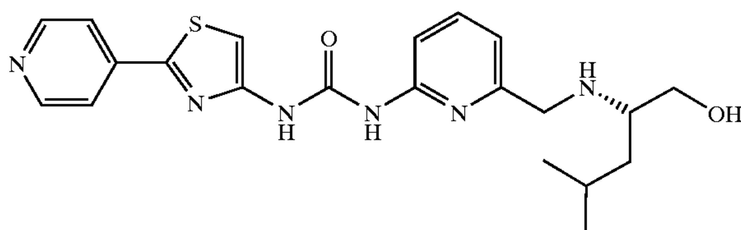
1-(6-[(1-Hydroxymethyl-3-methylbutylamino)methyl]-pyridin-2-yl)-3-(2-pyridin-4-yl-thiazol-4-yl)urea
