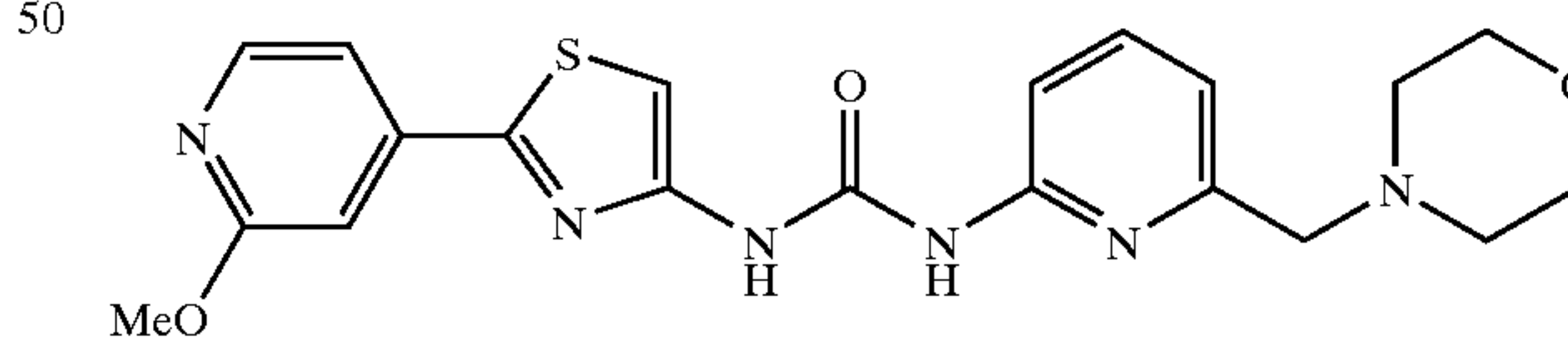
1-[2-(2-Methoxypyridin-4-yl)thiazol-4-yl]-3-(6-morpholin-4-ylmethyl-pyridin-2-yl)urea
