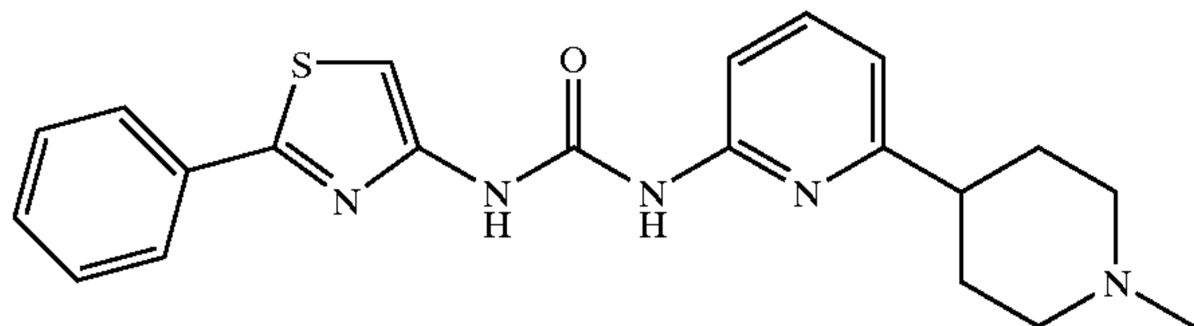
1-(1'-Methyl-1',2',3',4',5',6'-hexahydro-[2,4']bipyridinyl-6-yl)-3-(2-phenyl-thiazol-4-yl)-urea
