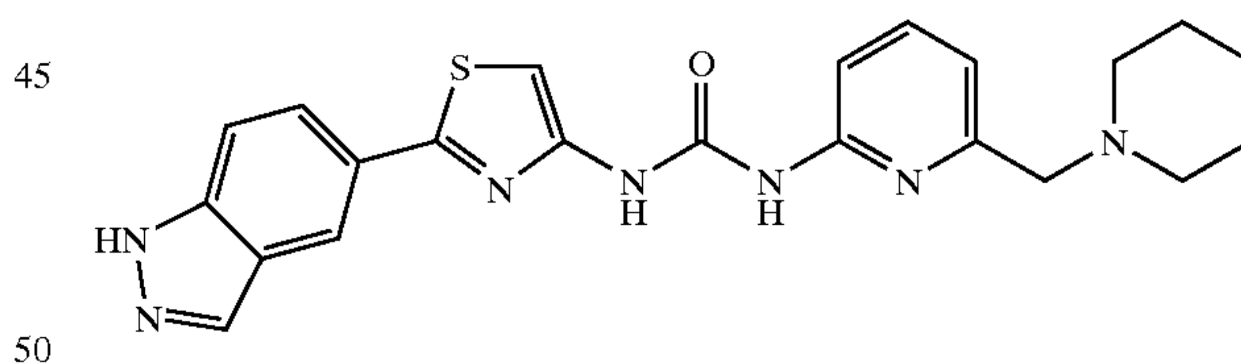
1-[2-(1H-Indazol-5-yl)-thiazol-4-yl]-3-(6-piperidin-1-ylmethylpyridin-2-yl)-urea
