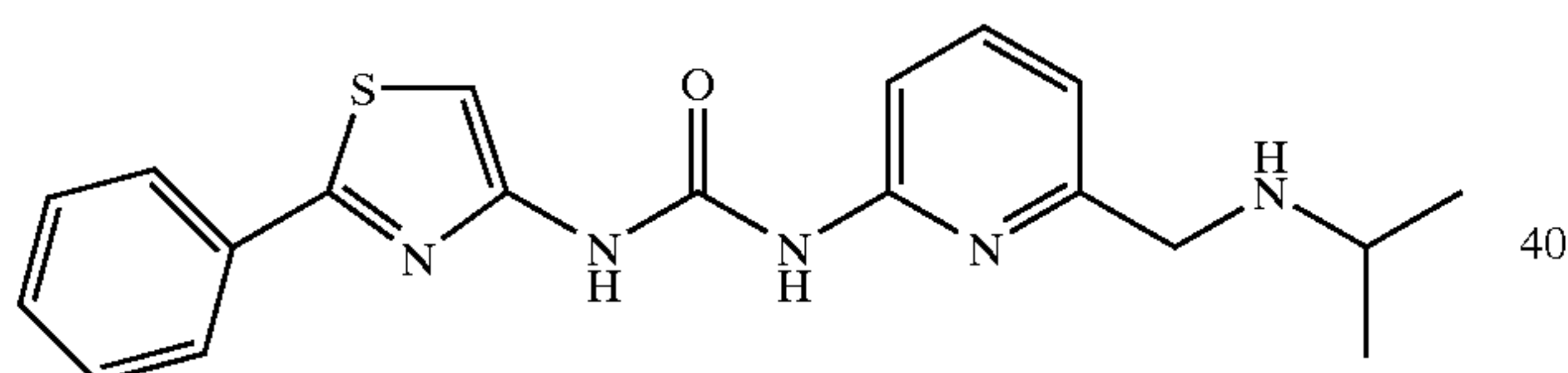
1-[6-(Isopropylamino-methyl)-pyridin-2-yl]-3-(2-phenyl-thiazol-4-yl)-urea
