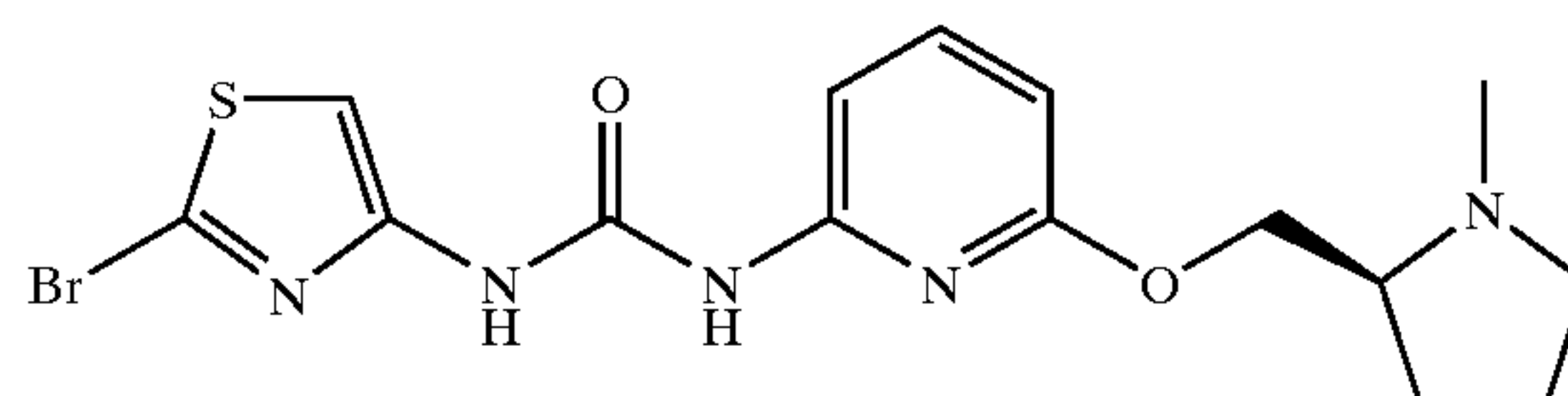
1-(2-Bromo-thiazol-4-yl)-3-[6-(1-methyl-pyrrolidin-2-ylmethoxy)-pyridin-2-yl]-urea
