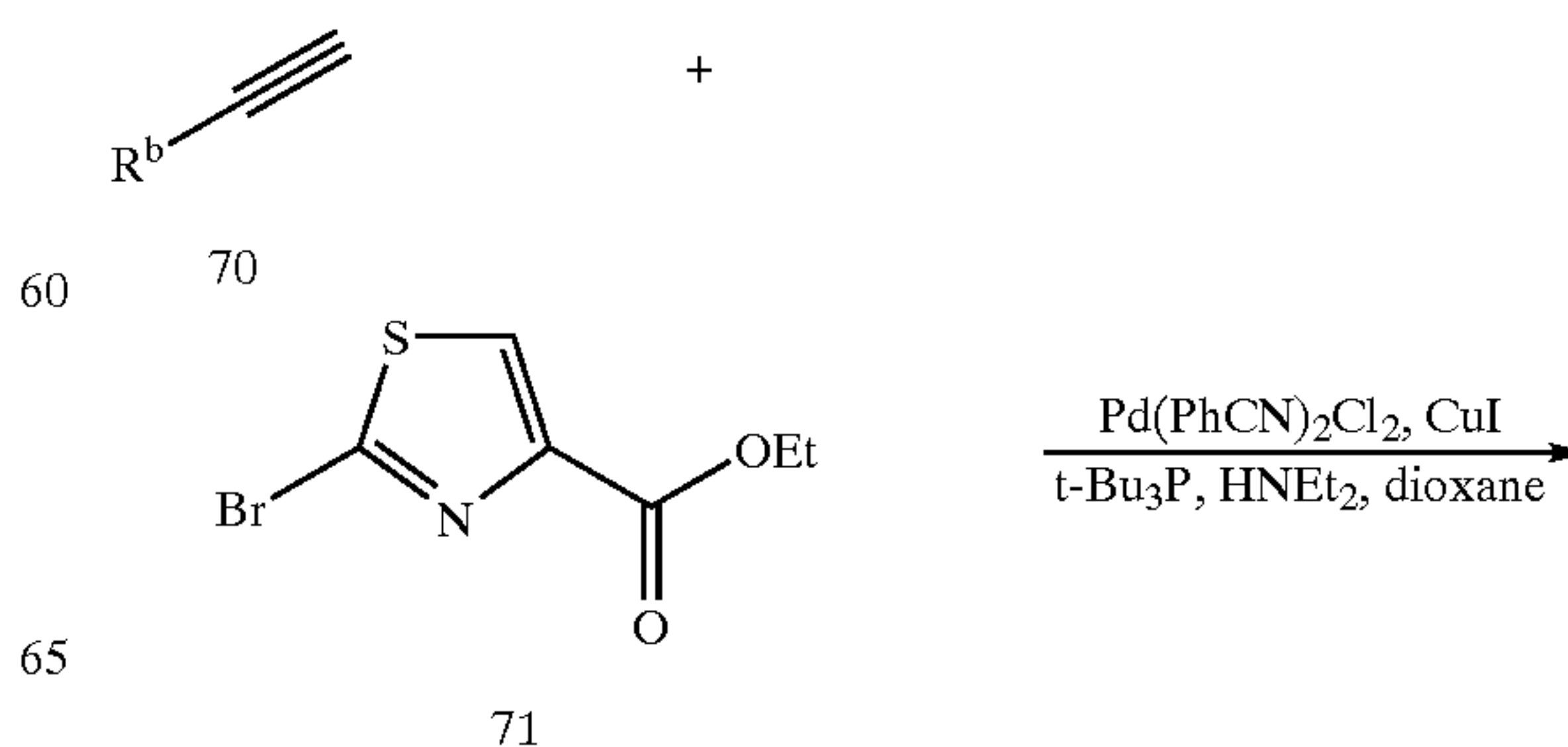
Scheme 19
