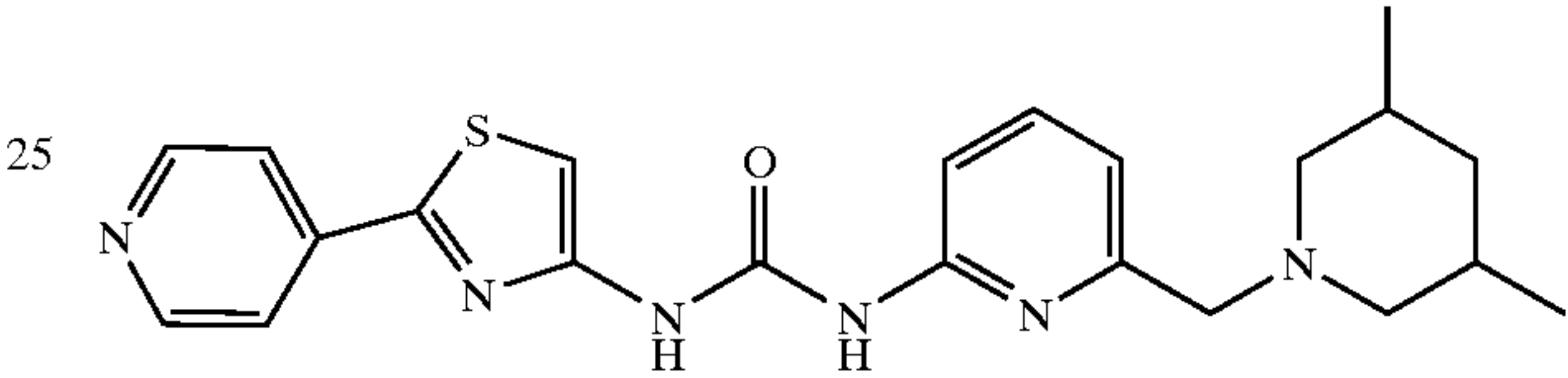
1-[6-(3,5-Dimethylpiperidin-1-ylmethyl)pyridin-2-yl]-3-(2-pyridin-4-ylthiazol-4-yl)urea Hydrochloride
