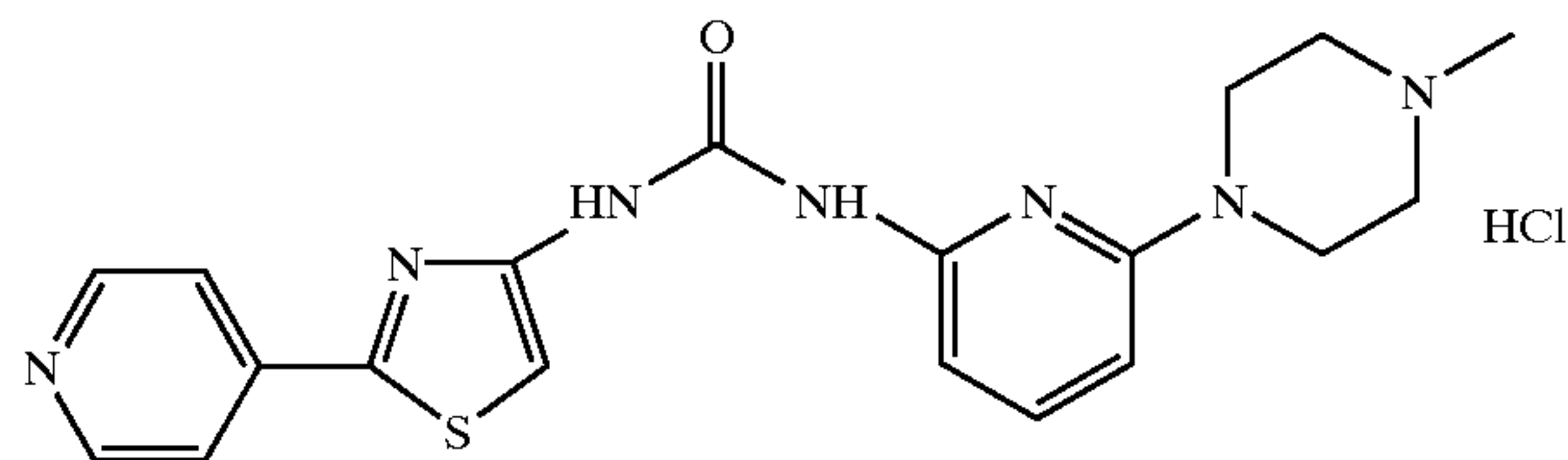
N-[2-(4-Pyridinyl)-4-thiazolyl]-N'-2-[6-(1-methyl-4-piperazinyl)pyridinyl]urea Hydrochloride
