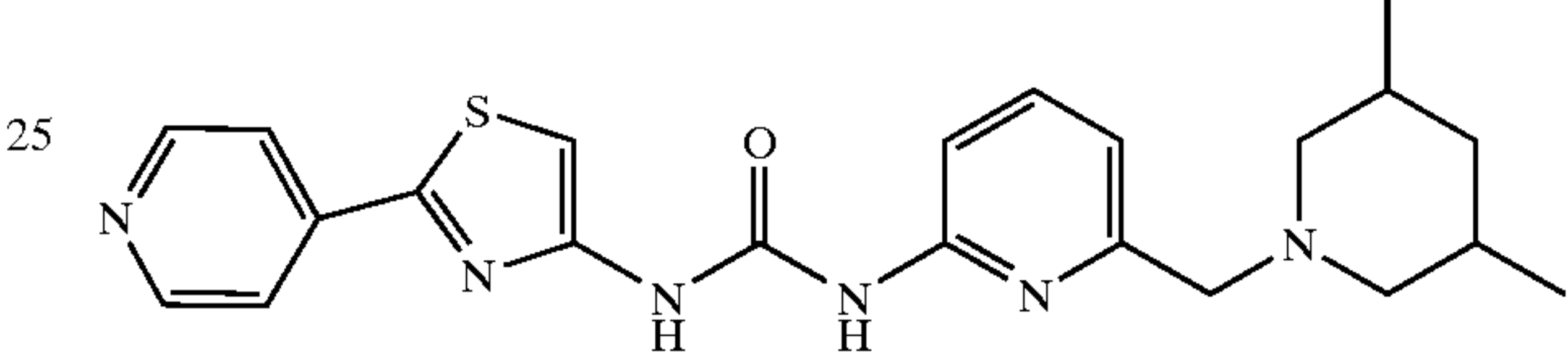
1-[6-(3,5-Dimethylpiperidin-1-ylmethyl)pyridin-2-yl]-3-(2-pyridin-4-ylthiazol-4-yl)urea Hydrochloride
