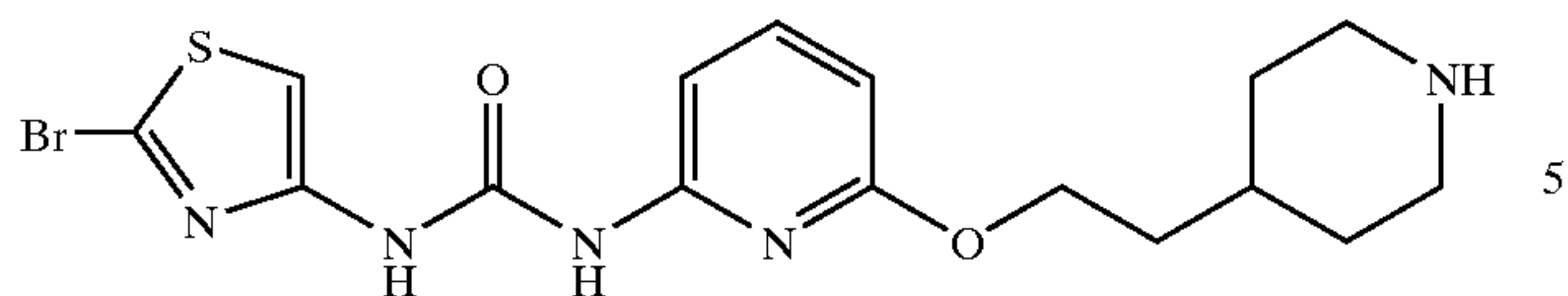
1-(2-Bromo-thiazol-4-yl)-3-[6-(2-piperidin-4-ylethoxy)-pyridin-2-yl]-urea
