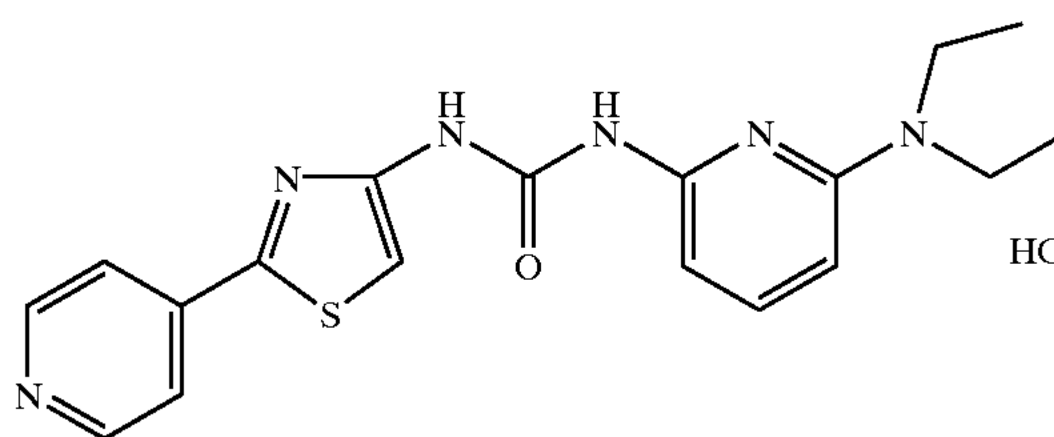
N-[2-(4-Pyridinyl)-4-thiazolyl]-N'-2-[6-(N,N-diethylamino)pyridinyl]urea Hydrochloride
