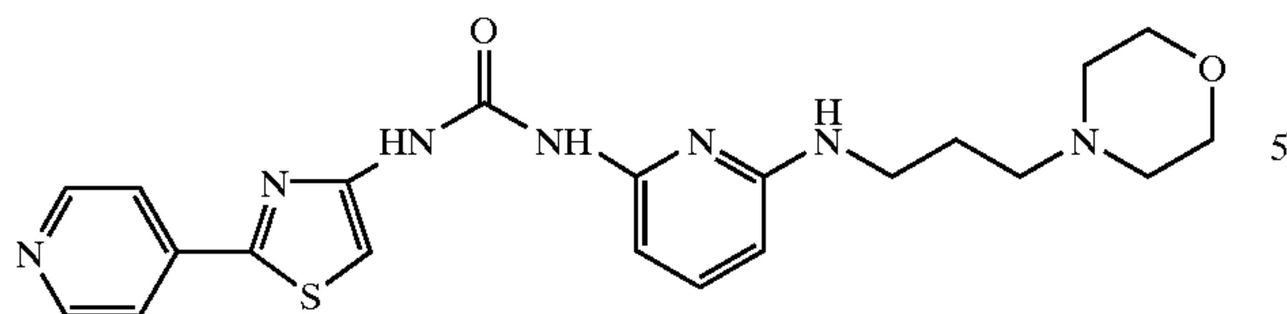
N-[2-(4-Pyridinyl)-4-thiazolyl]-N'-2-[6-[3-(1-morpholinyl)propyl]amino]pyridinyl]urea
