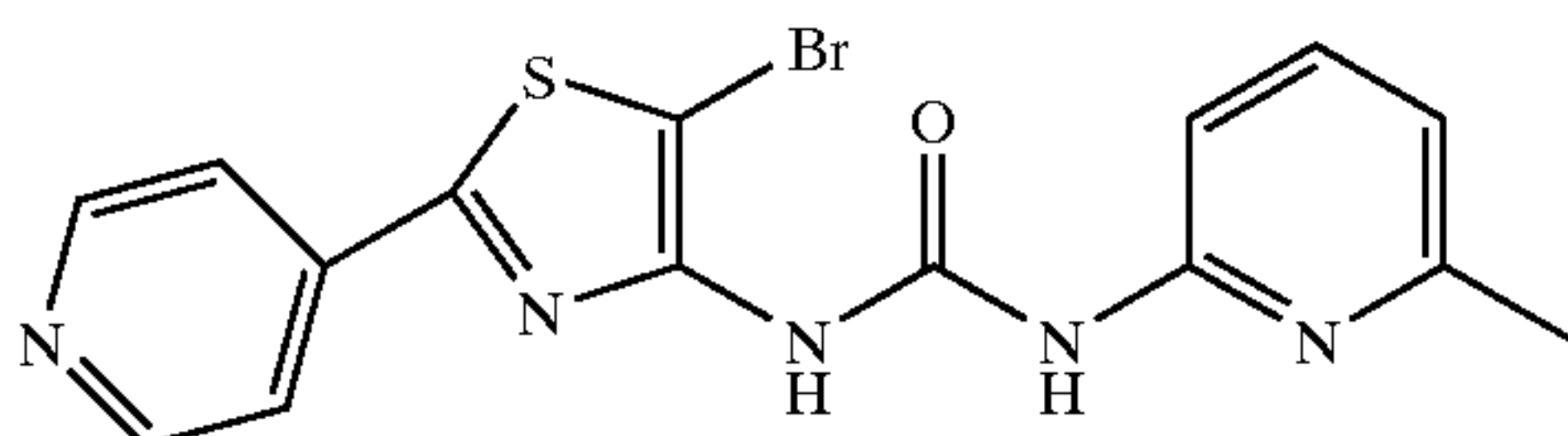
1-(5-Bromo-(2-pyridin-4-yl)thiazol-4-yl)-3-(6-methylpyridin-2-yl)urea
