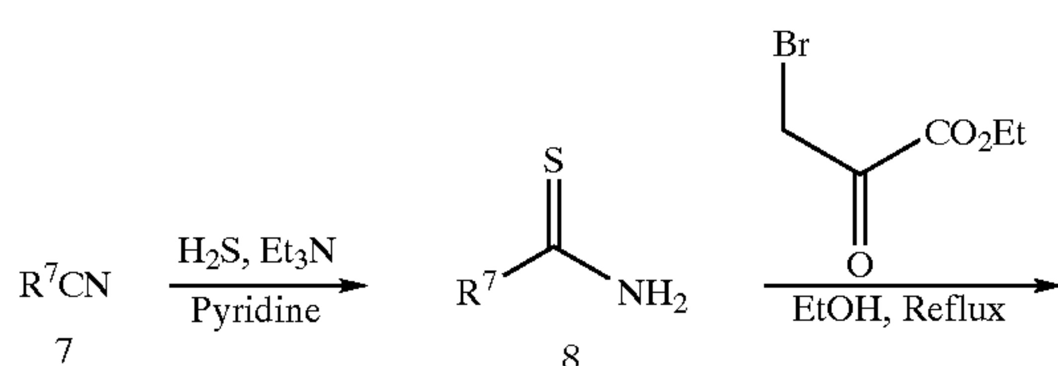
Scheme 3
