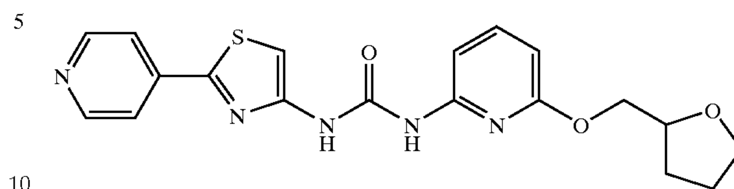
1-(2-Pyridin-4-yl-thiazol-4-yl)-3-[6-(tetrahydro-furan-2-ylmethoxy)-pyridin-2-yl]-urea
