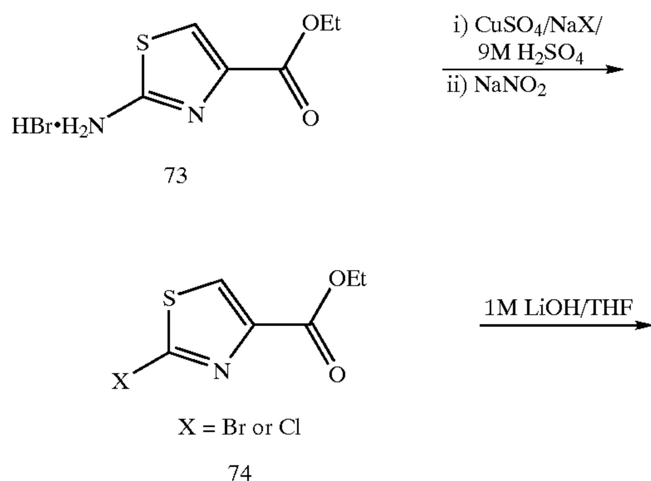
Scheme 20
