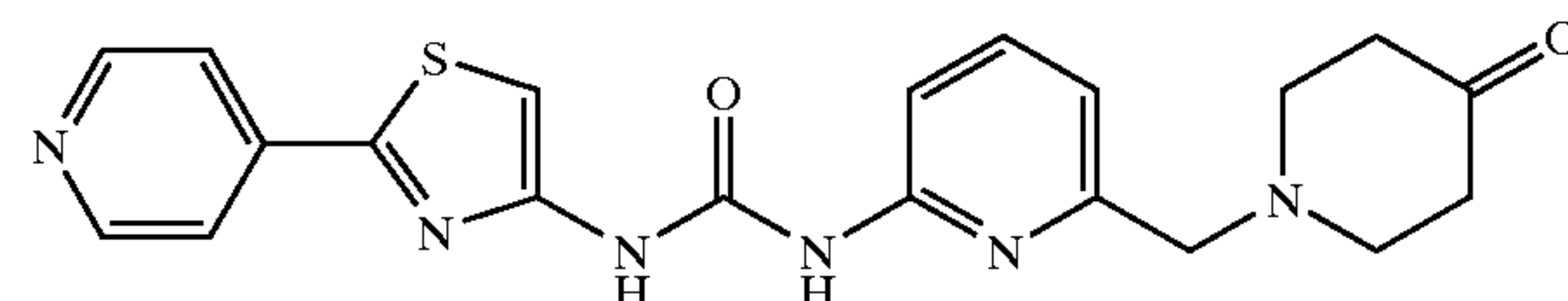
1-[6-(4-Oxo-piperidin-1-ylmethyl)pyridin-2-yl]-3-(2-pyridin-4-yl-thiazol-4-yl)urea
