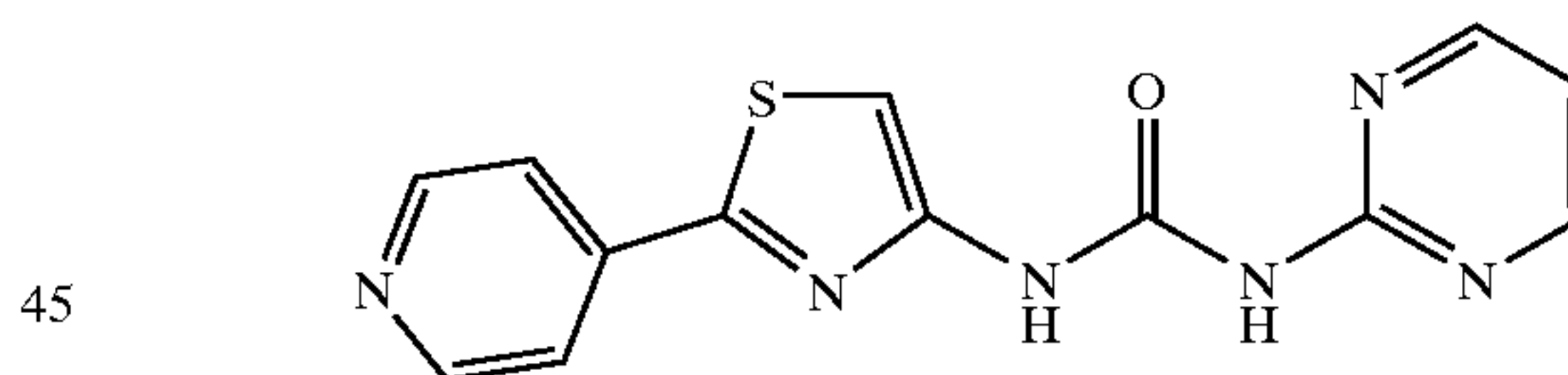
1-(2-Pyridin-4-yl-thiazol-4-yl)-3-pyrimidin-2-yl-urea
