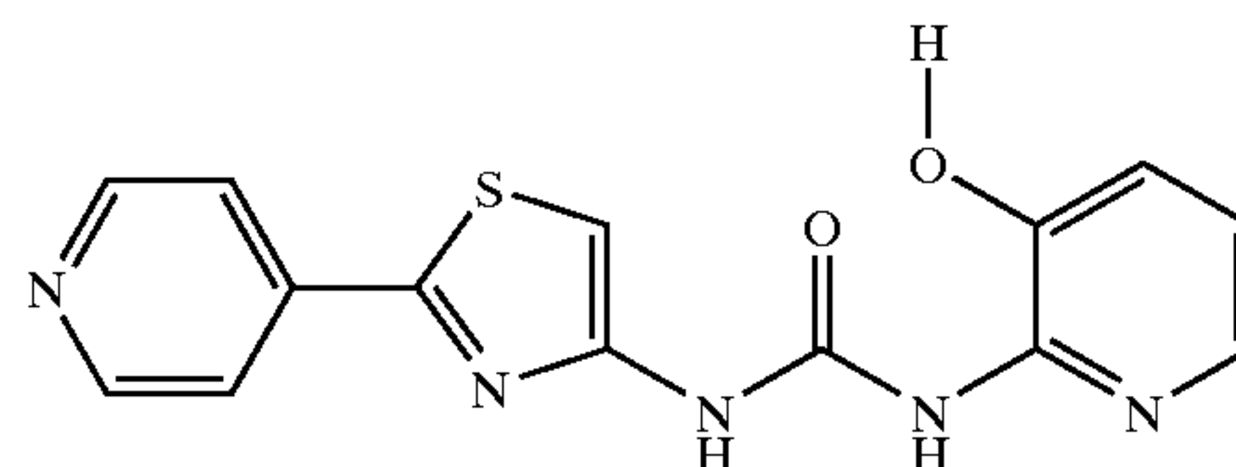
1-(3-Hydroxy-pyridin-2-yl)-3-(2-pyridin-4-yl-thiazol-4-yl)-urea
