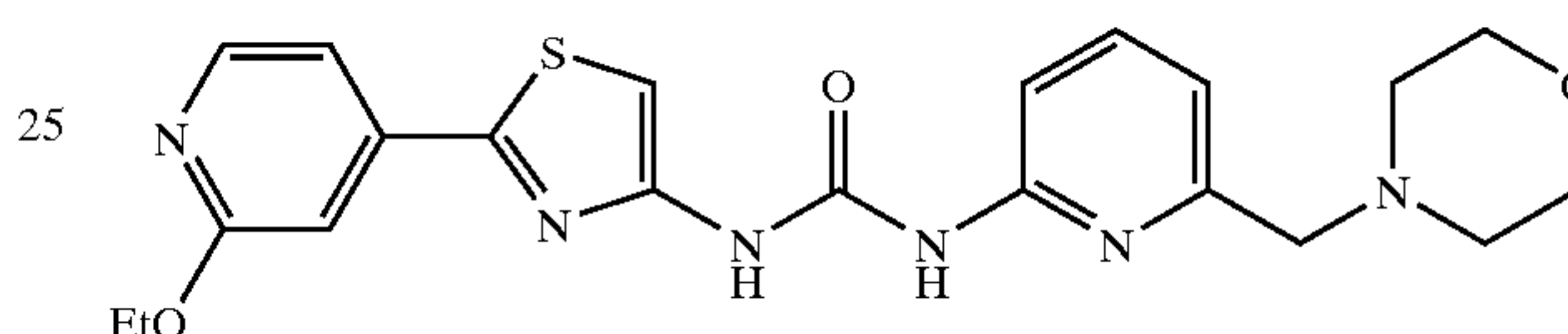
1-[2-(2-Ethoxypyridin-4-yl)thiazol-4-yl]-3-(6-morpholin-4-ylmethyl-pyridin-2-yl)urea
