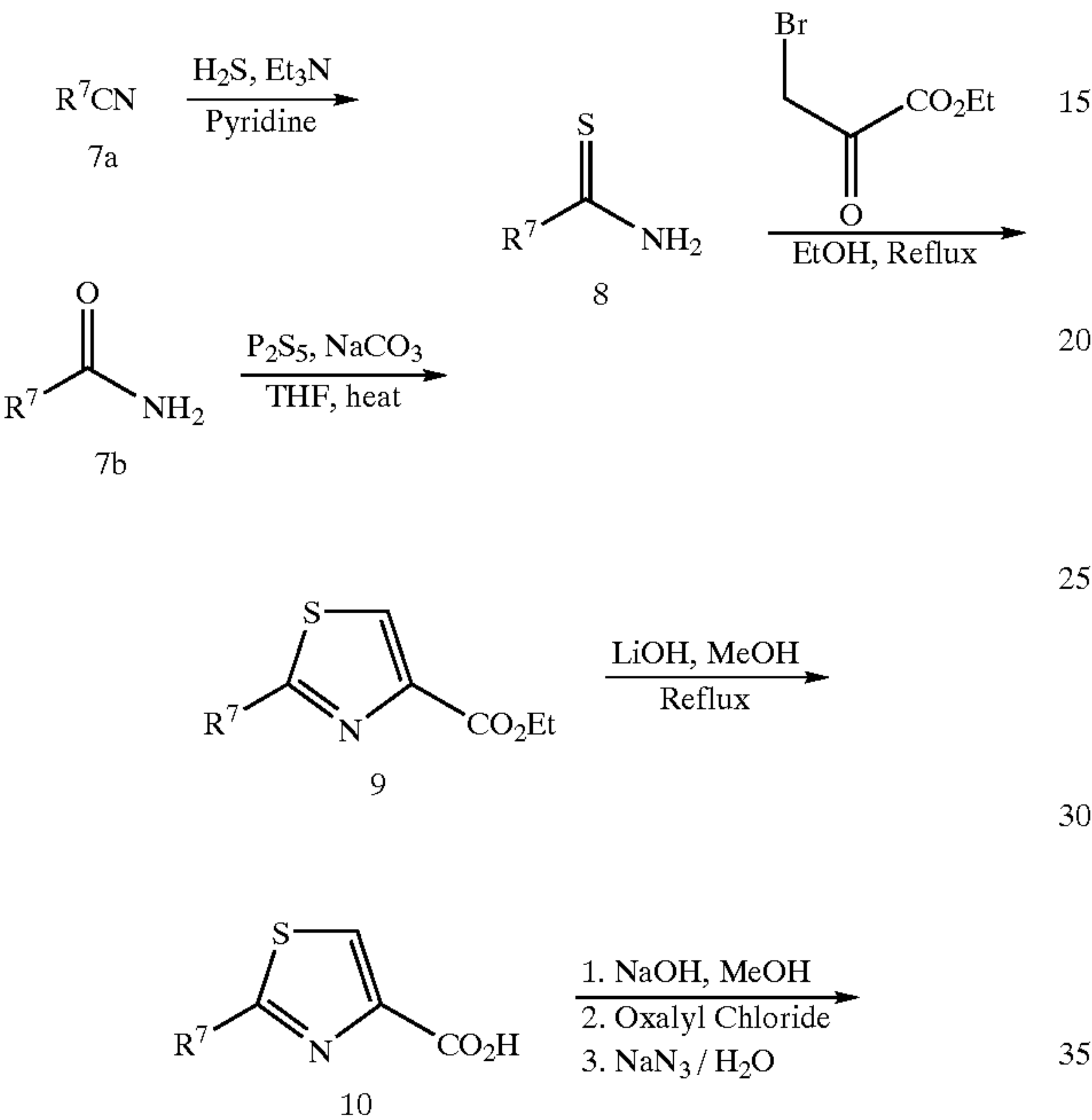
Scheme 4
