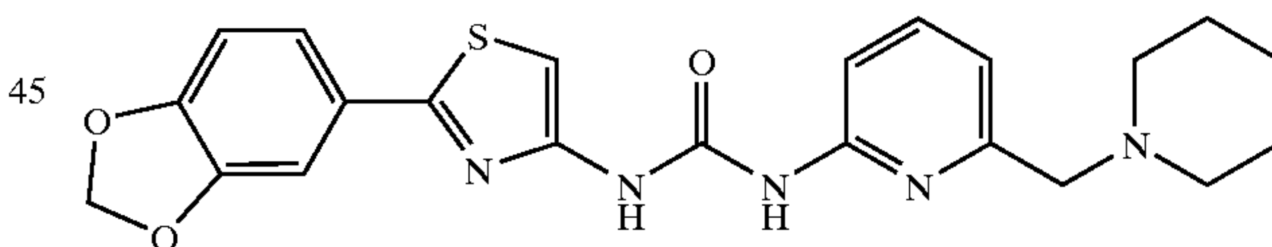
1-(2-Benzo[1,3]dioxol-5-ylthiazol-4-yl)-3-(6-piperidin-1-ylmethylpyridin-2-yl)urea
