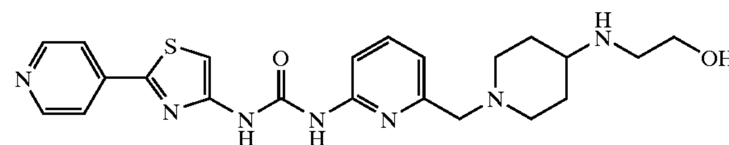
1-{6-[4-(2-Hydroxyethylamino)piperidin-1-ylmethyl]-pyridin-2-yl}-3-(2-pyridin-4-yl-thiazol-4-yl)urea
