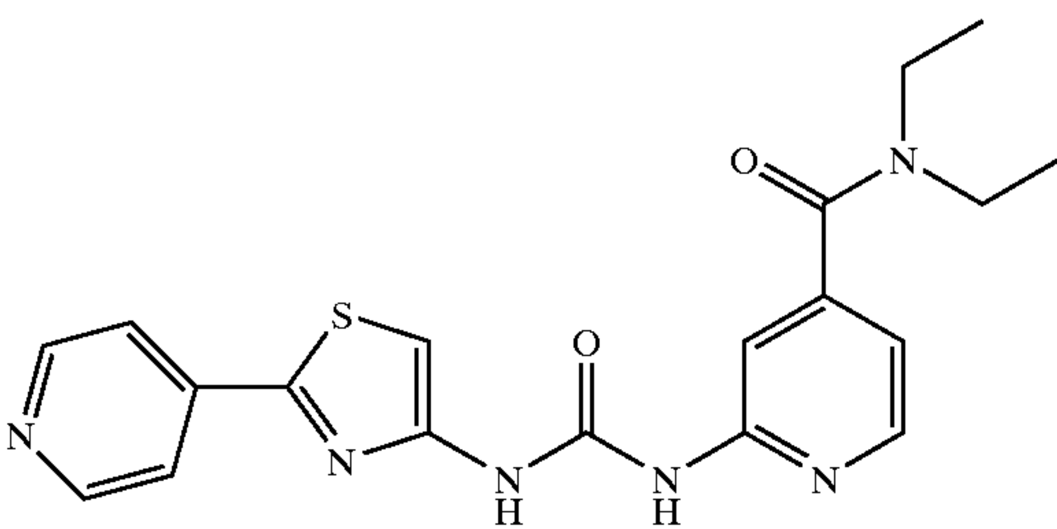
1-(4-Diethylaminomethyl-pyridin-2-yl)-3-(2-pyridin-4-yl-thiazol-4-yl)-urea
