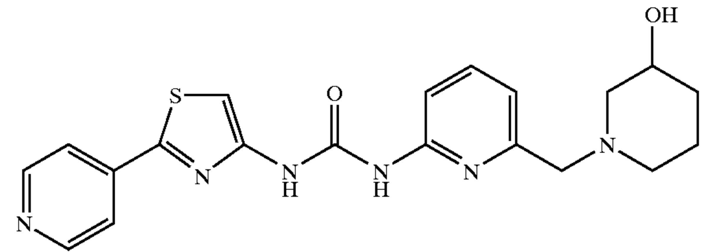
1-[6-(3-Hydroxy-piperidin-1-ylmethyl)-pyridin-2-yl]-3-(2-pyridin-4-yl-thiazol-4-yl)-urea
