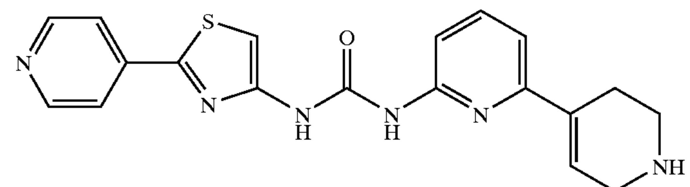
1-(2-Pyridin-4-yl-thiazol-4-yl)-3-(1',2',3',6'-tetrahydro-[2,4']bipyridinyl-6-yl)-urea
