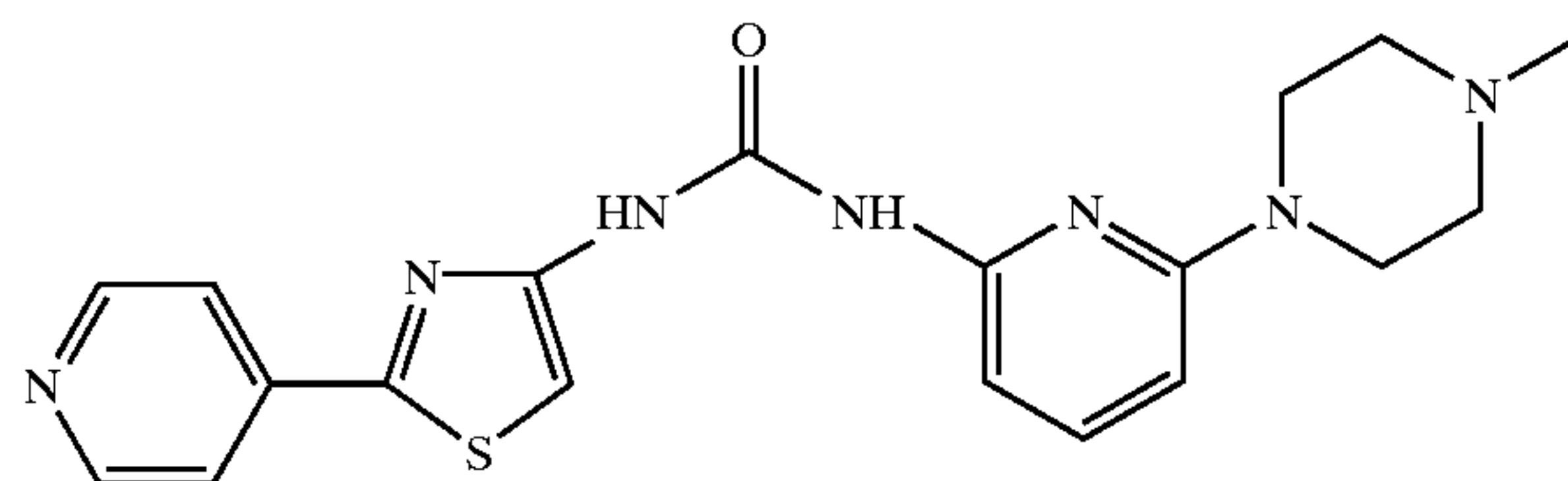
N-[2-(4-Pyridinyl)-4-thiazolyl]-N'-2-[6-(1-methyl-4-piperazinyl)pyridinyl]urea
