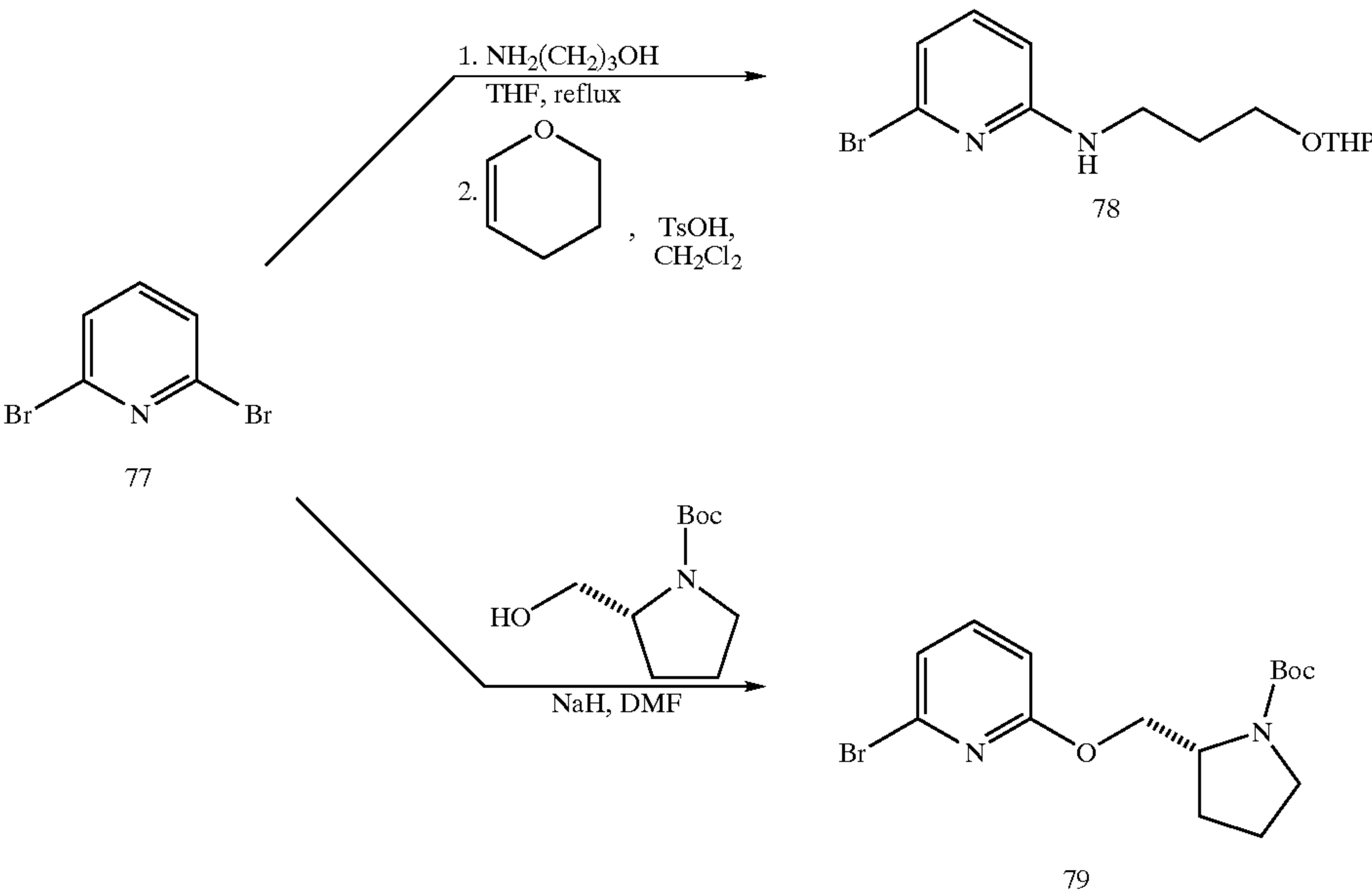
Scheme 21
