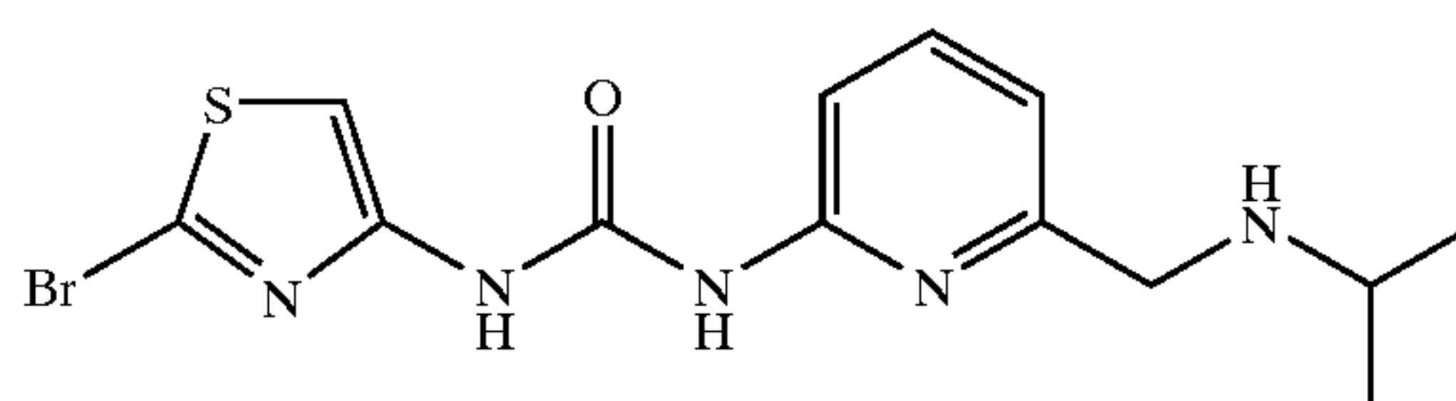
1-(2-Bromo-thiazol-4-yl)-3-[6-(isopropylamino-methyl)-pyridin-2-yl]-urea
