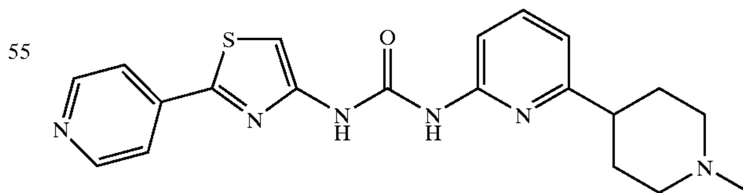
1-(1'-Methyl-1',2',3',4',5',6'-hexahydro-[2,4']bipyridinyl-6-yl)-3-(2-pyridin-4-yl-thiazol-4-yl)-urea
