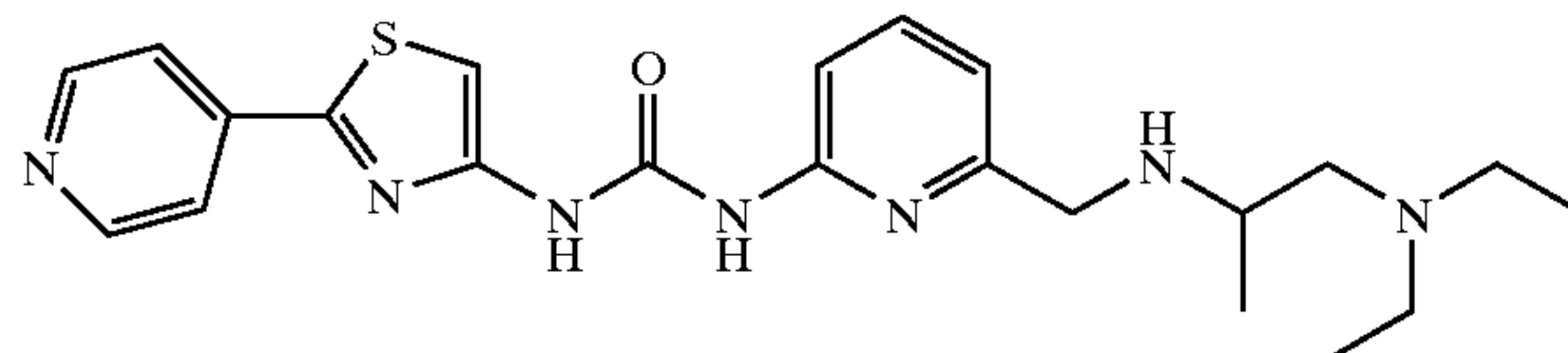
1-{6-[2-Diethylamino-1-methylethylamino)methyl]-pyridin-2-yl}-3-(2-pyridin-4-yl-thiazol-4-yl)urea
