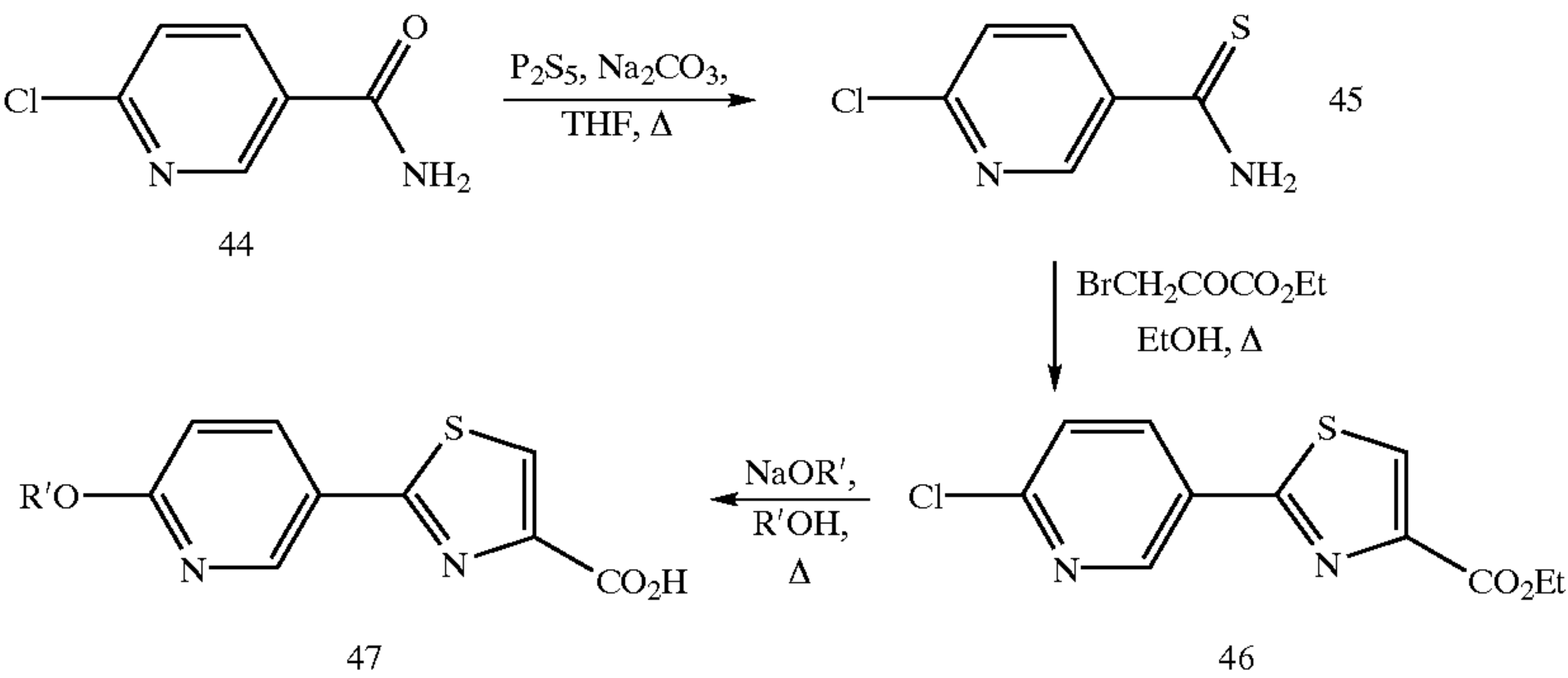
Scheme 13
