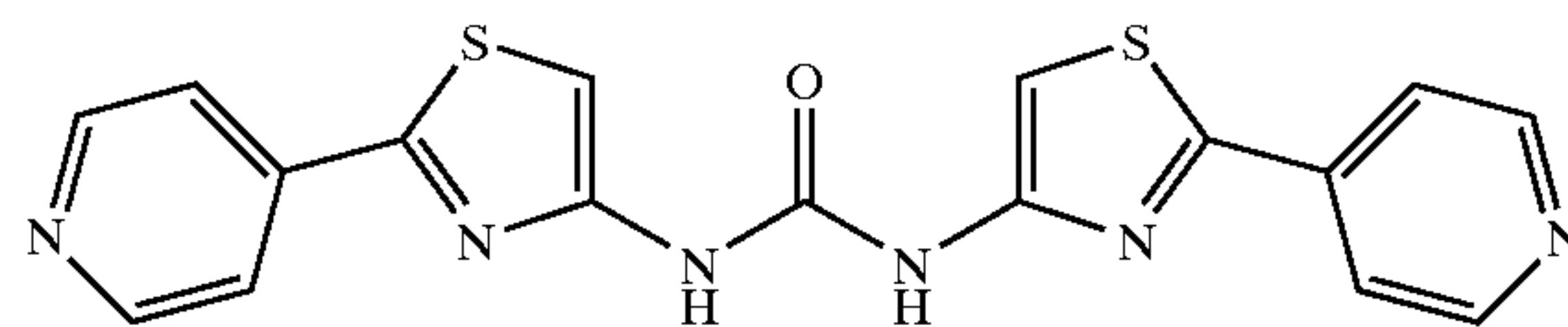
N,N'-bis [2-(4-Pyridinyl)-4-thiazolyl]urea
