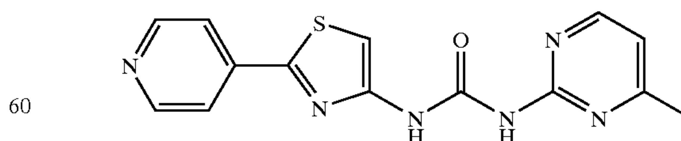
1-(4-Methyl-pyrimidin-2-yl)-3-(2-pyridin-4-yl-thiazol-4-yl)-urea
