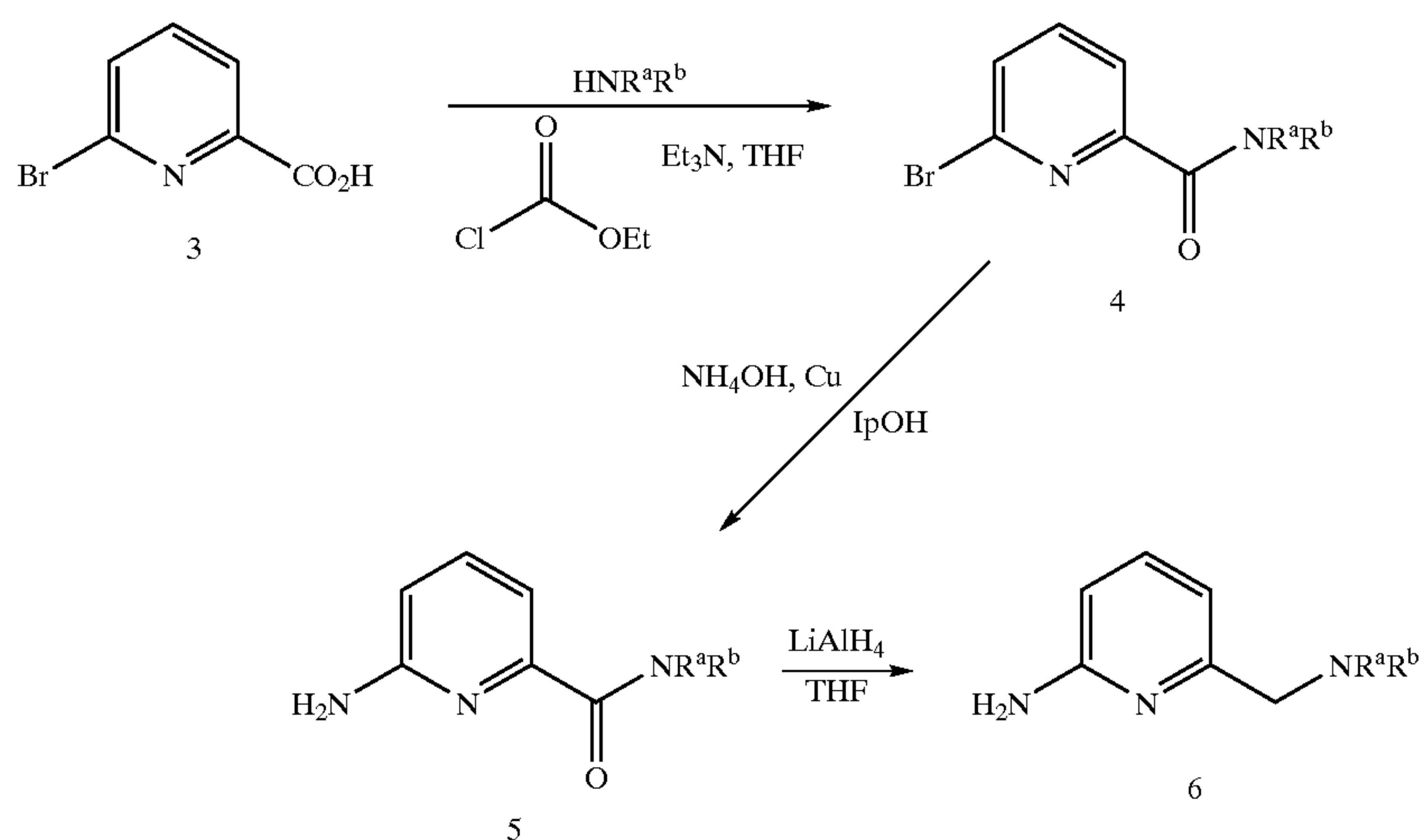
Scheme 2
