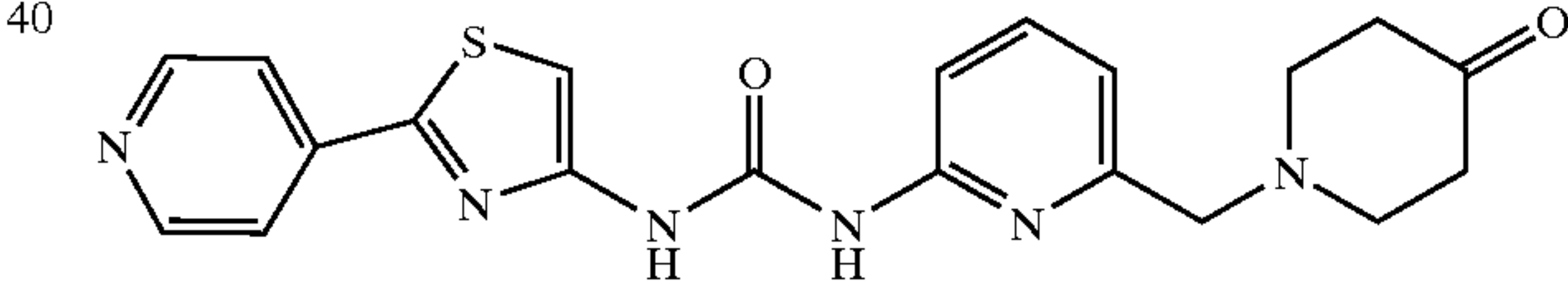
1-[6-(4-Oxo-piperidin-1-ylmethyl)pyridin-2-yl]-3-(2-pyridin-4-yl-thiazol-4-yl)urea hydrochloride
