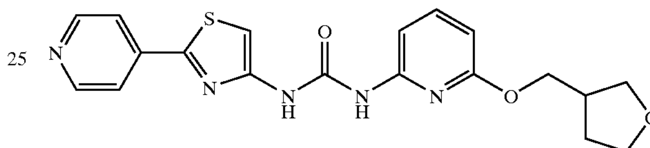
1-(2-Pyridin-4-yl-thiazol-4-yl)-3-[6-(tetrahydro-furan-3-ylmethoxy)-pyridin-2-yl]-urea
