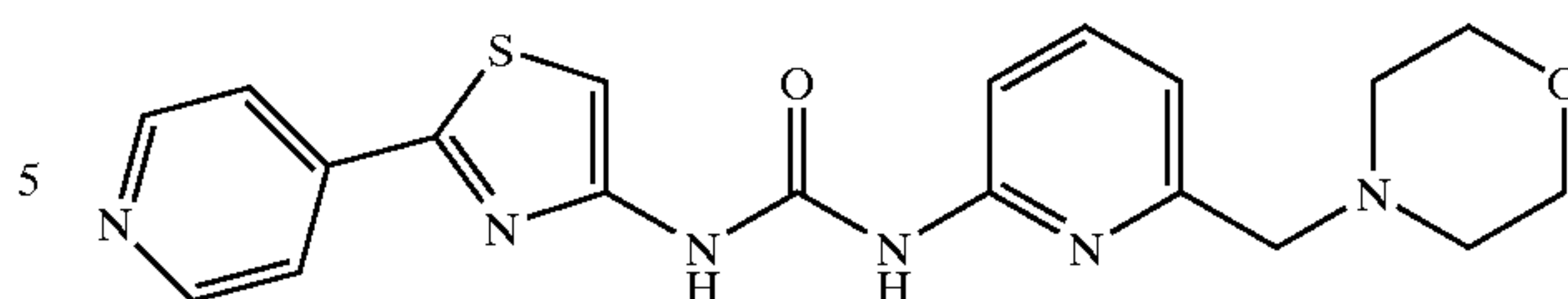
N-[2-(4-Pyridinyl)-4-thiazolyl]-N'-2-[6-(1-morpholinylmethyl)pyridinyl]urea
