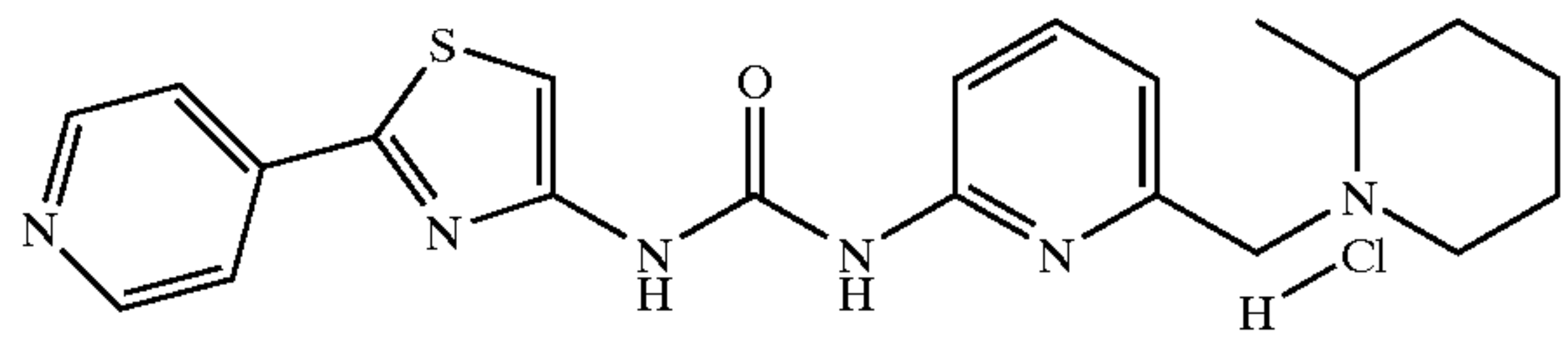
1-[6-(2-Methylpiperidin-1-ylmethyl)pyridin-2-yl]-3-(2-pyridin-4-yl-thiazol-4-yl)urea
