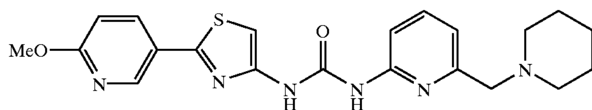
1-[2-(6-Methoxypyridin-3-yl)thiazol-4-yl]-3-(6-piperidin-1-ylmethylpyridin-2-yl)urea
