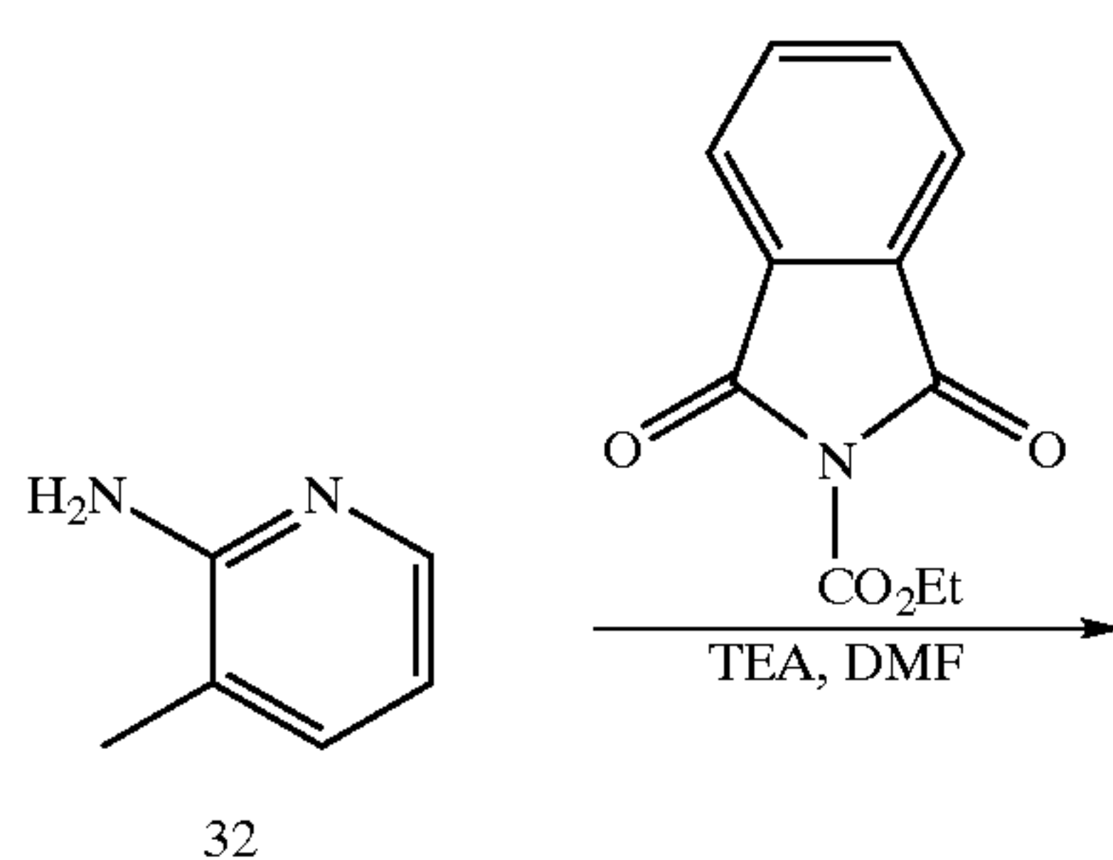
Scheme 10
