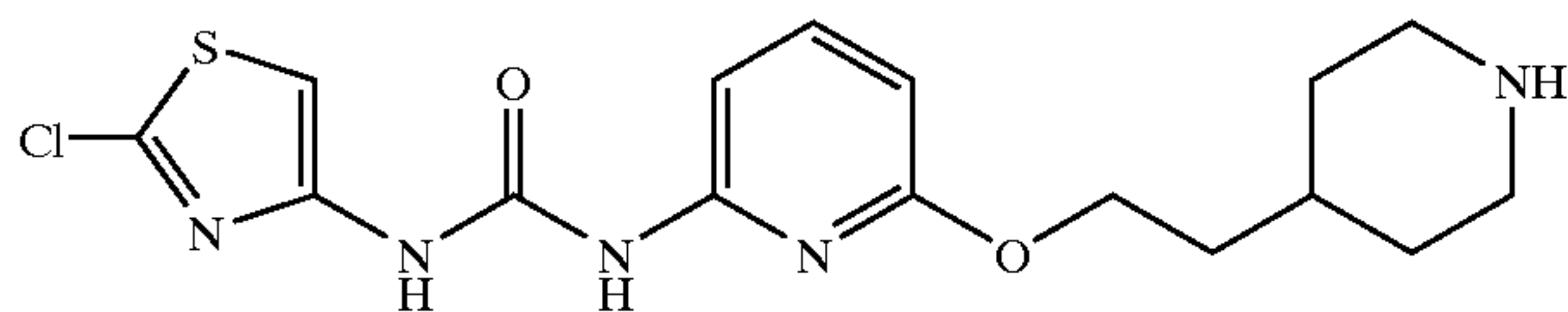
1-(2-Chloro-thiazol-4-yl)-3-[6-(2-piperidin-4-ylethoxy)-pyridin-2-yl]-urea
