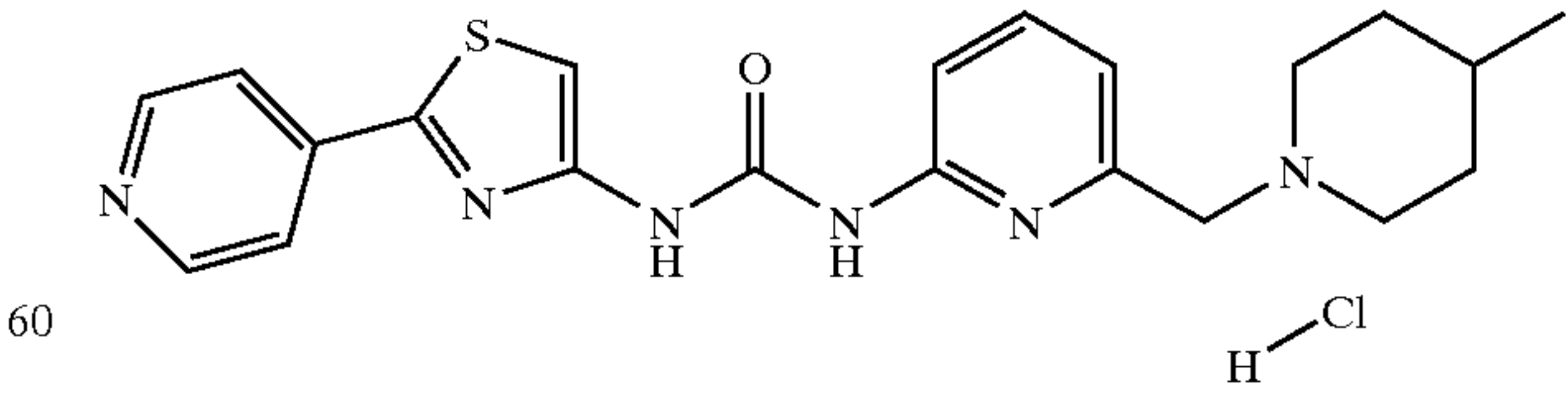
1-[6-(4-Methylpiperidin-1-ylmethyl)pyridin-2-yl]-3-(2-pyridin-4-yl-thiazol-4-yl)urea hydrochloride
