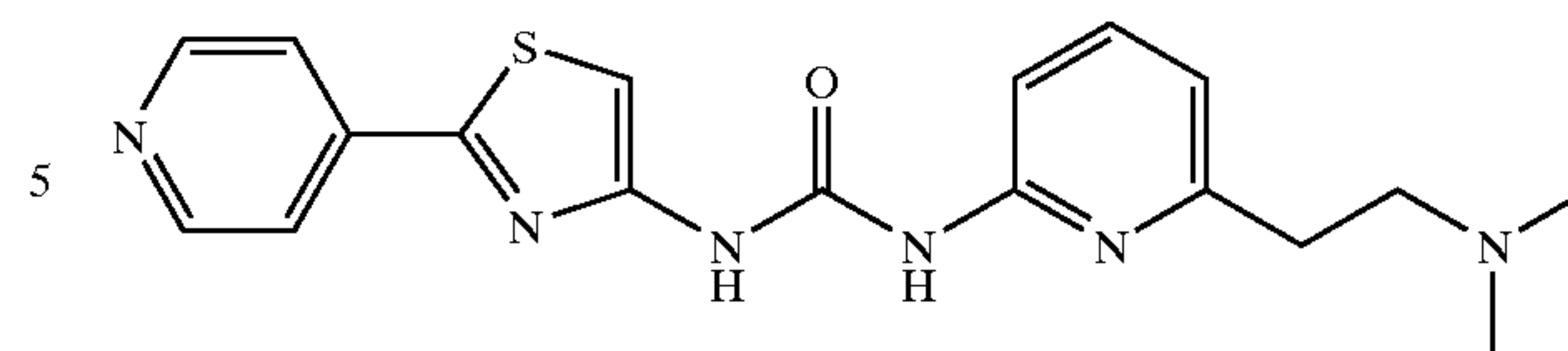
1-{6-[2-(N,N-Dimethylamino)ethyl]pyridin-2-yl}-3-(2-pyridin-4-yl-thiazol-4-yl)urea
