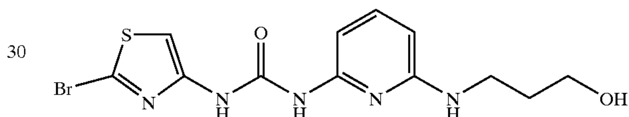
1-(2-Bromo-thiazol-4-yl)-3-[6(3-hydroxy-propylamino)-pyridin-2-yl]-urea
