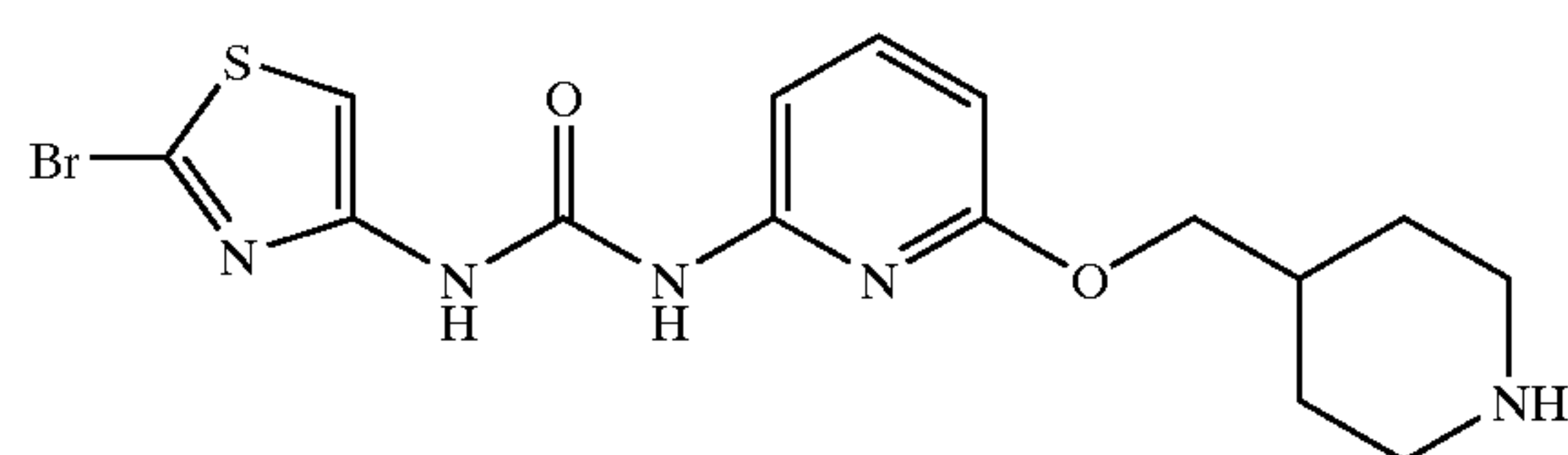
1-(2-Bromo-thiazol-4-yl)-3-[6-(piperidin-4-ylmethoxy)-pyridin-2-yl]-urea
