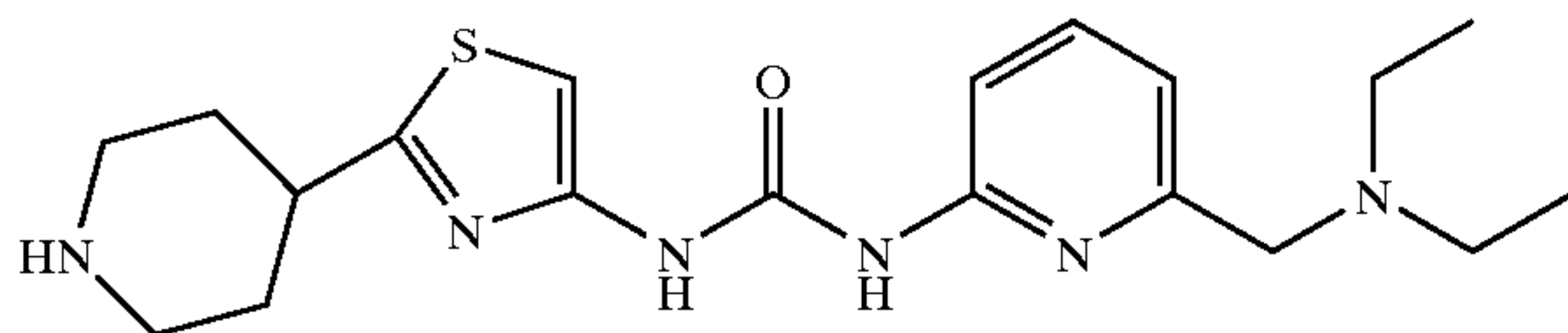
1-(6-Diethylaminomethyl-pyridin-2-yl)-3-(2-piperidin-4-yl-thiazol-4-yl)urea
