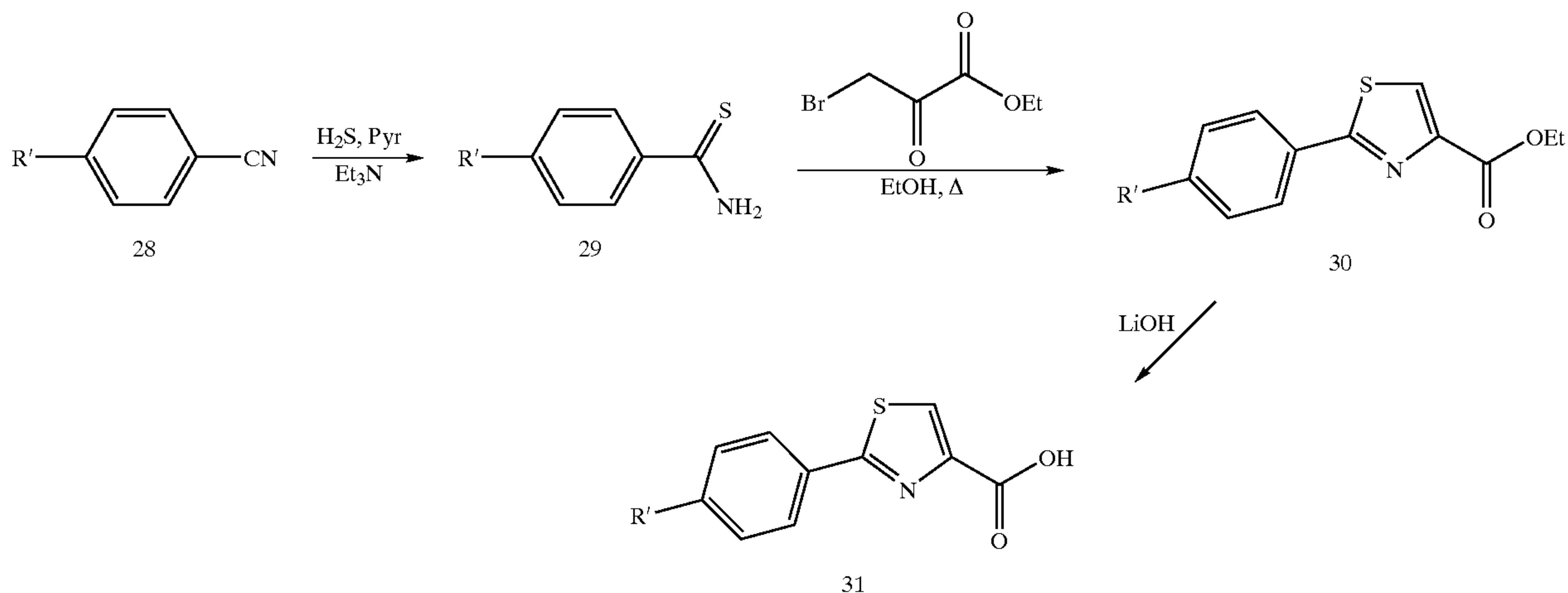
Scheme 9
