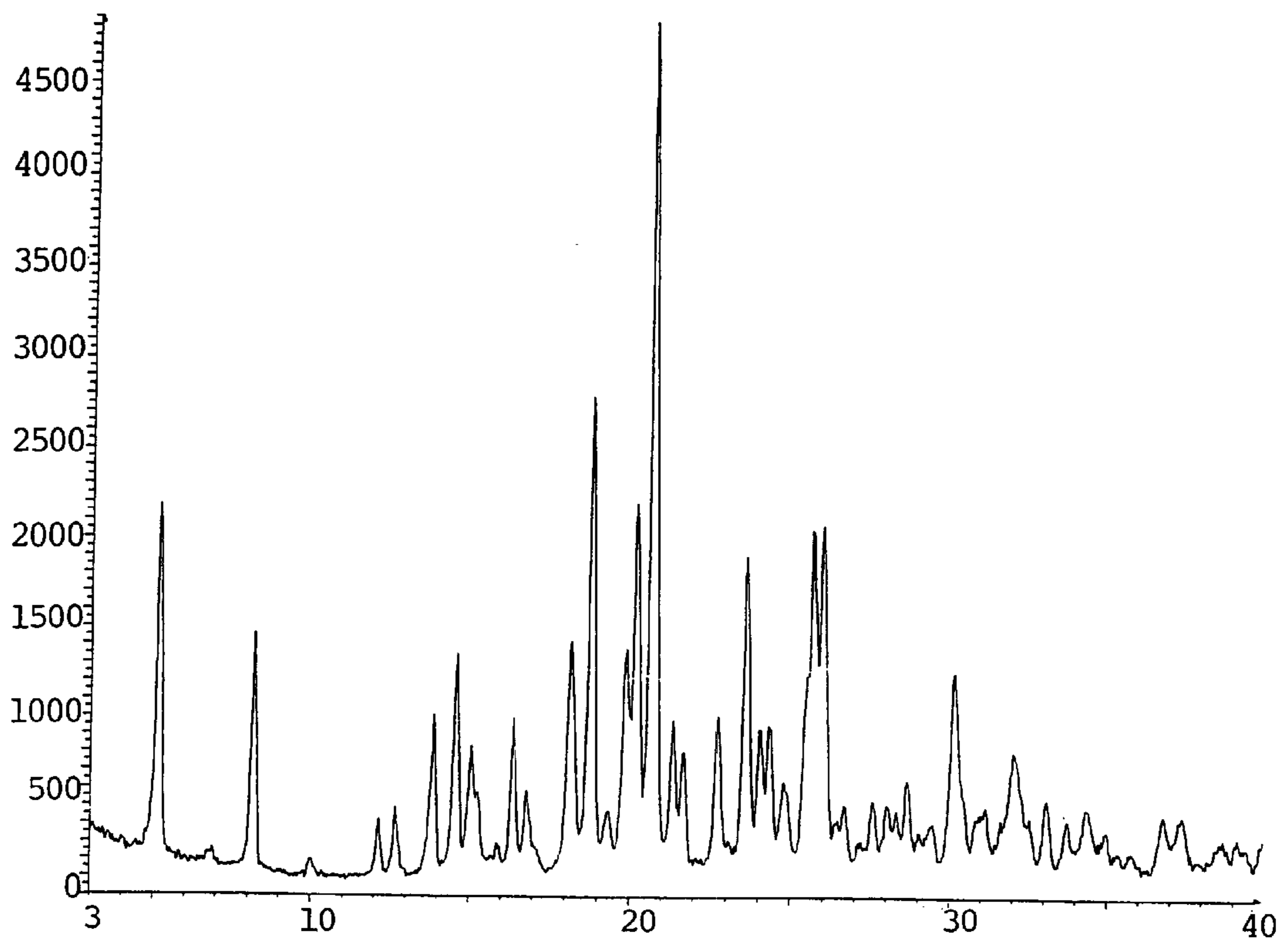
2-Theta - Scale
