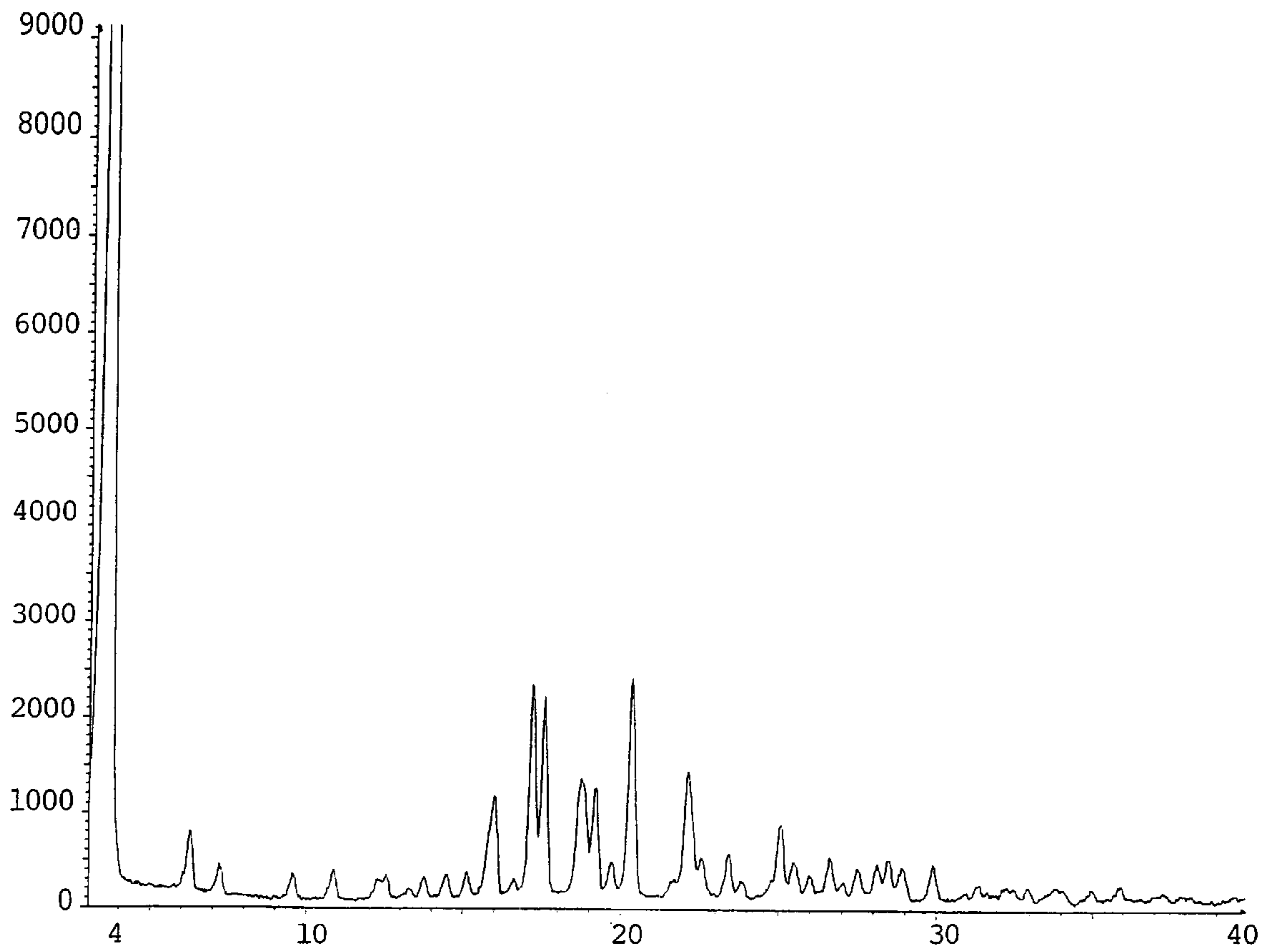
2-Theta - Scale
