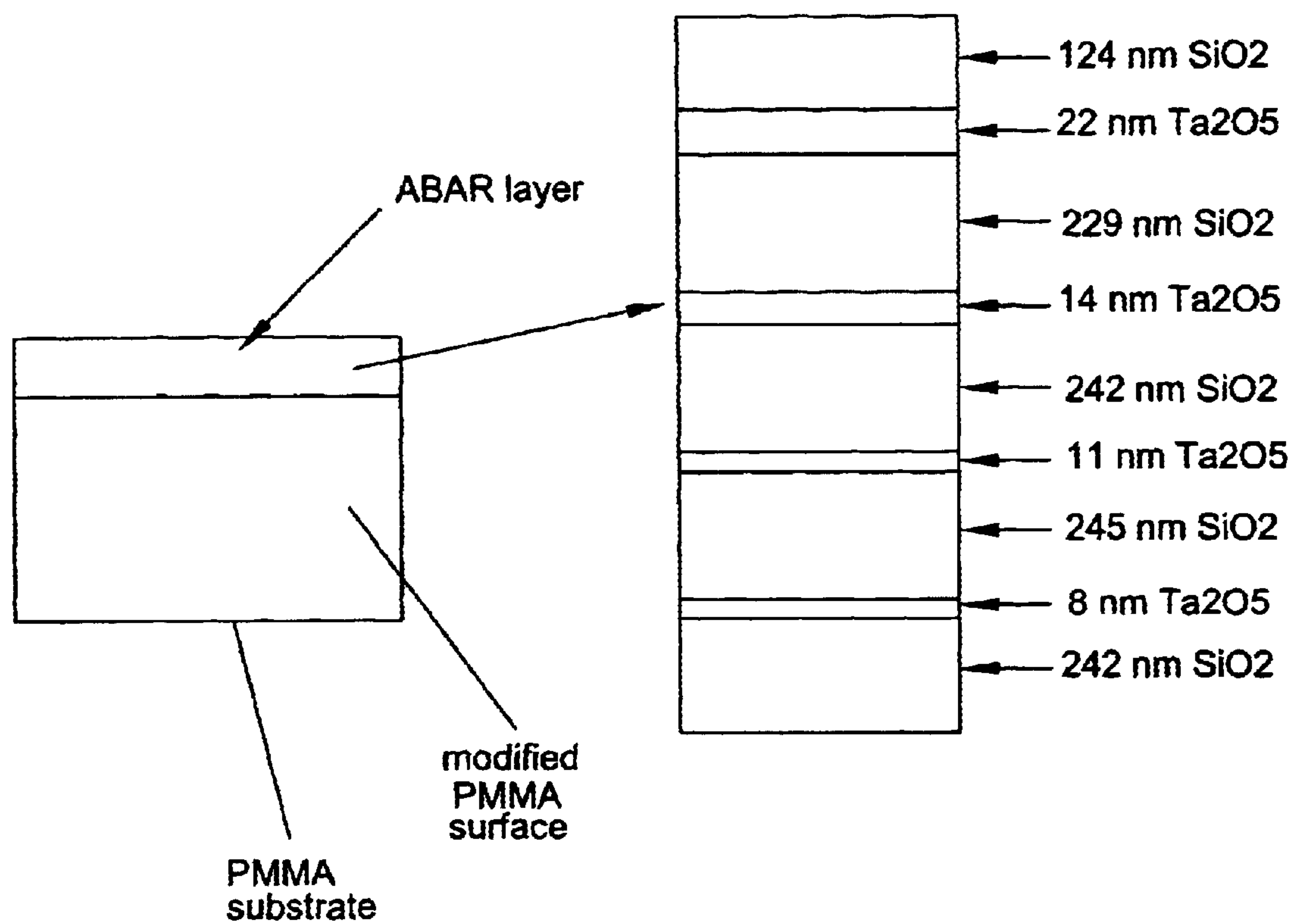
Diagrammatic structure of an abrasionproof anti_reflex layer system on PMMA (total layer thickness appr. 1.1 μm)
