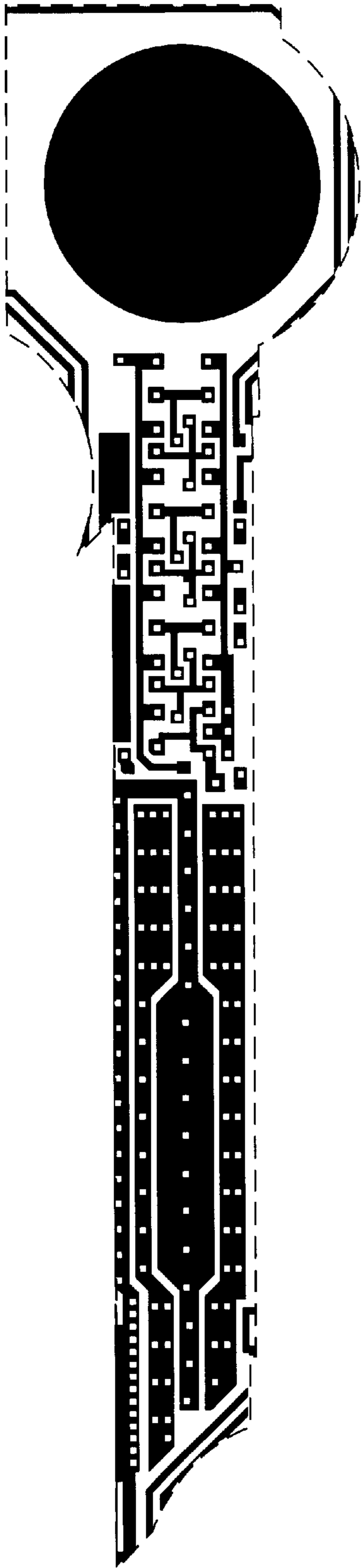
Metal 1 mask
