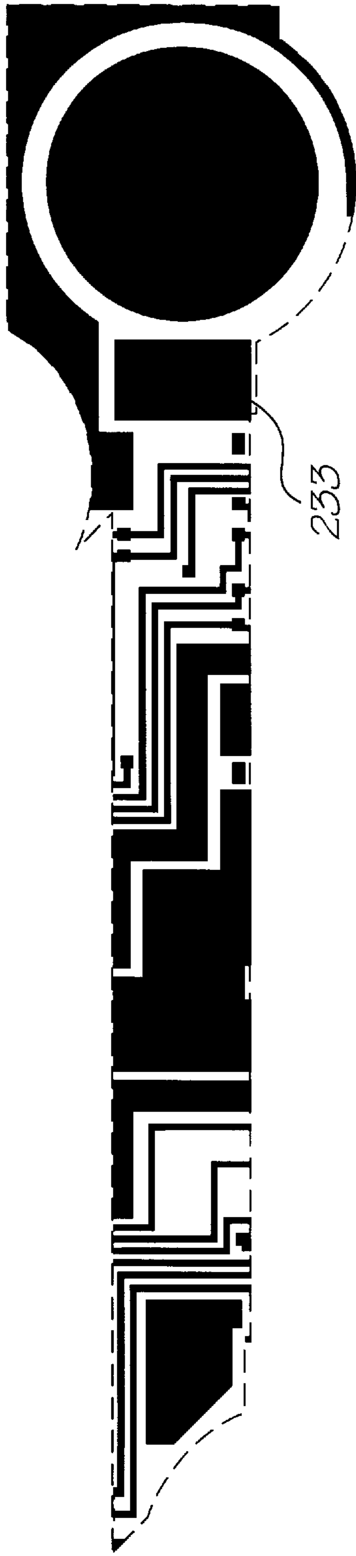
Metal 2 mask
