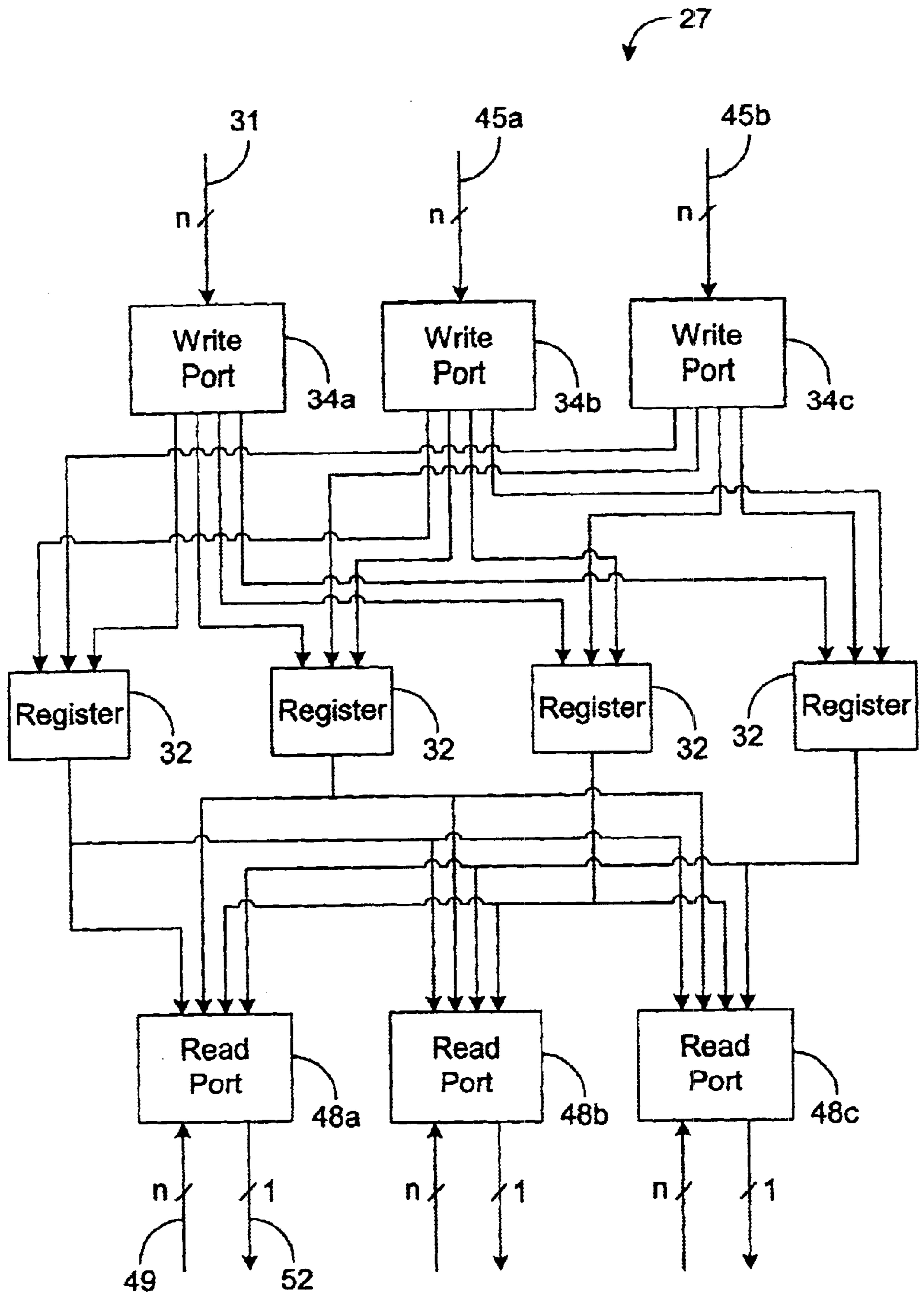
FIG. 2 (Prior Art)
