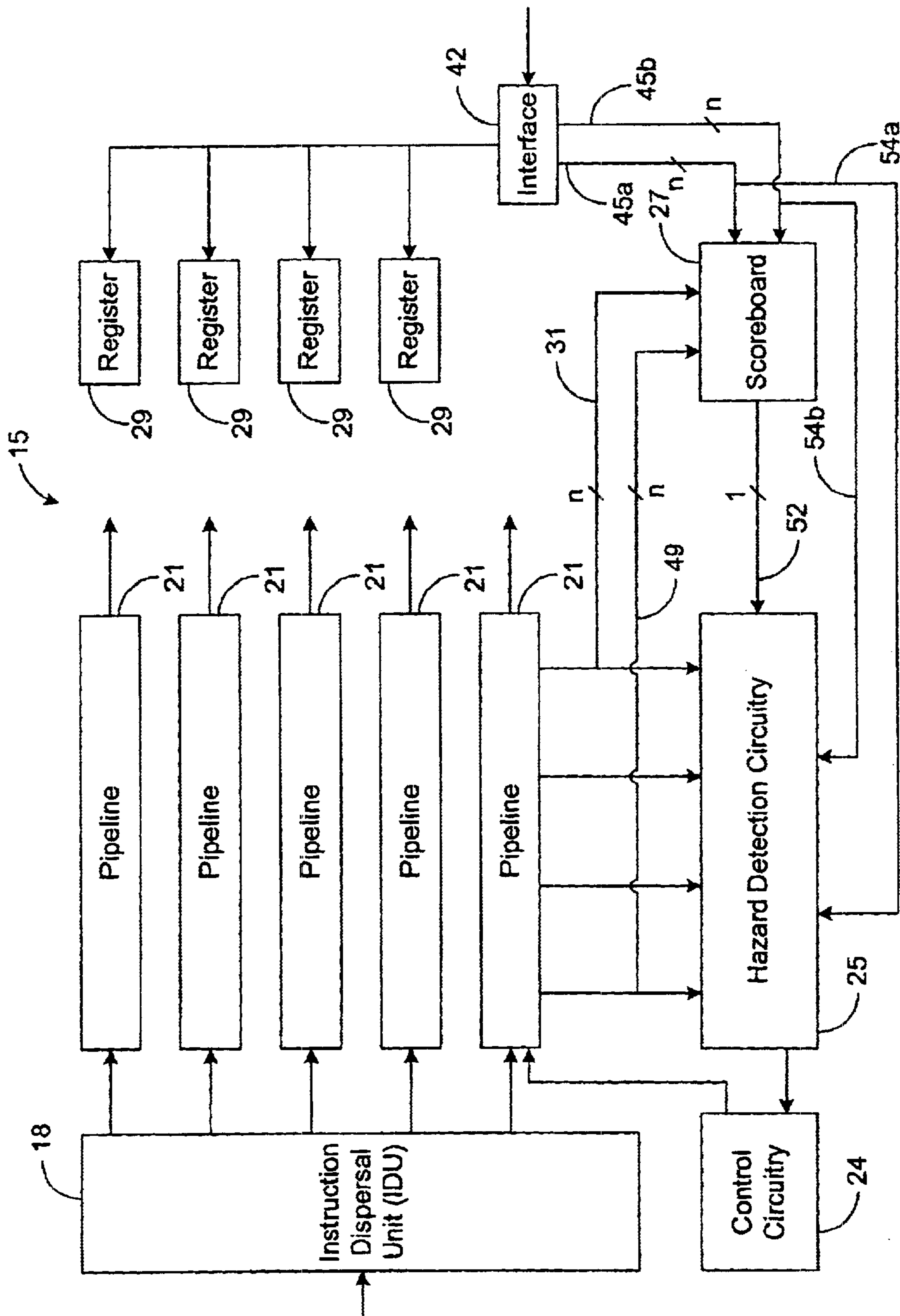
FIG. 1 (Prior Art)
