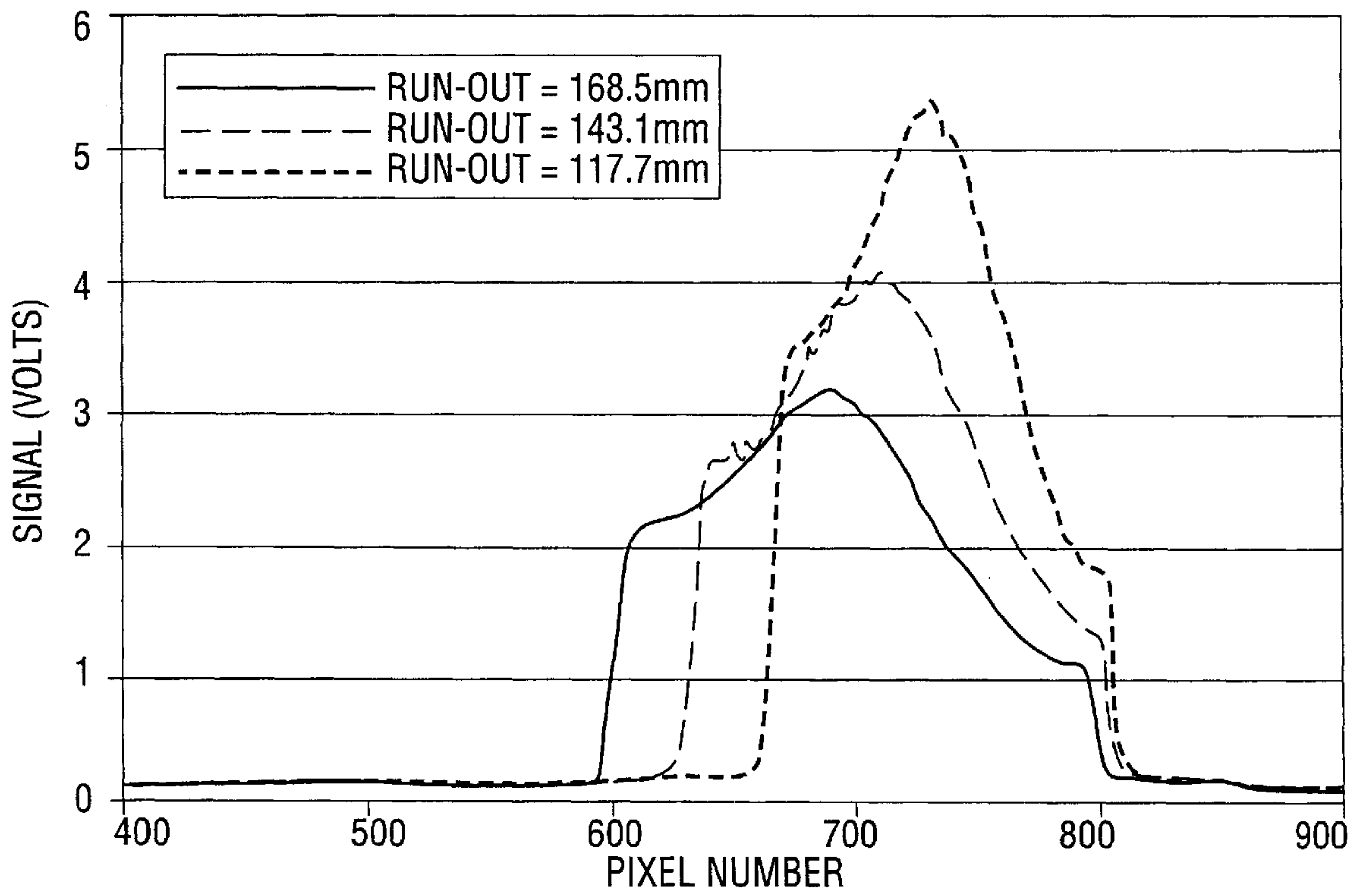
INCIDENT BEAM PROFILES AT DIFFERENT RUN-OUT DISTANCES
