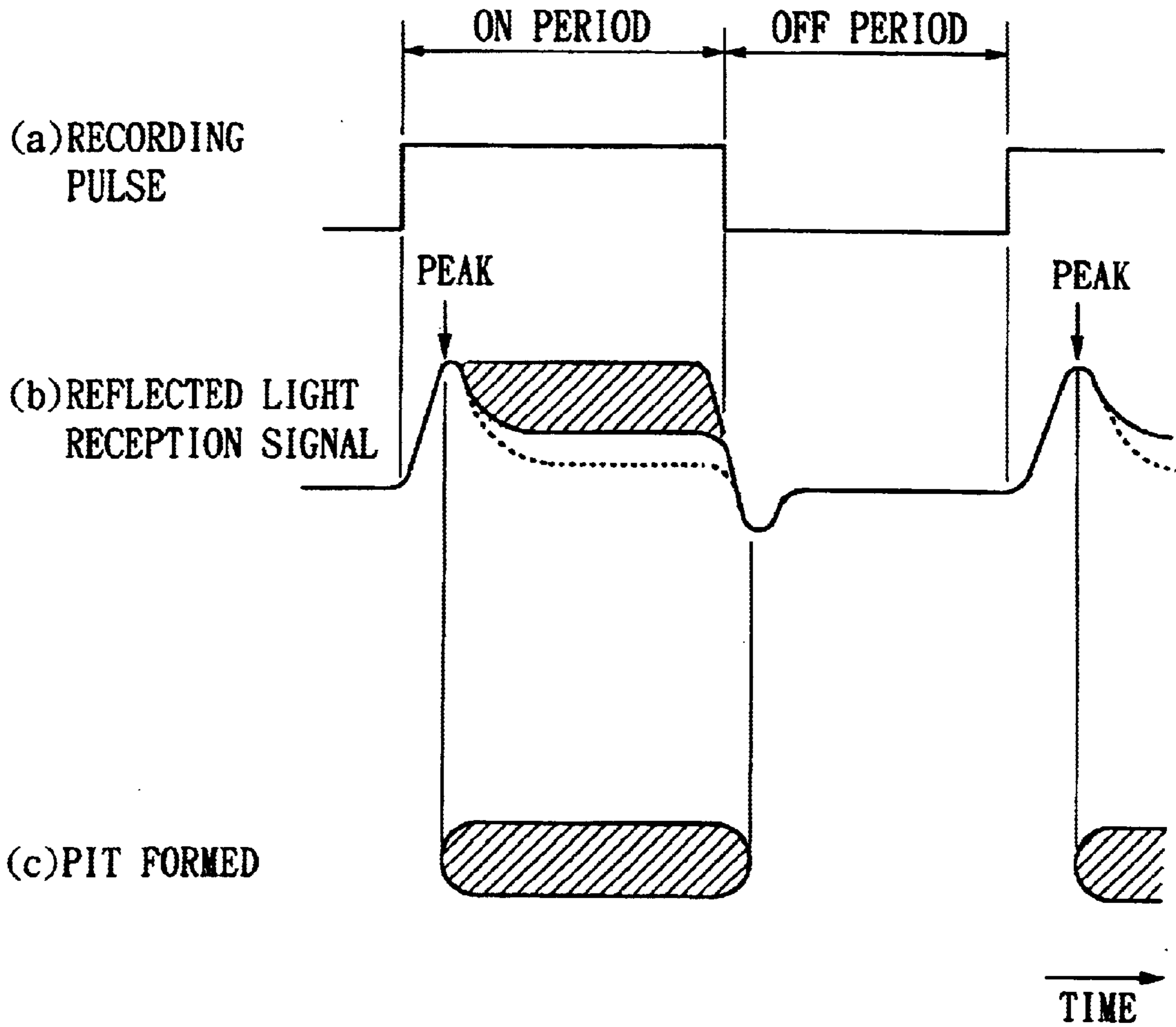
FIG. 4 PRIOR ART
