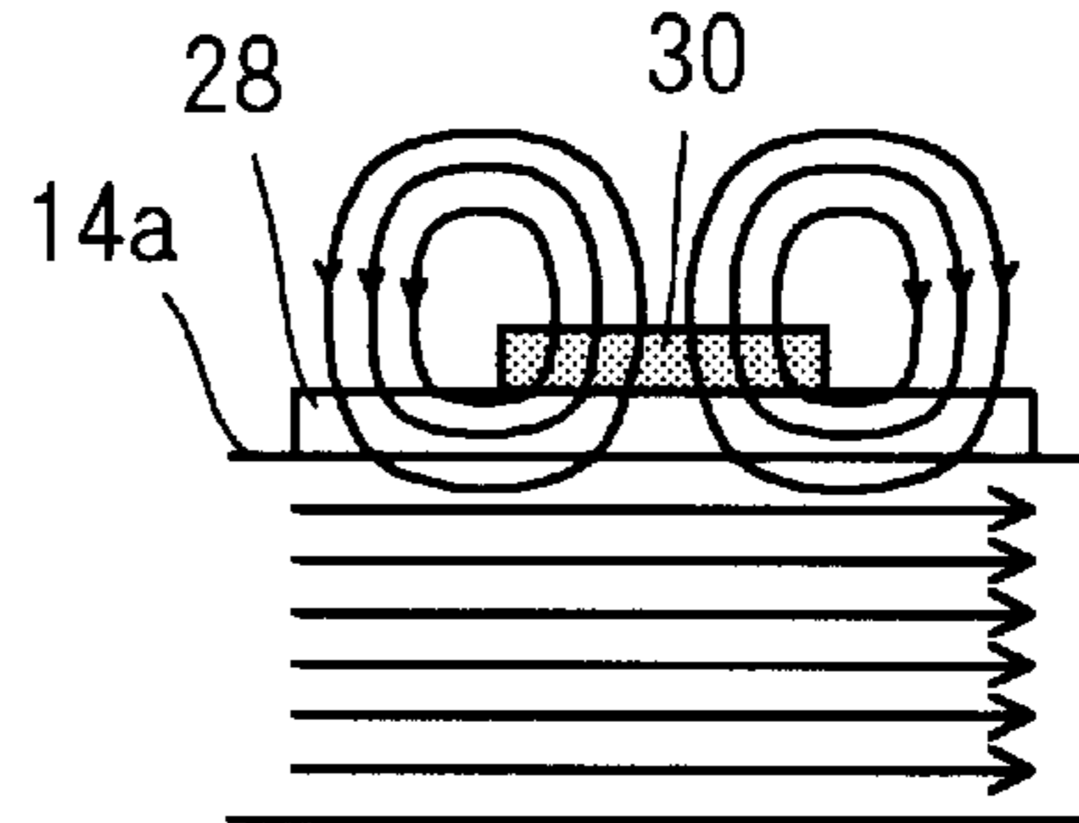
Shielding Magnet and Nonmagnetic Spacer FIG. 8 D
