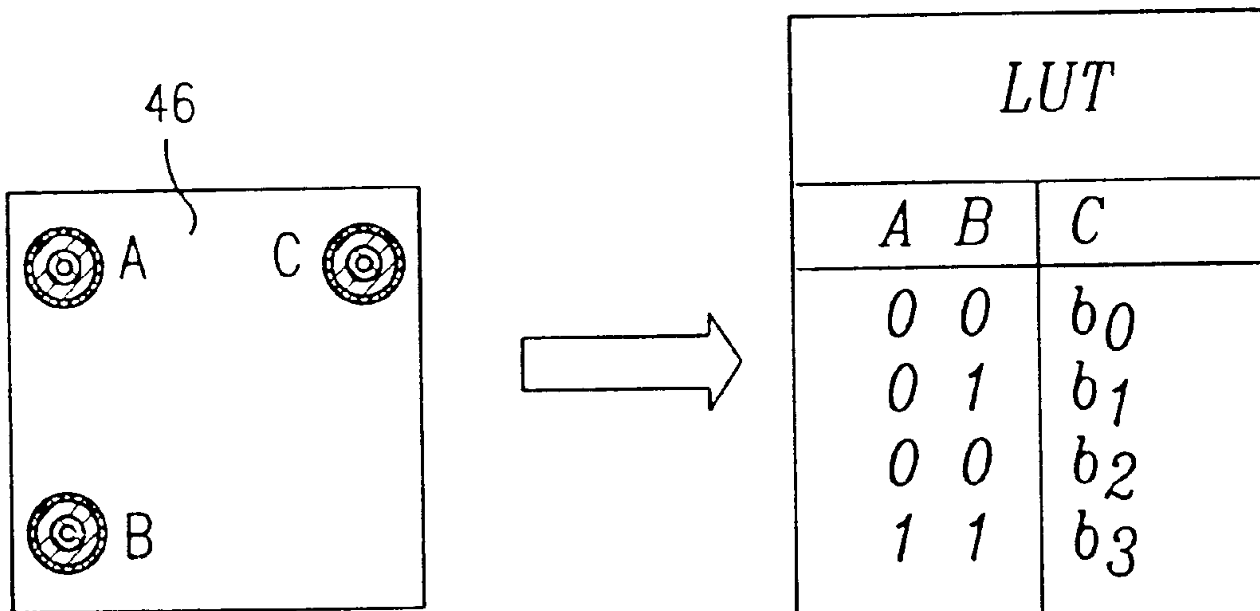
LOOK UP TABLE 2 INPUTS 1 OUTPUT
