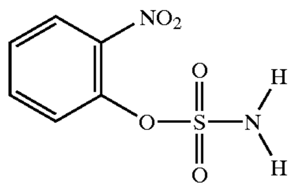
2-Nitrophenol-O-sulfamate(9c)
