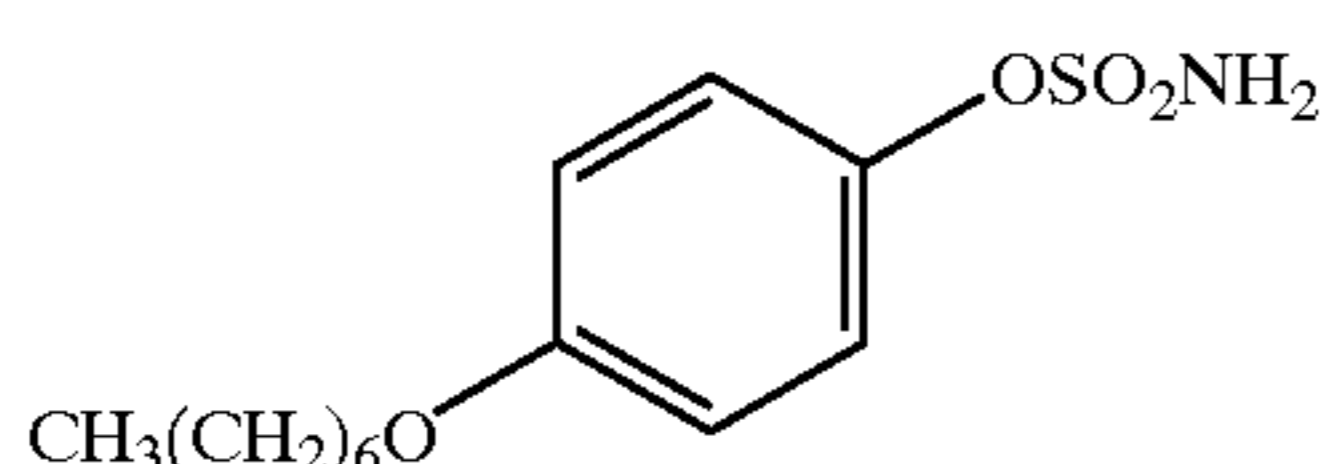
4-n-Heptyl phenyl-O-sulphamate (9a)
