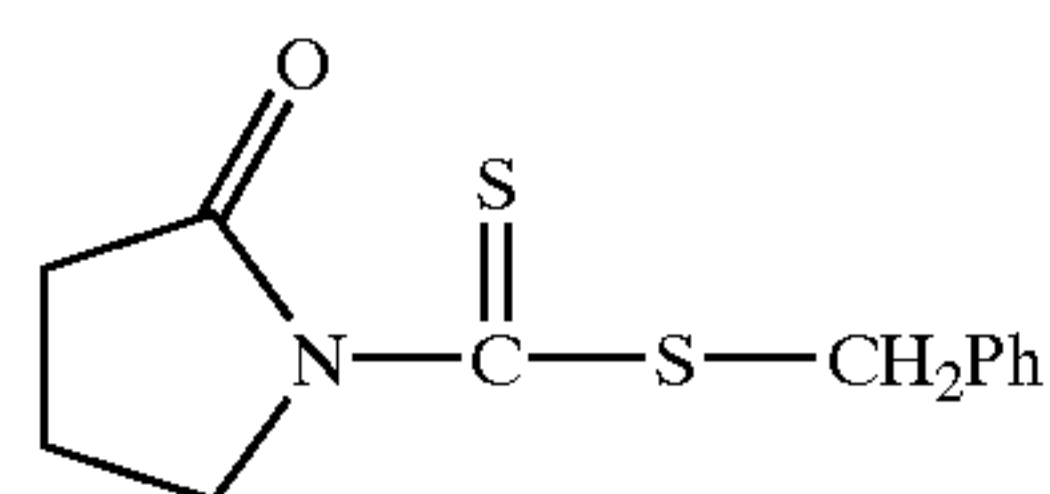
D = D2, R = benzyl; E = E1 = 1-(pyrrolidin-2-onyl)
