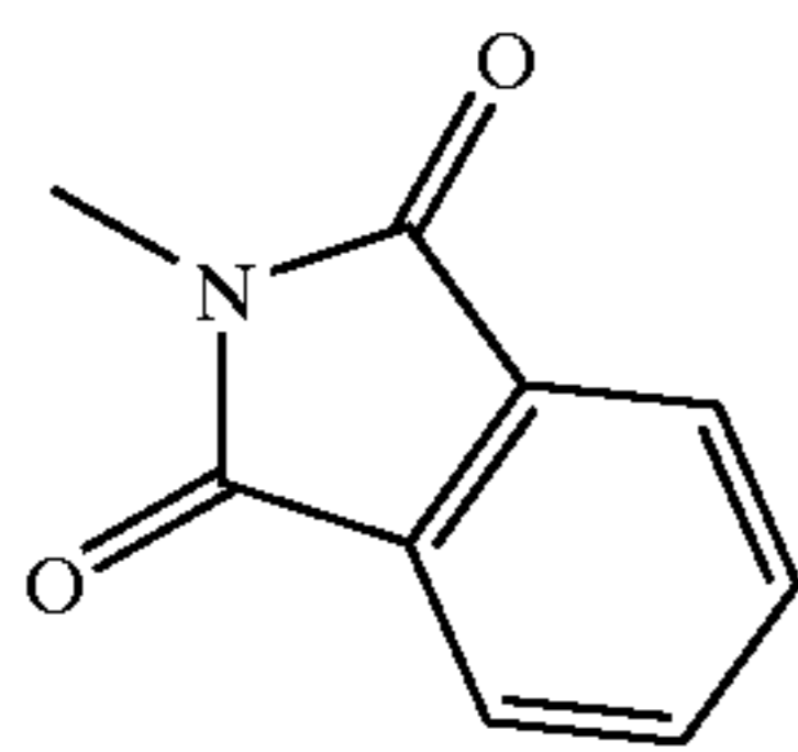
phthalimides
