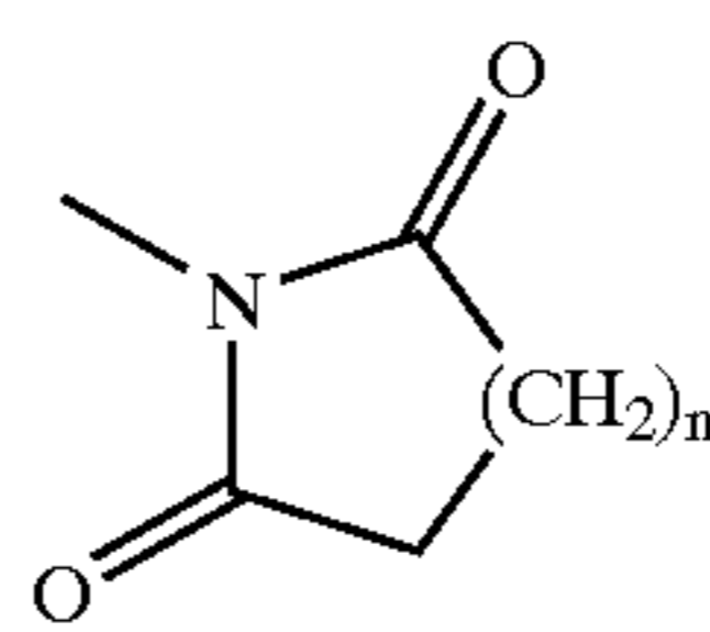
imide
