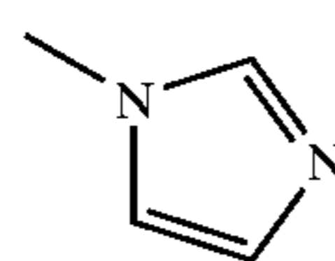
imidazoles
