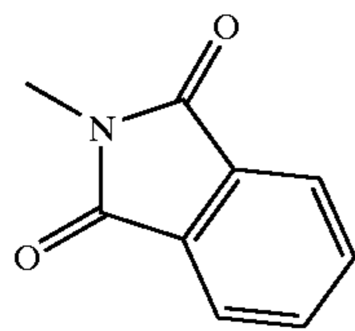
phthalimides
