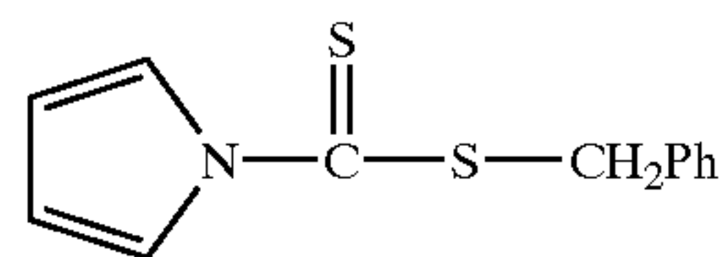
D = D2, R = benzyl; E = E1 = 1-pyrrolyl
