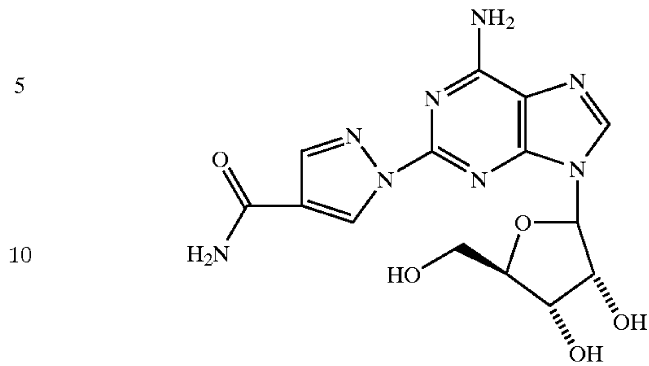
1-{9-[(4S,2R,3R,5R)-3,4-dihydroxy-5-(hydroxymethyl)oxolan-2-yl]-6-aminopurin-2-yl}pyrazole-4-carboxamide (20)
