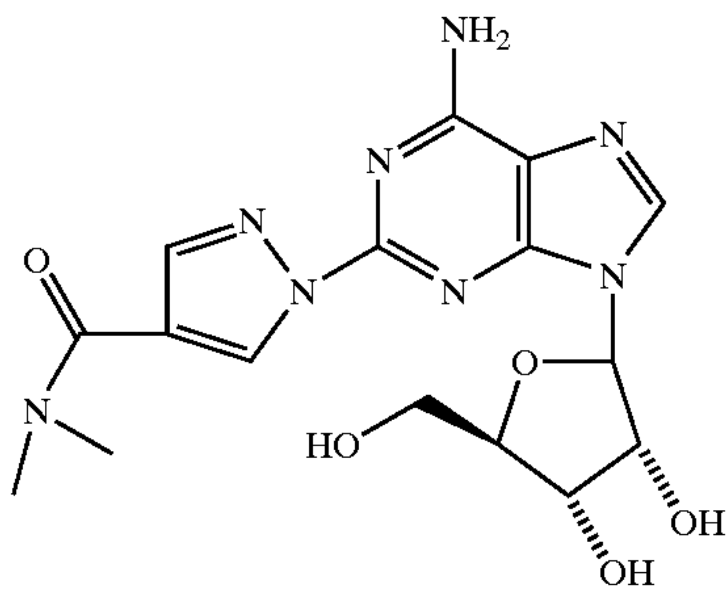
(1-{9-[(4S,2R,3R,5R)-3,4-dihydroxy-5-(hydroxymethyl)oxolan-2-yl]-6-aminopurin-2-yl}pyrazol-4-yl)-N,N-dimethylcarboxamide (18)
