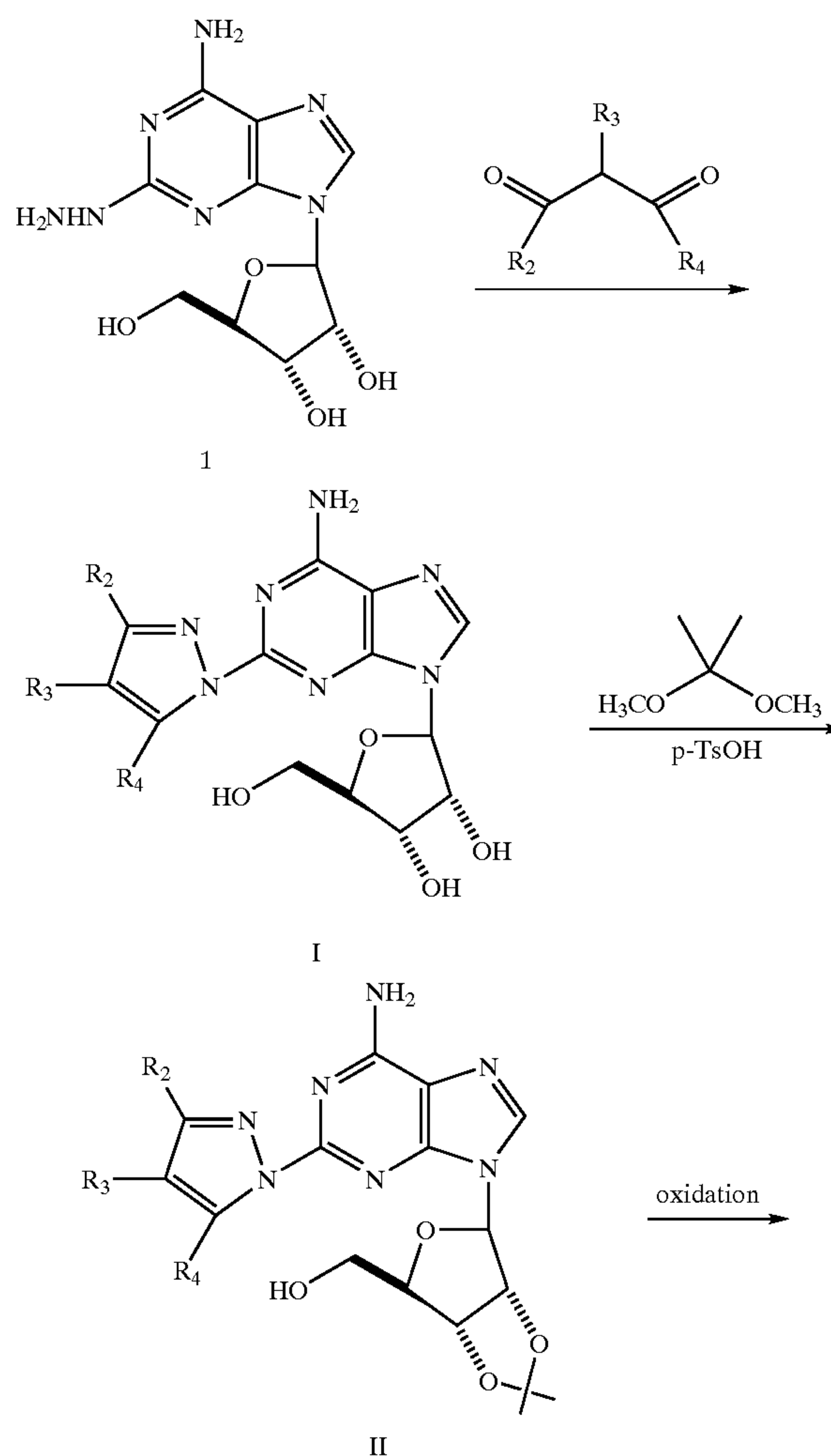
Scheme 1.
