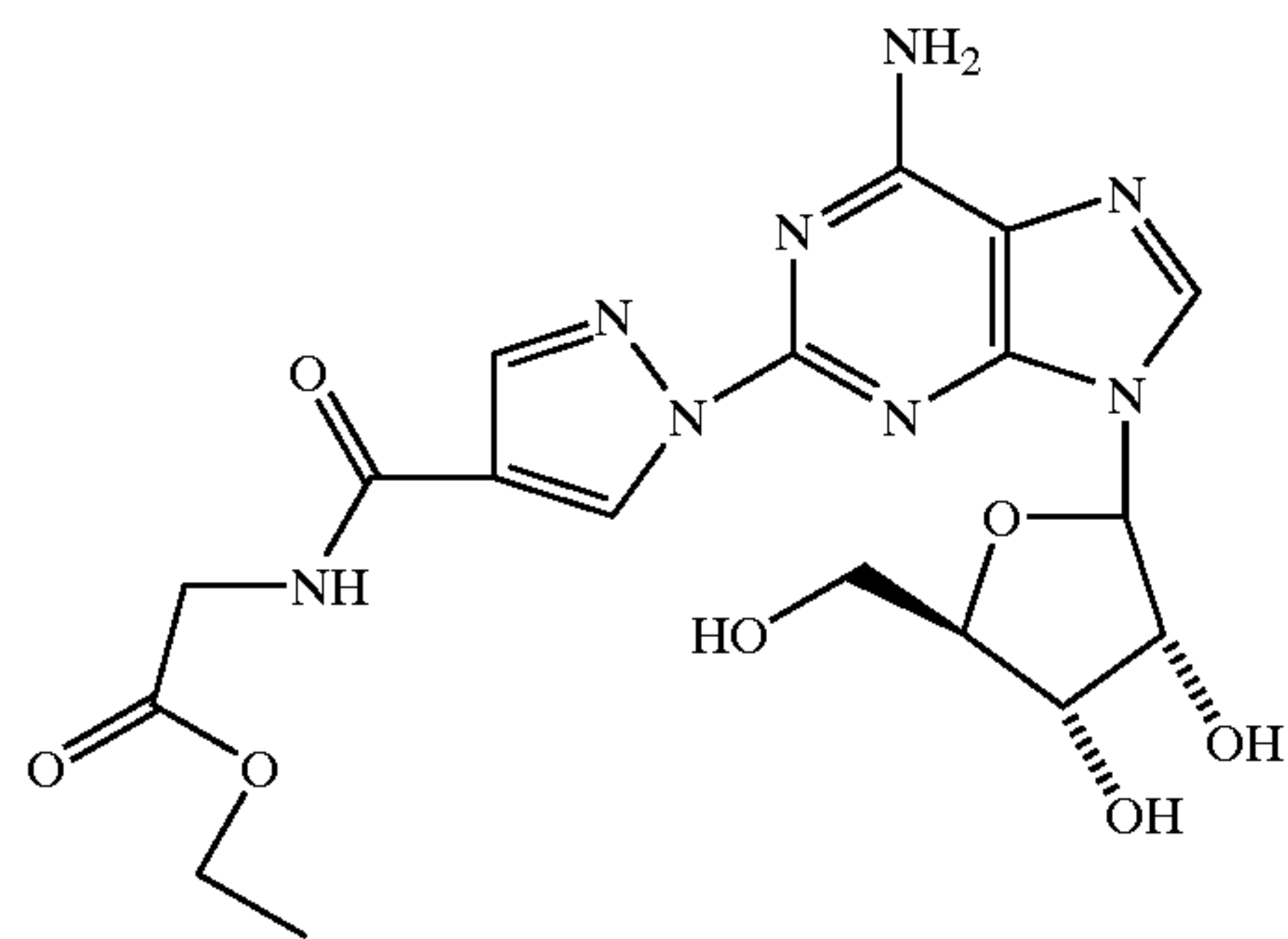
Ethyl 2-[(1-{9-[(4S,2R,3R,5R)-3,4-dihydroxy-5-(hydroxymethyl)oxolan-2-yl]-6-aminopurin-2-yl}pyrazol-4-yl)carbonylaminolacetate (23)
