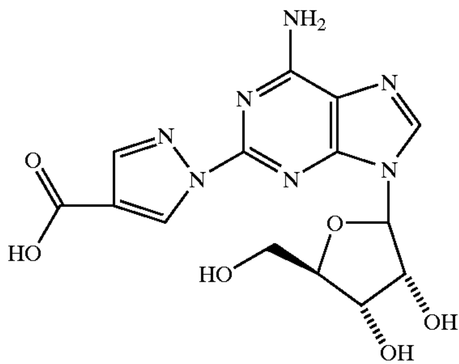
1-{9-[(4S,2R,3R,5R)-3,4-dihydroxy-5-(hydroxymethyl)oxolan-2-yl]-6-aminopurin-2-yl}pyrazole-4-carboxylic Acid (17)
