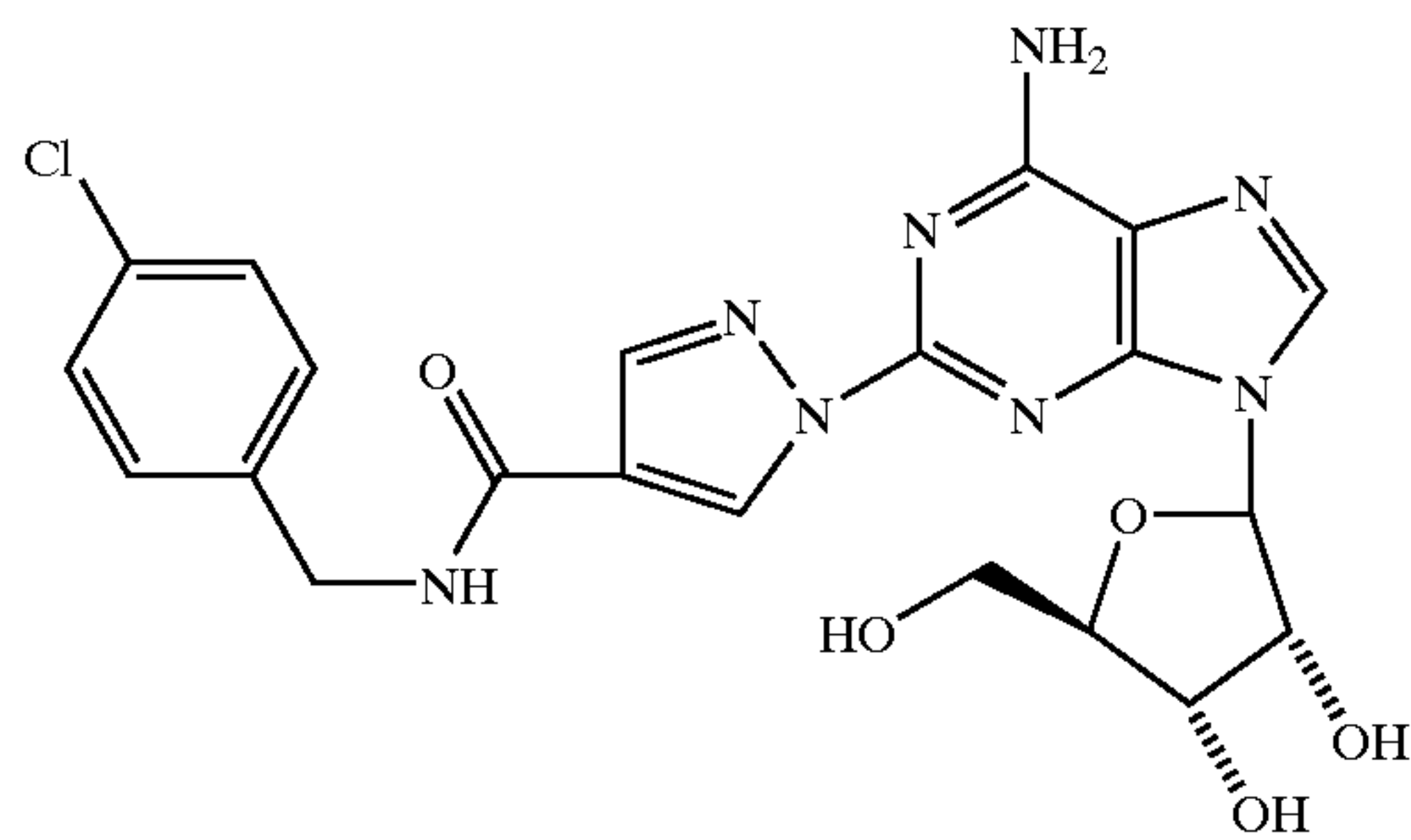
(1-{9-[(4S,2R,3R,5R)-3,4-dihydroxy-5-(hydroxymethyl)oxolan-2-yl]-6-aminopurin-2yl}pyrazol-4-yl)-N-[(4-chlorophenyl)methyl]carboxamide (22)
