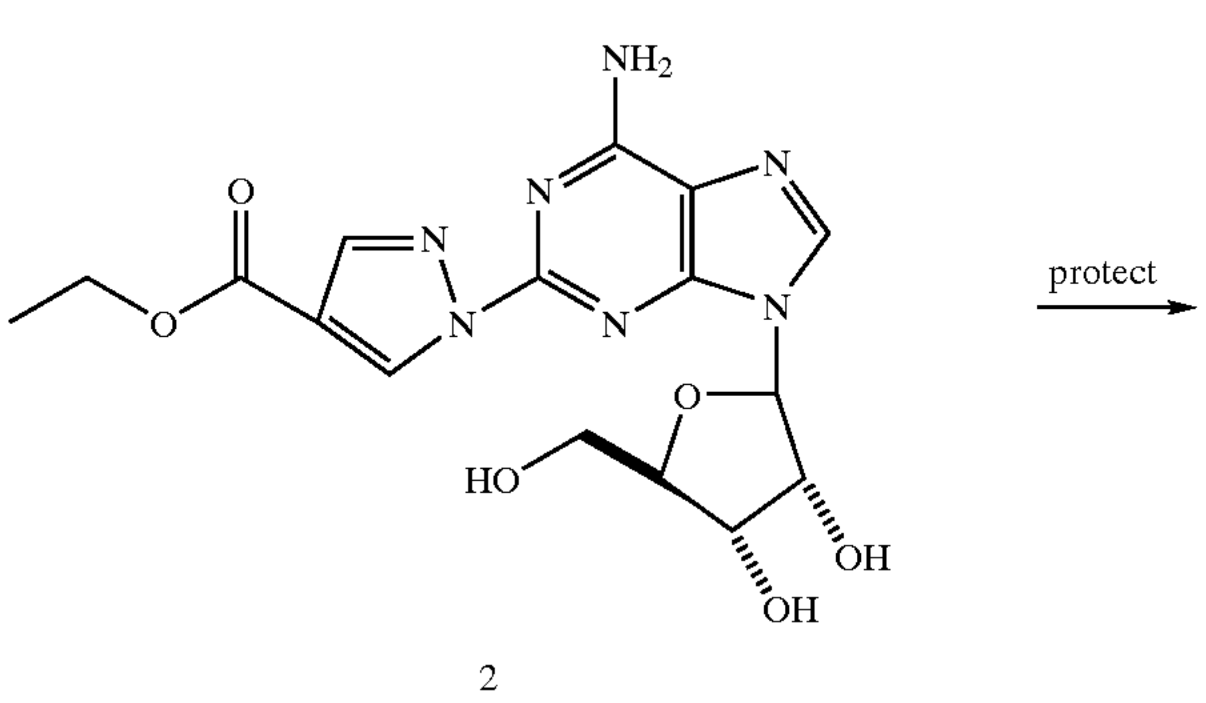
Scheme 2.
