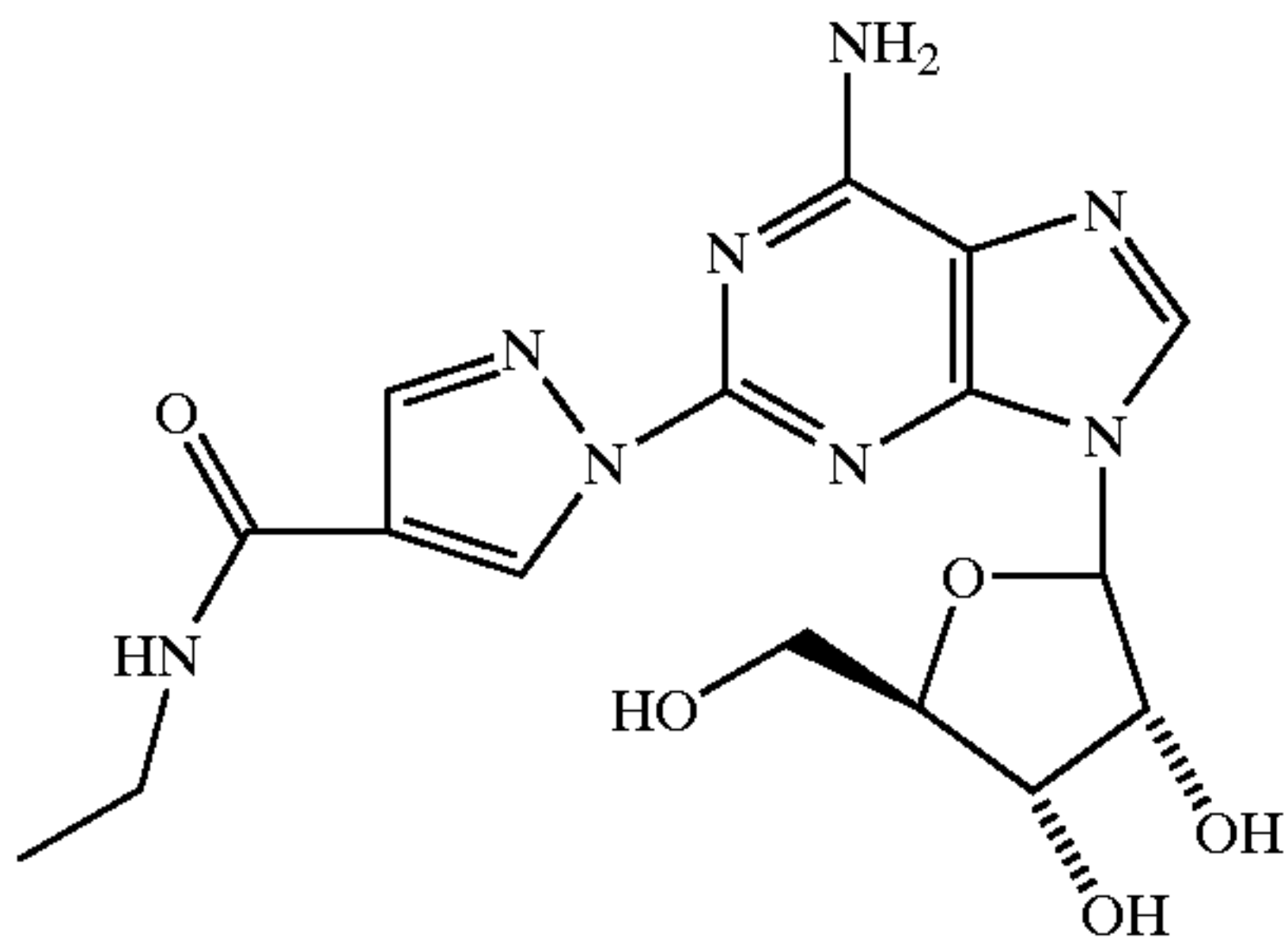
(1-{9-[(4S,2R,3R,5R)-3,4-dihydroxy-5-(hydroxymethyl)oxolan-2-yl]-6-aminopurin-2-yl}pyrazol-4-yl)-N-ethylcarboxamide (19)
