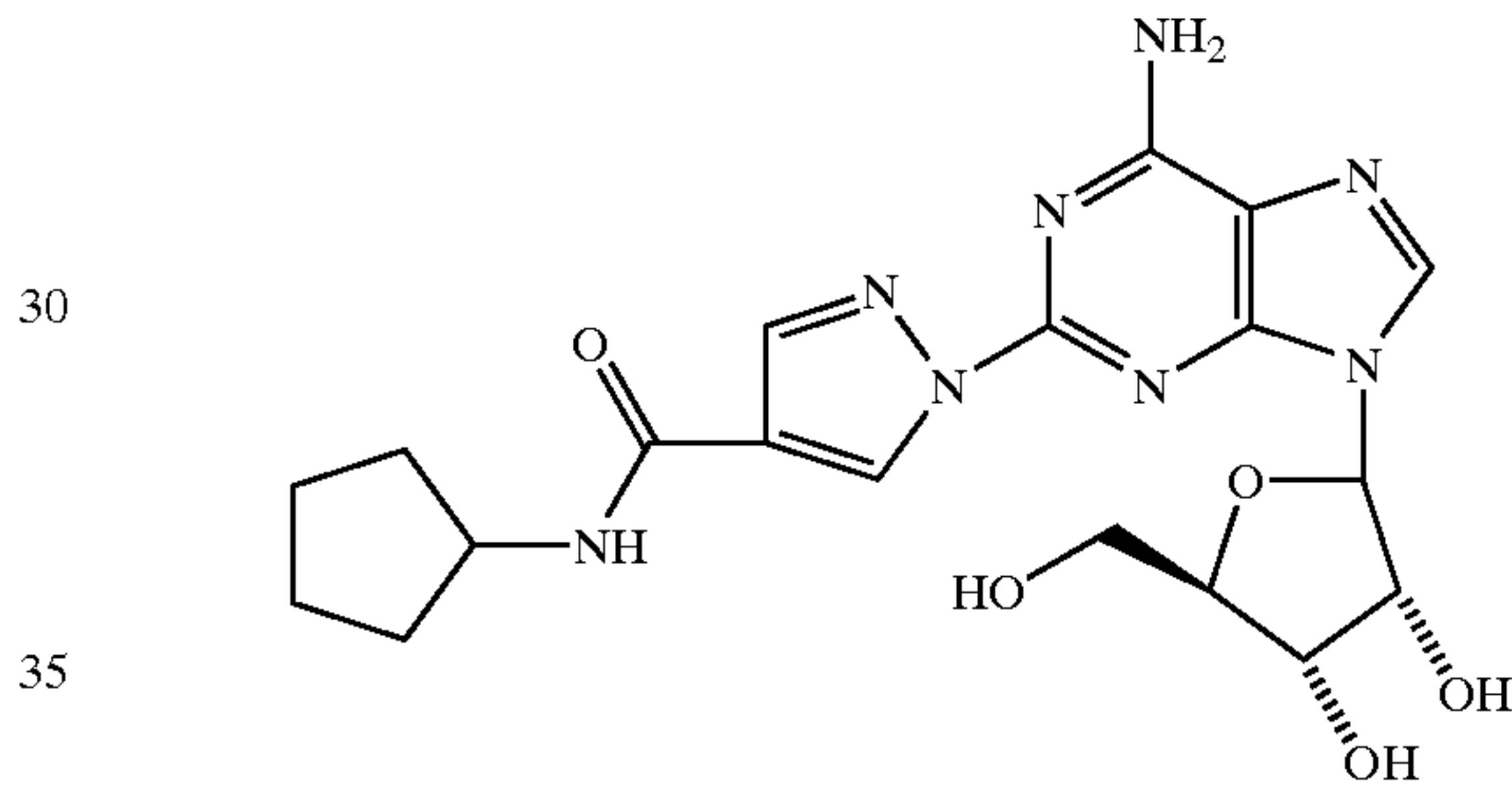
(1-{9-[(4S,2R,3R,5R)-3,4-dihydroxy-5-(hydroxymethyl)oxolan-2-yl]-6-aminopurin-2-yl}pyrazol-4-yl)-N-(cyclopentyl)carboxamide (21)
