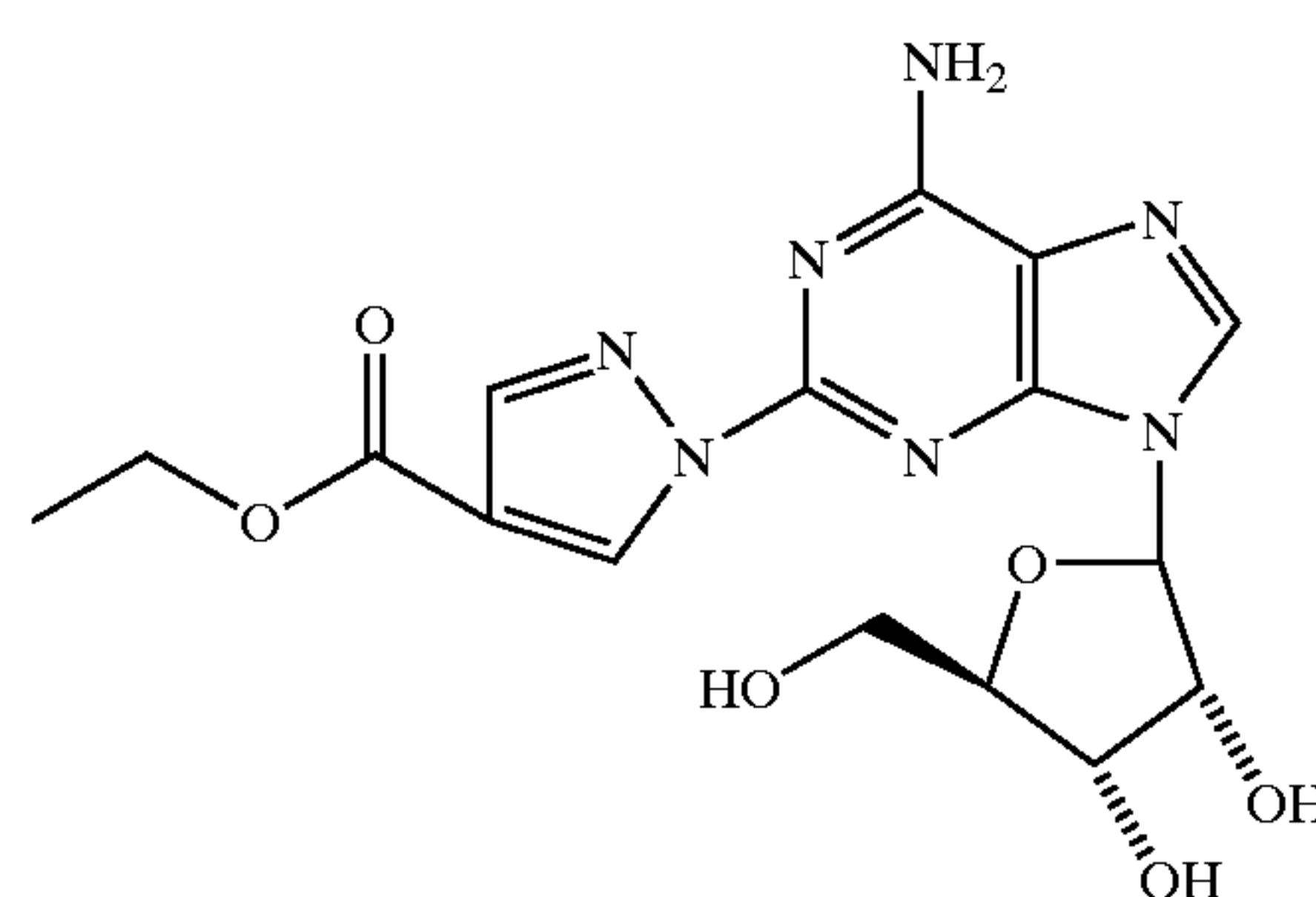
Ethyl 1-[9-[(4S,2R,3R,5R)-3,4-dihydroxy-5-(hydroxymethyl)oxolan-2-yl]-6-aminopurin-2-yl]pyrazole-4-carboxylate (12)
