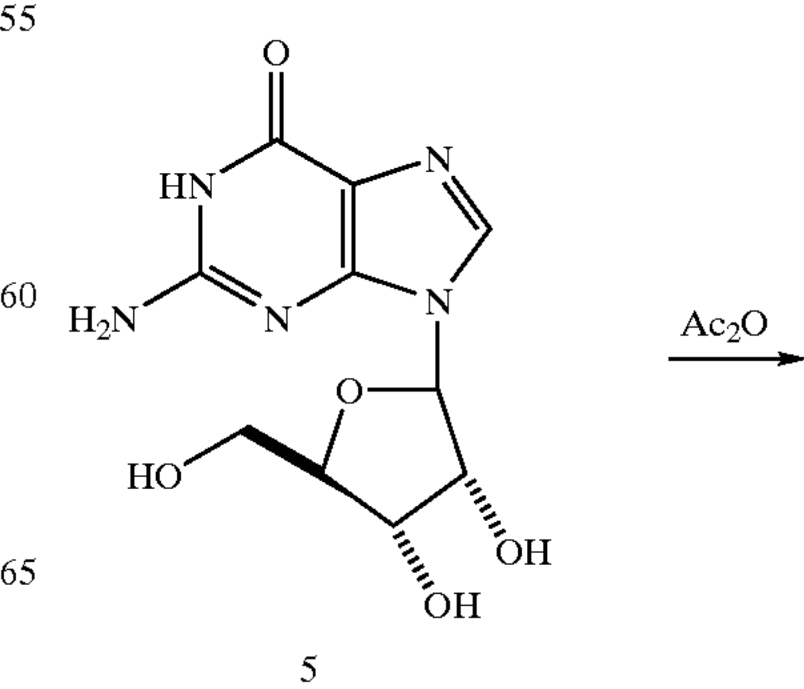
Scheme 3
