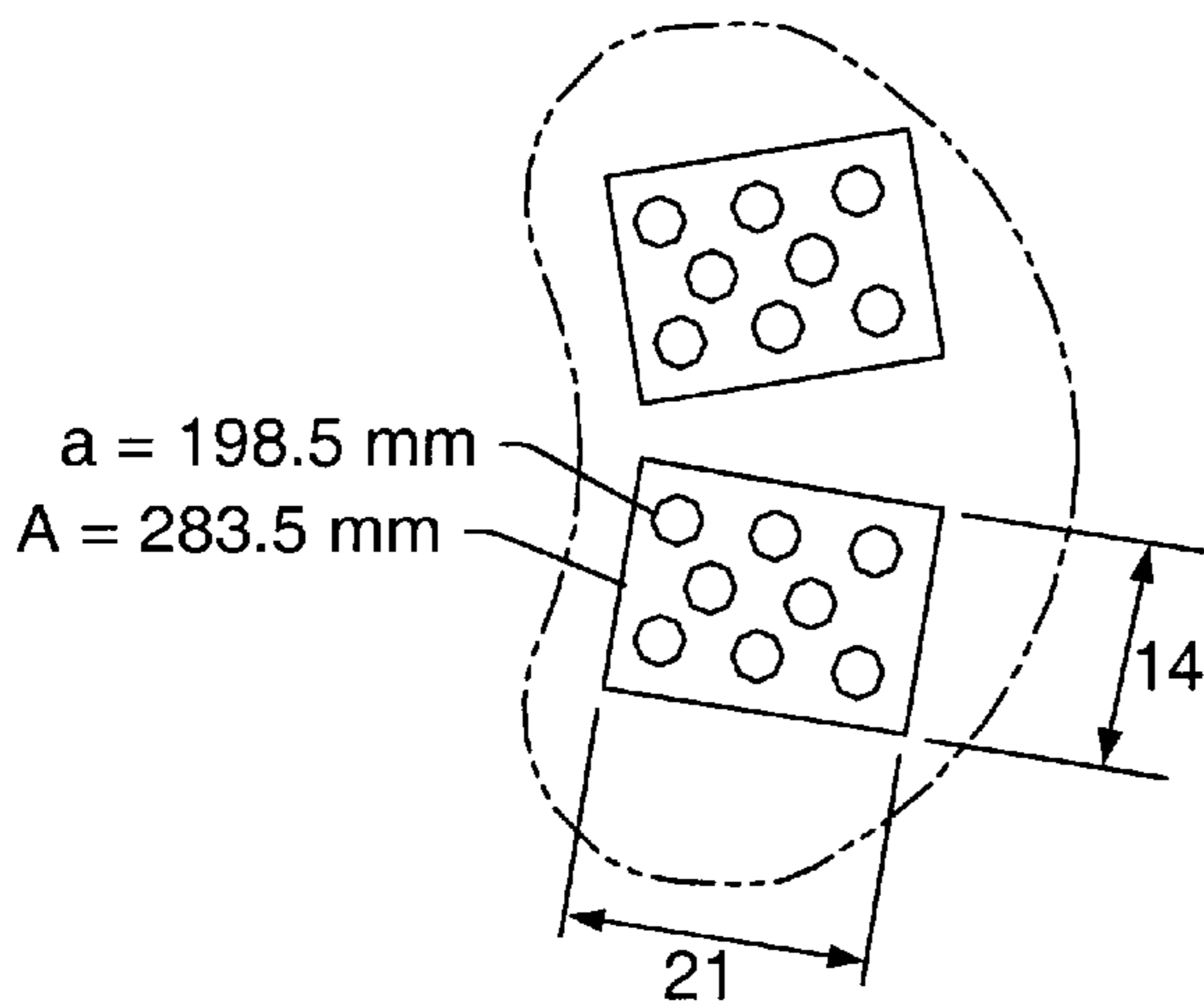
FIG. 22 (PRIOR ART)
