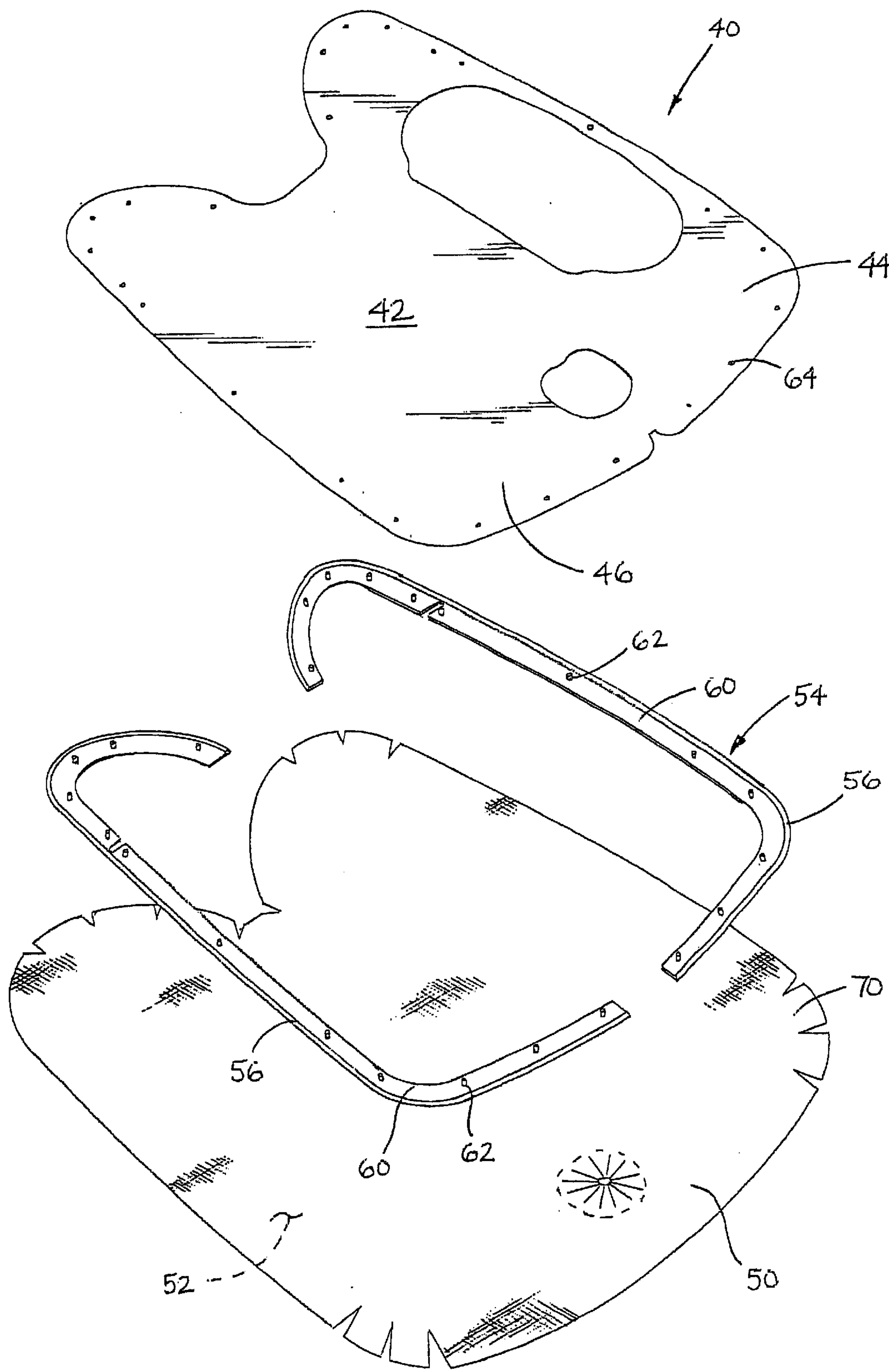
FIG. 1 PRIOR ART
