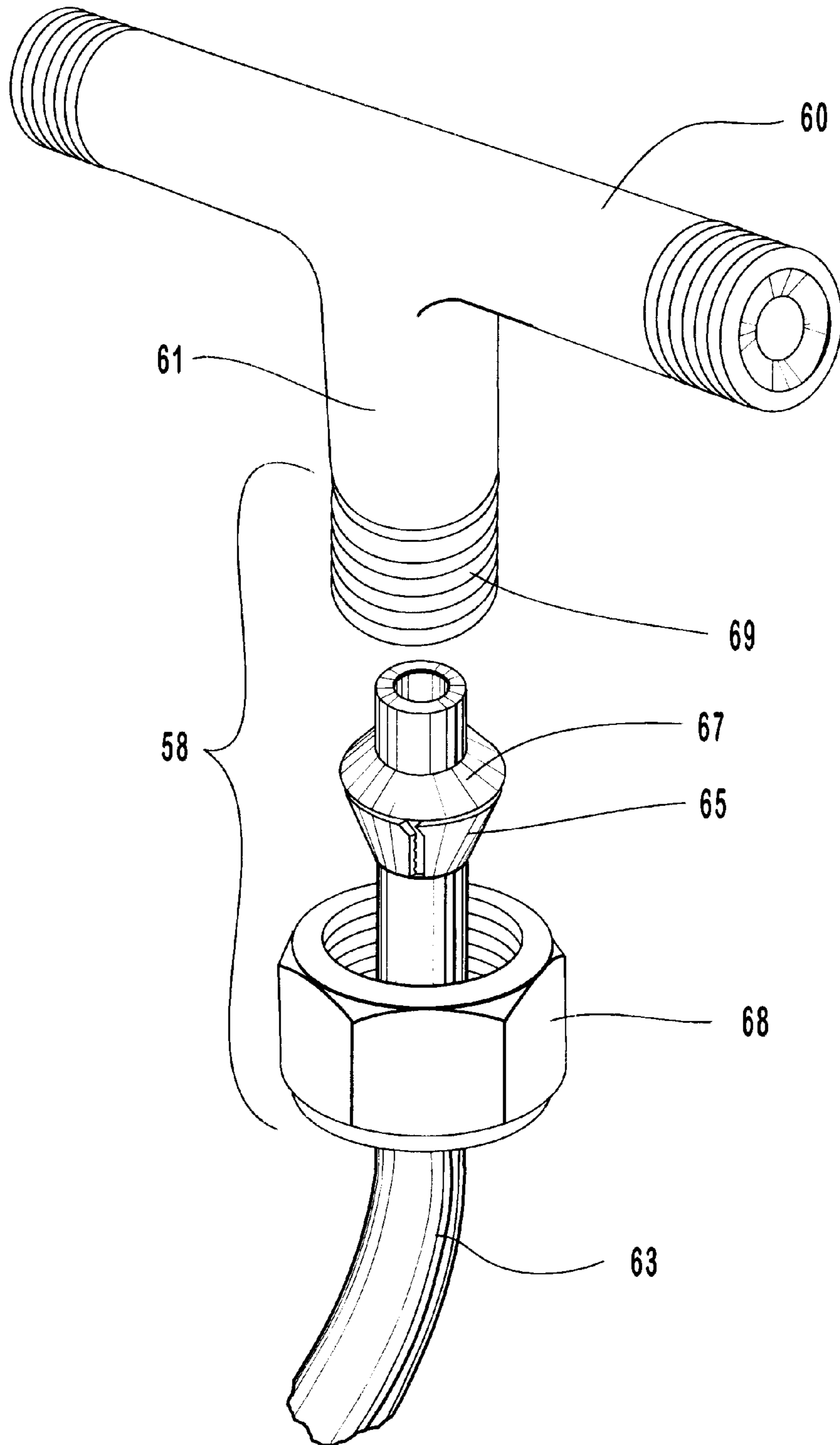
FIG. 2 ( PRIOR ART )
