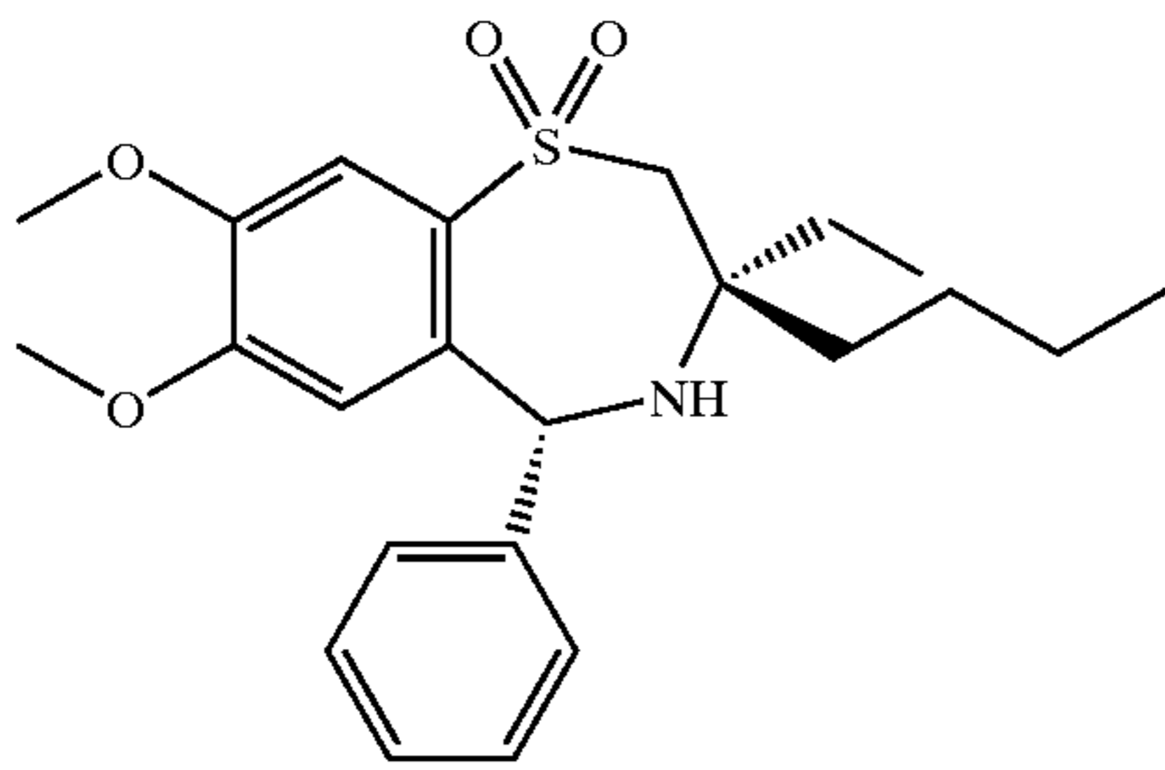
(3R,5R)-3-Butyl-3-ethyl-2,3,4,5-tetrahydro-7,8-dimethoxy-5-phenyl-1,4-benzothiazepine 1,1-Dioxide
