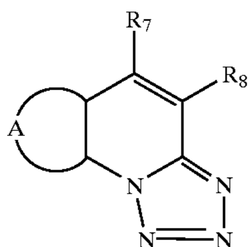
Intermediate Compound 4
