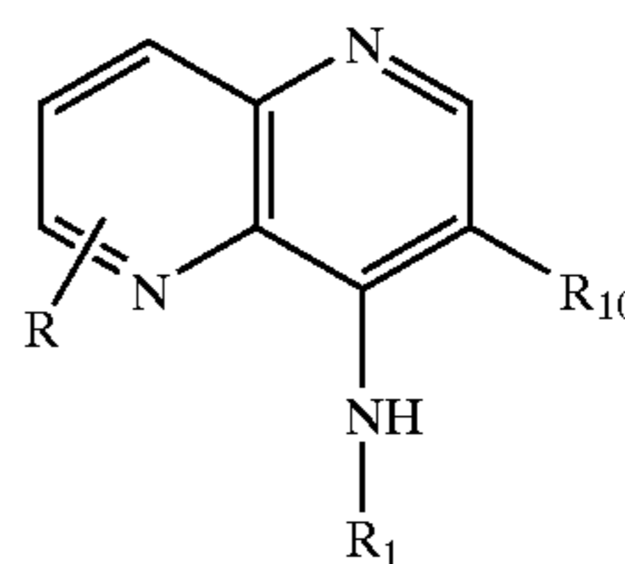
Intermediate Compound 6
