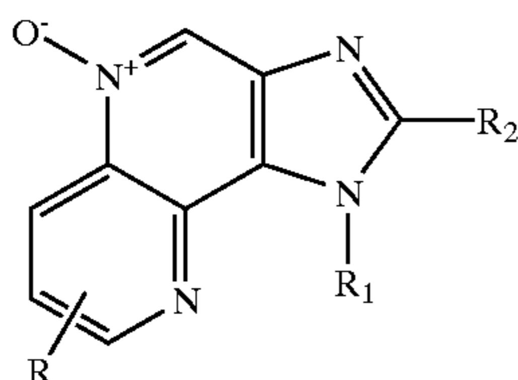
Intermediate Compound 3
