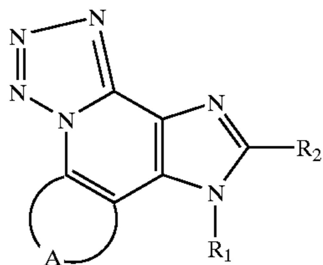
Intermediate Compound 1
