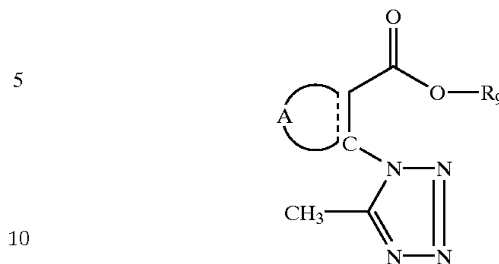
Intermediate Compound 5
