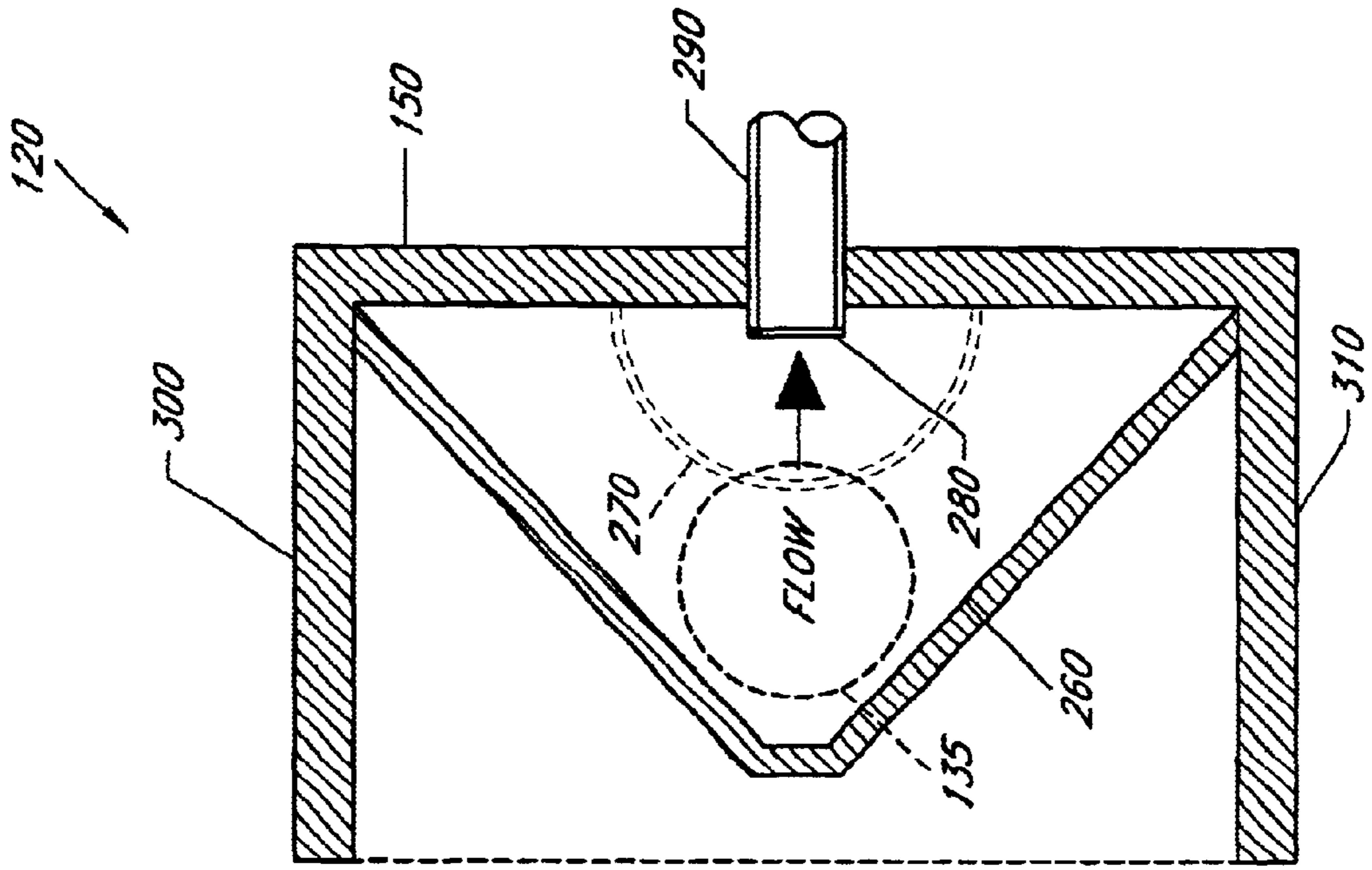
FIG 6: PLAN VIEW OUTLET DETAIL
