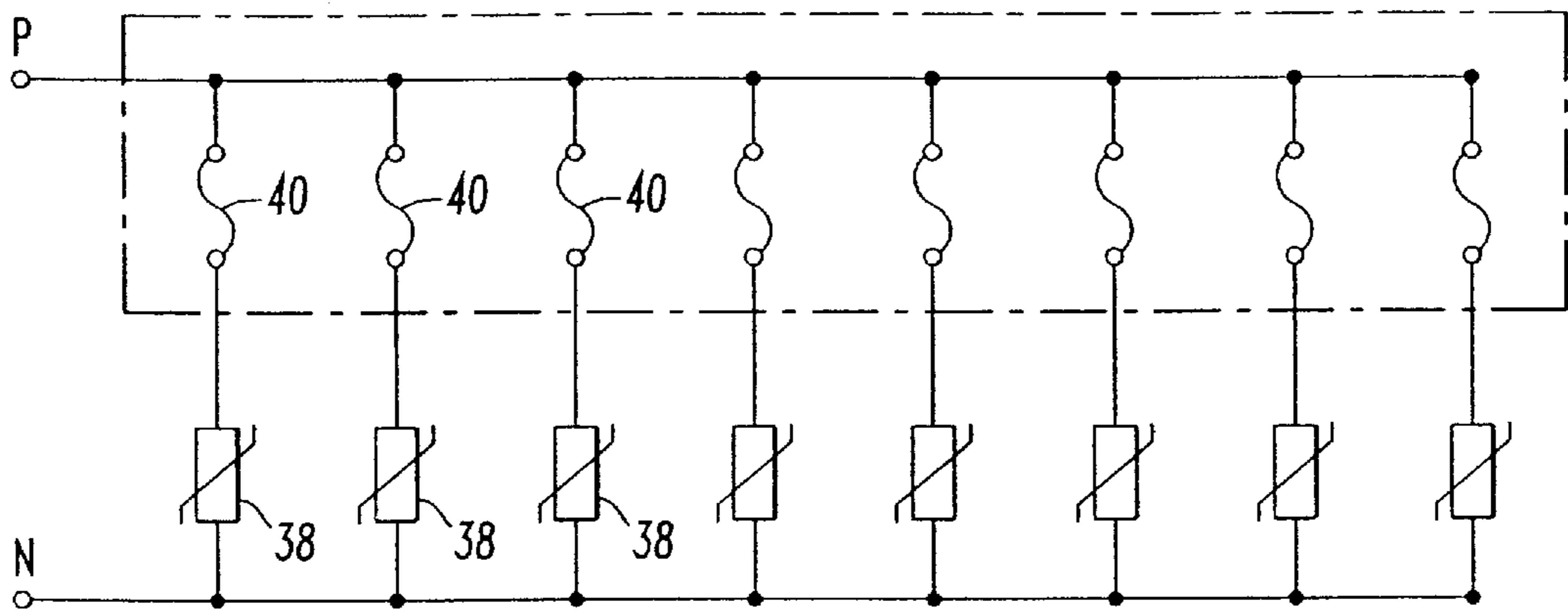
FIG. 2 PRIOR ART
