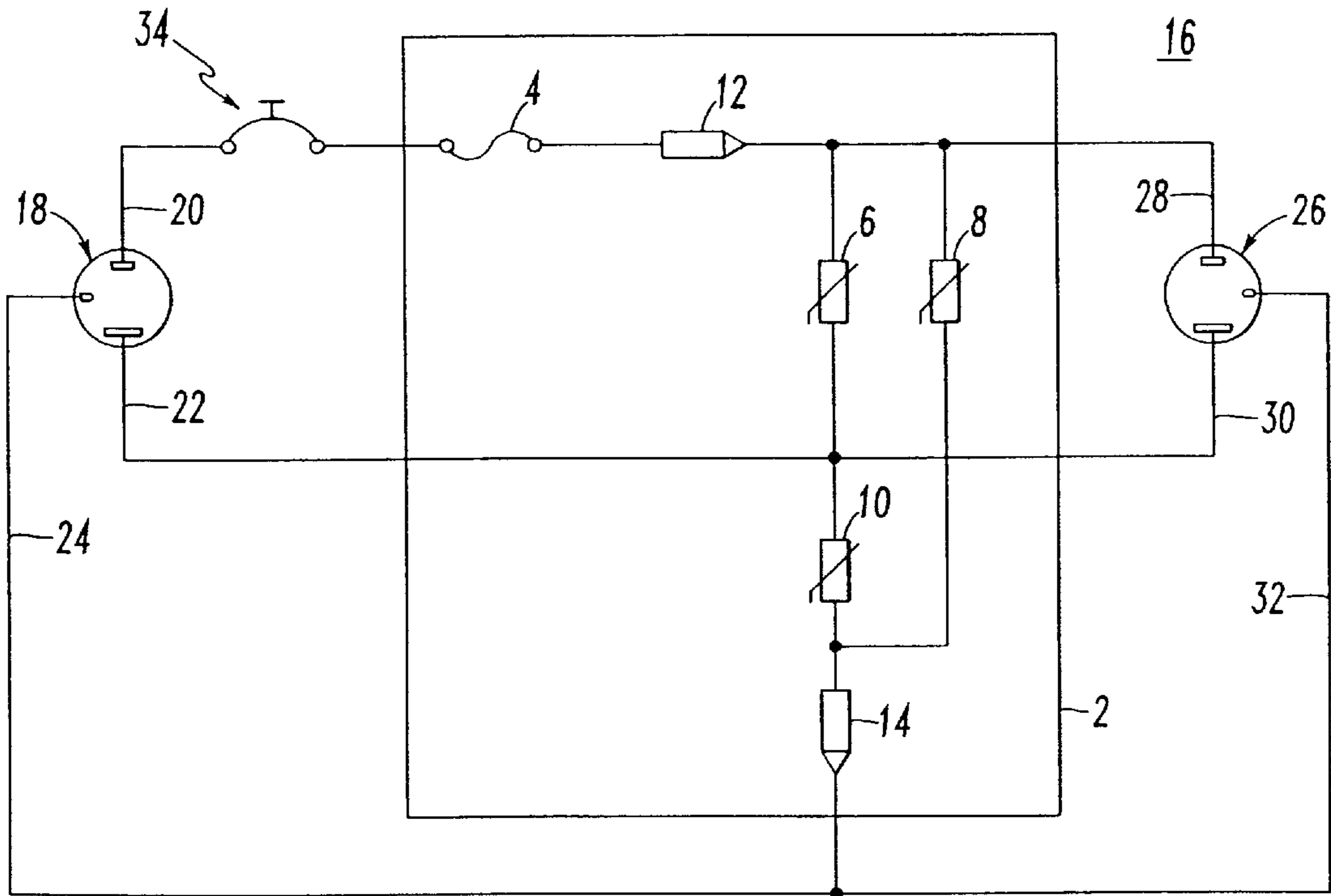
FIG. 1 PRIOR ART
