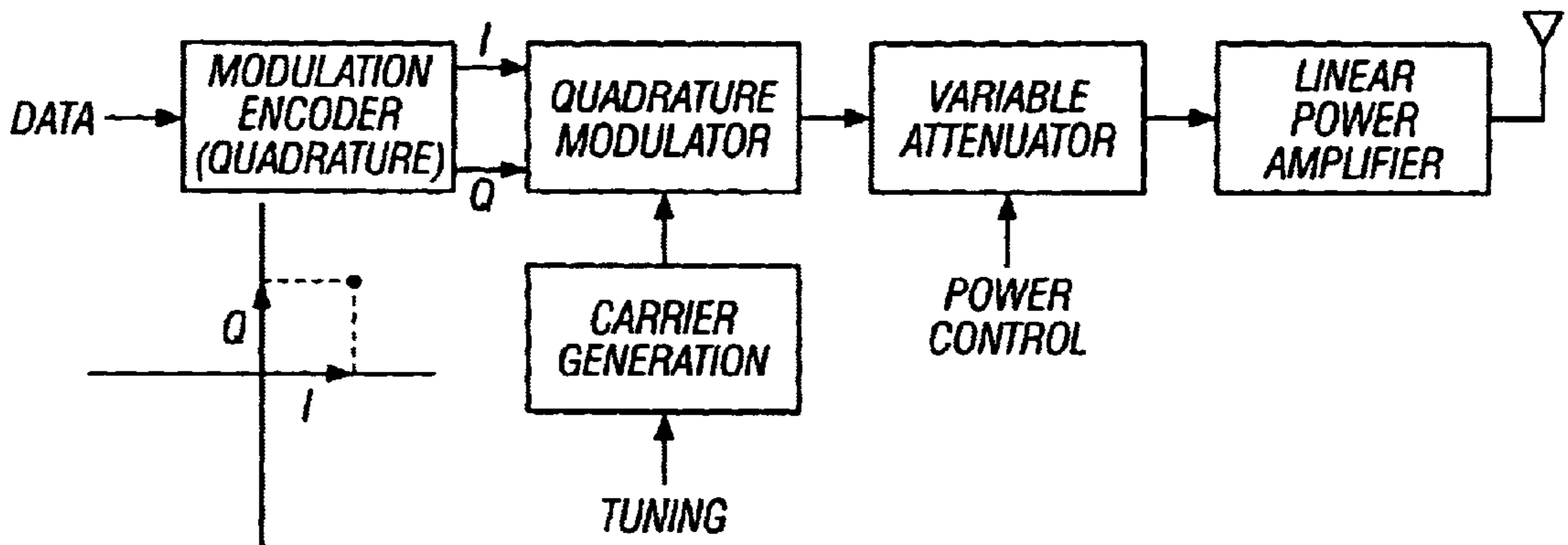
FIG. 6 (Prior Art)
