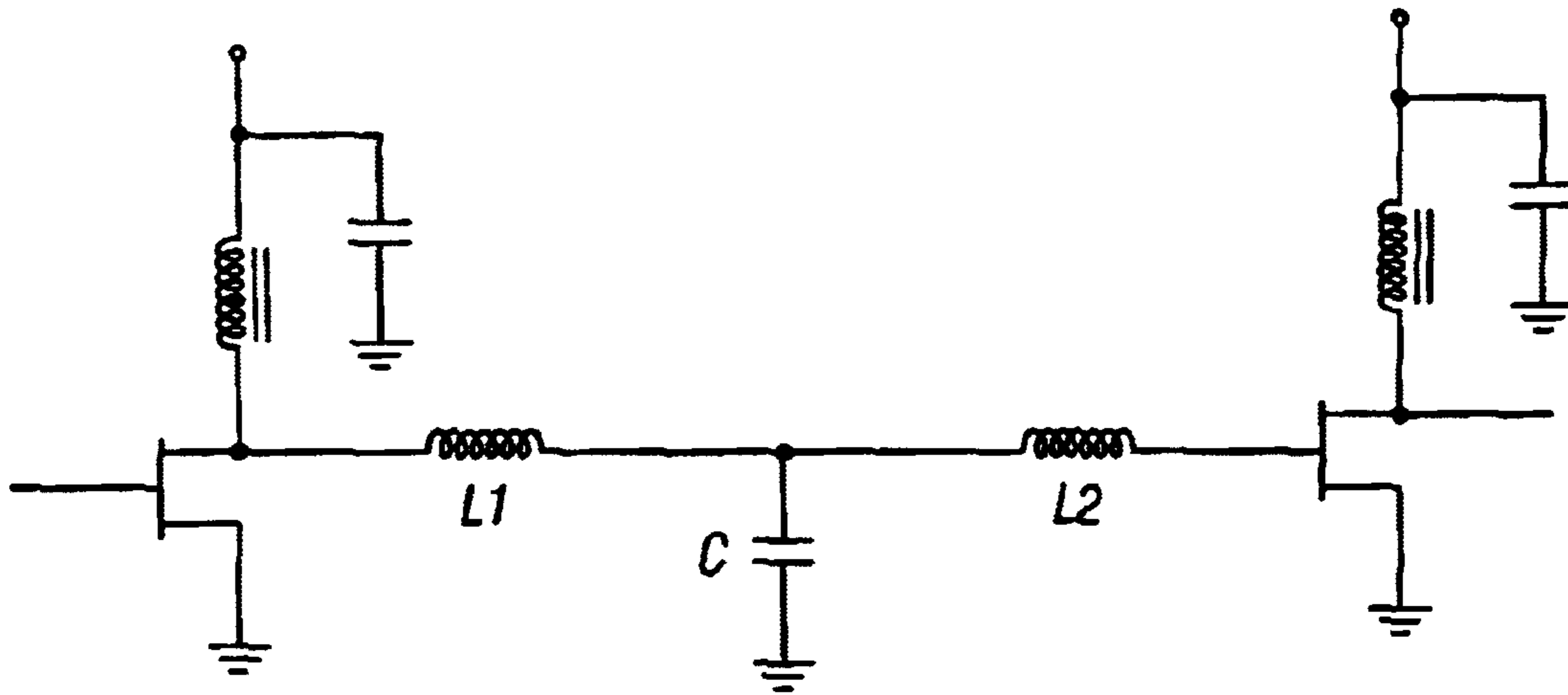
FIG. 4 (Prior Art)
