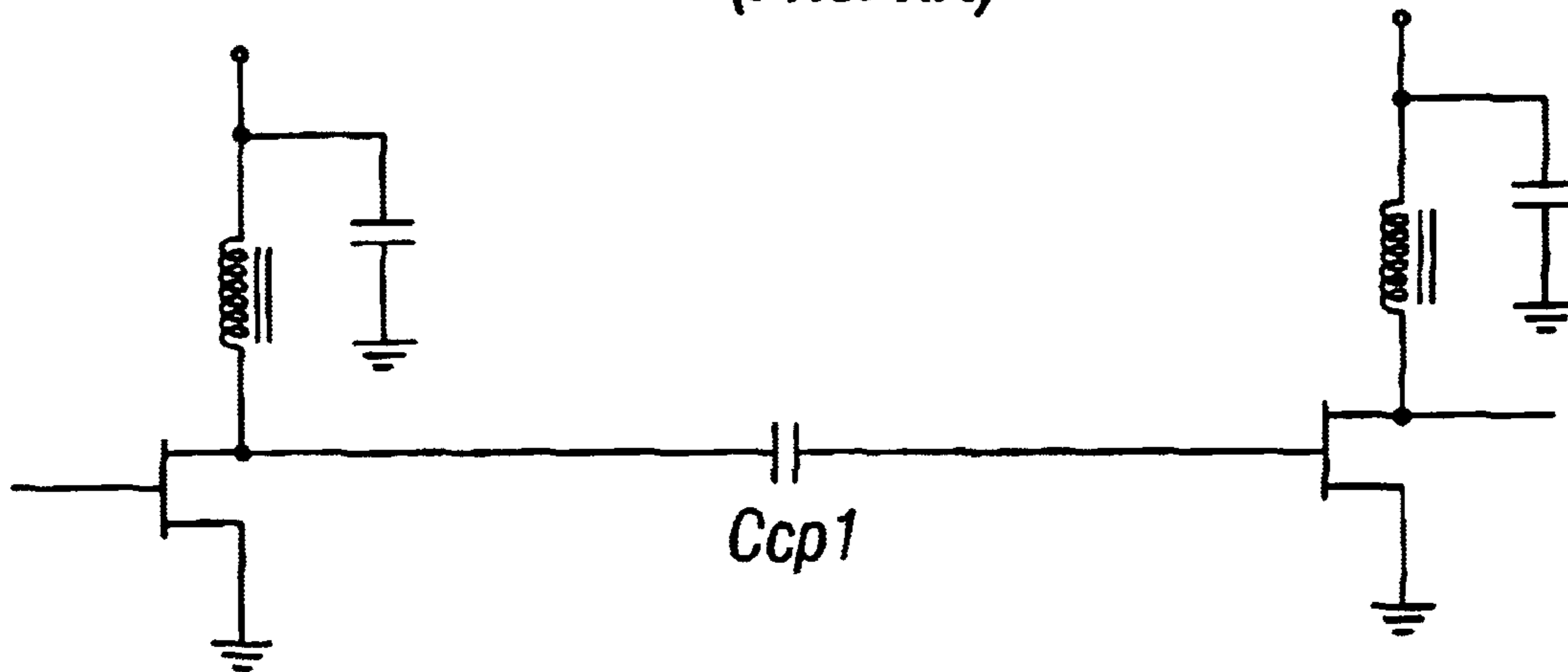
FIG. 5 (Prior Art)
