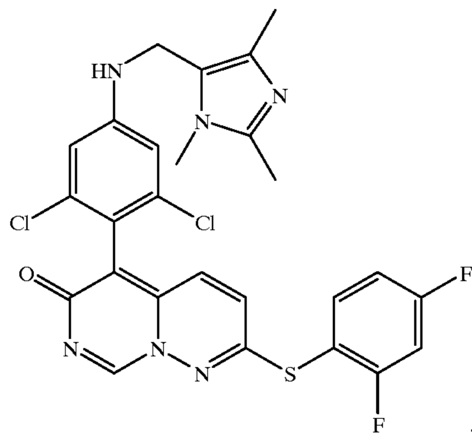
Compound 14
