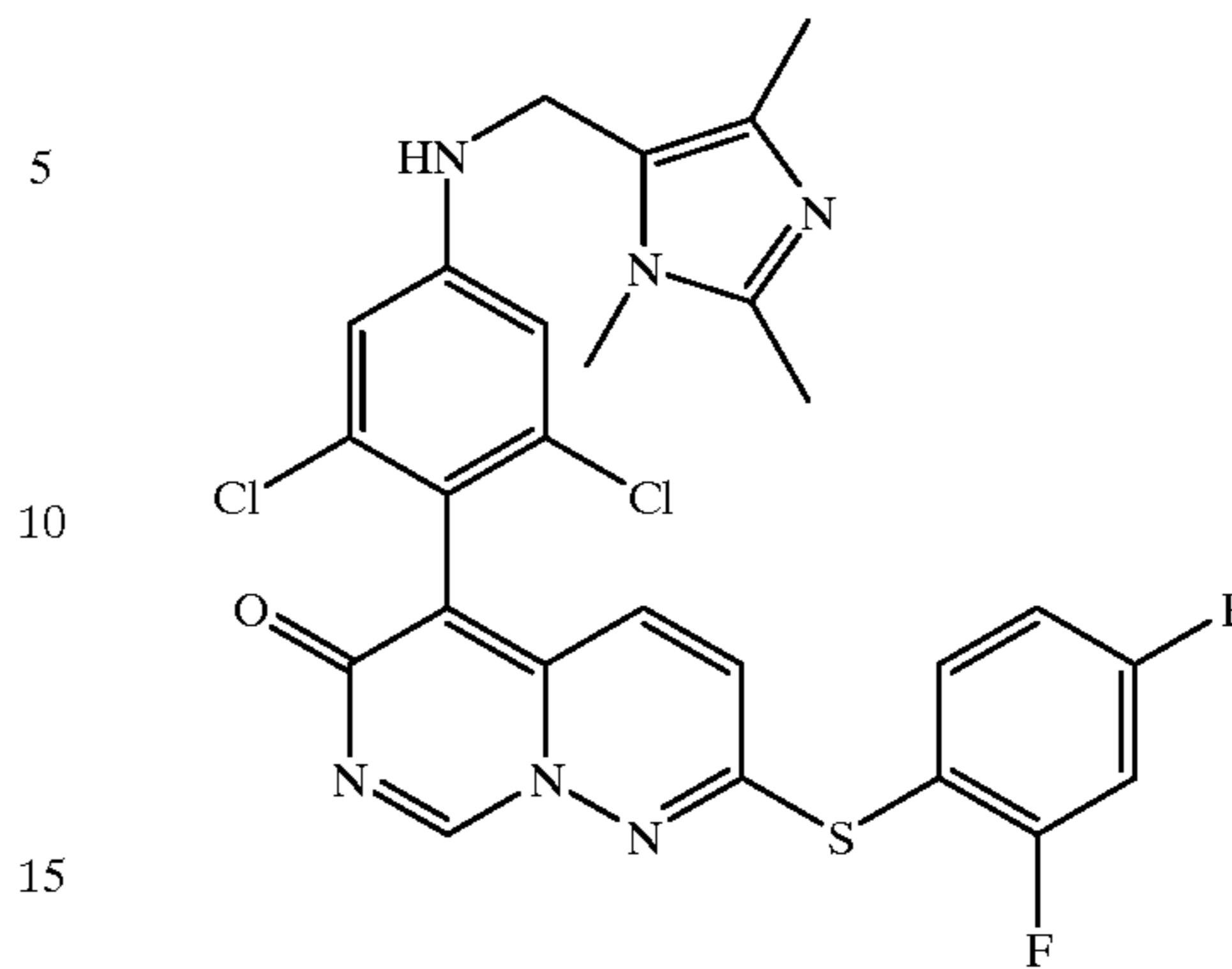
Compound 11
