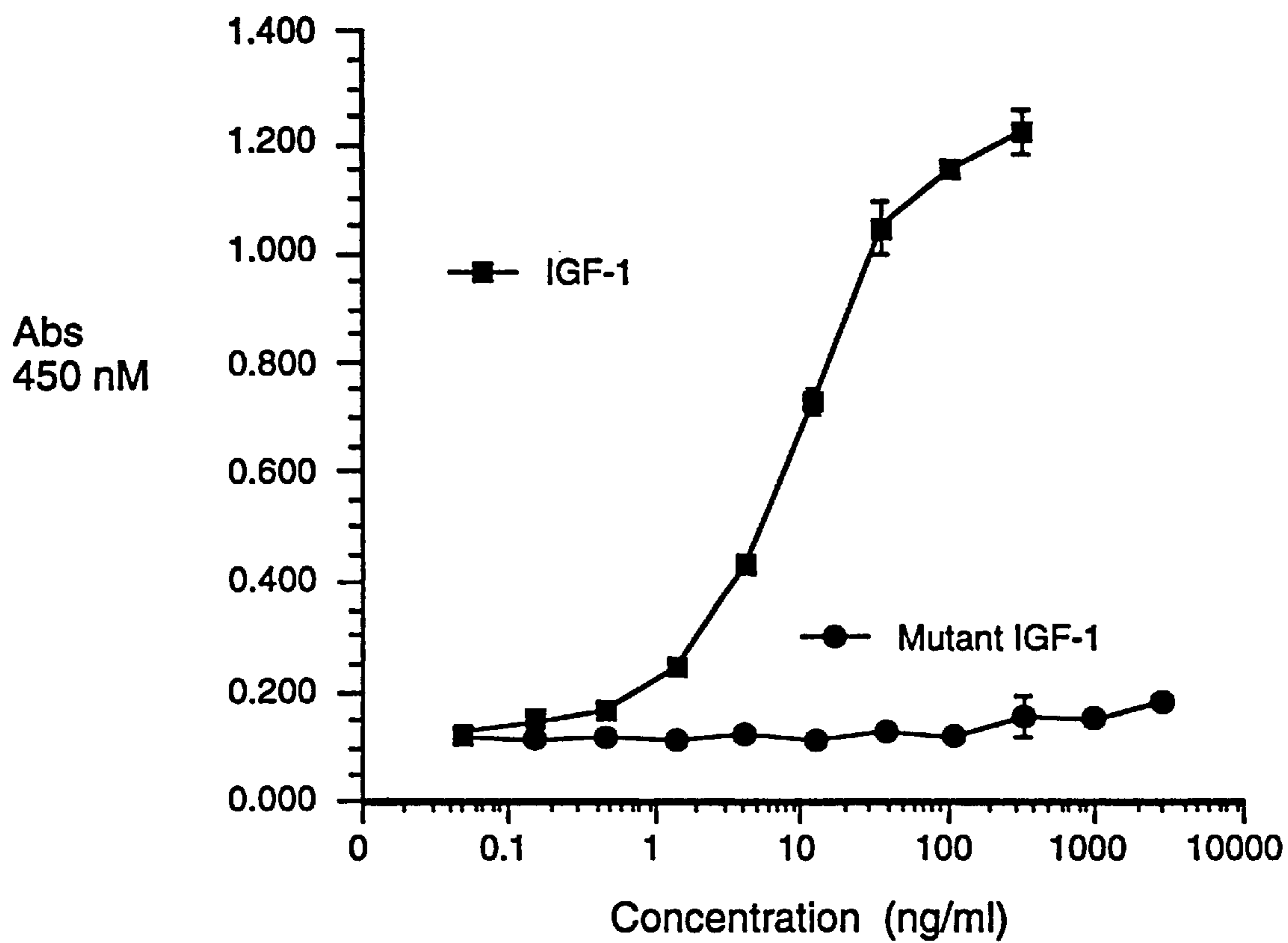
IGF-1 KIRA in Human MCF-7 Cells Comparison of IGF-1 and Mutant IGF-1
