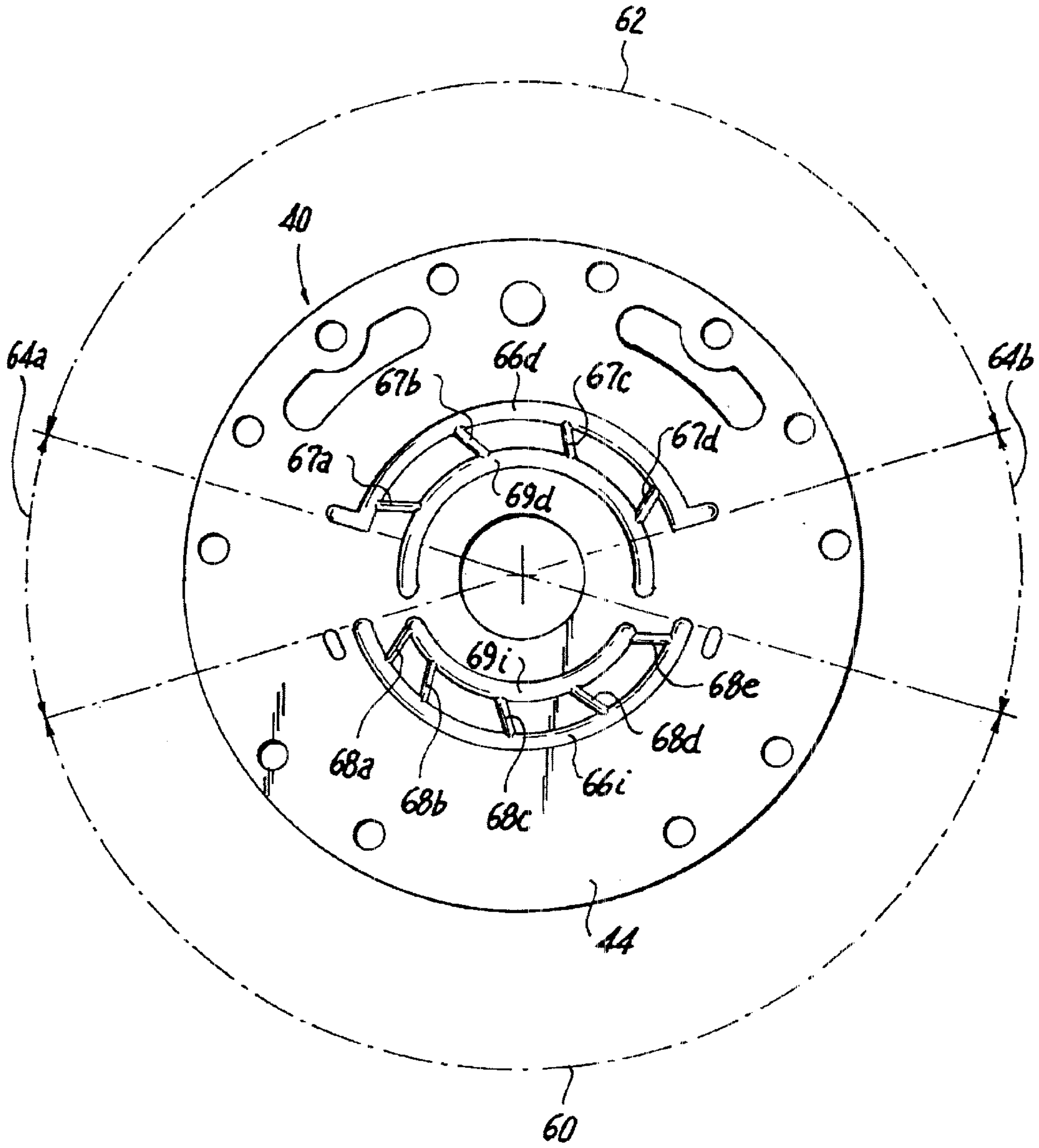
Fig. 3 (Prior Art)
