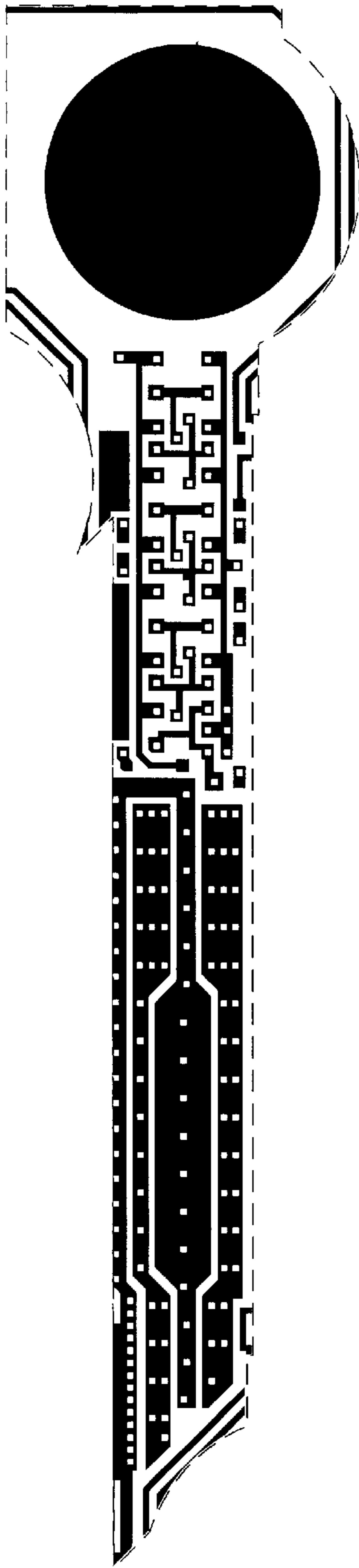
Metal 1 mask
