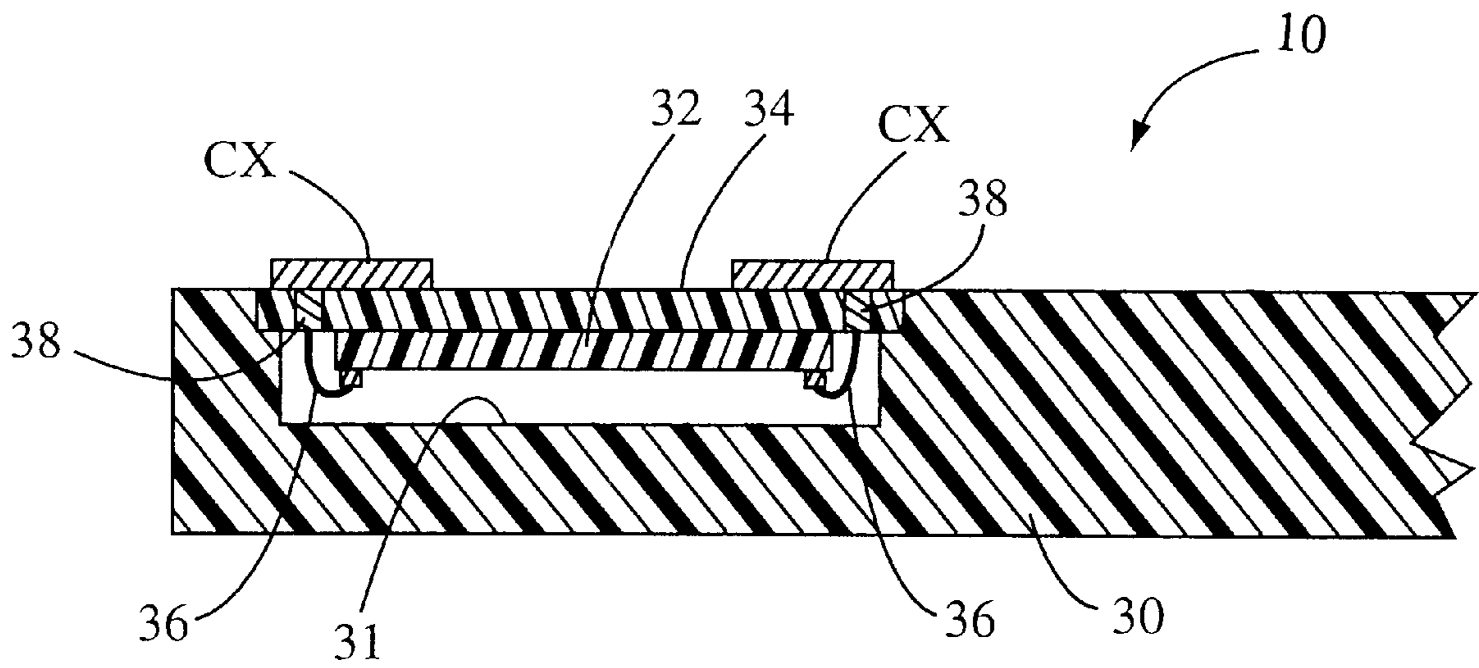
Fig. 3 (PRIOR ART)
